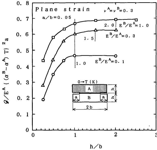
Fig.5.6 Effect of specimen size on energy release rate Q value in residual stress field.
