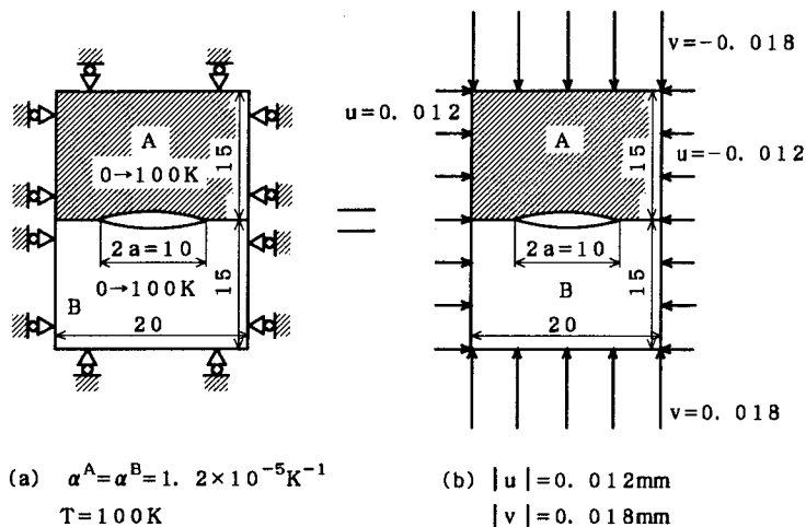
Fig.A.4 Two models for calculating Q value in residual stress field.
