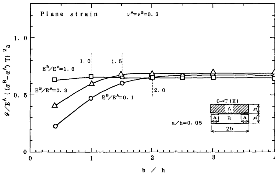
Fig.5.7 Effect of half width of specimen on energy release rate Q value in residual stress field.
