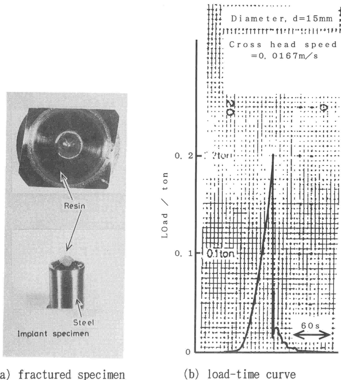
Fig.7.12 Experimental results of tension test using steel-resin joint.
