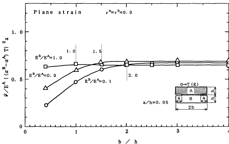
Fig.5.7 Effect of half width of specimen on energy release rate G value in residual stress field.
