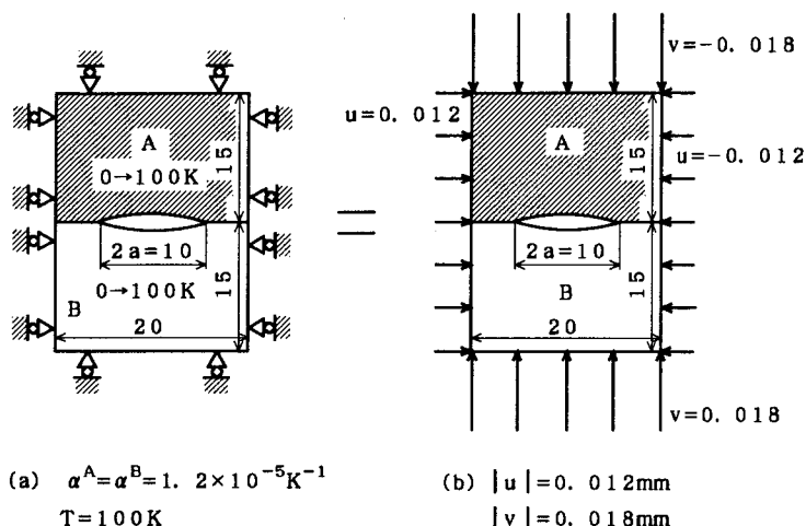
Fig.A.4 Two models for calculating Q value in residual stress field.
