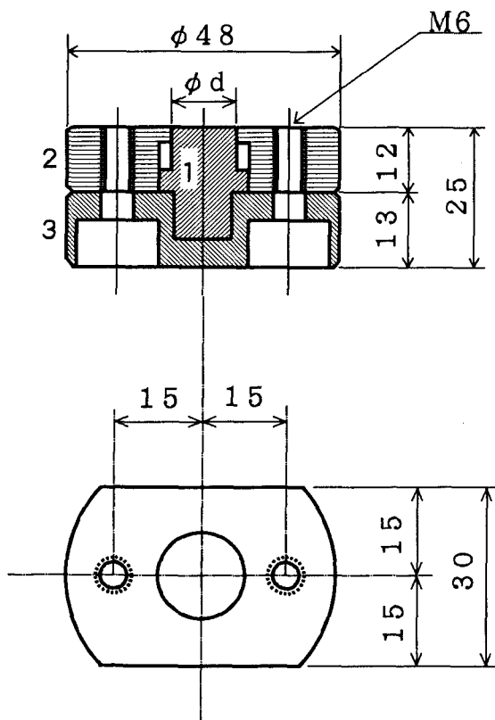
Fig.6.3 Torsional specimen.
