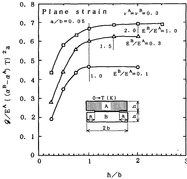
Fig.5.6 Effect of specimen size on energy release rate G value in residual stress field.
