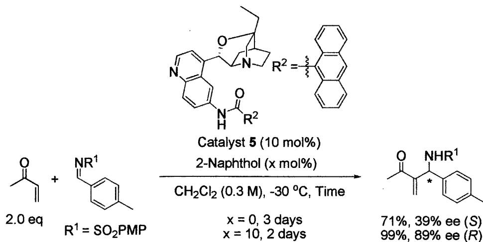
Scheme 1-22. Aza-MBH reaction using organocatalyst in the presence of acidic additives (Zhu)
