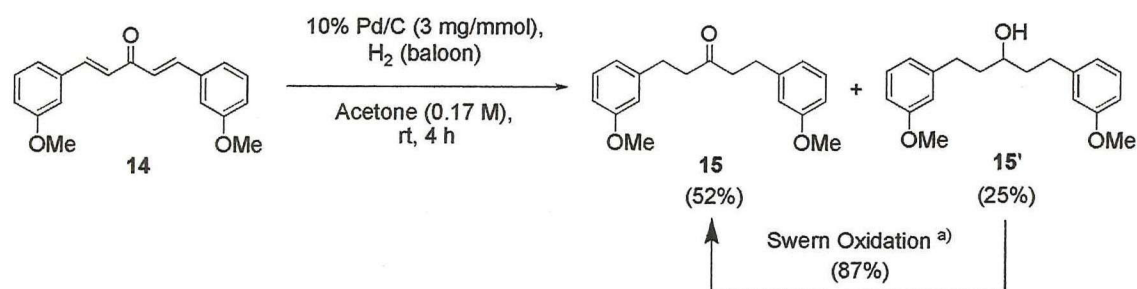
Scheme 2-2. Hydrogenation of 13 and bromination of 14 using alternative methods
