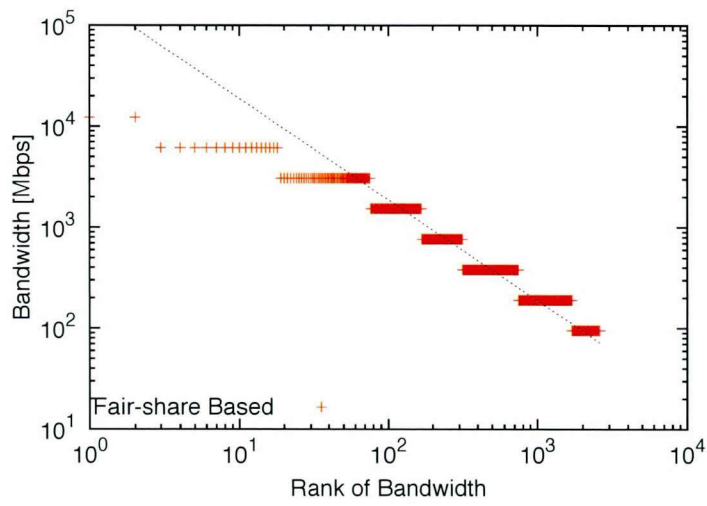
Figure 4.13: Bandwidth distribution obtained by simple bandwidth allocation
