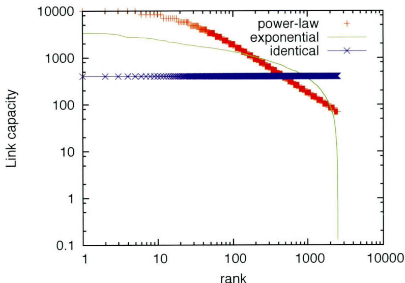
Figure 3.3: Normalized link bandwidth distributions
