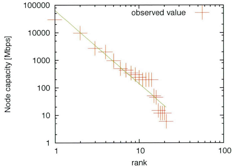
Figure 3.1: Node processing capacity distribution in the IJJ network
