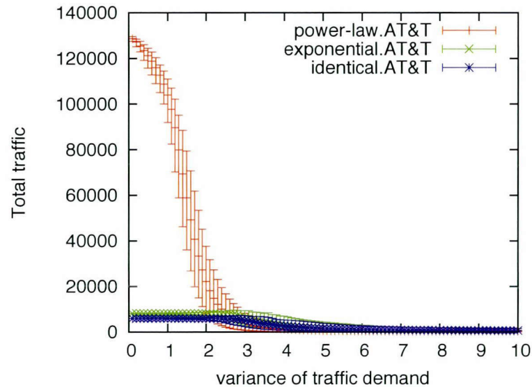
Figure 3.4: The amount of traffic that the AT&T topology can accommodate
