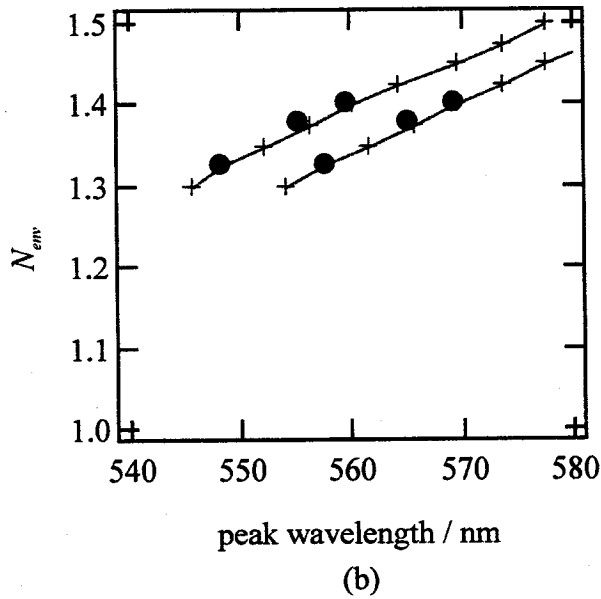
Fig. 4-1 Experimental (black lines) and calculated (gray lines) results of light scattering (a, upper) and extinction (a, lower) spectra of gold colloidal solution with N_{env} from 1.33 to 1.41. (b) Experimental (lower solid circles) and calculated (lower crosses with line) results of dependence on N_{env} upon peak wavelength of light scattering spectra. Experimental (upper solid circles) and calculated (upper crosses with line) results on dependence of N_{env} upon peak wavelength of light extinction spectra.
