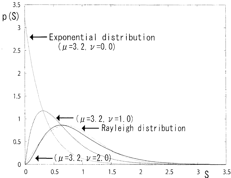
Figure 2.3: Curves of the parametric PDF.
