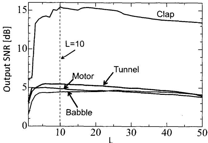
Figure 4.4: Practical wide-band noise suppression results for various L with Input SNR=0dB.
