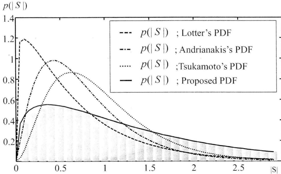
Figure 3.4: Speech histogram in 49-50 dB SNR interval and speech PDFs which are Lotter's PDF [3] (dashed line), Andrianakis's PDF [4] (dotted-dash line), Tsukamoto's PDF [5] (dotted line), and proposed PDF (solid line).
