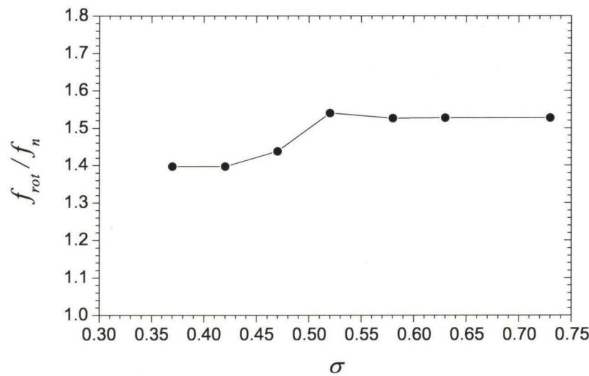
Fig. 5.8: Relation between cavitation number and rotation cavitation frequency
