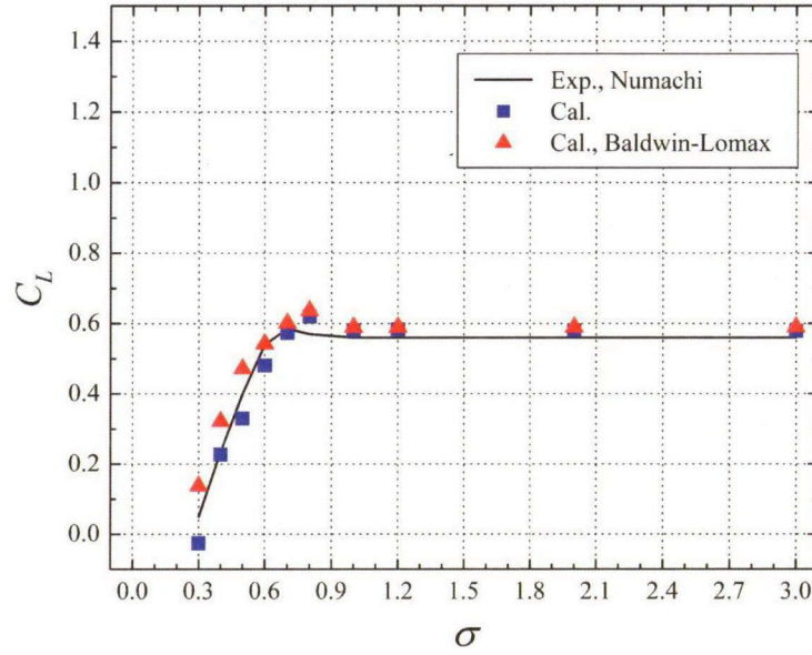
Fig. 3.3: Variations of lift coefficients C_L as function of cavitation number \sigma at \alpha = 2^\circ
