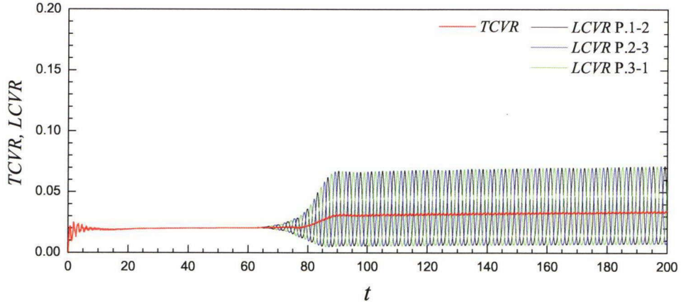
Fig. 7.4: Time evolution of cavity volume rate ( \phi_{ini} = 0.241 , \sigma = 0.42 , L_p = 500C )
