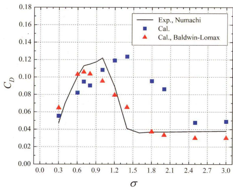
Fig. 3.6: Variations of drag coefficients as function of cavitation number at \alpha = 8^\circ
