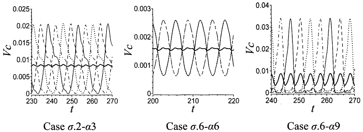
Fig. 4.6: Influence of \sigma and \alpha on time evolution of cavitation volume in each passage of 4-blades cascade (solid lines: P.1-2; dash lines: P.2-3; dot lines: P.3-4; dash-dot lines: P.4-1; bold lines: average)
