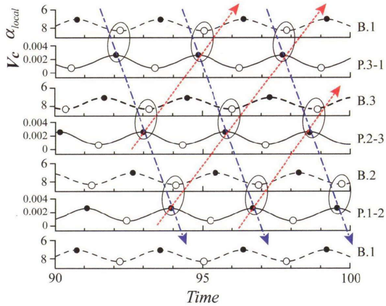
Fig. 4.5: Time evolutions of local flow angle (dash lines) and cavity volume (solid lines) in each passage of N = 3 ; Case \sigma.6 - \alpha 6 )
