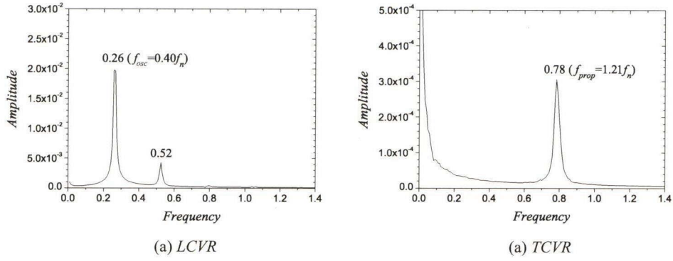
Fig. 7.5: Frequency analysis of cavity volume rate ( \phi_{ini} = 0.241 , \sigma = 0.42 , L_p = 500C )
