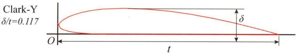
Fig. C1: Clark-Y 11.7% hydrofoil
