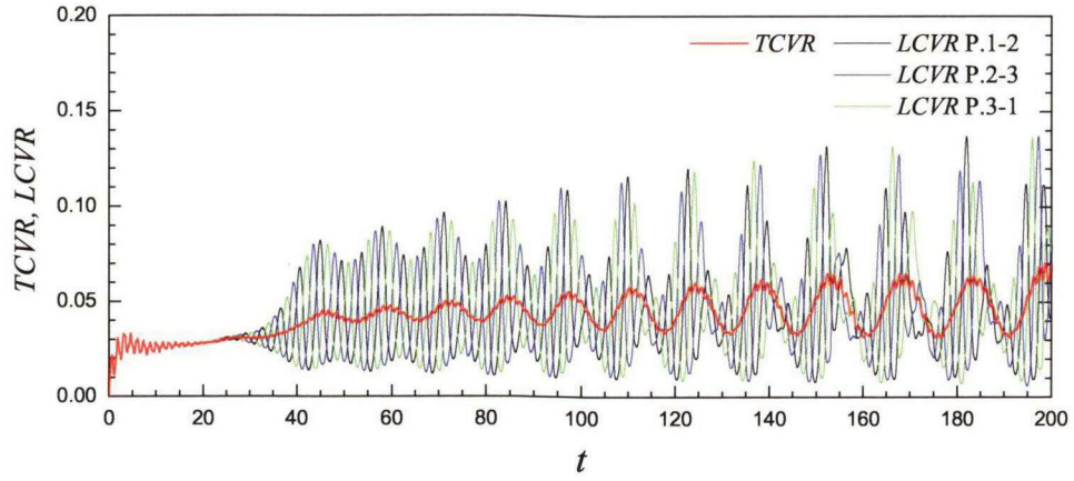
Fig. 7.7: Time evolution of cavity volume rate ( \phi_{ini} = 0.241 , \sigma = 0.42 , L_p = 20C )
