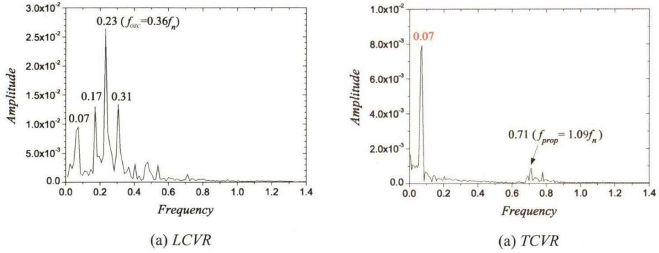
Fig. 7.8: Frequency analysis of cavity volume rate ( \phi_{ini} = 0.241 , \sigma = 0.42 , L_p = 20C )
