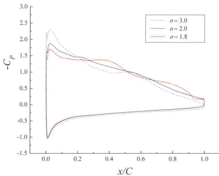
Fig. 3.8: Comparisons of pressure coefficient around a hydrofoil without the turbulence model at \alpha = 8^\circ
