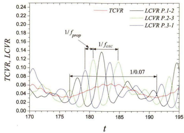
Fig. 7.9: Cavity volume rate and fluctuating period ( \phi_{ini} = 0.241 , \sigma = 0.42 , L_p = 20C )
