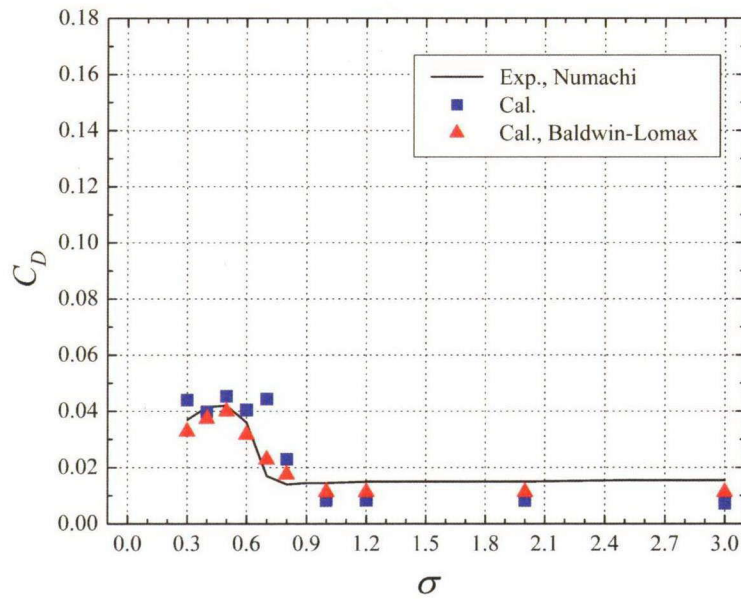
Fig. 3.4: Variations of drag coefficients C_D as function of cavitation number \sigma at \alpha = 2^\circ
