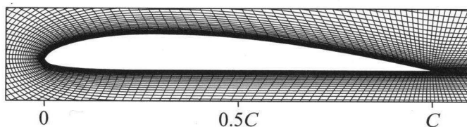
Fig. 3.2: Grid around a 2D Clark-Y 11.7% hydrofoil
