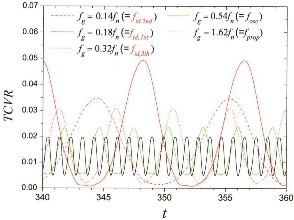
Fig. 6.1: Time evolution of TCVR at each forcing mode of inflow fluctuation
