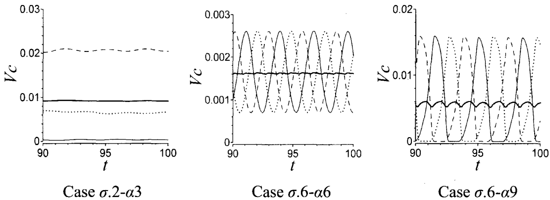
Fig. 4.3: Influence of \sigma and \alpha on time evolution of cavitation volume in each passage of 3-blades cascade (solid lines: P.1-2; dash lines: P.2-3; dot lines: P.3-1; bold lines: average)
