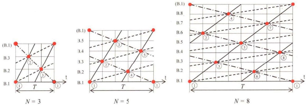
Fig. 4.7: Chart for propagations of maximum cavitation(●): trigger (‘-1’, dash lines), basic mode (‘-2’, solid lines) and forward rotation (‘+1’, dash-dot lines)
