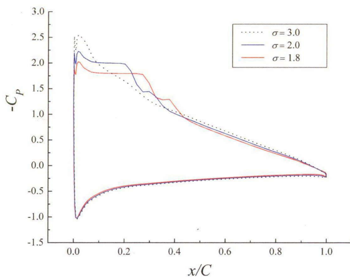
Fig. 3.9: Comparisons of pressure coefficient around a hydrofoil with the turbulence model at \alpha = 8^\circ
