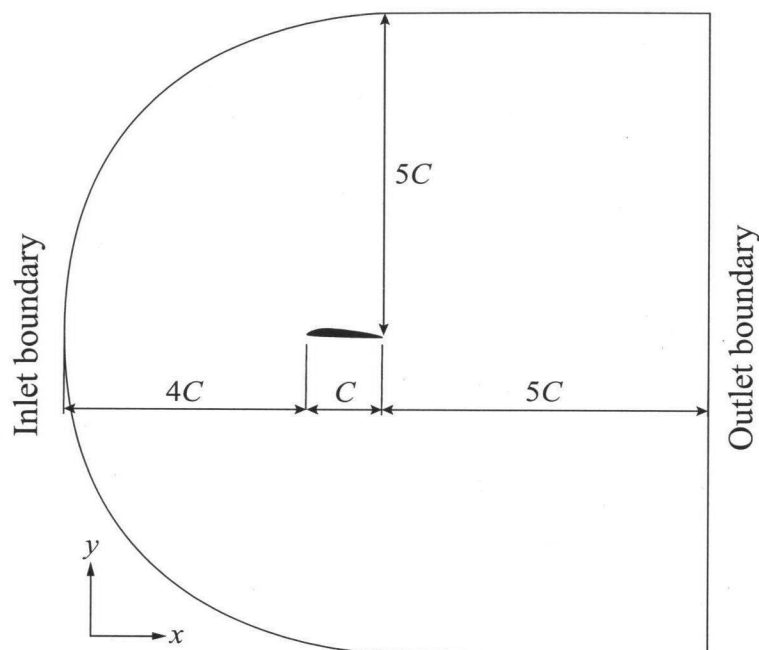
Fig. 3.1: Computational domain around a 2D Clark-Y 11.7% hydrofoil (applied C-type grid system)
