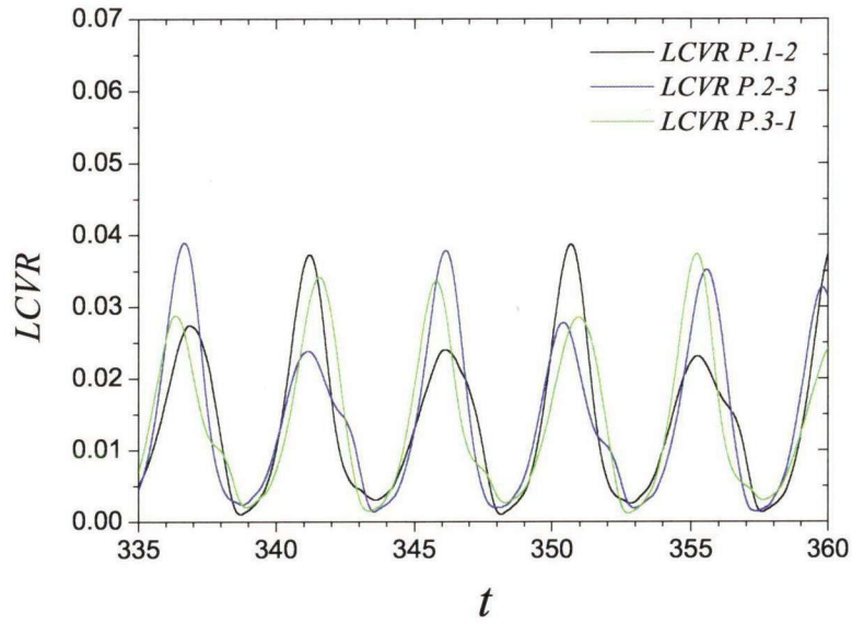
Fig. 6.4: Time evolution of local cavity volume rate for inflow fluctuation with f_{id,3th}
