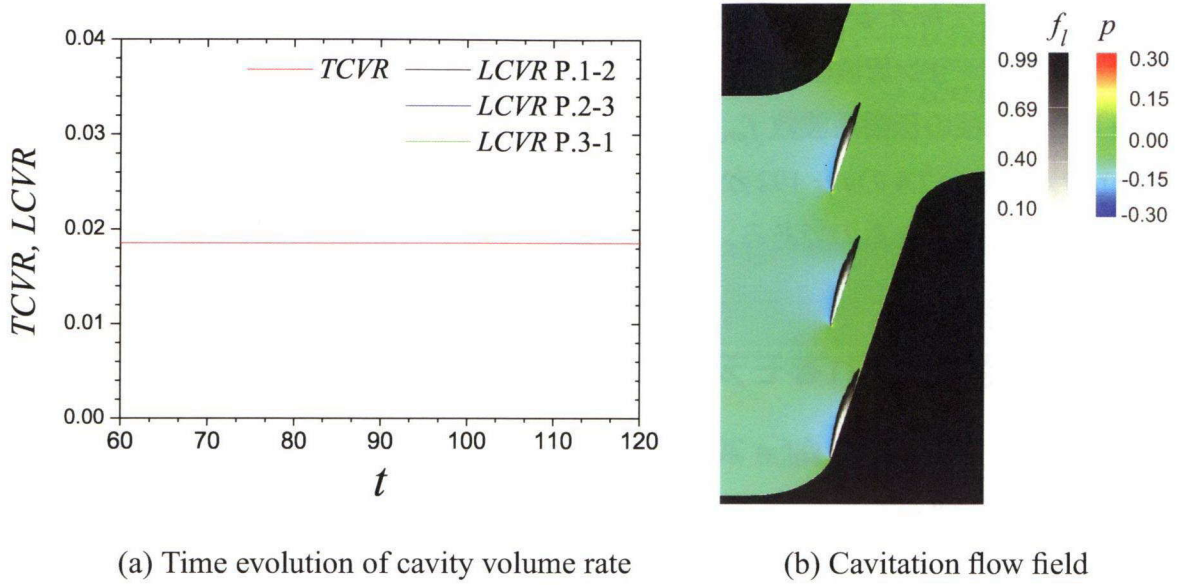
Fig. 7.3: Time evolution of cavity volume rate and flow field generated quasi-steady partial cavitation on steady inflow ( \sigma = 0.42 , \alpha = 5^\circ , TCVR and LCVR \approx 0.019 )
