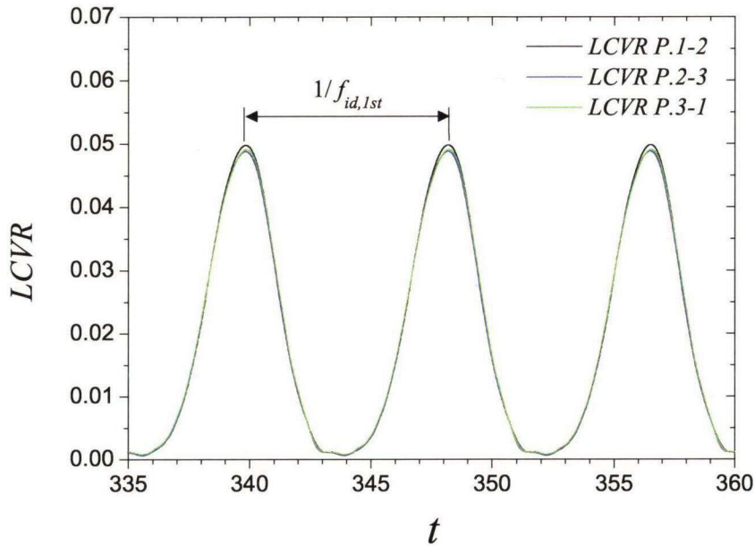
Fig. 6.2: Time evolution of local cavity volume rate for inflow fluctuation with f_{id,1st}
