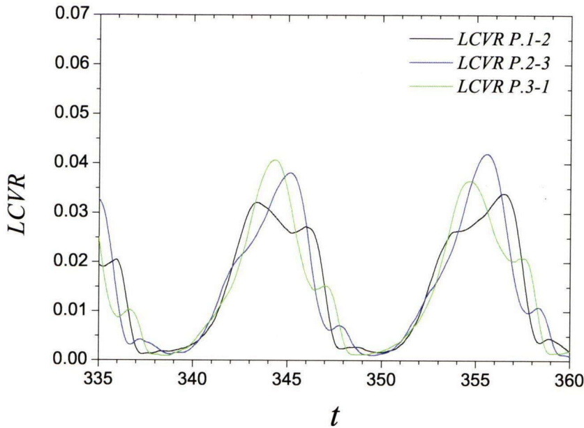
Fig. 6.3: Time evolution of local cavity volume rate for inflow fluctuation with f_{id,2nd}
