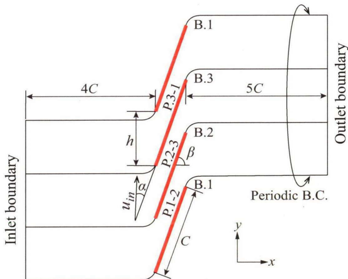
Fig. 5.1: Computational domain including 3-blades cascade (H-type grid)
