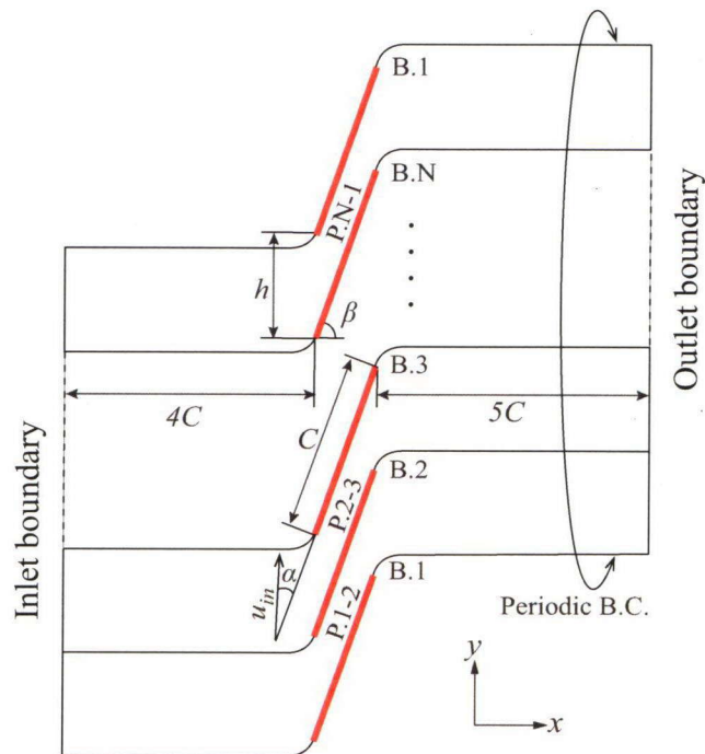
Fig. 4.2: Computational domain including cascade
