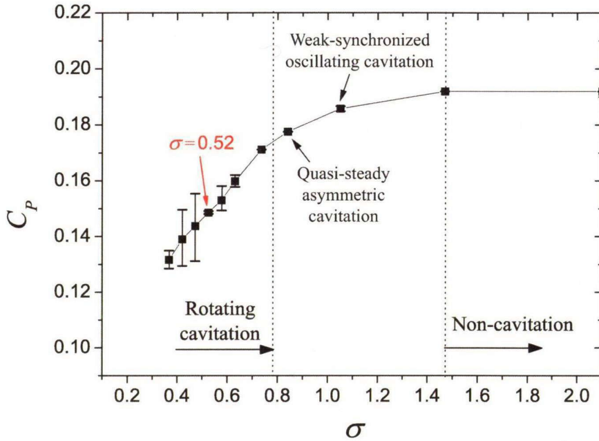
Fig. 5.3: Pressure coefficient C_p as a function of the cavitation number \sigma at the angle of attack \alpha = 6^\circ
