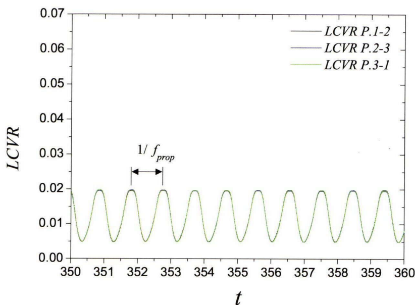
Fig. 6.6: Time evolution of local cavity volume rate for inflow fluctuation with f_{prop}
