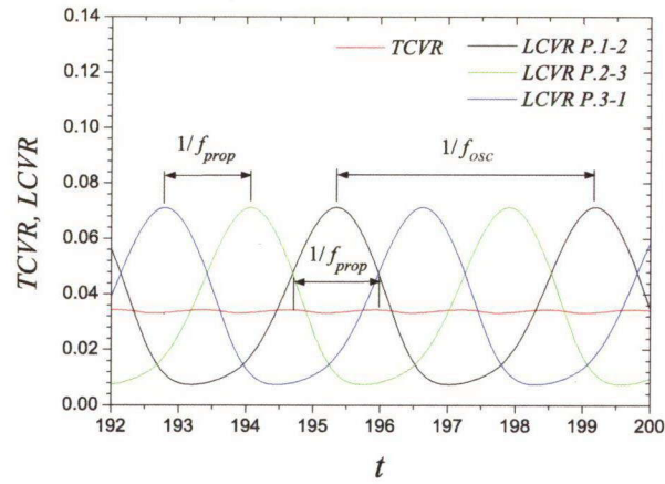
Fig. 7.6: Cavity volume rate and fluctuating period ( \phi_{ini} = 0.241 , \sigma = 0.42 , L_p = 500C )
