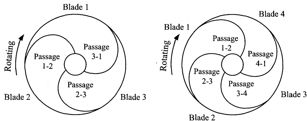
Fig. 4.1: 3-blades (left) and 4-blades (right) inducer of turbo-pump in rocket engine
