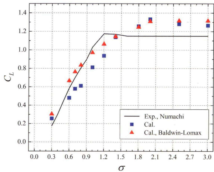
Fig. 3.5: Variations of lift coefficients as function of cavitation number at \alpha = 8^\circ
