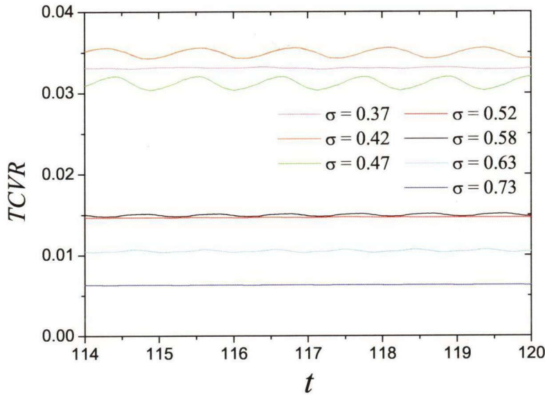
Fig. 5.5: Time evolution of TCVR for each cavitation number
