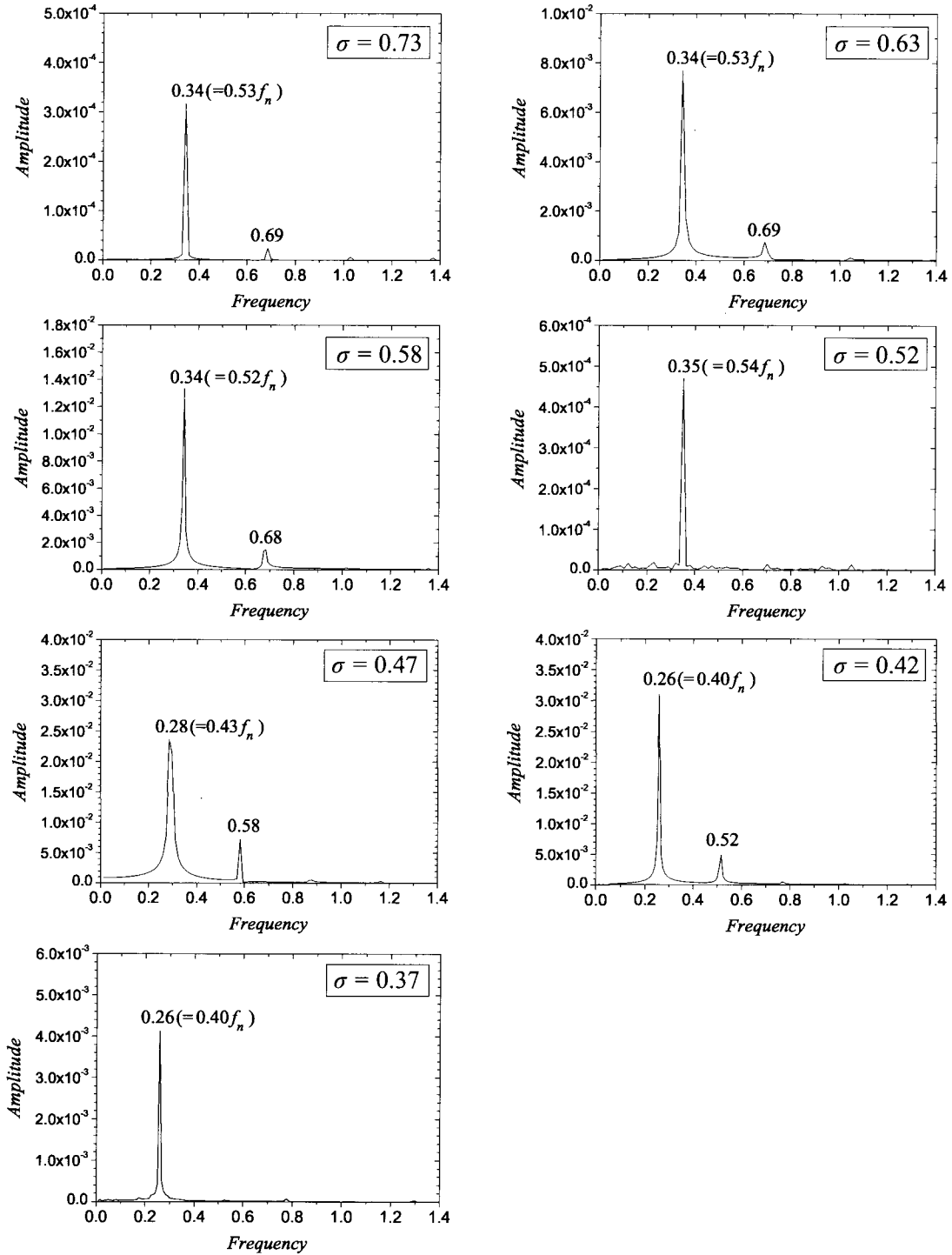
Fig. 5.6: Frequency analysis of LCVR in case of rotation cavitation mode
