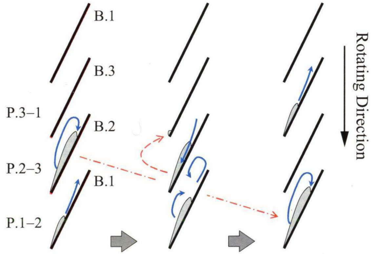
Fig. 4.4: Typical pattern of cavity propagation (solid lines: flow; dash lines: trigger; dash-dot lines: transfer)
