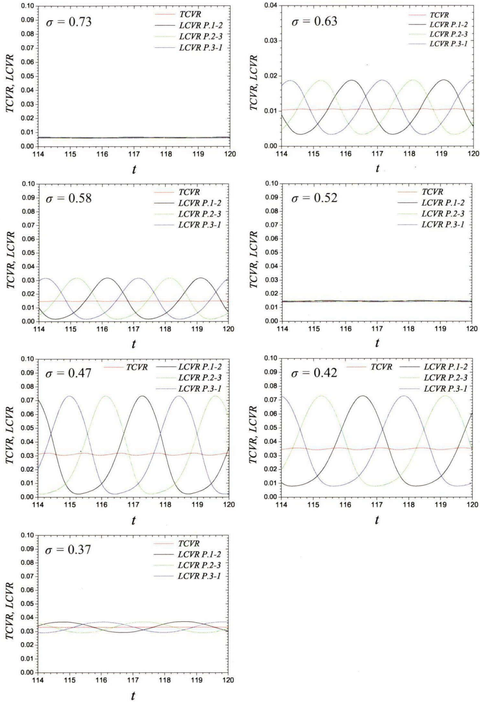
Fig. 5.4: Time evolution of cavity volume rate in case of rotation cavitation mode
