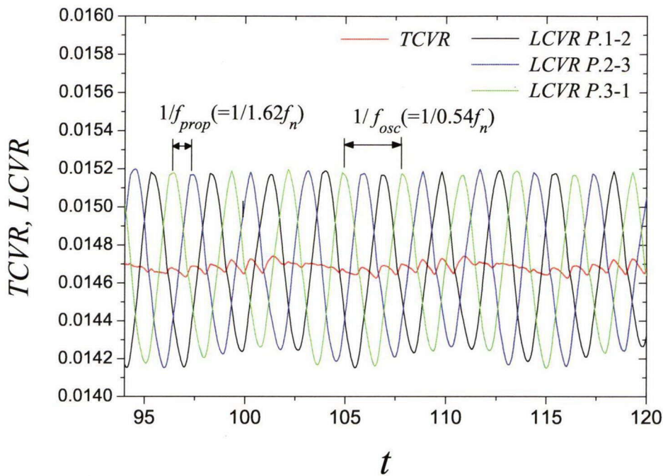
Fig. 5.10: Time evolution of cavity volume rate for each cavitation number at \sigma = 0.52
