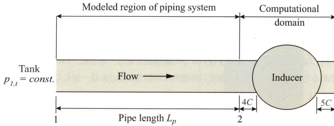
Fig. 7.1: Schematic of pumping system including a tank and a pipe
