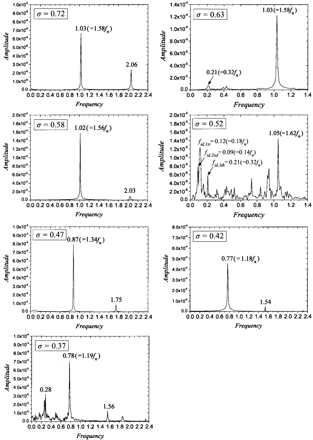
Fig. 5.9: Frequency analysis of TCVR in case of rotation cavitation mode
