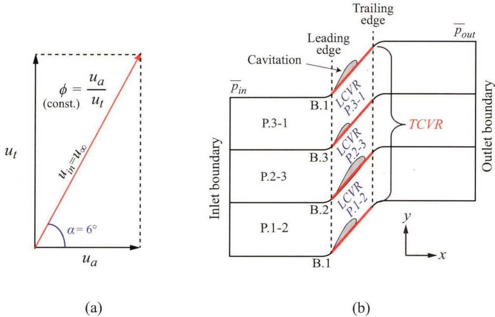
Fig. 5.2: Schematic for each coefficient definition; (a) flow coefficient (b) pressure coefficient and cavity volume rate
