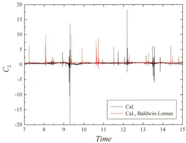
Fig. 3.11: Time evolution of lift coefficients at \alpha = 8^\circ and \sigma = 0.6
