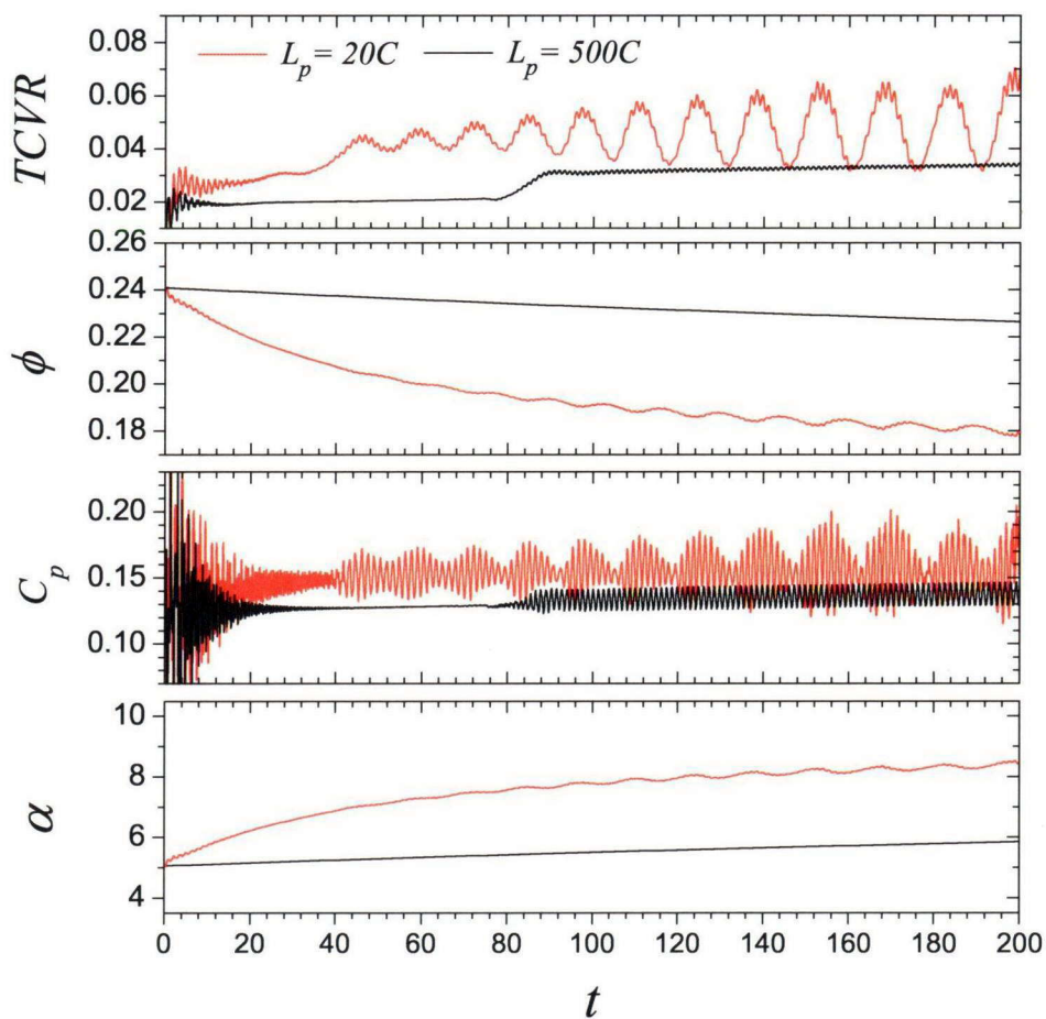
Fig. 7.10: Time evolution of total cavity volume rate TCVR , flow rate coefficient \phi and pressure coefficient C_p , angle of attack \alpha for L_p = 20C and 500C ( \phi_{ini} \approx 0.241 , \sigma = 0.42 )
