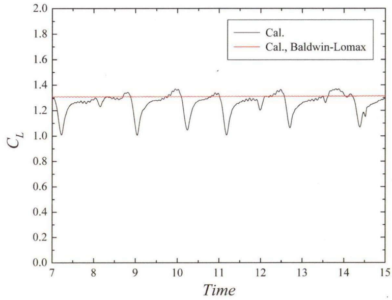
Fig. 3.10: Time evolution of lift coefficients at \alpha = 8^\circ and \sigma = 3.0
