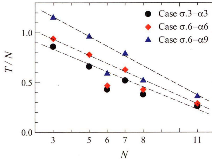
Fig. 4.8: Period of rotating cavitation
