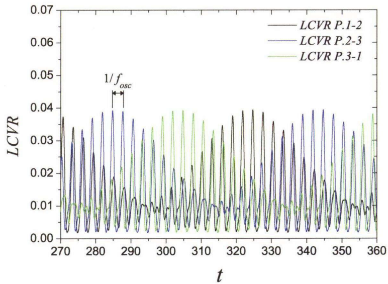
Fig. 6.5: Time evolution of local cavity volume rate for inflow fluctuation with f_{osc}
