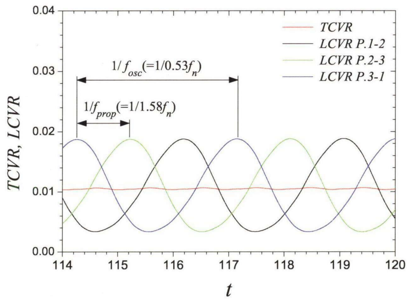
Fig. 5.7: Cavity volume rate and fluctuating period at \sigma = 0.63
