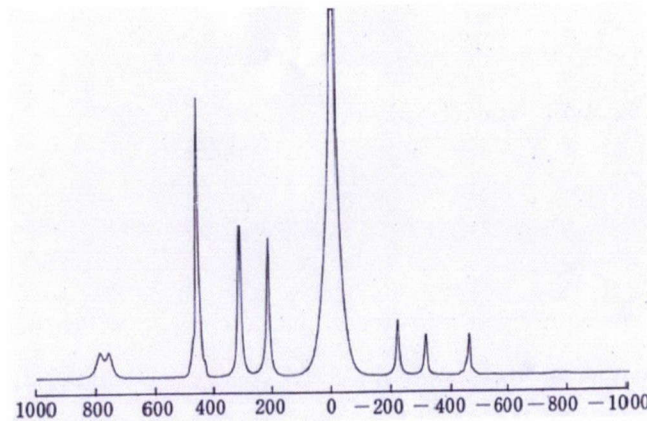
Figure 1-2 Raman spectrum of carbon tetrachloride [1]. Peaks by Stokes Raman scattering, Rayleigh scattering, and anti-Stokes Raman scattering are observed at above 0cm -1 , 0 cm -1 and below 0 cm -1 , respectively.
