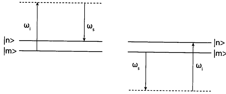
Figure 1-4 Processes of Raman scattering expressed by Eq. 1-12. A: Raman scattering generates after the excitation of energy level of a molecule. B: Raman scattering generates before the excitation of energy level of a molecule.
