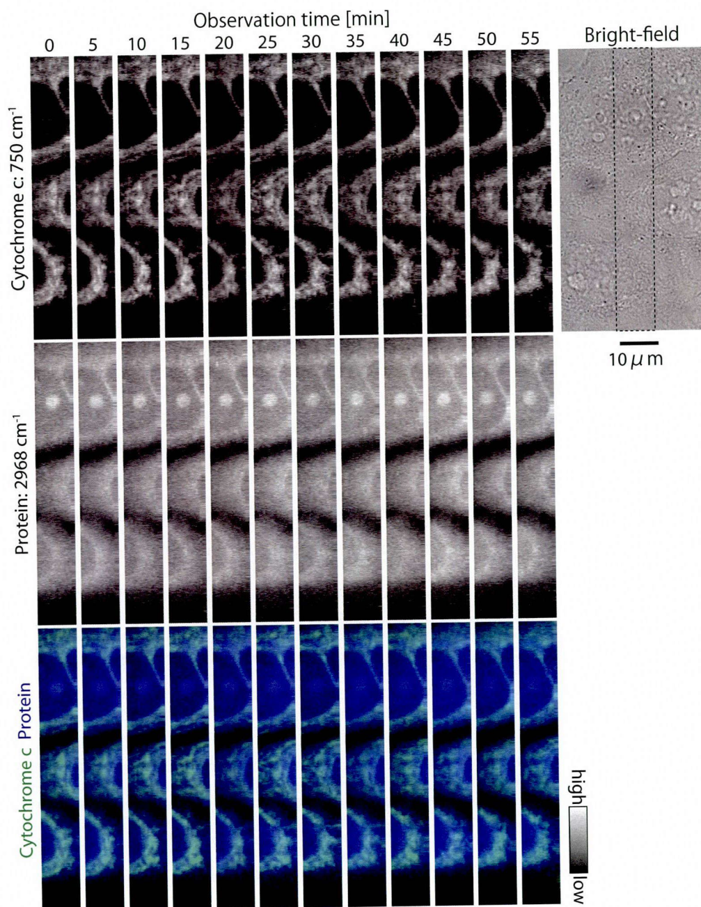
Figure 2-19B Time-lapse Raman images of living HeLa cells. Both cytochrome c and protein did not change in their distributions through the observation. The excitation laser intensity was 1.5 mW/μm² and the exposure time was 1.5 seconds per line. The images
