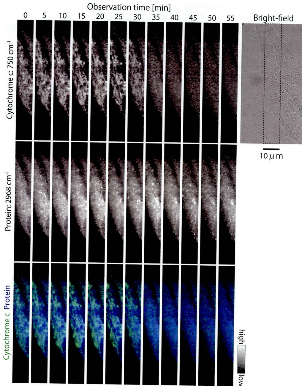
Figure 2-19A Time-lapse Raman images of apoptotic HeLa cell. The area indicated with the dotted line in the bright-field image was observed. Raman images of cytochrome c (750 \text{cm}^{-1} ), protein (2968 \text{cm}^{-1} ) and overlay of them are shown. The images were obtained at 5 minutes intervals with a frame rate of 80 seconds/image. At 30 minutes, cytochrome c started to be released from mitochondria. Protein shows the shape of the cell and the distribution did not change through the observation. The excitation laser intensity was 1.5 \text{mW}/\mu\text{m}^2 and the exposure time was 1.5 seconds per line. The images consist of 360 \times 20 pixels. The slit was set to 50 \mu\text{m} .
