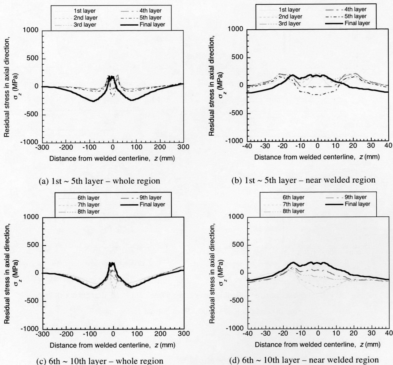
Fig. 6.15 Axial residual stress distribution at inner surface of piping after each weld layer under the condition of W in narrow groove model.
