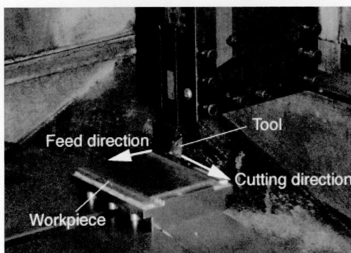
Fig. 2.19 Photograph of test specimen and tool on the lathe machine.
