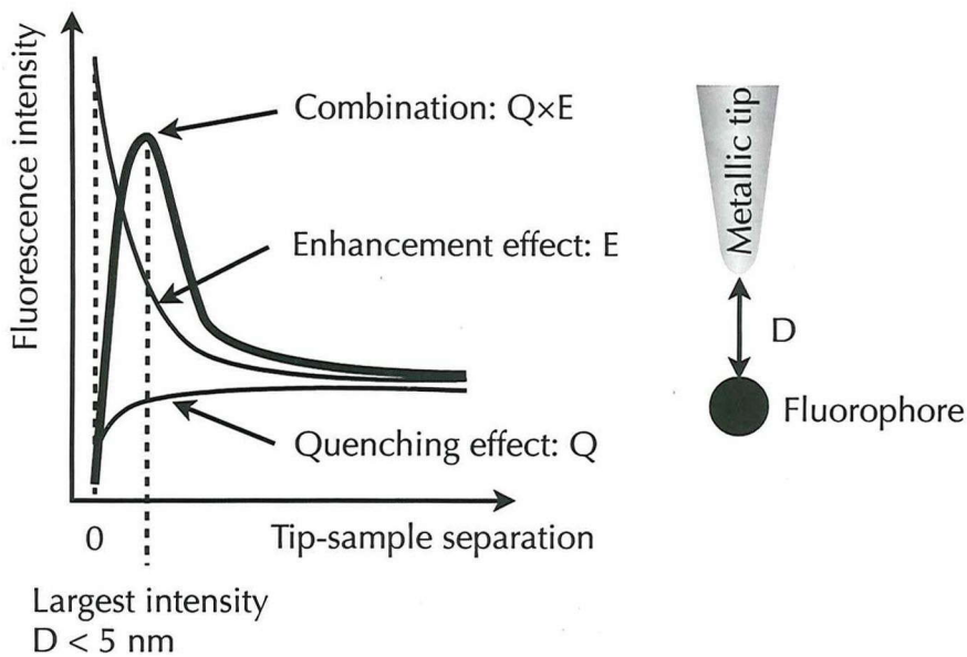
Figure 2.6.1 Schematic graph of fluorescence as a function of tip-sample separation
