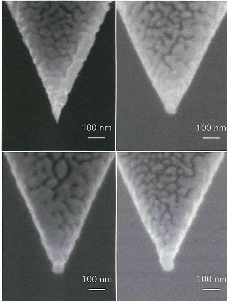
Figure 2 scanning electron microscopy images of Ag-coated tip
