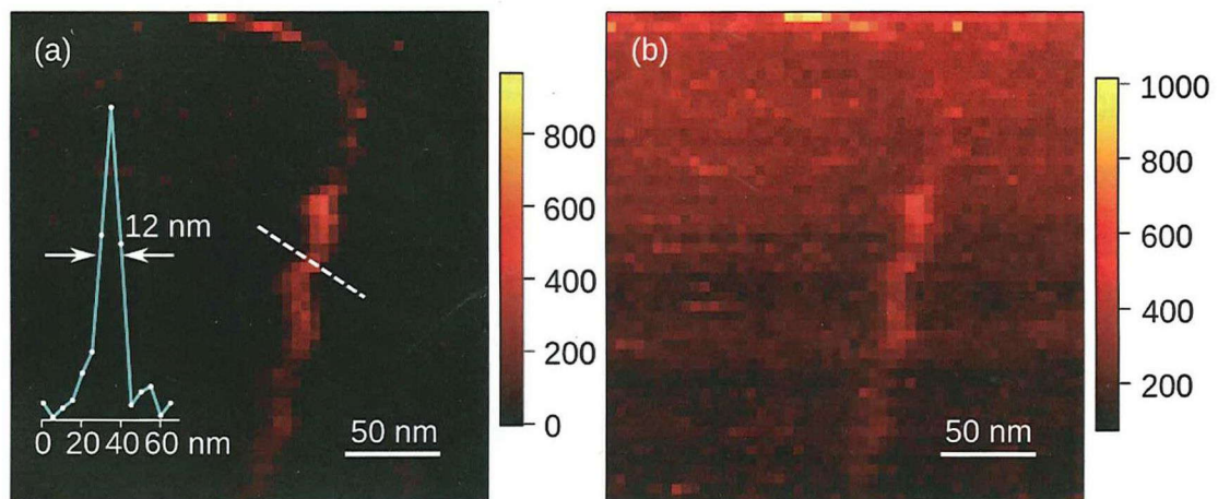
Figure 4.4.1 (a) Far-field free tip-enhanced Raman image of SWNTs. The inset graph is a cross section of SWNTs indicated by a dashed line. (b) Tip-enhanced Raman image with far-field signal. Both images have scan points of 50 \times 50 . The scale bar is 50 nm.
