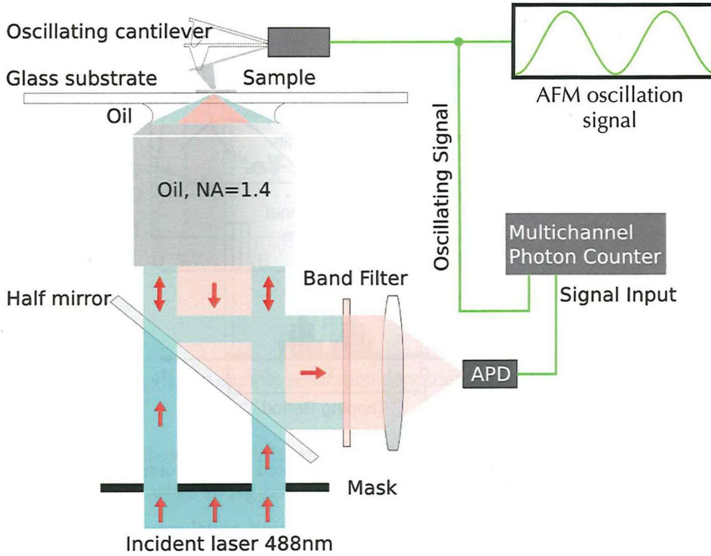
Figure 5.3.1 Schematic illustration of experimental setup
