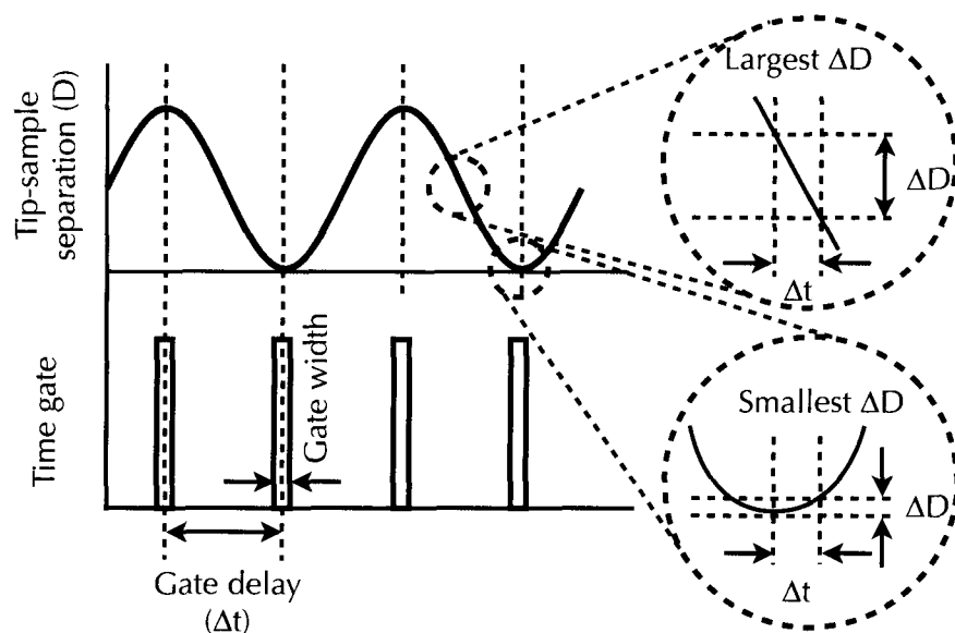
Figure 3.3.1 Schematic illustration of time gating for sectioning tip-sample separation
