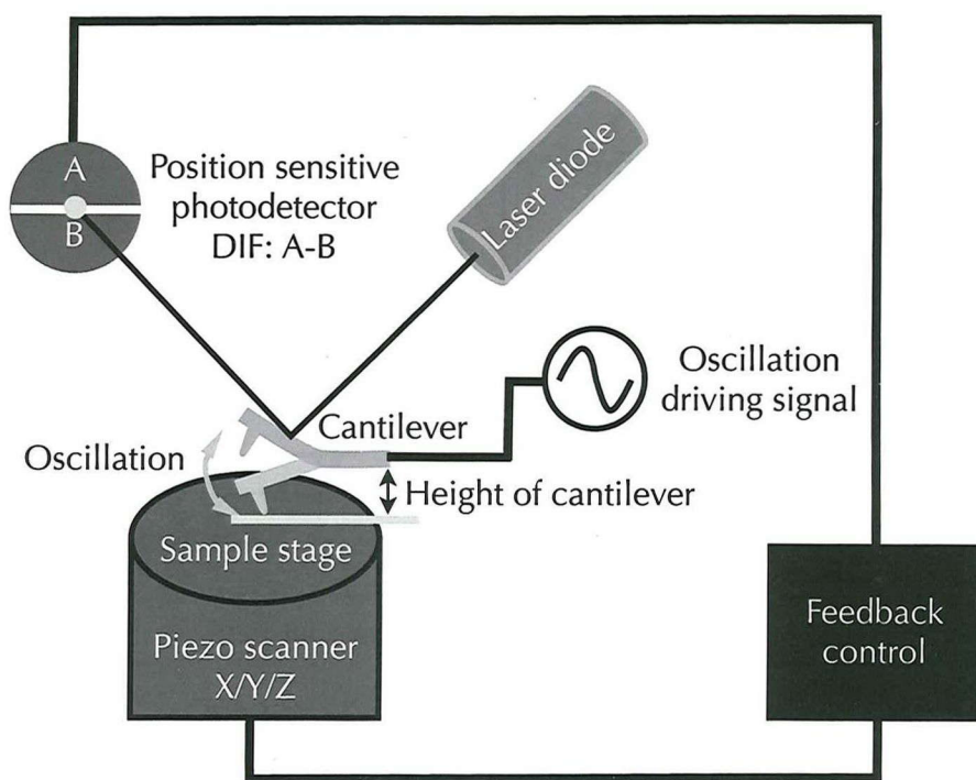
Figure 3.1.1 Tapping mode AFM system
