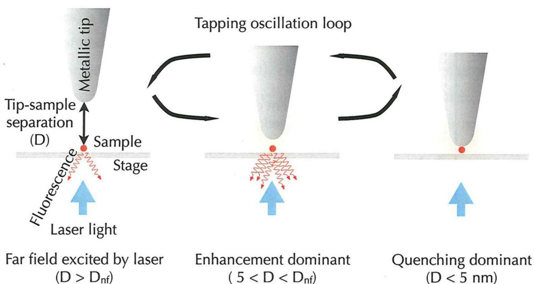
Figure 2.6.2 Tip-sample separation control for fluorescence intensity detection
