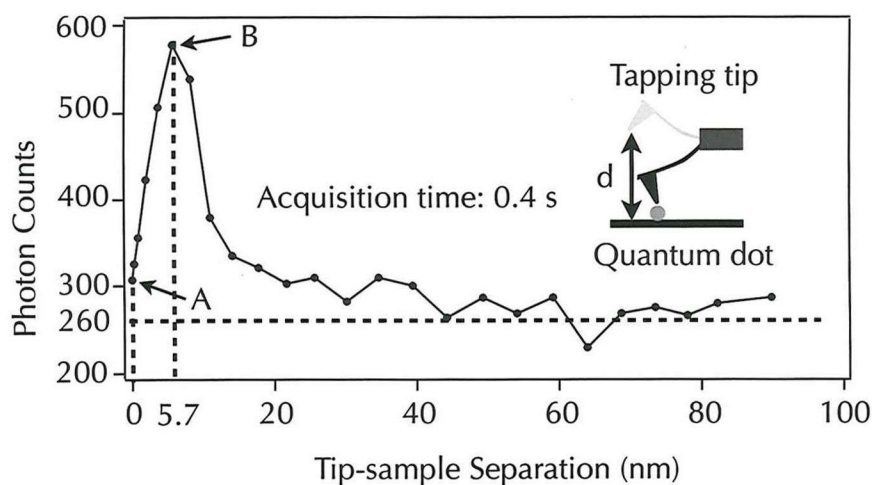
Figure 5.4.1 Tip-sample separation dependent fluorescence intensity
