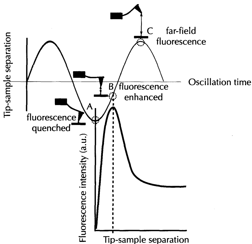
Figure 5.2.1 Schematic illustration of measuring tip-sample separation dependent fluorescence intensity
