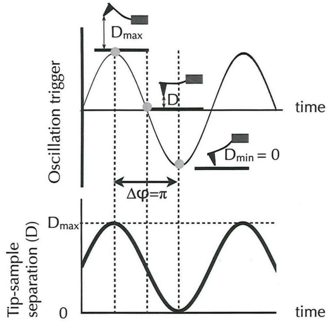
Figure 3.2.1 Tip-sample separation as a function of time
