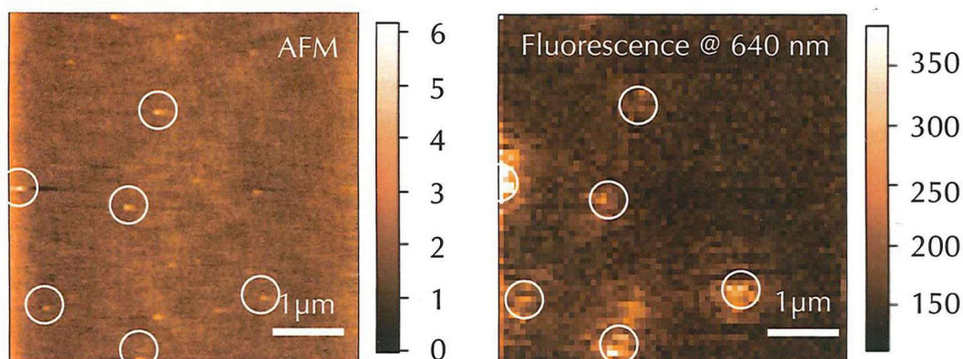
Figure 5.1.2 AFM image (left) and far-field fluorescence image (right) of quantum dots. Fluorescence image is constructed from emission intensity at 640 nm. The color bar of AFM image indicates height information in nm. The color bar in the fluorescence image indicates intensity information in arbitrary unit.
