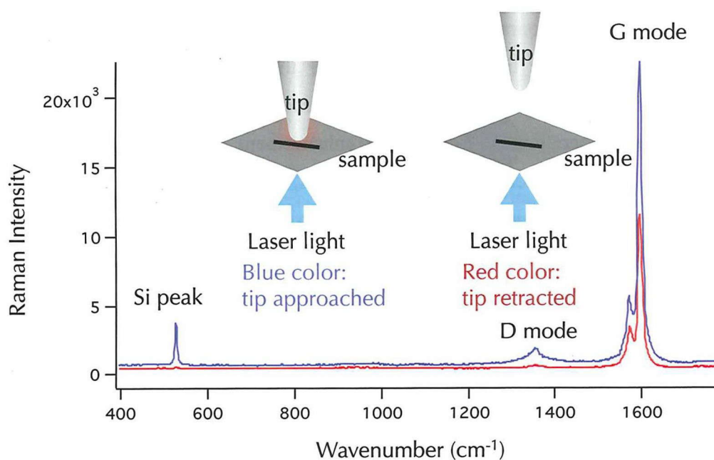
Figure 2.3.2 Illustration of tip-enhanced Raman spectrum from SWNTs
