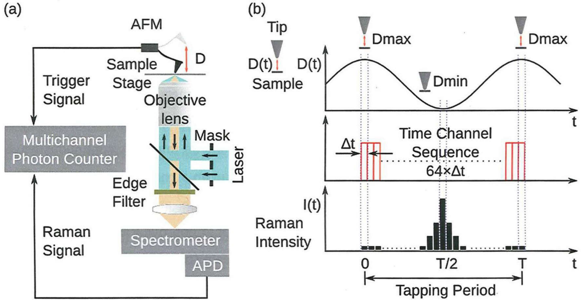
Figure 4.2.1 (a) Experimental setup for tip-enhanced near-field Raman microscopy through tapping-mode AFM configuration. (b) Schematic of time-correlated photon counting for Raman measurement.
