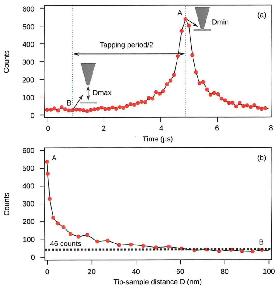
Figure 4.3.1 (a) Time-correlated Raman intensity measured while an Ag-coated nanotip is tapping on top of SWNTs. (b) Tip-sample distance dependent Raman intensity converted from position A to position B in graph (a).
