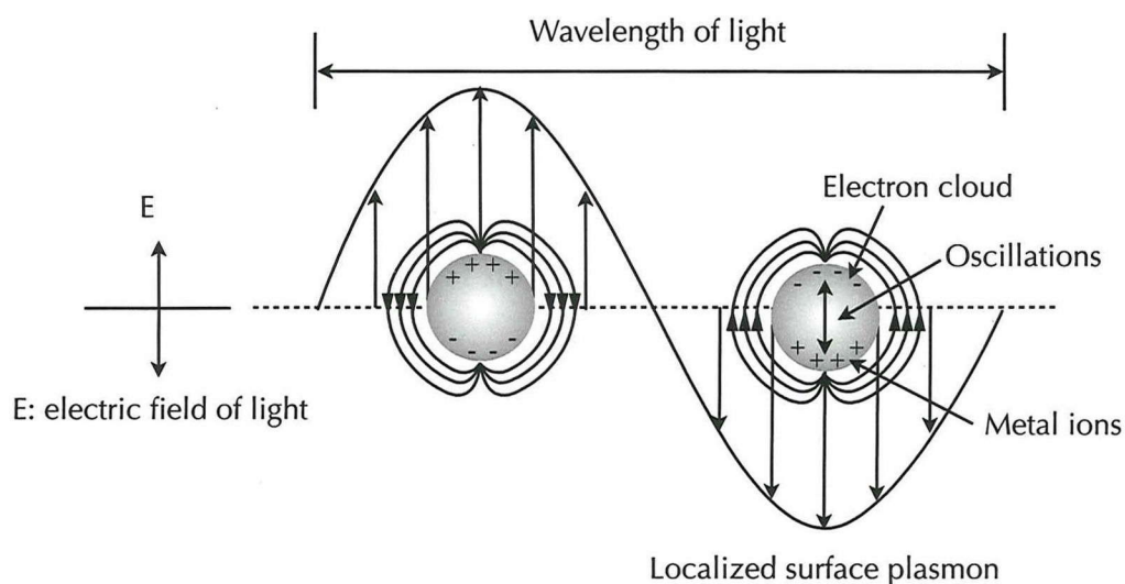
Figure 2.2.3 Schematic diagram of a localized surface plasmon
