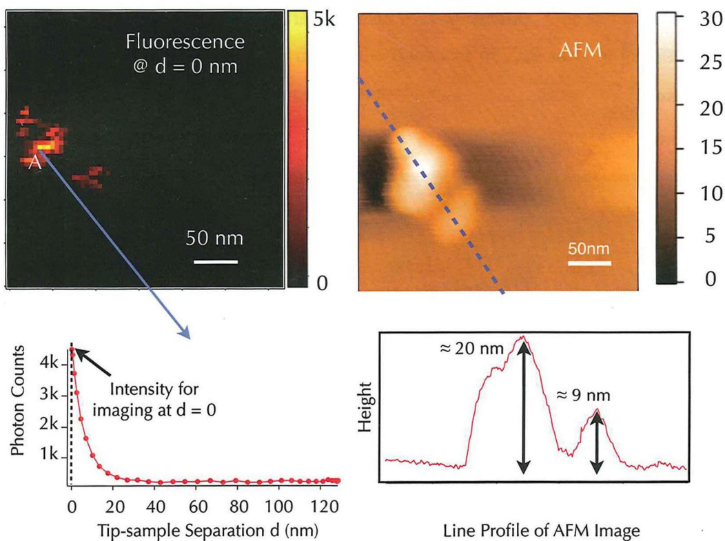
Figure 5.5.1 Tip-enhanced fluorescence image (top left) and AFM image (top right) of the same quantum dots. The scale bar is 50 nm in both images. Tip-sample separation dependent fluorescence intensity at position “A” in fluorescence image is illustrated in the bottom left. A line profile of sample depicted by the dashed line in AFM image is illustrated in the bottom right.
