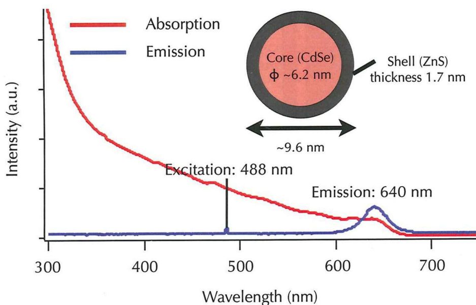
Figure 5.1.1 Absorption (red color) and fluorescence emission (blue color) of quantum dots. The schematic illustration shows the core/shell structure of a quantum dot.
