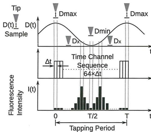
Figure 5.3.2 Schematic of time-correlated photon counting
