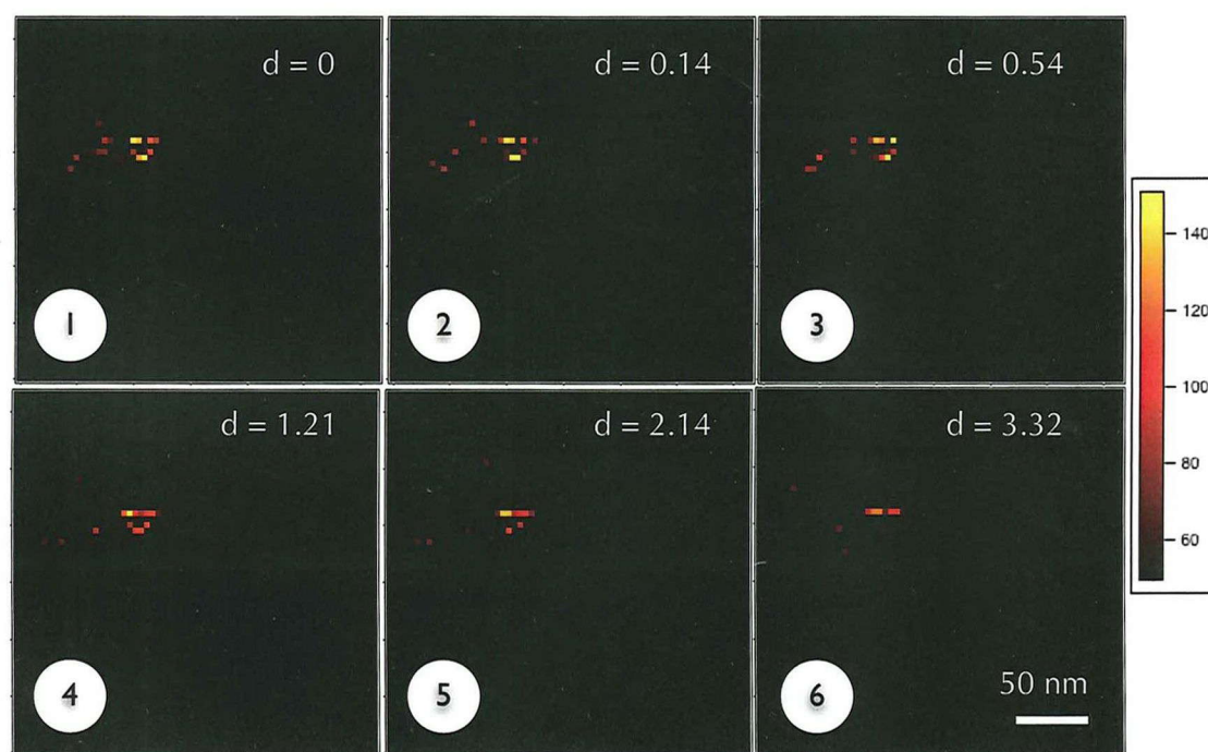
Figure 5.5.3 A group of fluorescence images of a single quantum dot at different tip-sample separations ( d , unit: nm). The scale bar is 50 nm.
