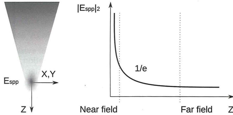
Figure 3.1.2 Near field and far field
