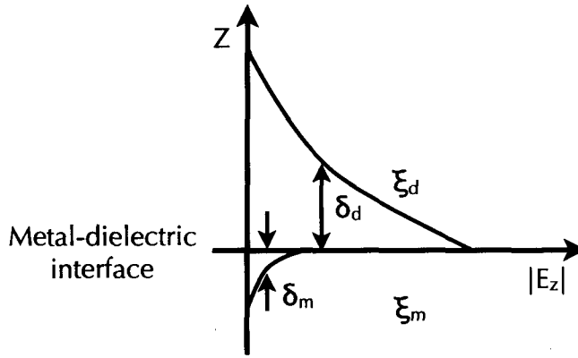
Figure 2.2.2 Field distribution of a SPP
