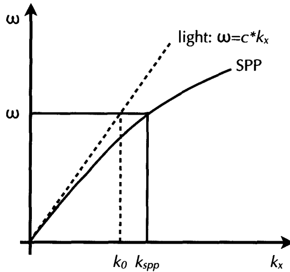
Figure 2.2.1 Dispersion curves of light and a SPP
