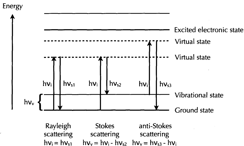
Figure 2.3.1 Different possibilities of light scattering
