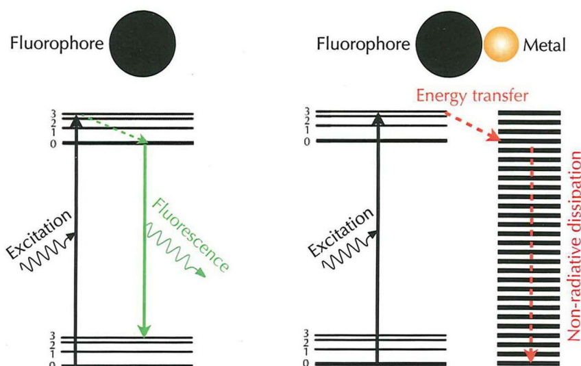
Figure 2.5.1 Fluorescence and quenching in a nanoparticle-fluorophore system
