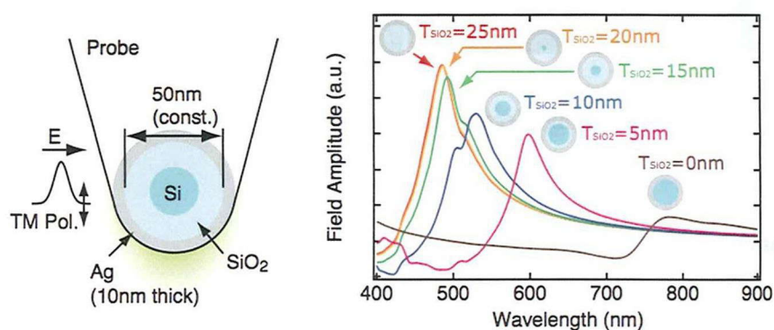
Figure 1. Calculation of \text{SiO}_2 thickness dependence of plasmonic resonant wavelength, referred from ref. 1
