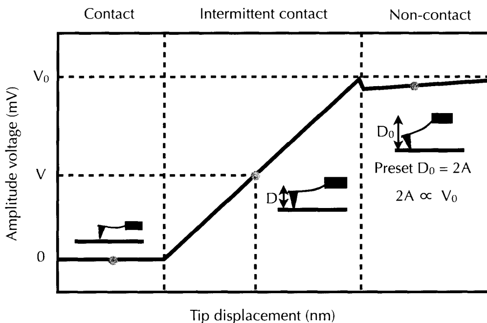
Figure 3.4.1 Process of force curve measurement
