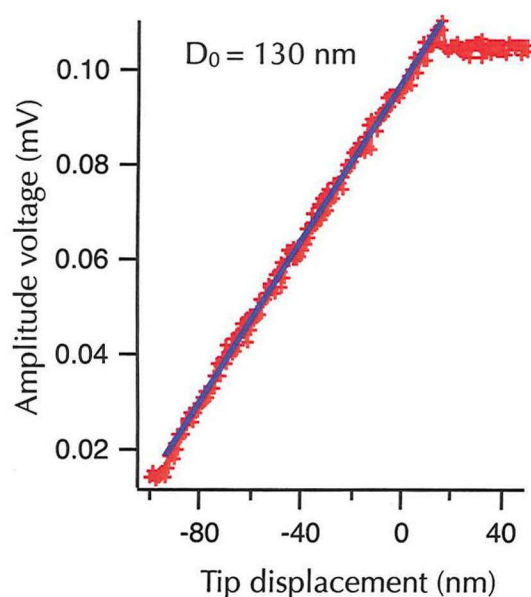
Figure 3.4.2 Experimental data of force curve measurement
