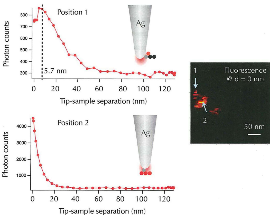
Figure 5.5.2 Tip-sample separation dependent fluorescence intensity at two different positions of the aggregated sample.
