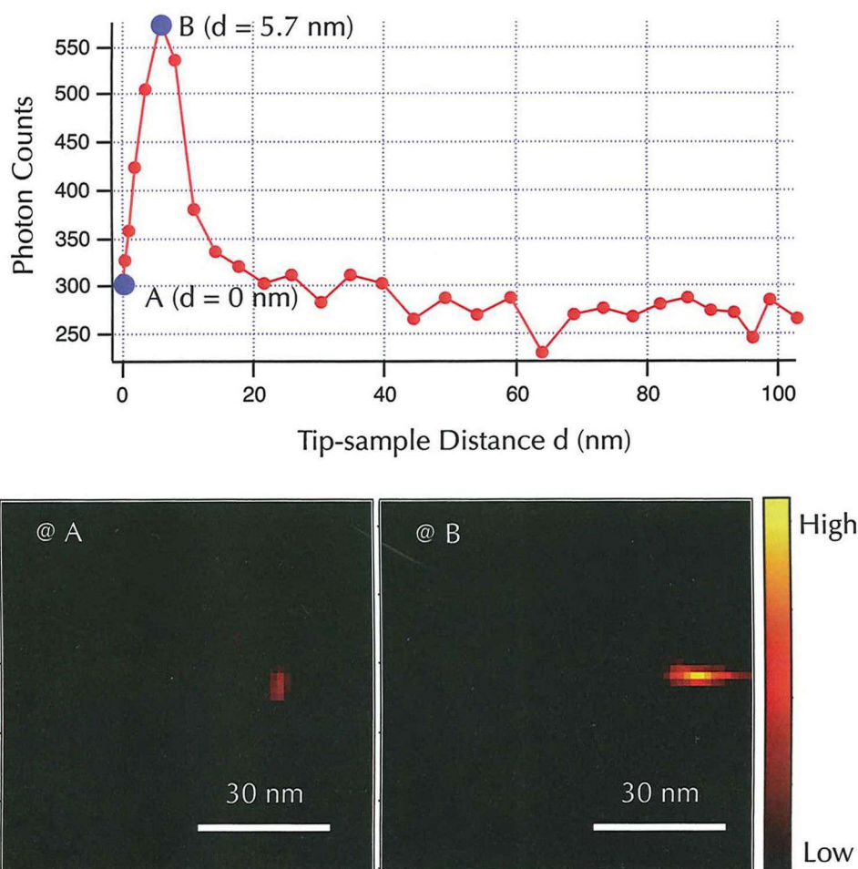
Figure 5.5.4 Comparison of tip-enhanced fluorescence imaging at different tip-sample separations. The scale bar is 30 nm.
