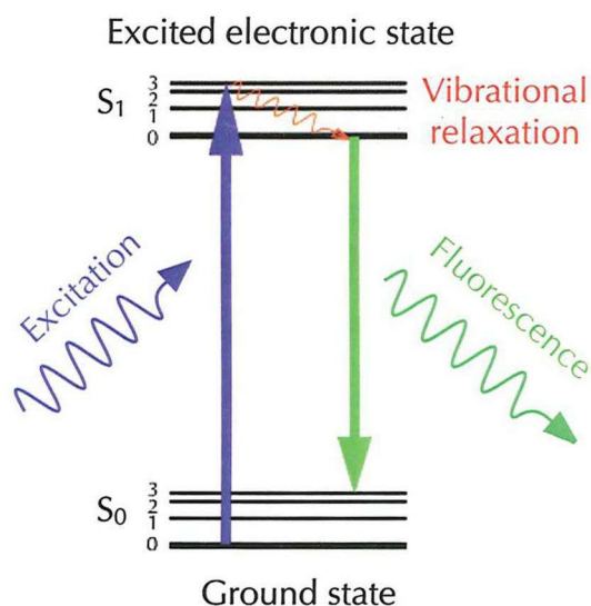
Figure 2.1.1 Jablonski diagram of fluorescence
