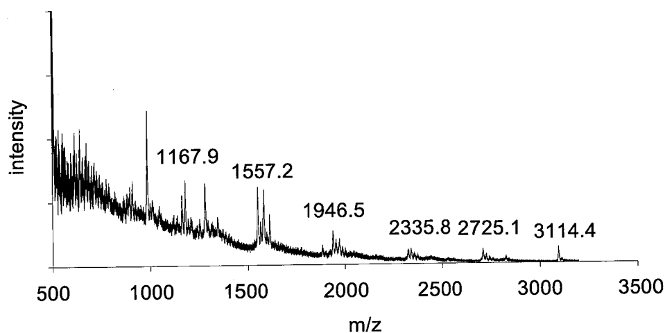
Figure 1. MALDI-TOF mass spectrum of 1-(P) .
