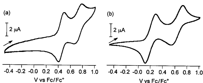
Figure 9. Cyclic voltammograms of a) 8red and b) 9red in dichloromethane ( 5.0 \times 10^{-4} M) containing 0.1 M \text{Bu}_4\text{NClO}_4 at a platinum working electrode with scan rate 100 \text{ mVs}^{-1} at 25^\circ\text{C} under an argon atmosphere.
