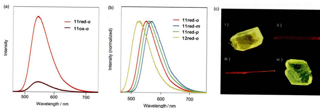
Figure 3. a) Emission spectra of 11red-o ( \lambda_{\text{ex}} = 430 nm) and 11ox-o ( \lambda_{\text{ex}} = 449 nm) and b) 11red-o ( \lambda_{\text{ex}} = 430 nm), 11red-m , ( \lambda_{\text{ex}} = 458 nm), 11red-p ( \lambda_{\text{ex}} = 446 nm), and 12red-o ( \lambda_{\text{ex}} = 415 nm) in dichloromethane ( 1.0 \times 10^{-5} M). c) Photographs (under 365 nm) of i) 11red-o , ii) 11red-m , iii) 11red-p , and iv) 12red-o .
