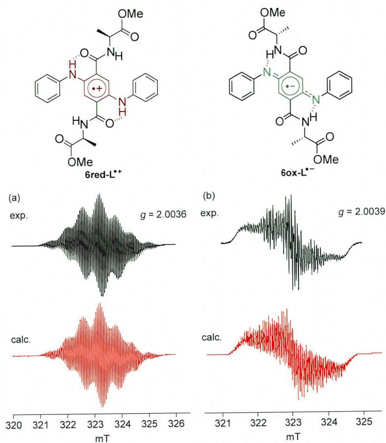
Figure 5. ESR spectra of a) 6red-L •+ in acetonitrile ( 1.0 \times 10^{-3} M) and b) 6ox-L •- in dichloromethane ( 1.0 \times 10^{-3} M) at 25 °C under a nitrogen atmosphere (black), and the simulated spectra (red).
