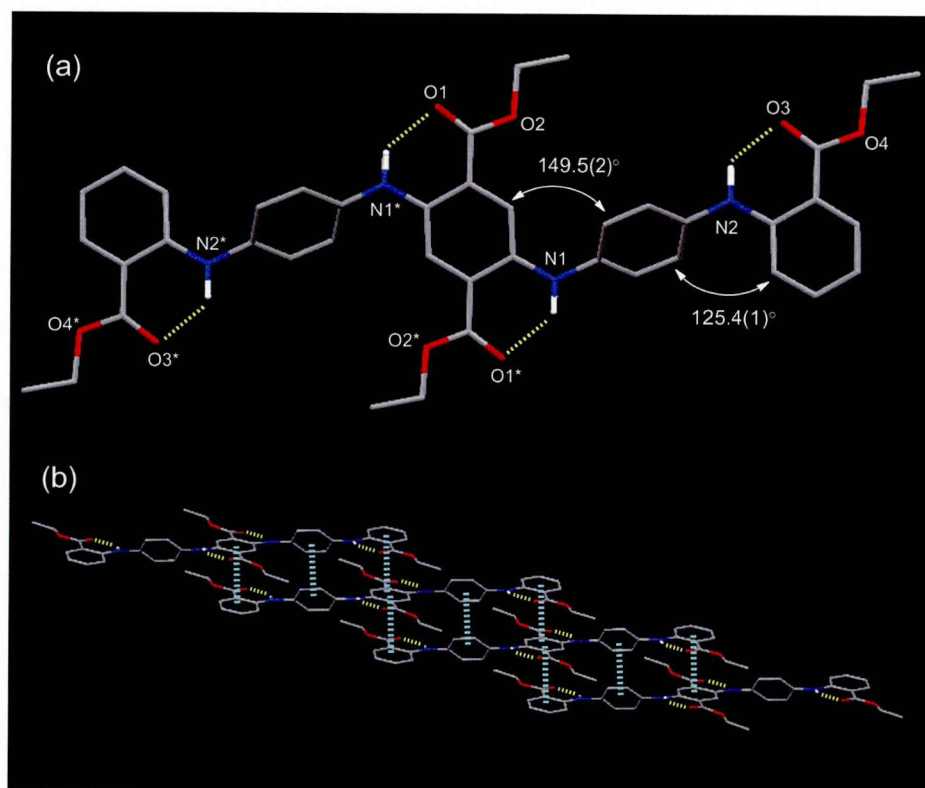
Figure 5. a) Crystal structure of 3 . b) Portion of a layer containing the ordered-layer structure through \pi - \pi stacking in the crystal packing of 3 .
