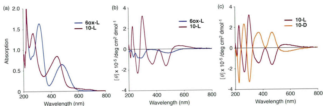
Figure 14. a) The electronic spectra of 6ox-L and 10-L . b) CD spectra of 6ox-L and 10-L . c) CD spectra of 10 in acetonitrile ( 1.0 \times 10^{-4} M) at 25 °C under an argon atmosphere.
