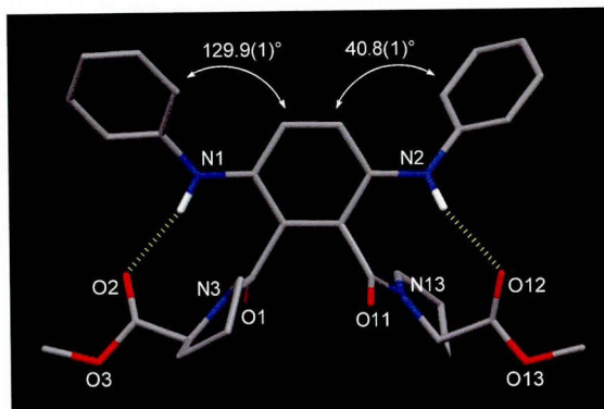
Figure 6. The structure of 9red as determined by X-ray crystallography.
