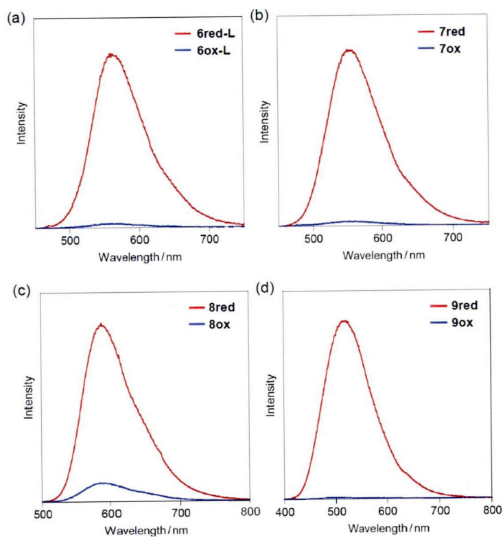
Figure 6. a) Emission spectra of 6red-L ( \lambda_{\text{ex}} = 430 nm) and 6ox-L ( \lambda_{\text{ex}} = 449 nm), (b) 7red ( \lambda_{\text{ex}} = 430 nm) and 7ox ( \lambda_{\text{ex}} = 458 nm), (c) 8red ( \lambda_{\text{ex}} = 409 nm) and 8ox ( \lambda_{\text{ex}} = 409 nm), and (d) 9red ( \lambda_{\text{ex}} = 375 nm) and 9ox ( \lambda_{\text{ex}} = 375 nm) in dichloromethane ( 1.0 \times 10^{-5} M) at 25 °C under a nitrogen atmosphere.
