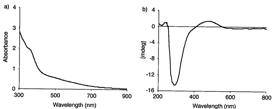
Figure 2. a) The electronic spectrum and b) CD spectrum of 1-(P) in dichloromethane at 25 °C under a nitrogen atmosphere.
