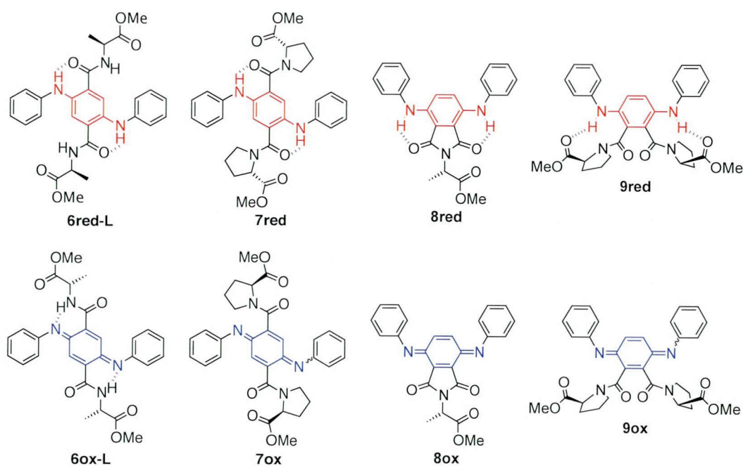
Figure 5. Phenylenediamines and quinonediimines bearing amino acid moieties.
