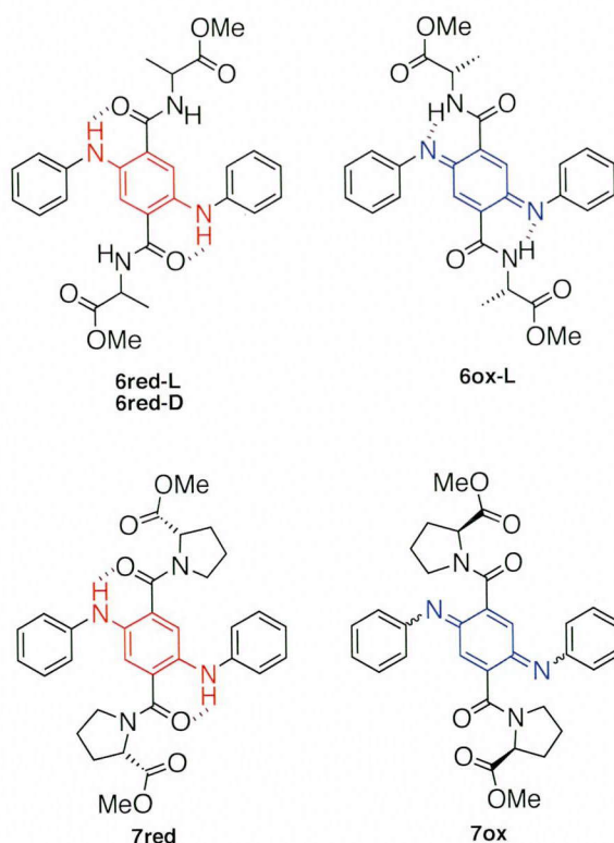
Figure 1. Phenylenediamines and quinonediimines bearing amino acid moieties.
