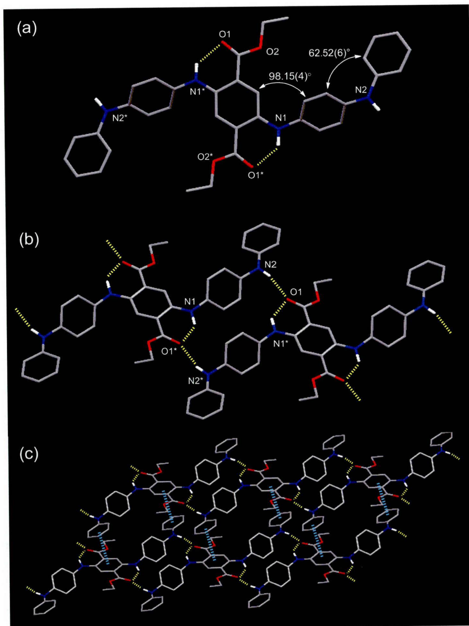
Figure 6. a) Crystal structure of 5 . b) Portion of a layer containing the sheet-like self-assembly through intermolecular hydrogen bonding networks. c) Portion of the \pi - \pi stacking in the crystal packing of 5 .
