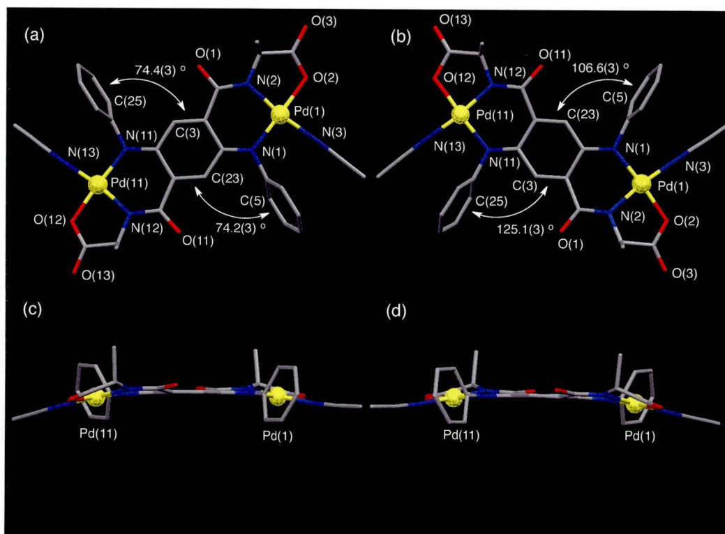
Figure 13. a) Top view and c) side view of molecular structure of 10-L . b) Top view and d) side view of molecular structure of 10-D (hydrogen atoms are omitted for clarity).
