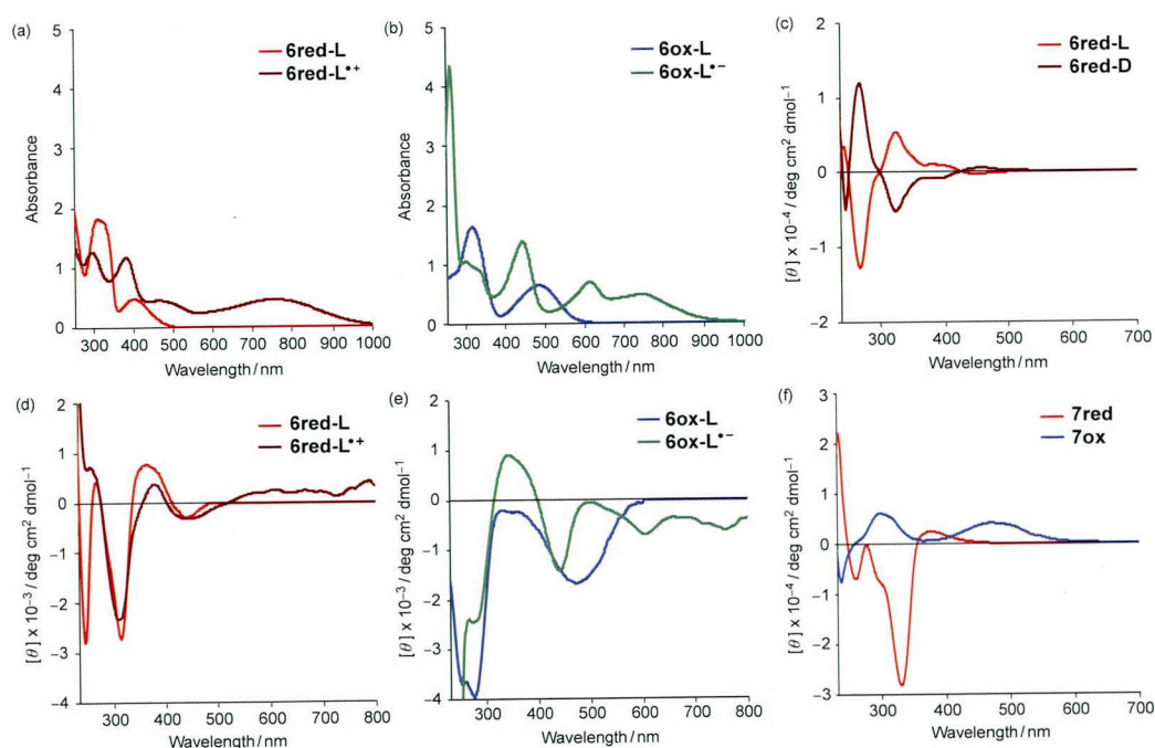
Figure 2. The electronic spectra of a) 6red-L and 6red-L •+ , b) 6ox-L and 6ox-L •- in acetonitrile ( 1.0 \times 10^{-4} M). The CD spectra of c) 6red-L and 6red-D , f) 7red in dichloromethane ( 1.0 \times 10^{-4} M), and d) 6red-L and 6red-L •+ , e) 6ox-L and 6ox-L •- in acetonitrile ( 2.5 \times 10^{-4} M) at 25 °C under a nitrogen atmosphere.
