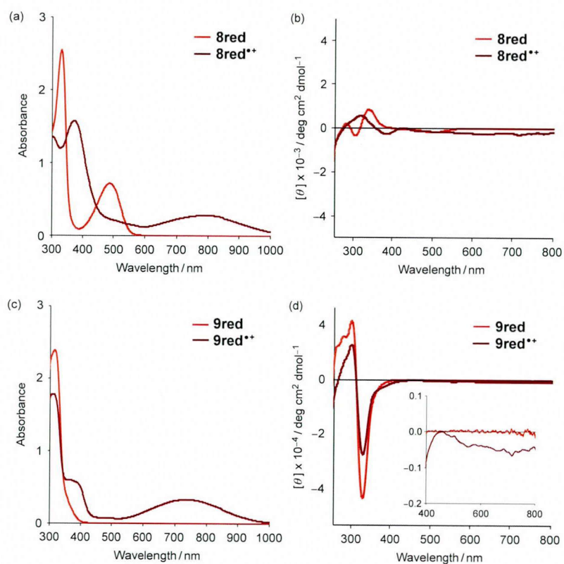
Figure 10. The electronic spectra of a) 8red and 8red •+ . b) The CD spectra of 8red and 8red •+ . c) The electronic spectra of 9red and 9red •+ . d) The CD spectra of 9red and 9red •+ . All these spectra measured in acetonitrile ( 1.0 \times 10^{-4} M) at 25 °C under a nitrogen atmosphere.
