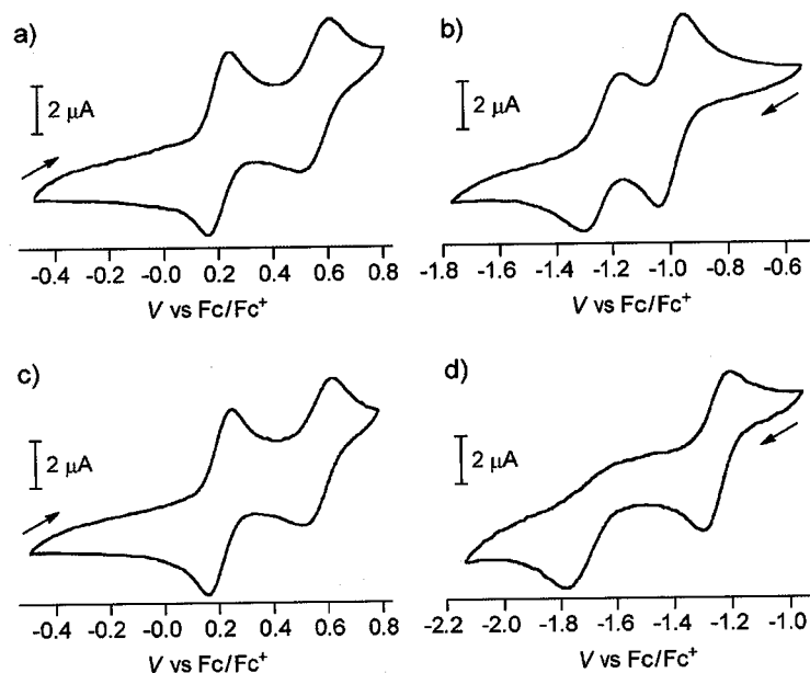
Figure 4. Cyclic voltammograms of a) 6red-L , b) 6ox-L , c) 7red , d) 7ox in dichloromethane ( 5.0 \times 10^{-4} M) containing 0.1 M \text{Bu}_4\text{NClO}_4 at a platinum working electrode with scan rate 100 \text{ mVs}^{-1} at 25^\circ\text{C} under an argon atmosphere.
