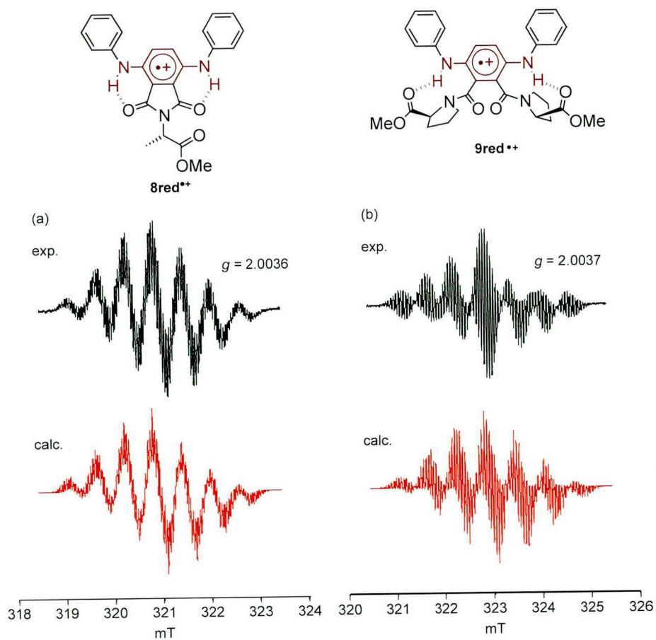
Figure 11. ESR spectra of a) 8red •+ in acetonitrile (1.0 x 10 -3 M) and b) 9red •+ in dichloromethane (1.0 x 10 -3 M) at 25 °C under a nitrogen atmosphere (black), and the simulated spectra (red).
