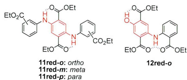
Figure 1. Phenylenediamine and phenylaminophenol derivatives.
