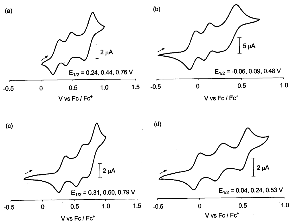
Figure 7. Cyclic voltammograms of (a) 2-L , (b) 4-L , (c) 3 , and (d) 5 in dichloromethane ( 5.0 \times 10^{-4} M) containing 0.1 M \text{Bu}_4\text{NClO}_4 at a platinum working electrode with a scan rate 100 \text{ mV s}^{-1} under an argon atmosphere.
