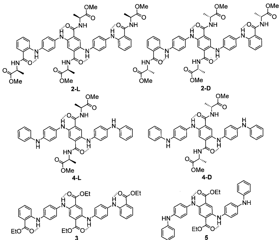
Figure 3. Structures of aniline tetramer derivatives.
