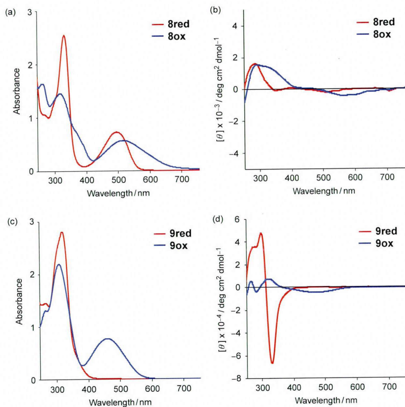
Figure 8. a) The electronic spectra of 8red and 8ox . b) The CD spectra of 8red and 8ox . c) The electronic spectra of 9red and 9ox . d) The CD spectra of 9red and 9ox . All these spectra measured in acetonitrile ( 1.0 \times 10^{-4} M) at 25 °C under a nitrogen atmosphere.
