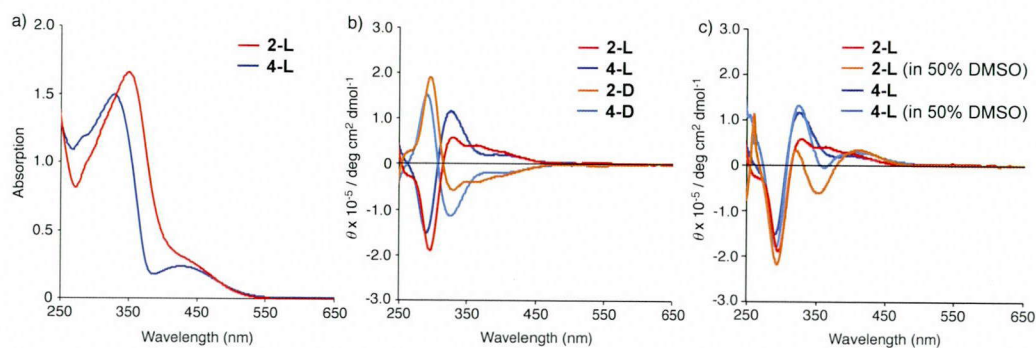
Figure 4. a) Absorption spectra of 2-L and 4-L . b) CD spectra of 2 and 4 in dichloromethane ( 5.0 \times 10^{-5} M) under a nitrogen atmosphere. c) CD spectra of 2-L and 4-L in dichloromethane-DMSO (1:1) ( 5.0 \times 10^{-5} M) at 25 °C under a nitrogen atmosphere.
