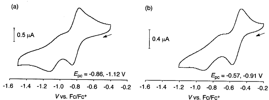
Figure 15. Cyclic voltammograms of a) 6ox-L and b) 10-L in DMSO ( 5.0 \times 10^{-4} \text{ M} ) containing 0.1 \text{ M Bu}_4\text{NClO}_4 at a glassy carbon working electrode with scan rate 10 \text{ mVs}^{-1} at 25^\circ\text{C} under an argon atmosphere.
