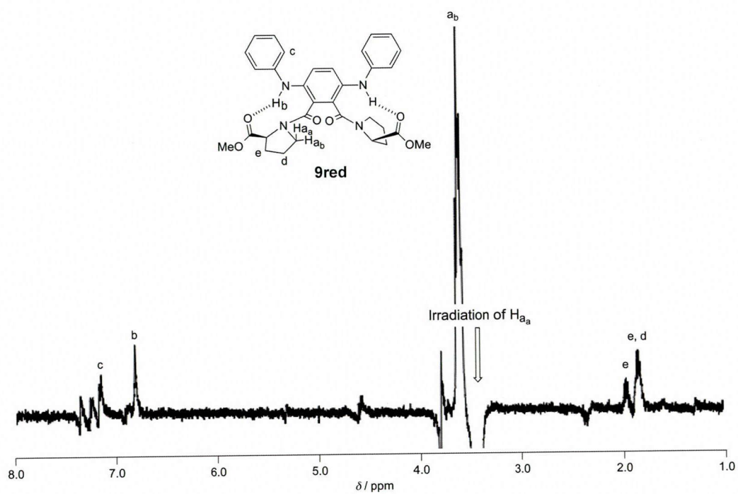
Figure 7. 400 MHz ^1\text{H} NMR difference NOE experiment performed at 25 °C with 1 second irradiation of a freeze-pump-thaw degassed solution of 9red in \text{CD}_2\text{Cl}_2 .
