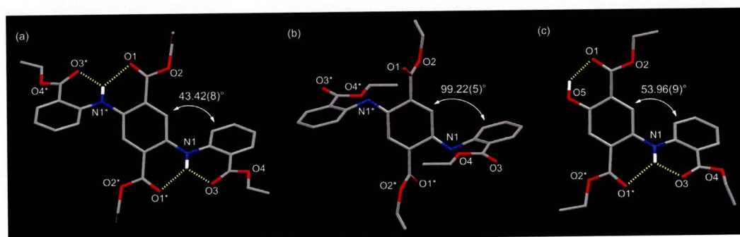
Figure 2. Crystal structures of (a) 11red-o , (b) 11ox-o , and (c) 12red-o .
