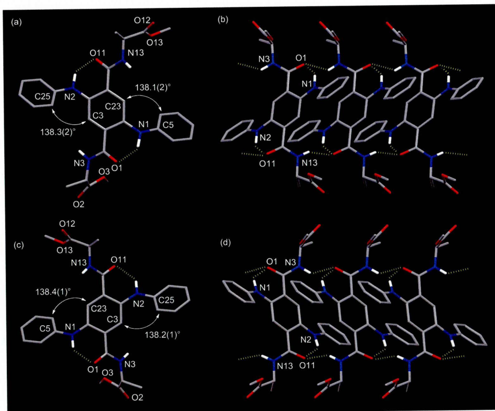
Figure 3. Molecular structures of a) 6red-L and c) 6red-D . A portion of a layer containing a sheet-like molecular arrangement through the intermolecular hydrogen bonding networks in the crystal packing of b) 6red-L and d) 6red-D .
