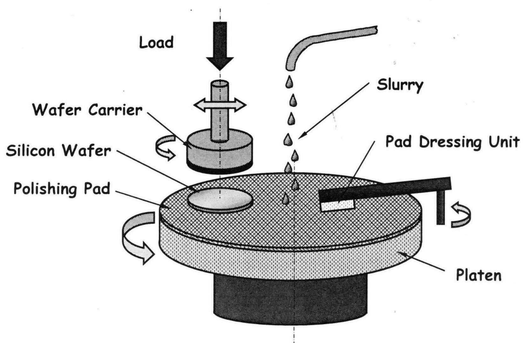
Fig. 2-1 Polishing unit
