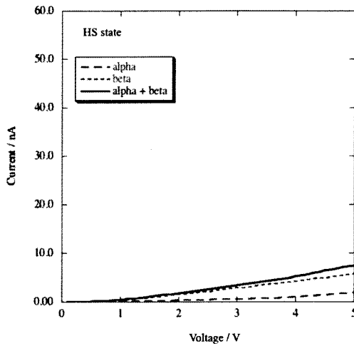
Figure 7.11: I - V curves of [\text{S-Cu}^{2+}\text{-S}]_2 with the backbone model connected to the hollow site of Au(111) surface in HS and BS LS states at 300 K temperature.
