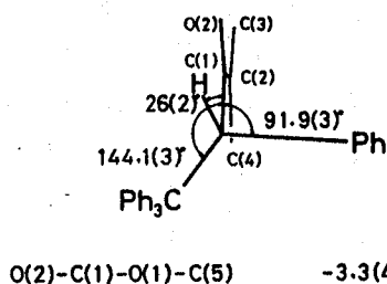
(R)-TrBzMA 1
