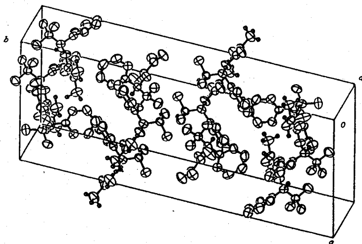
Figure 40. The crystal structure of t-BBMA(ORTEP II)
