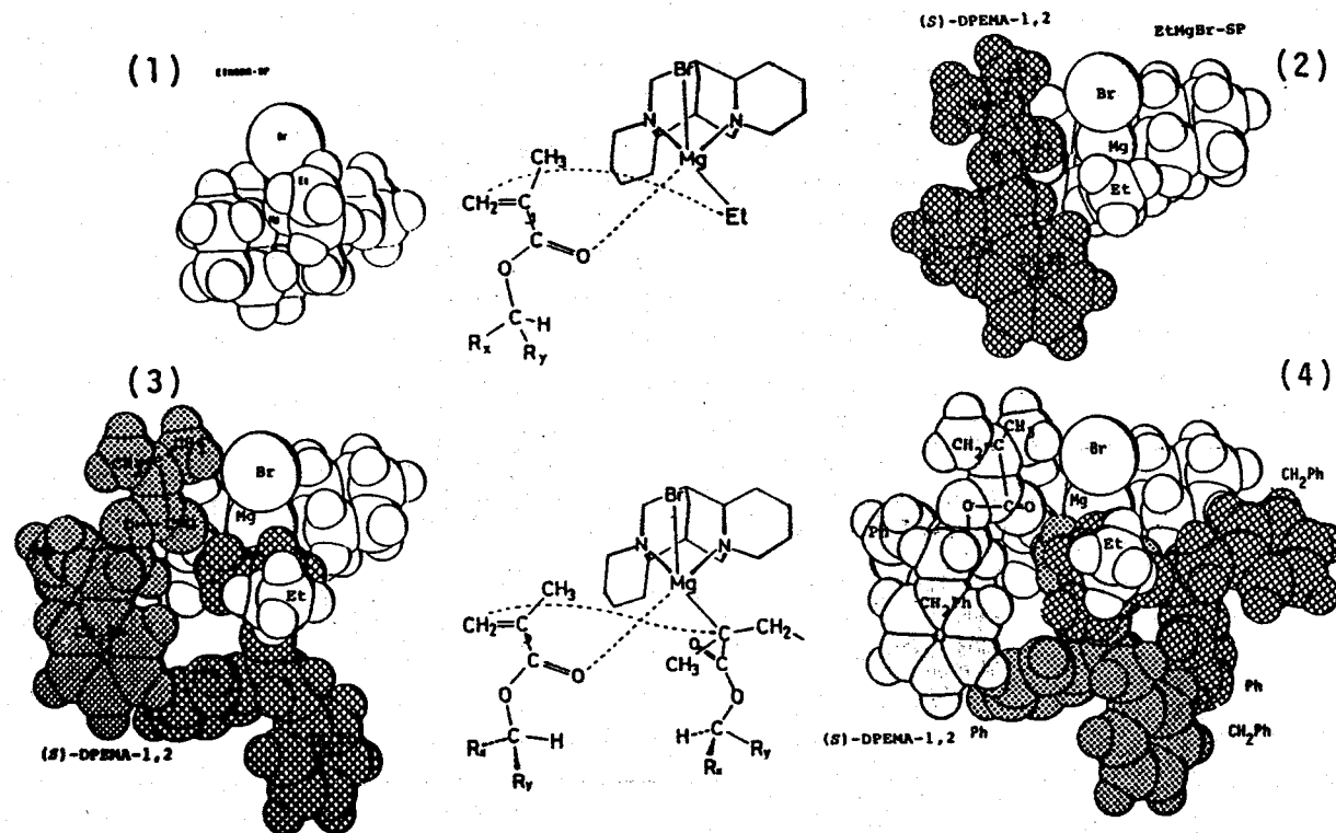
Figure 44. The postulated mechanism of enantiomer selection for DPEMA-1,2
