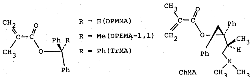
Scheme 9.
