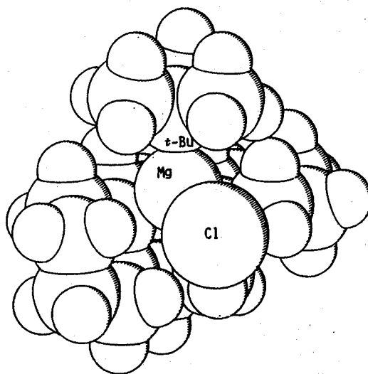
Figure 24. The space-filling model of 4g (PLUTO)
