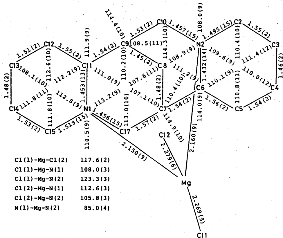
Figure 11. Bond lengths[Å] and bond angles[°] in 4g'
