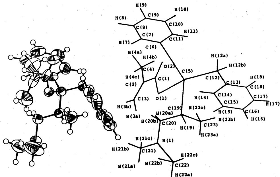
Figure 32. The molecular structure of ChMA (ORTEP II)
