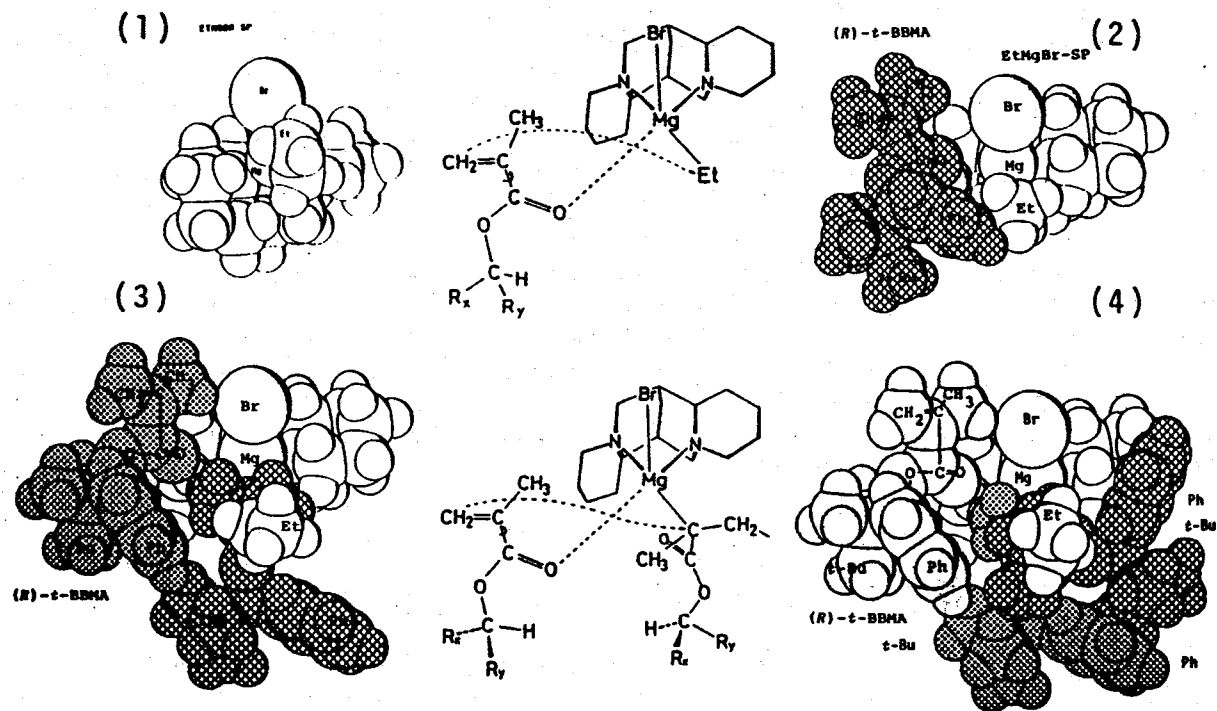
Figure 45. The postulated mechanism of enantiomer selection for t -BBMA
