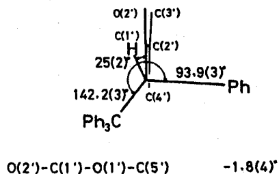
(R)-TrBzMA 2
