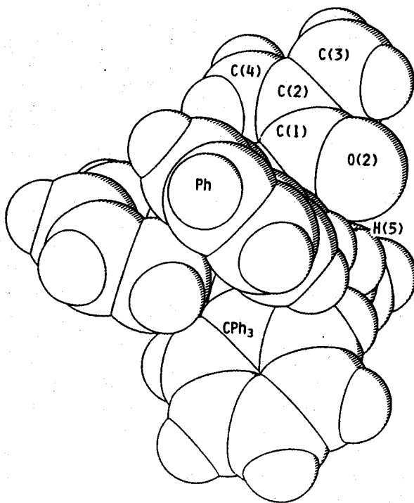
Figure 46. The space-filling model of ( S )-TrBzMA (PLUTO)
