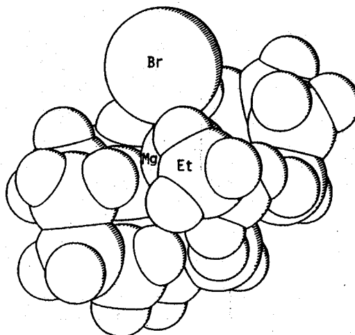
Figure 25. The space-filling model of 5 (PLUTO)
