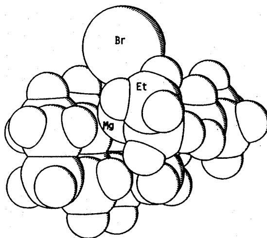
Figure 22. The space-filling model of 4a (PLUTO)
