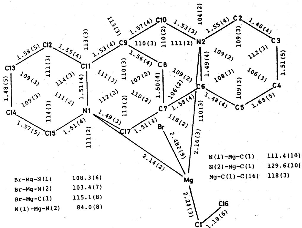
Figure 9. Bond lengths[Å] and bond angles[°] in 4a
