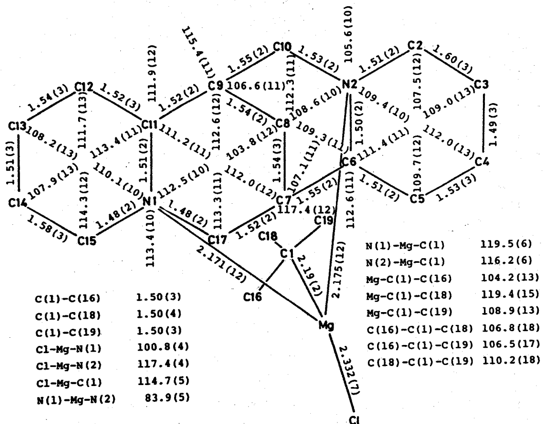
Figure 10. Bond lengths[Å] and bond angles[°] in 4g
