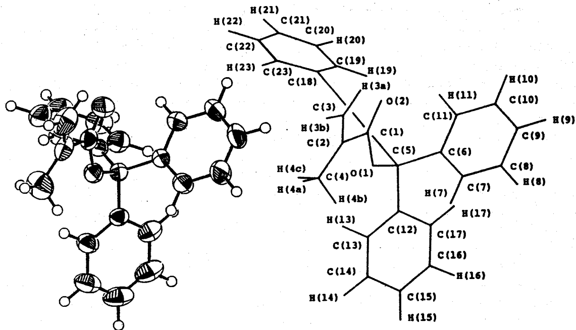
Figure 28. The molecular structure of TrMA(ORTEP II)
