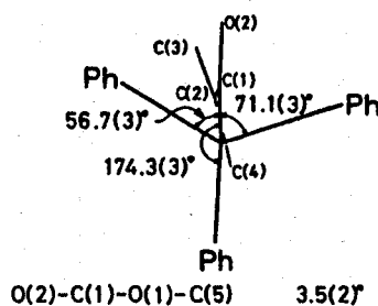
TrMA
