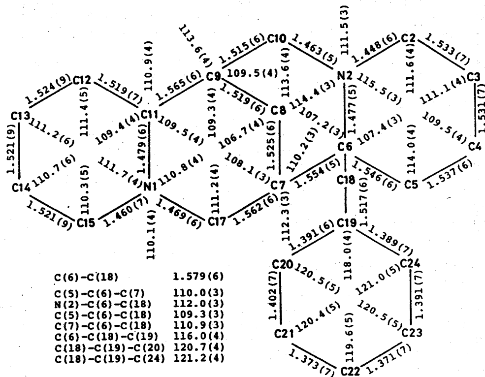
Figure 8. Bond lengths[Å] and bond angles[°] in 2c
