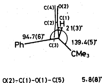
(R)-t-BBMA 1
