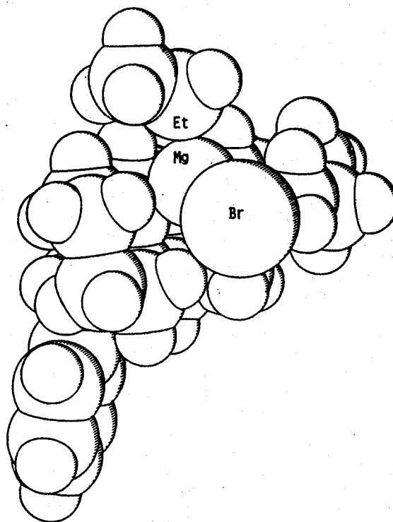
Figure 23. The space-filling model of 7 (PLUTO)
