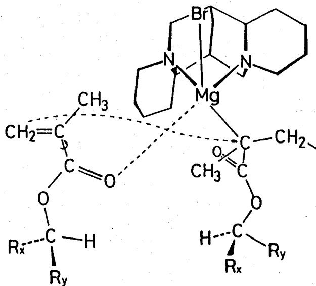
Scheme 12.
