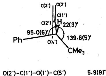
(R)-t-BBMA 2
