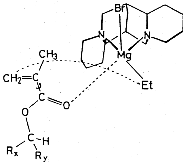
Scheme 11.
