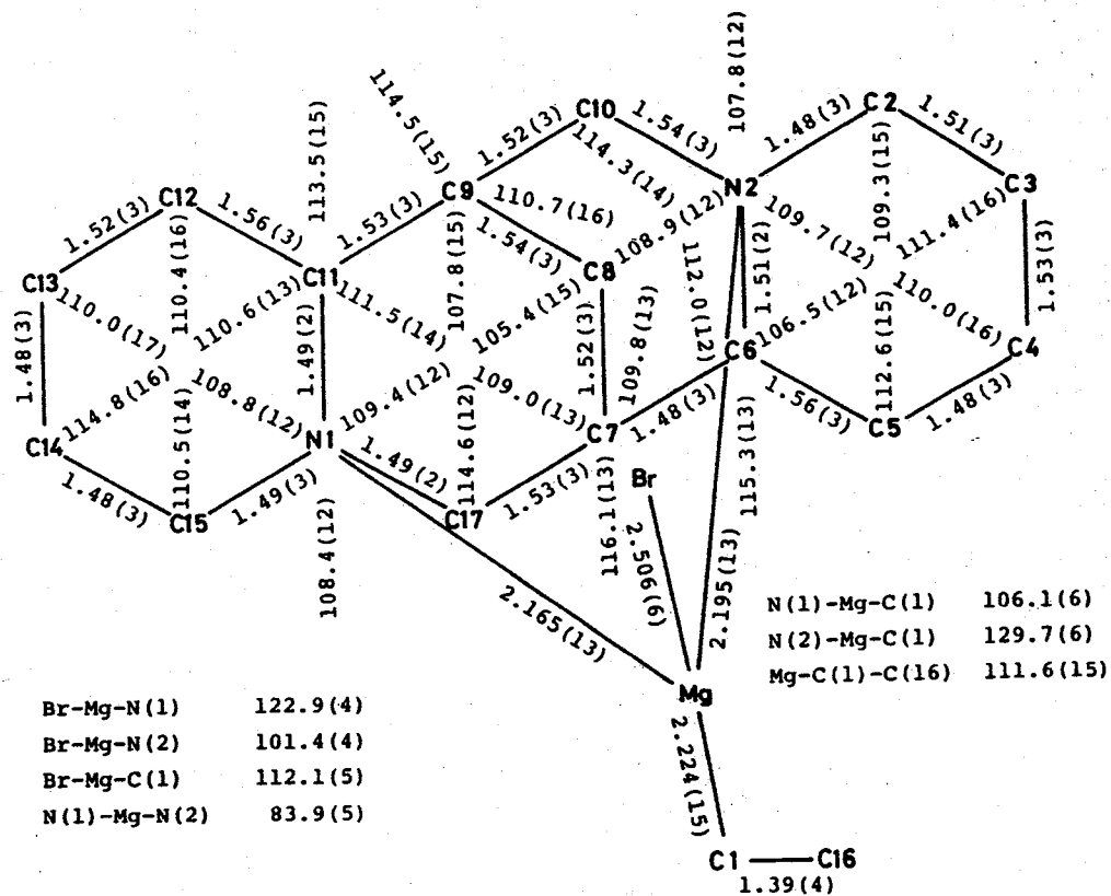
Figure 12. Bond lengths[Å] and bond angles[°] in 5
