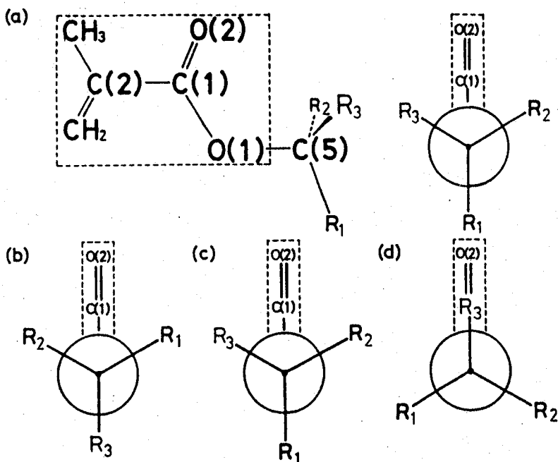
Figure 33. The possible conformations of the methacrylate molecules
