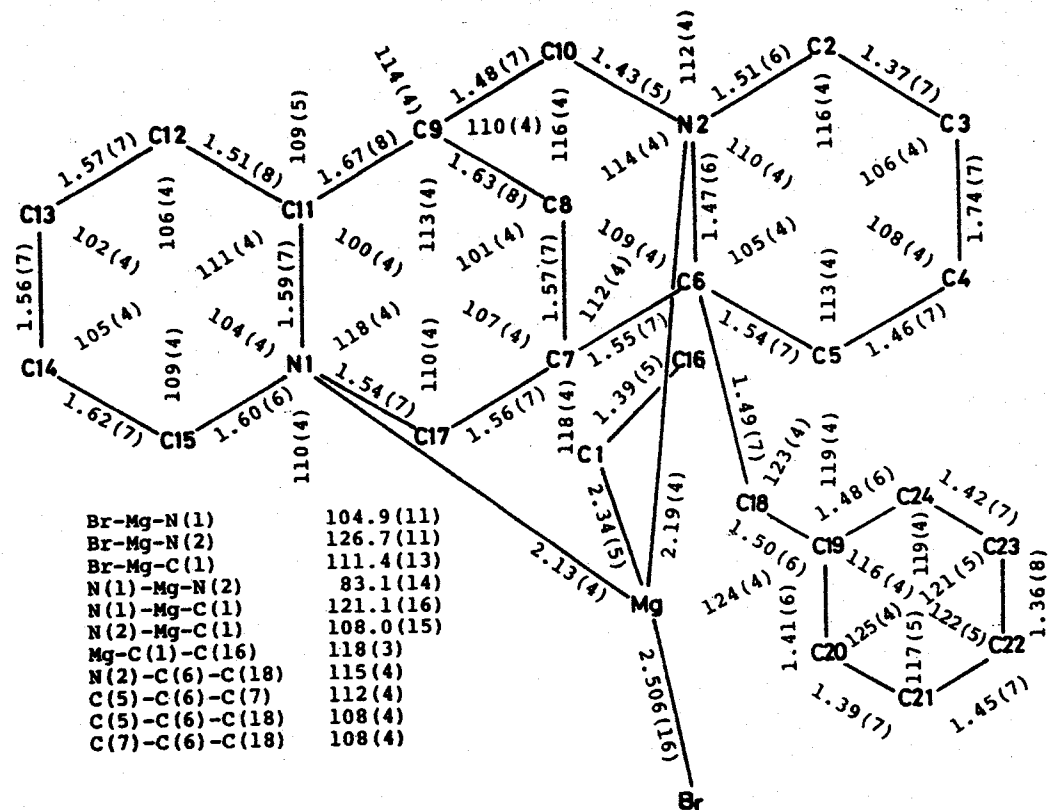
Figure 13. Bond lengths[Å] and bond angles[°] in 7
