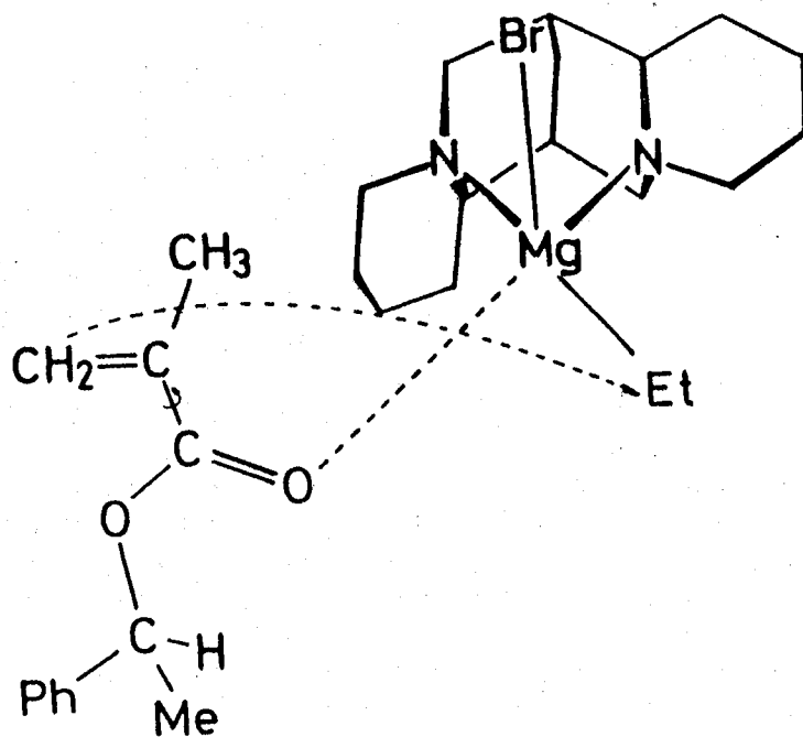
Scheme 7.
