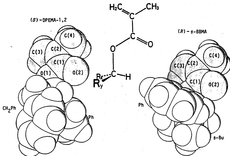
Figure 43. The space-filling models of DPEMA-1,2(left) and t -BBMA(right) (PLUTO)
