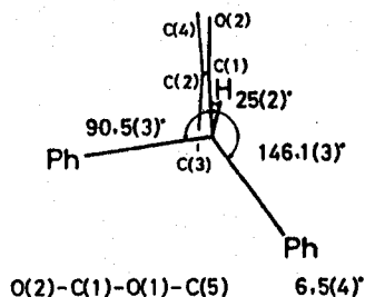
DPMMA
