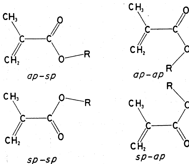
Scheme 10.
