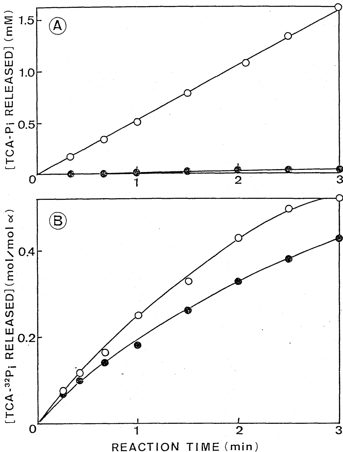
Fig. 7. Effects of DCCD-treatment of EF 1 on its steady-state ATPase and single turnover of DNS-ATP hydrolysis. (A) EF 1 at 0.87 μM was preincubated with (●) or without (○) 0.2 mM DCCD in 2 mM EDTA and 50 mM Tris-acetate at pH 7.0 and 30°C for 20 min. Then, EF 1 solution was diluted to 0.087 μM in 5 mM phosphoenolpyruvate, 0.11 mg/ml pyruvate kinase, 2.5 mM MgCl 2 , 0.2 mM EDTA and 50 mM Tris-HCl at pH 8.0 and 30°C. The reaction was started by addition of 5 mM ATP. (B) EF 1 at 1.6 μM was preincubated with (●) or without (○) 0.2 mM DCCD under the same conditions as A, then allowed to react with 2.8 μM DNS-AT 32 P for 1 min. The reaction was started by addition of 3 mM Mg 2+ .
