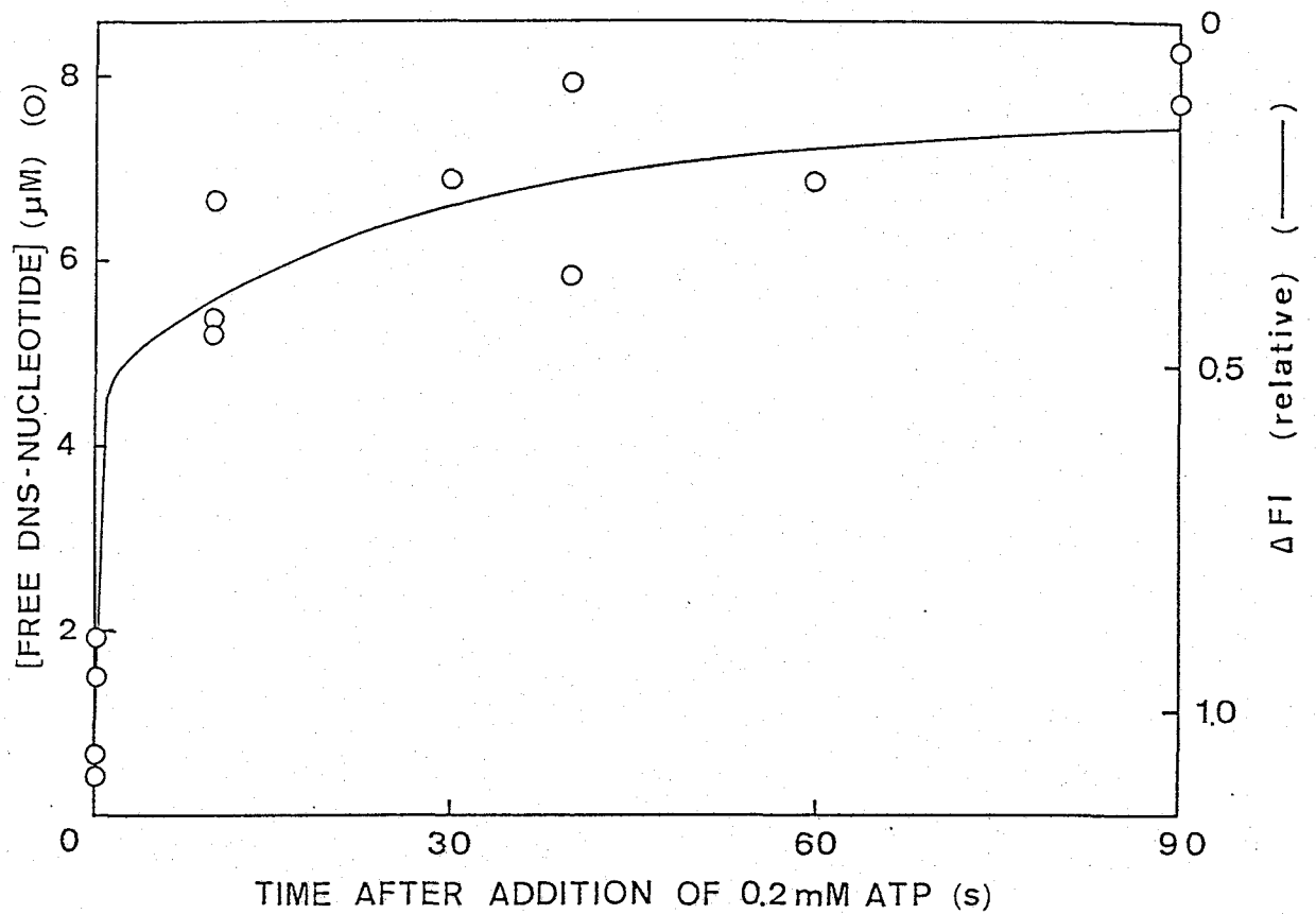
Fig. 16. Comparison of the time course of a decrease in fluorescence with that of release of DNS-nucleotide on addition of ATP to F_1 -DNS-ATP. A mixture containing 8.6 \mu\text{M} DNS-ATP, 9.2 \mu\text{M} F_1 , and 10 mM [ ^3\text{H} ]glucose was incubated with 5 mM \text{MgCl}_2 for 90 s, and then 0.2 mM ATP was added. The reaction was stopped by filtration through an XM-100A membrane at the time indicated. The extent of a decrease in fluorescence intensity, \Delta\text{FI} , is plotted as relative to difference between the intensity before addition of 0.2 mM ATP (1.0) and that of free DNS-ADP (0).
