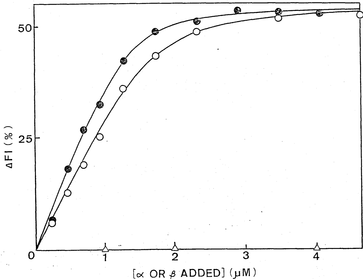
Fig. 10. Fluorescence titration of DNS-ATP with \alpha subunit in the presence of \text{Mg}^{2+} . The extent of fluorescence increase of 1.1 \mu\text{M} DNS-ATP after addition of 3 \text{ mM } \text{Mg}^{2+} was plotted against the amount of \alpha subunit at 30^\circ (O) or 4^\circ\text{C} (●). Other conditions are the same as described in Fig. 8. The extent of fluorescence decrease of free DNS-ATP in the presence of free \text{Mg}^{2+} (cf. Fig. 9, curve c) was corrected. The solid lines are the theoretical curves (see the text). When 1.1 \mu\text{M} DNS-ATP was allowed to react with \beta subunit in the presence of \text{Mg}^{2+} at 30^\circ\text{C} , no fluorescence change was observed ( \Delta ).
