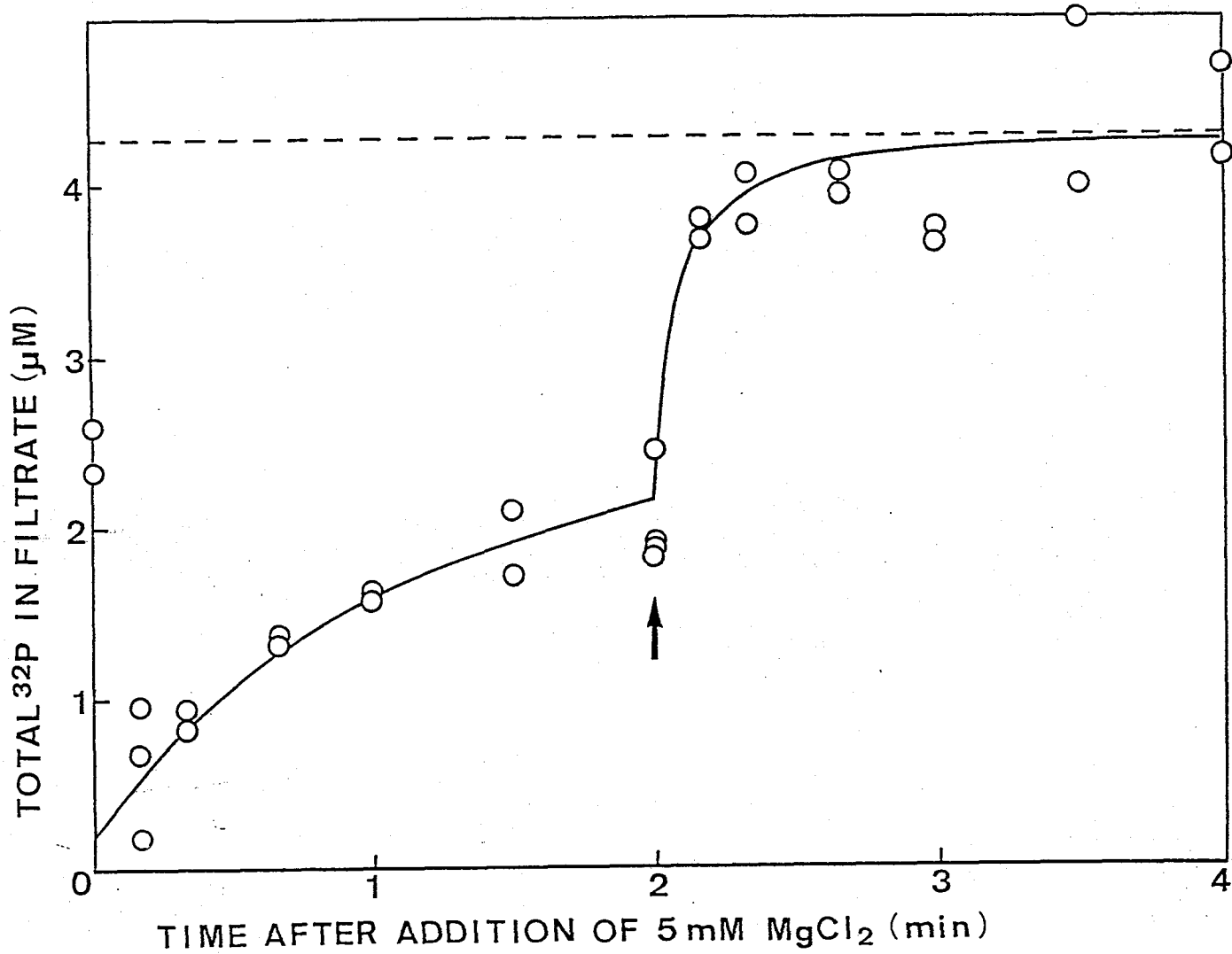
Fig. 15. Acceleration by ATP of free ^{32}\text{P} liberation from the \text{F}_1\text{-DNS-AT}^{32}\text{P} system. The reaction was carried out under the identical conditions as described in the legend to Fig. 13 except that the reaction was stopped by filtration through an XM-100A membrane.
