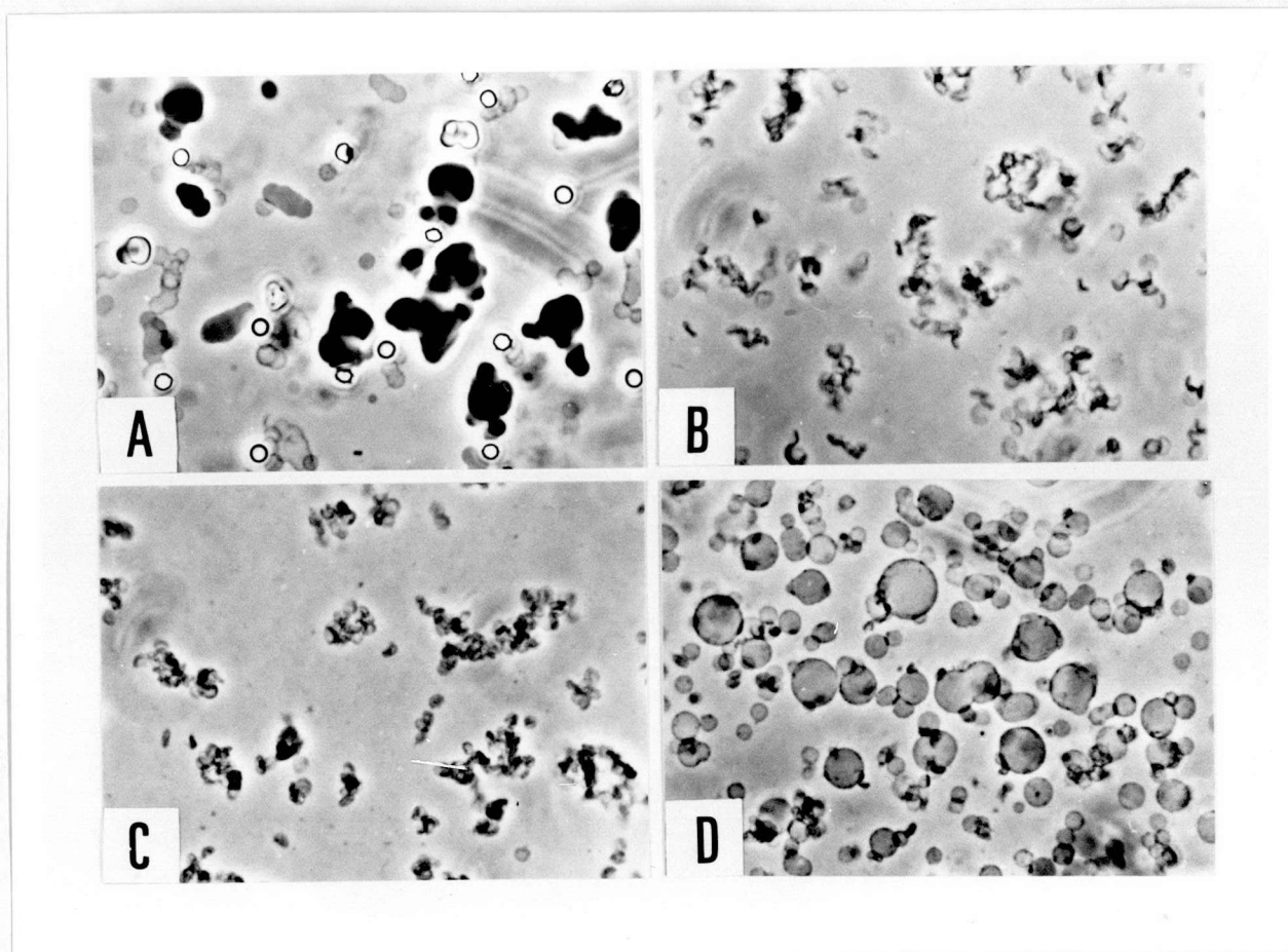
Fig. 1. Restoration of fusion activity of erythrocyte ghosts by including bovine serum albumin. (A), Virus-induced fusion of intact erythrocytes. Intact cells were agglutinated by HVJ (312 HAU/ml) for 15 min in an ice bath, and subsequently incubated for 30 min at 37°. Many large fused cells which partially lost internal hemoglobin could be seen. (B), Ghosts prepared according to Dodge et al (11) and then suspended in TBS were treated with HVJ (312 HAU/ml) as described in (A). Note that no fused ghosts could be observed and ghosts were still somewhat agglutinated even after the end of incubation at 37°. (C), The same as (B) except that applied dose of HVJ was 3,000 HAU/ml. Neither fused ghosts could be seen. (D), The same as (C) except that ghosts loaded with 5 % BSA (see "Materials and Methods") were substituted for unsealed ghosts. Many fused ghosts could be seen. Phase microscopy, x350.
