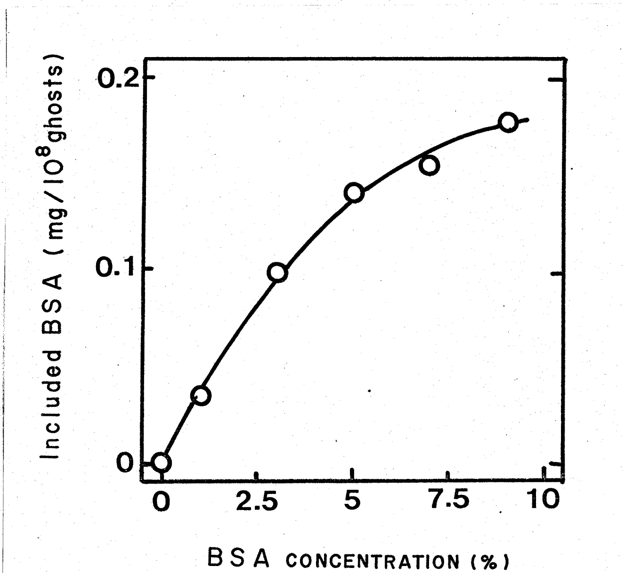
Fig. 3. The amount of BSA included within ghosts. Ghosts loaded with increasing concentrations of BSA were prepared as described in "Materials and Methods". The amount of included BSA was estimated by subtracting the amount of original membrane proteins (which was determined using the ghosts resealed in the absence of BSA) from the total proteins of ghosts. The value was normalized against ghost: number which was determined with a Coulter counter.
