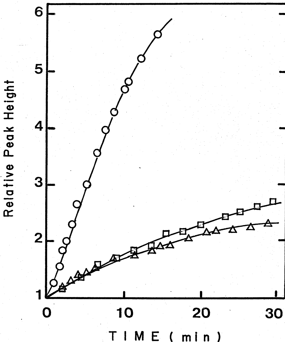
Fig. 12. Phospholipid intermixing between viral envelope and the erythrocyte membrane. Either intact erythrocytes (○) or resealed ghosts prepared in the presence (□) or absence (△) of 5% BSA were agglutinated by HVJ (a mixture of spin-labeled HVJ (300 HAU/ml) and non-labeled HVJ (5,200 HAU/ml)) for 15 min in an ice bath, then lightly centrifuged. The packed aggregates were taken into a quartz tube and incubated at 37°. Time-dependent changes of ESR spectrum of PC* were followed and relative increase of central peak height was plotted against incubation time at 37°.
