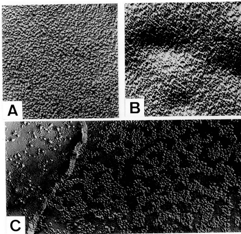
Fig. 13. Rearrangement of intramembrane particles during virus-induced cell fusion reaction. (A), Protoplasmic fracture face (PF) of freeze-cleaved intact erythrocytes. (B), The same as (A) except that intact cells were agglutinated by HVJ for 30 min in an ice bath, then subjected to freeze-fracturing. (C), PF (center to right) and external fracture face (EF, left) of intact cells which were agglutinated by HVJ (800 HAU/ml) for 30 min in an ice bath and incubated at 37^{\circ} for 30 min. Clustering of intramembrane particles took place all over the fracture face. Note that pits on the EF were also clustered and their pattern seemed to be continued to that of the particles on PF. \times 100,000 .
