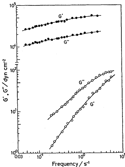
Figure III-8. Frequency dependence of G' and G'' at 25°C for an aqueous M-2 solution of 3.23 wt%. (O) and (●), before and after preheating at 150°C for 10 min, respectively.
