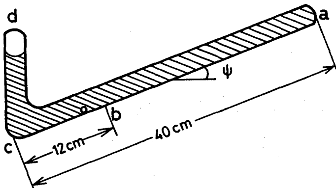
Figure III-1. Schematic diagram of a rolling-ball viscometer.
