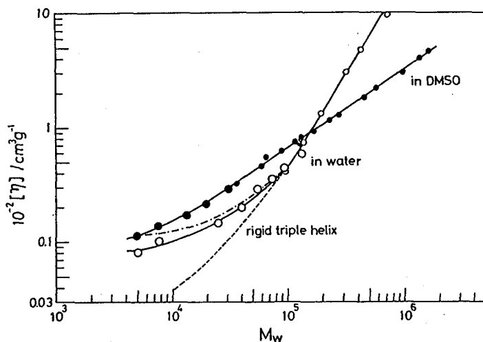
Figure IV-2. Double-logarithmic plots of [\eta] vs. M_w for schizophyllan in water and DMSO at 25°C. The smaller circles indicate the data obtained for higher-molecular weight samples in Chapter II, and the dashed and dot-dash lines represent, respectively, the calculated values for the schizophyllan triple helix with a pitch (per residue) of 0.30 nm and a diameter of 2.6 nm and for polymer mixtures consisting of triple helices and single randomly coiled chains.
