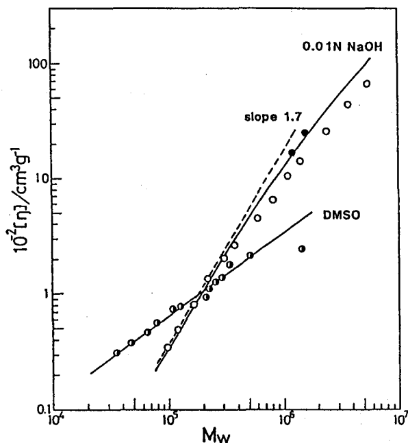
Figure V-10. Comparison of [\eta] data for Polytran scleroglucan in 0.01 N NaOH (○) and DMSO (●) with those (the solid lines) for schizophyllan 2 in the same solvents. The filled circles represent the data for Polytran samples H-1 and F-1 in 0.05 N NaOH.
