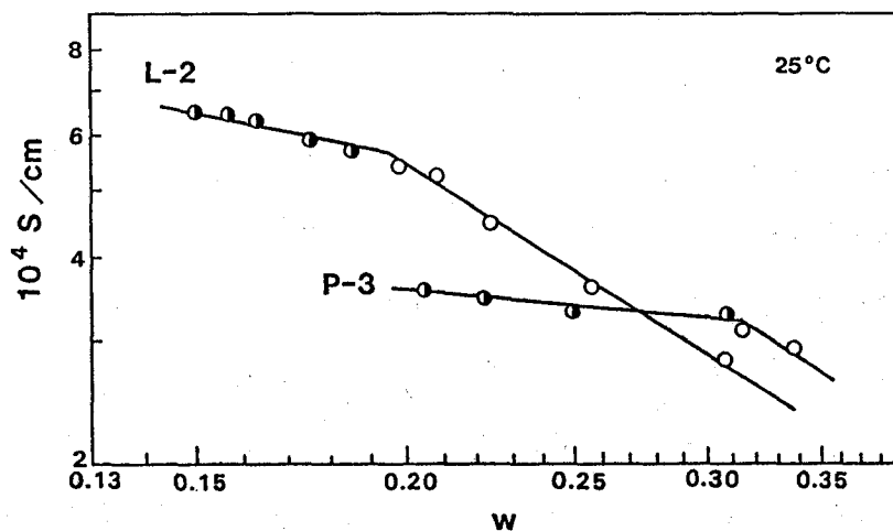
Figure VI-3. Double-logarithmic plots of S vs. w for samples L-2 and P-3 at 25°C. (●), biphasic solutions; (○), birefringent solutions.
