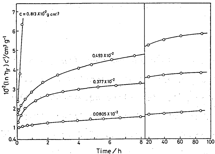
Figure III-7. Time dependence of (\ln \eta_r)/c at 25°C for aqueous solutions of sample M-2 preheated at 150°C for 10 min.
