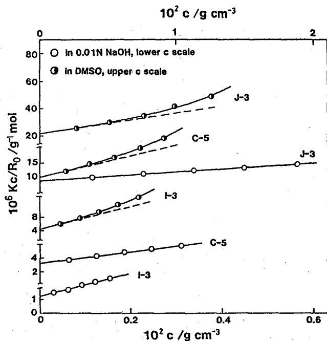
Figure V-7. Plots of Kc/R_0 vs. c for Polytran samples in 0.01 N NaOH (the lower c scale) and DMSO (the upper c scale) at 25°C.
