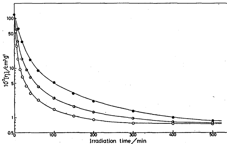
Figure II-1. Changes in \ln \eta of schizophyllan that occurred when aqueous solutions of concentrations 0.10 (O), 0.20 (◐), and 0.40 (●) \times 10^{-2} \text{ g cm}^{-3} were sonicated at 19.5 kHz.
