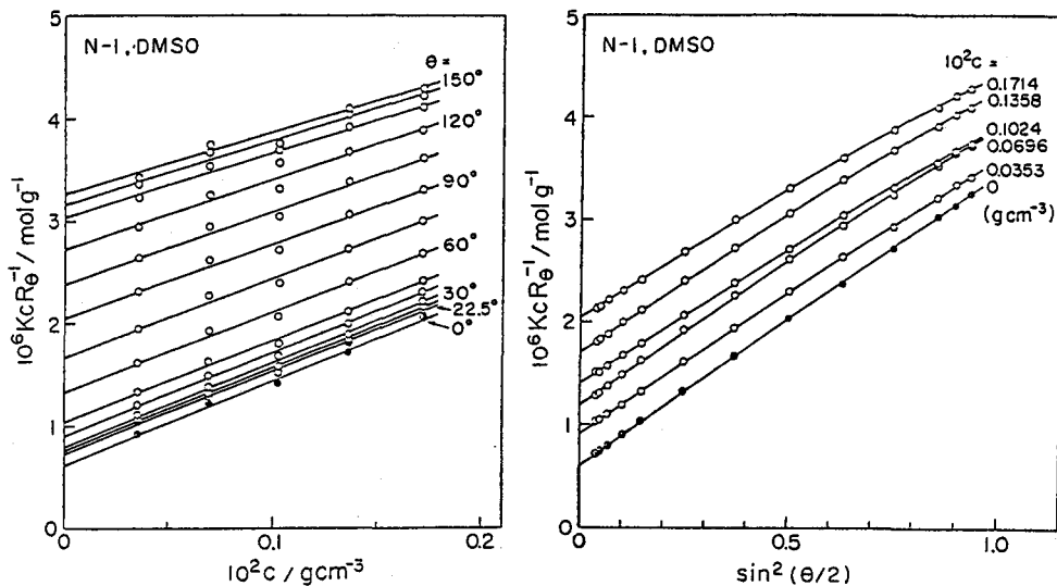
Figure II-7. Light-scattering envelopes for sample N-1 in DMSO at 25°C. K , the optical constant; R_\theta , the reduced scattering intensity; \theta , the scattering angle.
