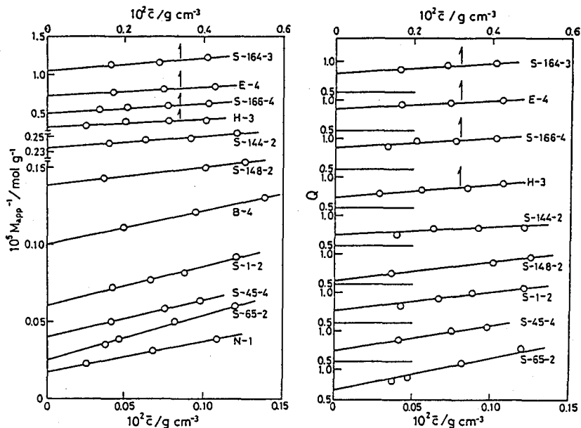
Figure II-5. Plots of M_{app}^{-1} vs. \bar{c} and Q vs. \bar{c} for indicated schizophyllan samples in water at 25°C.
