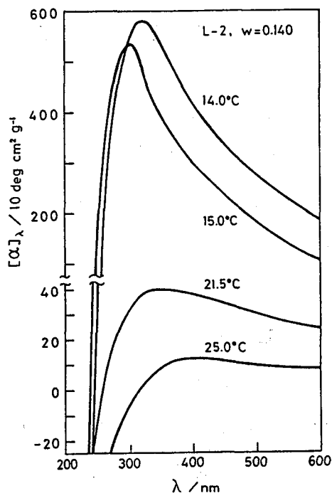
Figure VI-6. ORD curves for the solution of sample L-2 with w = 0.140 at different temperatures.
