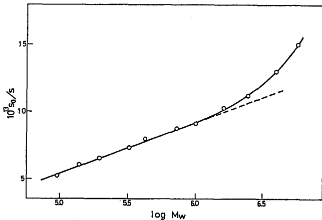
Figure II-10. Molecular weight dependence of s_0 for schizophyllan in water at 25°C.
