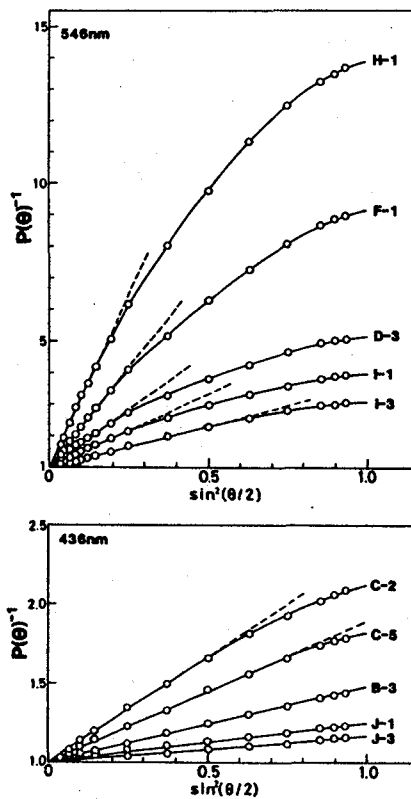
Figure V-8. Particle scattering functions for Polytran samples in 0.01 N NaOH at 25°C.
