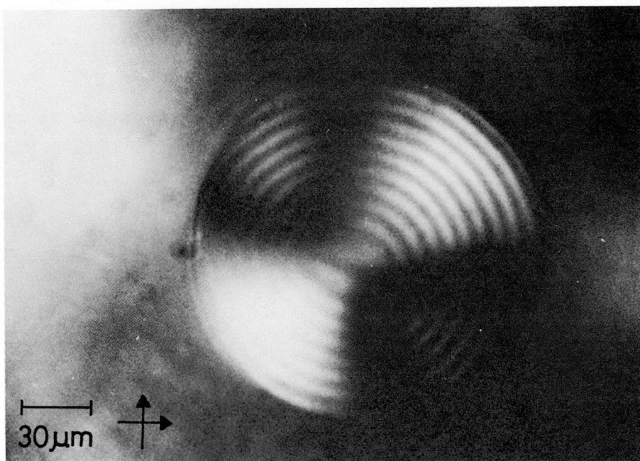
Figure VI-1. Spherulite in the aqueous solution of Polytran sample L-2 with w = 0.1567 at 25^{\circ}\text{C} . The bright region on the top left-hand side shows the reflection of light from another large spherulite in the solution.
