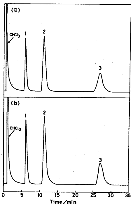
Figure V-3. Gas chromatograms of the acetylated products obtained from methylation experiments. (a), sample N-2; (b), sample S-2.
