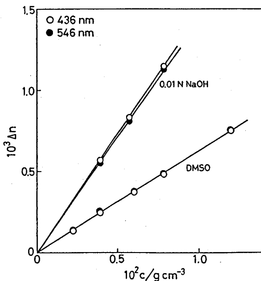
Figure V-2. Excess refractive indices \Delta n plotted against c for Polytran scleroglucan in 0.01 N aqueous NaOH and DMSO at 25°C.
