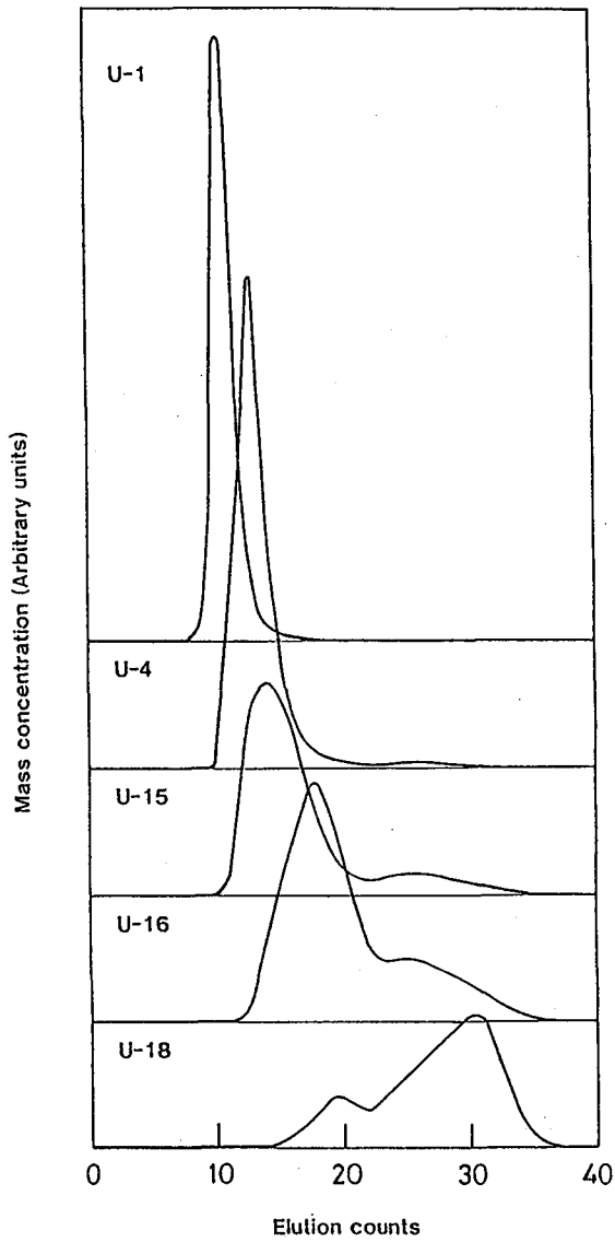
Figure IV-1. Gel-filtration chromatograms of schizophyllan samples in 0.05 M aqueous sodium acetate.
