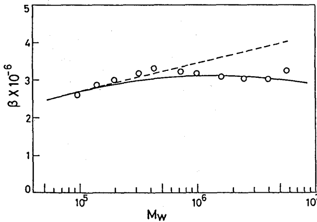
Figure II-15. Flory-Scheraga-Mandelkern parameter \beta (in conventional units) for schizophyllan in water at 25°C. The solid line refers to the wormlike cylinder with q = 200 nm, M_L = 2150 nm -1 , and d = 2.6 nm, and the dashed line to the rigid cylinder with the same M_L and d values.
