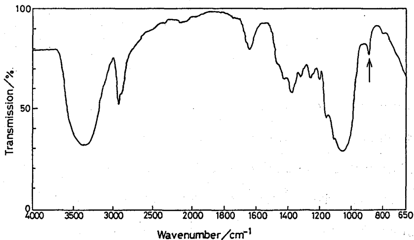
Figure V-6. IR spectrum for Polytran sample S-2.
