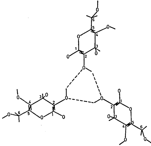
Figure II-12. Cyclic triad of hydrogen bonds among three schizophyllan chains. Hydrogen bonds are represented by dashed lines.
