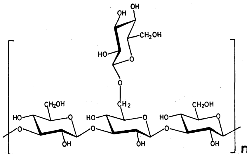
Figure I-1. Repeating unit of schizophyllan.
