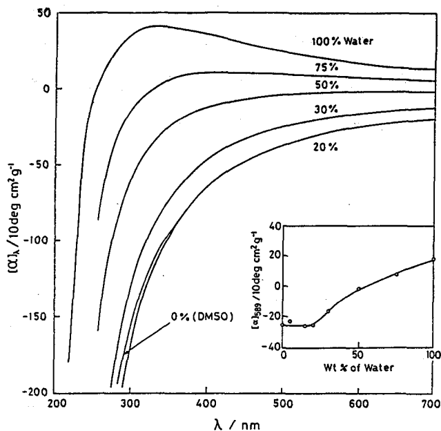
Figure III-3. ORD curves for sample S-144-2 in water-DMSO mixtures at 25°C. \lambda denotes the wavelength. The insert shows the composition dependence of [\alpha]_{589} for the same sample in the mixed solvents.
