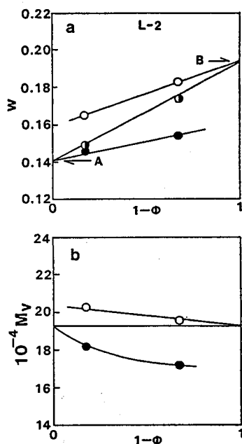
Figure VI-8. Phase separation data for sample L-2 at 25°C. (◐), biphasic mixtures; (●) and (O), separated isotropic and cholesteric solutions, respectively. Arrows A and B indicate A and B point concentrations determined by polarizing microscopy.
