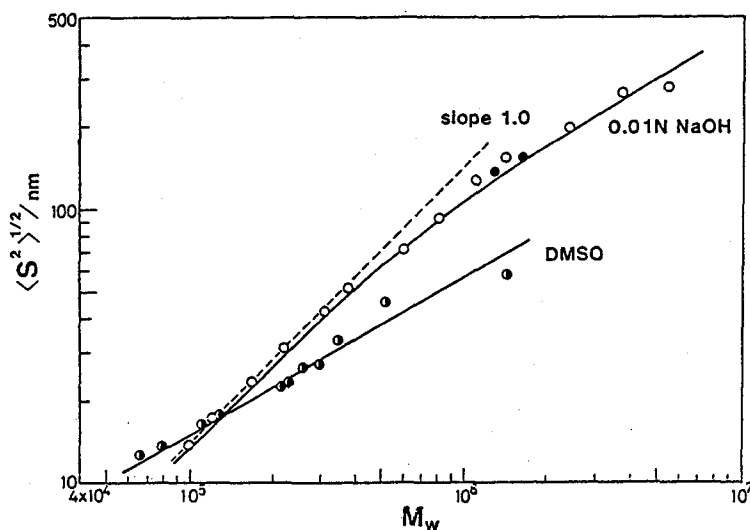
Figure V-9. Comparison of \langle S^2 \rangle^{1/2} data for Polytran scleroglucan in 0.01 N NaOH (○) and DMSO (●) with those (the solid lines) for schizophyllan 2 in the same solvents. The filled circles represent the data for Polytran samples H-1 and F-1 in 0.05 N NaOH.
