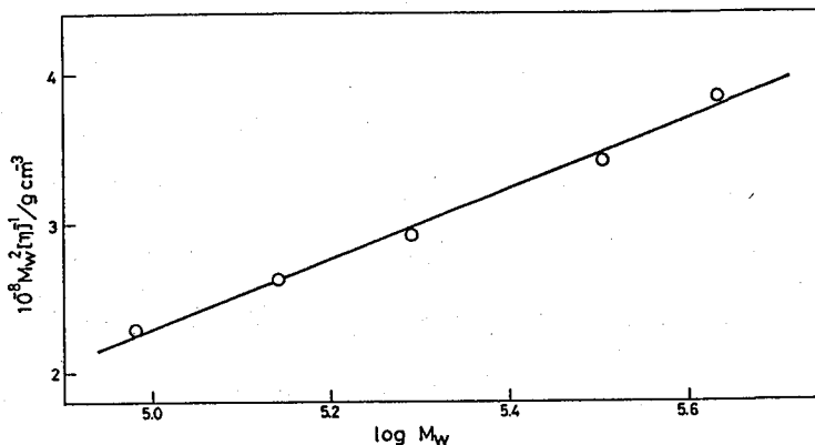
Figure II-13. Plot of M_w^2/|\eta| vs. \log M_w for schizophyllan in water at 25°C.
