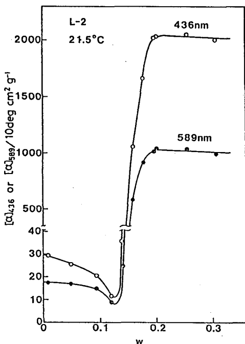
Figure VI-5. Concentration dependence of [\alpha]_{436} and [\alpha]_{589} for sample L-2.
