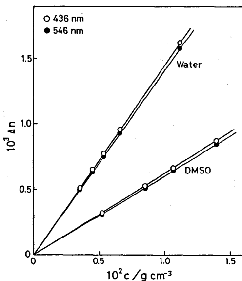
Figure II-3. Excess refractive indices \Delta n plotted against c for schizophyllan in water and DMSO at 25°C.
