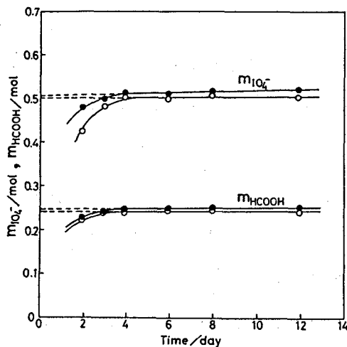
Figure V-4. Amount of periodate m_{IO_4^-} (moles per glucose residue) consumed and that of formic acid m_{HCOOH} produced by periodate oxidation of Polytran samples N-2 (○) and S-2 (●).
