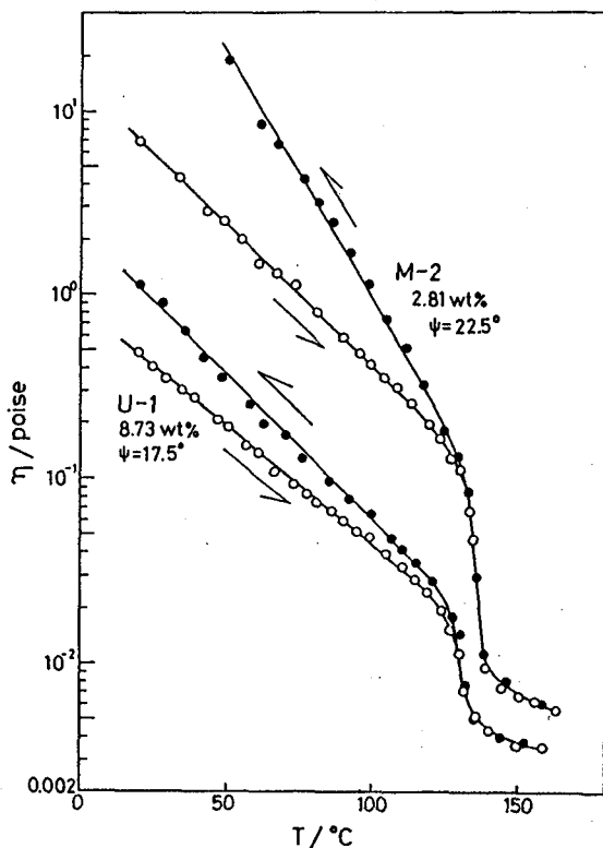
Figure III-5. Temperature dependence of \eta for schizophyllan samples M-2 and U-1 in pure water. Unfilled circles, heating; filled circles, cooling; rate of heating or cooling, 0.50 \pm 0.03 \text{ deg min}^{-1} .
