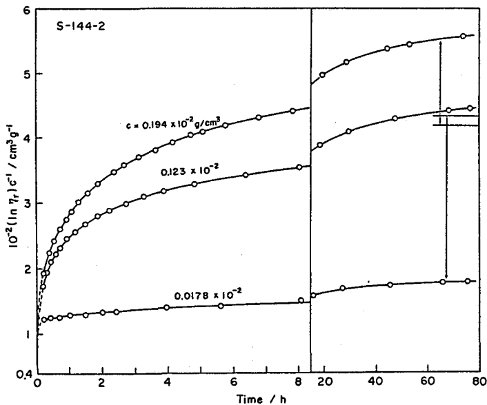
Figure III-4. Increases in (\ln \eta_r)/c with time after dilution of DMSO solutions of sample S-144-2 with water to 10 wt% DMSO. The values of c indicate the polymer concentrations in 10 wt% DMSO. See the text for the implication of the two segments.
