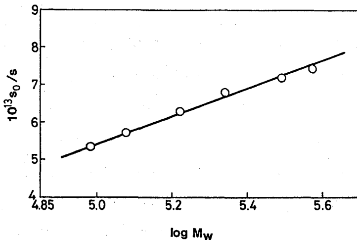
Figure V-12. Plot of s_0 vs. \log M_w for Polytran scleroglucan in 0.01 N NaOH.
