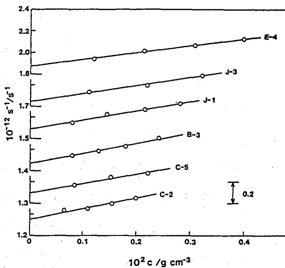
Figure V-11. Concentration dependence of s^{-1} for Polytran samples in 0.01 N NaOH at 25°C.
