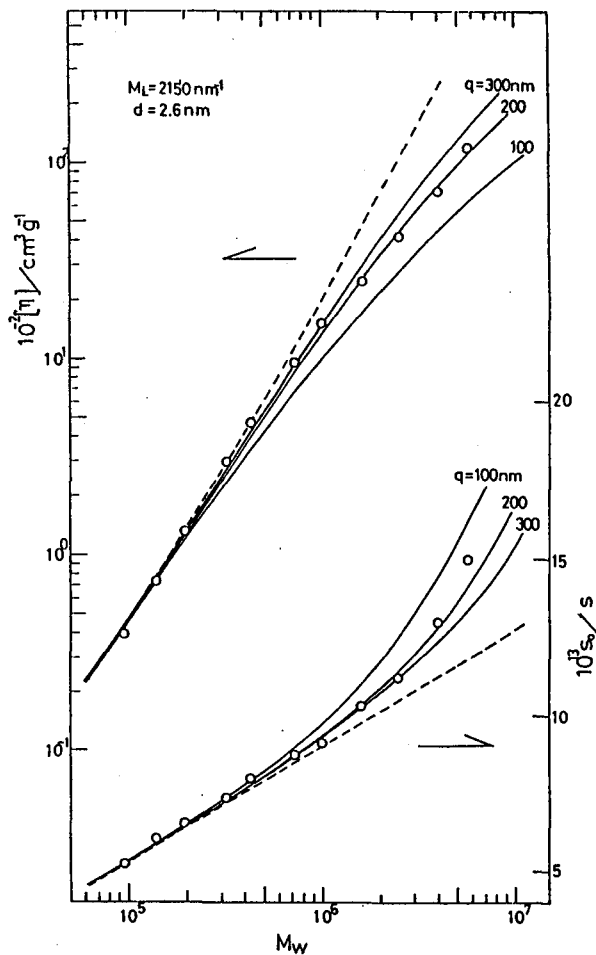
Figure II-14. Comparison of the experimental s_0 and \ln| for schizophyllan with the theoretical values for wormlike cylinders 3,5 calculated for q = 100, 200, 300 \text{ nm} , and \infty (the dashed lines) with M_L and d fixed to 2150 \text{ nm}^{-1} and 2.6 \text{ nm} , respectively.
