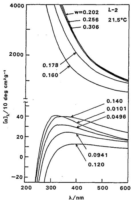
Figure VI-4. ORD curves for aqueous solutions of sample L-2 with different w at 21.5^{\circ}\text{C} .
