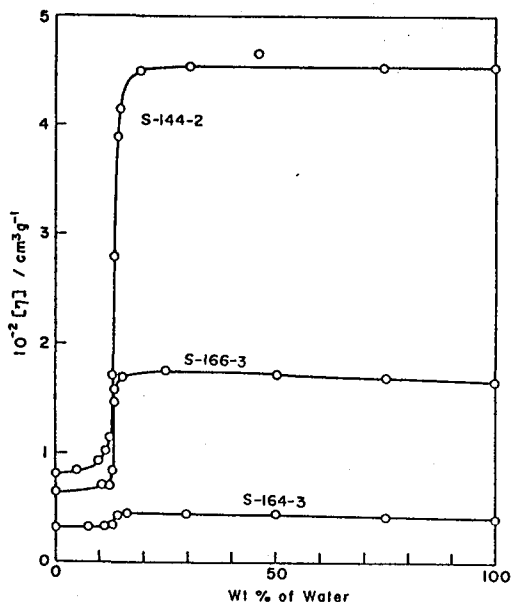
Figure III-2. Composition dependence of [\eta] for indicated schizophyllan samples in water-DMSO mixtures at 25°C.
