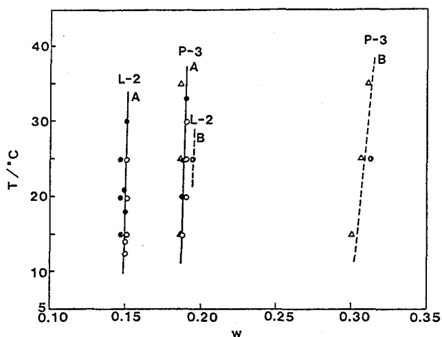
Figure VI-7. Phase diagrams for samples L-2 and P-3. Circles, from microscopic observations; triangles, from phase separation experiments.
