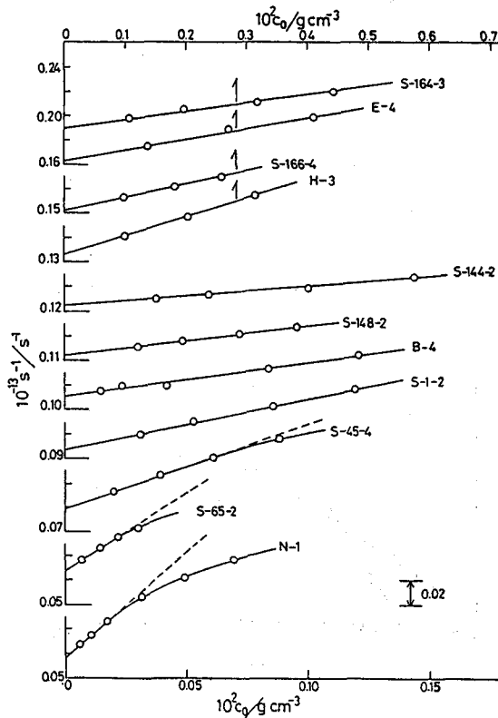
Figure II-9. Concentration dependence of s^{-1} for schizophyllan samples in water at 25^\circ\text{C} .
