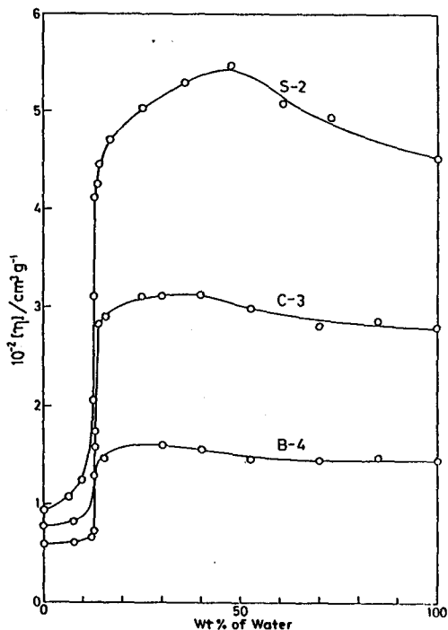
Figure V-13. Composition dependence of [\eta] for indicated Polytran samples in water-DMSO mixtures at 25°C.
