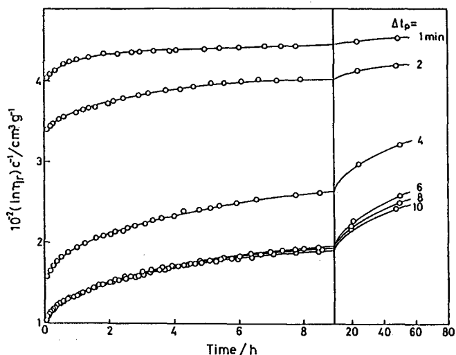
Figure III-6. Increases in (\ln \eta_r)/c at 25^\circ\text{C} with time that occurred after aqueous schizophyllan solutions preheated at 150^\circ\text{C} for periods \Delta t_p of 1 - 10 min were cooled to 25^\circ\text{C} . Sample, M-2; c , 0.106 \times 10^{-2} \text{ g cm}^{-3} .
