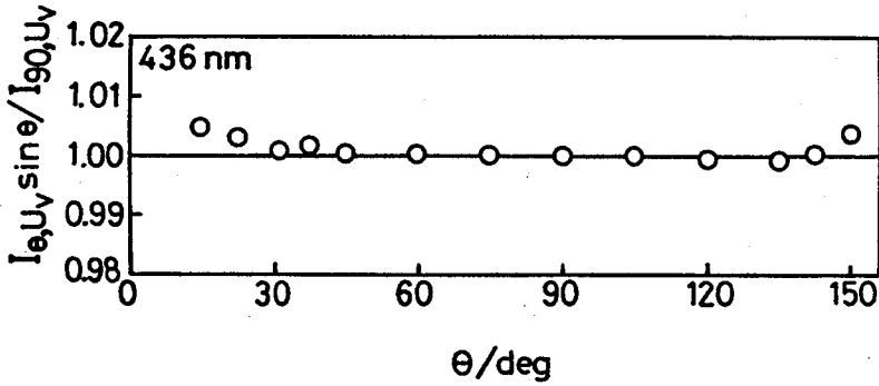
Figure V-1. Normalized intensities (I_{\theta, U_v} / I_{90, U_v}) \sin \theta for pure benzene at 25°C.
