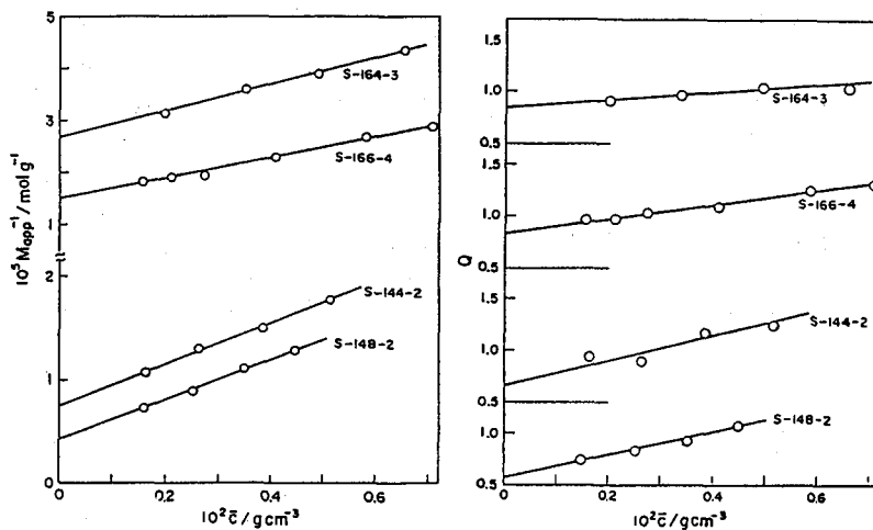
Figure II-6. Plots of M_{app}^{-1} vs. \bar{c} and Q vs. \bar{c} for indicated schizophyllan samples in DMSO at 25°C.
