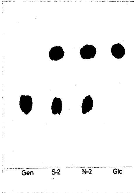
Figure V-5. Paper chromatograms of the enzymatic hydrolysates obtained from Polytran samples N-2 and S-2 with \text{exo-}\beta\text{-1,3-D-glucanase} , and those of glucose (Glc) and gentiobiose (Gen) as standard sugars.
