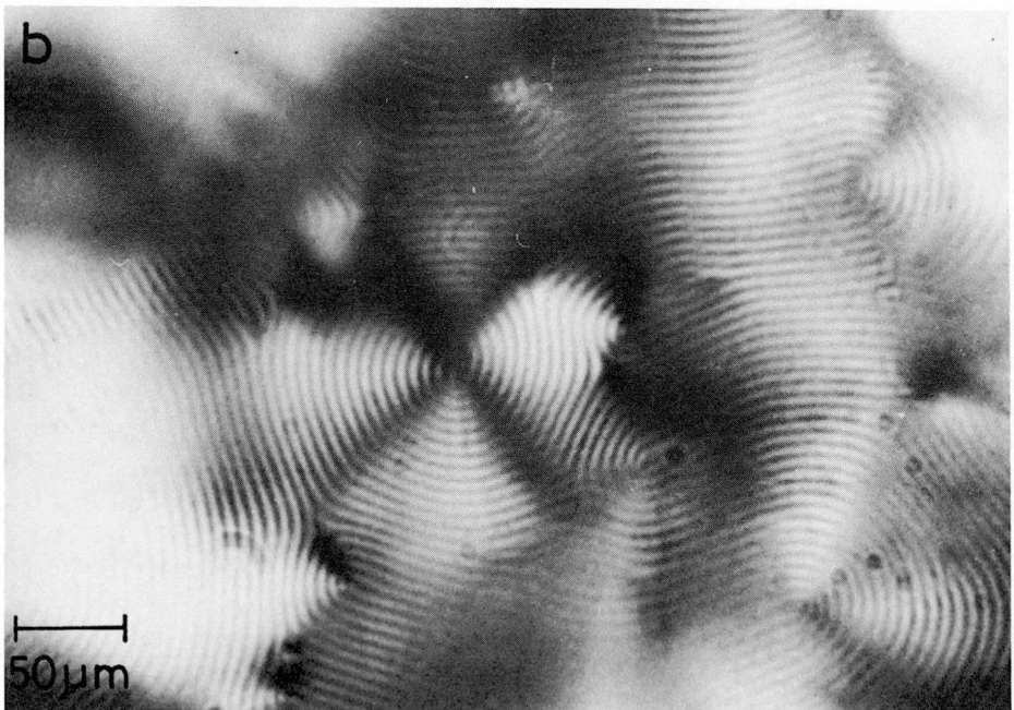
Figure VI-2. Microscopic patterns for the birefringent solution of sample L-2 with w = 0.2089 at 25^{\circ}\text{C} . (a), near the cell wall; (b), near the center of the cell.
