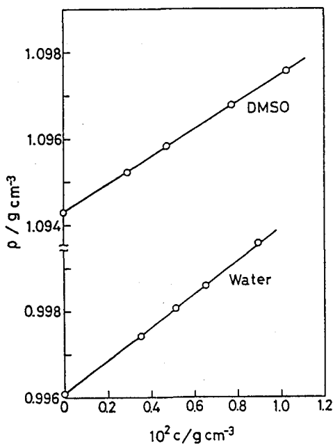
Figure II-2. Densities \rho of aqueous or DMSO solutions of schizophyllan as a function of c .
