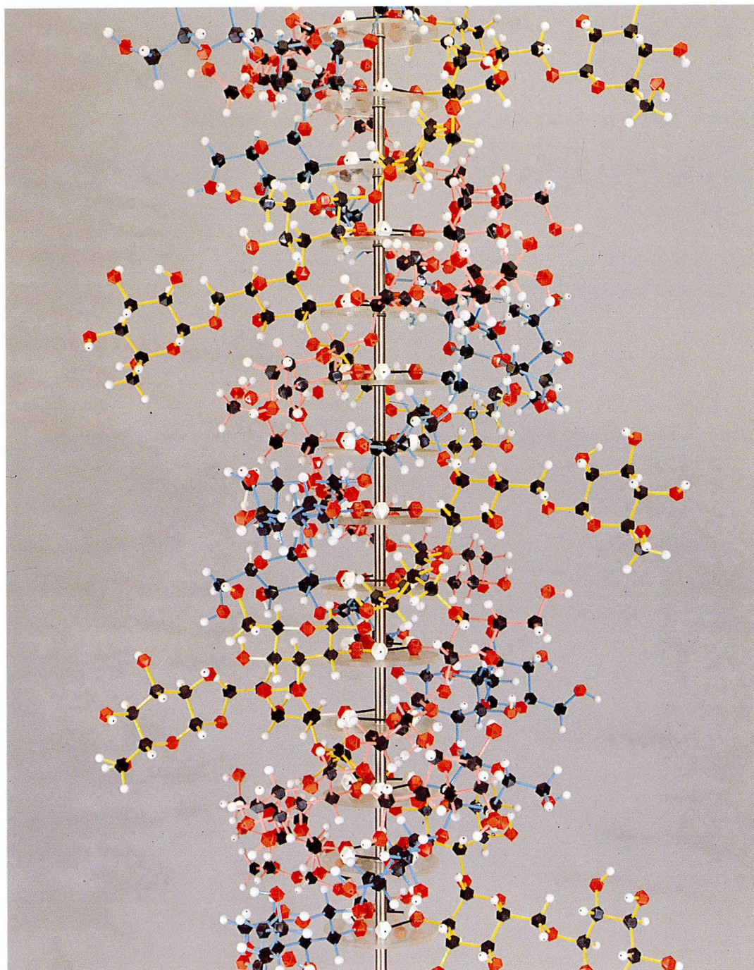
Figure II-11. Molecular model of the schizophyllan triple helix.
