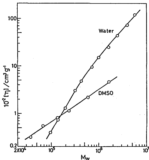
Figure II-8. Double logarithmic plots of [\eta] vs. M_w for schizophyllan in water and DMSO at 25°C.
