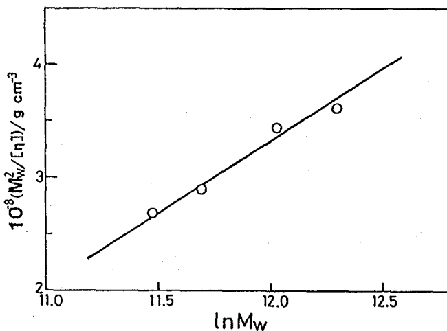
Figure V-14. Plot of M_w^2 / [\eta] vs. \ln M_w for Polytran scleroglucan in 0.01 N NaOH.
