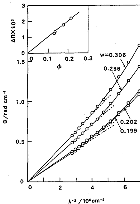
Figure VI-9. Plots of \Theta vs. \lambda^{-2} for sample L-2. The insert shows the dependence of the layer birefringence \Delta n on polymer volume fraction.
