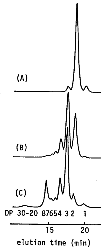
Figure A-3-2. GPC curves of oligo(MMA)s derived from oligo(TrMA)s prepared with Sp-EtFlLi at [TrMA]/[Li]=2 (A), 3 (B), and 5 (C).
