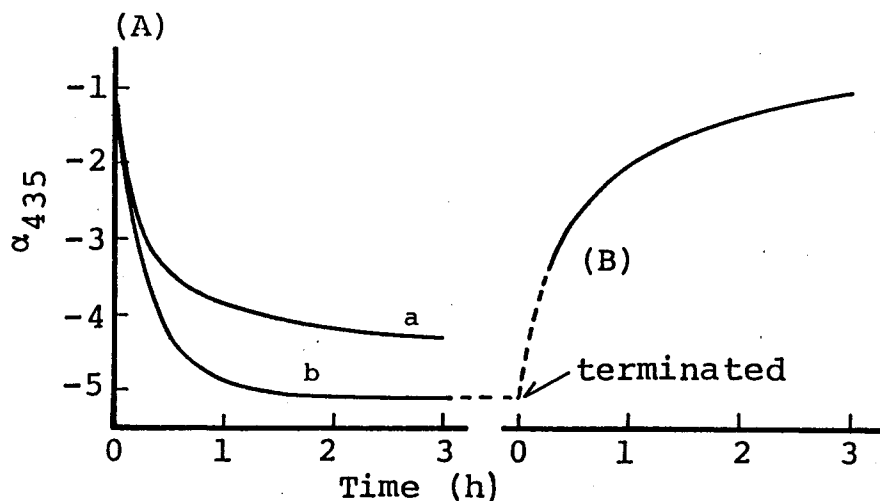
Figure B-2-2. Change of optical activity of polymerization systems of DMPMA with TMEDA-DPEDA-Li in toluene at -40^{\circ}\text{C} (A) and at room temperature after termination (B); a: [\text{DMPMA}]/[\text{Li}]=40 and b: [\text{DMPMA}]/[\text{Li}]=20 .
