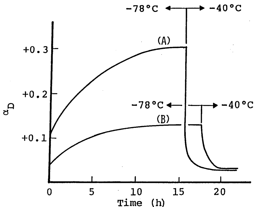
Figure B-1-1. Change of optical activity of polymerization systems of CPDPMA with DDB-DPEDA-Li (A) and with PMP-DPEDA-Li (B) in toluene at -78°C and -40°C. (CPDPMA 0.15 g, toluene 3 ml, [CPDPMA]/[Li]=20, cell length 1.0 cm)
