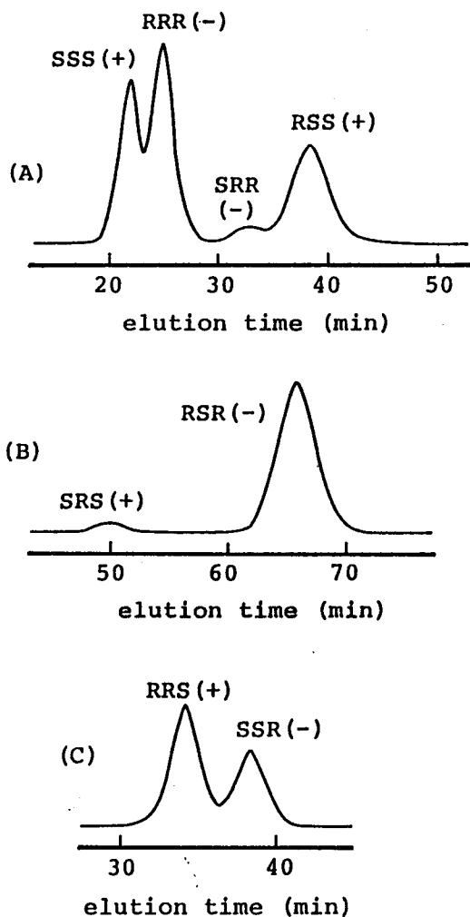
Figure A-1-12. Chromatograms of optical resolution of MMA-trimers mm and mr (A), rr (B), and mr (C) derived from TrMA-trimers prepared with Sp-F1Li at [TrMA]/[Li]=3 .
