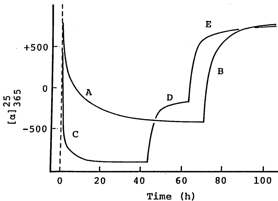
Figure B-2-4. Change of specific rotation of poly(DMPMA) of DP=37 (Run 5 in Table B-2-1) in the mixtures of \text{CH}_3\text{OH} and acids at 25^\circ\text{C} ; in \text{CH}_3\text{OH} -0.01% \text{CH}_3\text{SO}_3\text{H} (curve A), in \text{CH}_3\text{OH} -13.0% \text{CH}_3\text{SO}_3\text{H} (curve B), in \text{CH}_3\text{OH} -1.5% \text{CF}_3\text{CO}_2\text{H} (curve C), in \text{CH}_3\text{OH} -0.9% \text{CF}_3\text{CO}_2\text{H} -0.5% \text{CH}_3\text{SO}_3\text{H} (curve D), and in \text{CH}_3\text{OH} -0.5% \text{CF}_3\text{CO}_2\text{H} -9.5% \text{CH}_3\text{SO}_3\text{H} (curve E).
