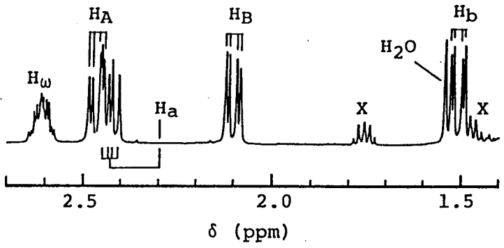
Figure A-1-8. 500 MHz ^1\text{H} NMR spectra of MMA-dimers meso (A) and racemo (B) ( \text{CDCl}_3 , 35^\circ\text{C} , TMS).
