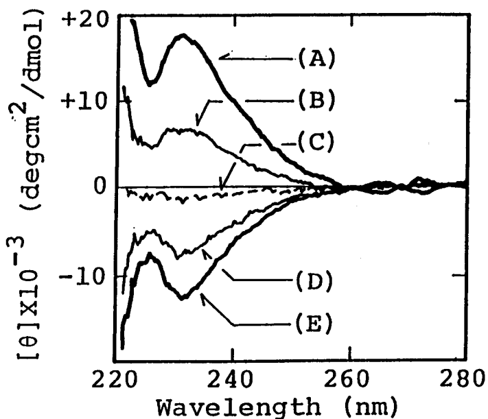
Figure B-1-6. Change of CD spectra of poly(CHDPMA) of DP=34 (Run 1 in Table B-1-3) in \text{CHCl}_3 at 60^\circ\text{C} : 0 min (A), 5 min (B), 10 min (C), 20 min (D), and 60 min (E) after dissolution in \text{CHCl}_3 .
