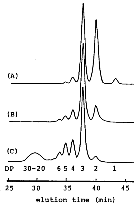
Figure A-1-5. GPC curves of oligo-(MMA)s derived from oligo(TrMA)s prepared with PMP-FILi at [\text{TrMA}]/[\text{Li}] = 2 (A), 3 (B), and 5 (C).
