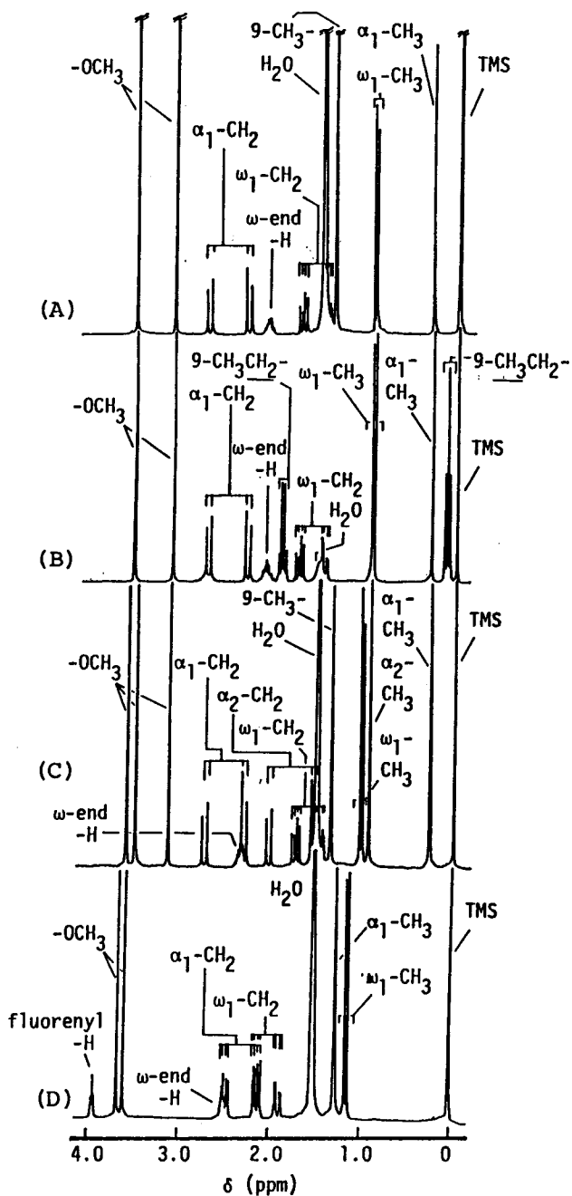
Figure A-3-4. 270 MHz ^1\text{H} NMR spectra of MMA-dimer m having a 9-methylfluorenyl group at the \alpha -end (A), MMA-dimer m having a 9-ethylfluorenyl group (B), MMA-trimer mm having a 9-methylfluorenyl group (C), and MMA-dimer m having a fluorenyl group (D). ( \text{CDCl}_3 , 35^\circ\text{C} , TMS)
