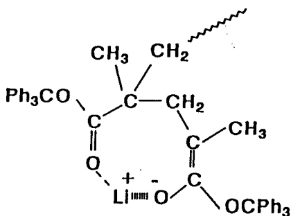
Scheme A-1-2. Intramolecular solvation of \omega -end anion.
