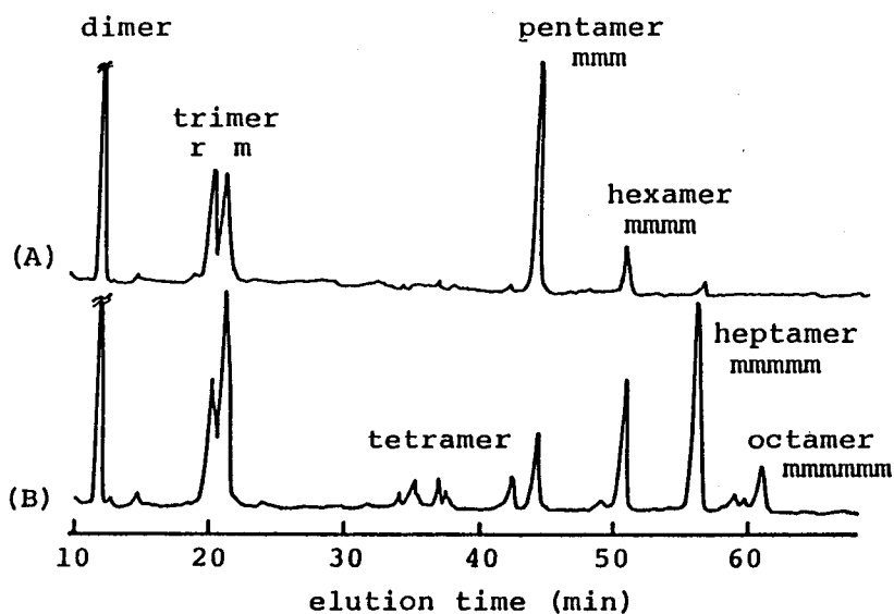
Figure A-2-2. Chromatograms of separation of diastereomers of oligo(MMA)s derived from oligo(TrMA)s prepared with Sp-F1Li at [TrMA]/[Li]=3 (A) and 5 (B) and terminated with methyl iodide.
