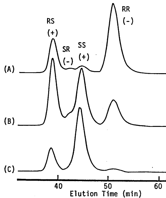
Figure A-2-4. Chromatograms of optical resolution of MMA-trimer derived from TrMA-trimer prepared with Sp-FlLi at [TrMA]/[Li]=2 (A) and 3 (B) and terminated with methyl iodide.
