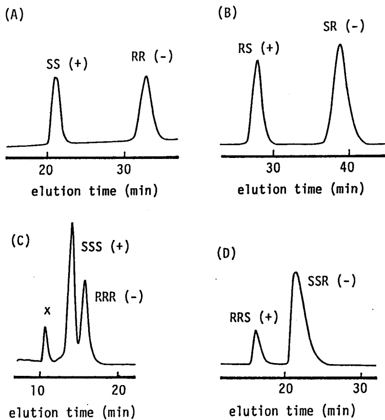
Figure A-3-6. Chromatograms of optical resolution of MMA-dimers m (A) and r (B) and MMA-trimers mm (C) and mr (D) derived from corresponding oligo(TrMA) prepared with Sp-EtFlLi at [TrMA]/[Li]=2 .
