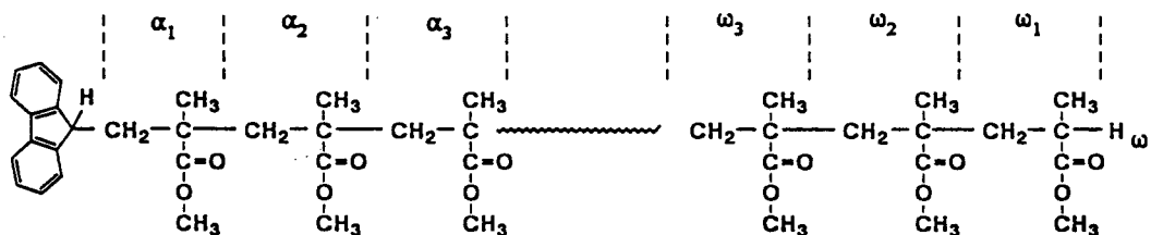
Scheme A-1-1. Structure and numbering system of monomeric units of oligo- and poly(MMA) having a fluorenyl group at the \alpha -end.
