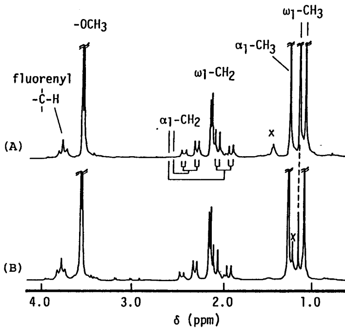
Figure A-2-5. 100 MHz ^1\text{H} NMR spectra of MMA-dimer derived from TrMA-dimer prepared with Sp-FlLi at [\text{TrMA}]/[\text{Li}]=2 and terminated with methyl iodide (A) and methyl iodide -\text{d}_3 (B). ( \text{CDCl}_3 , 35^\circ\text{C} , TMS).
