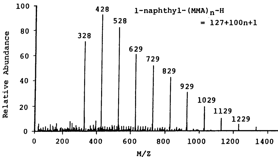
Figure B-4-2. FD mass spectrum of hexane-soluble oligo(MMA) prepared with 1-NpMgBr.
