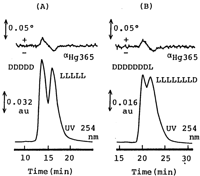
Figure B-4-5. Chromatograms of MMA-pentamer mmmmm (A) and octamer mmmmmmmr (B) prepared with l-NpMgBr (sample 2.1 mg (A), 2.0 mg (B)).
