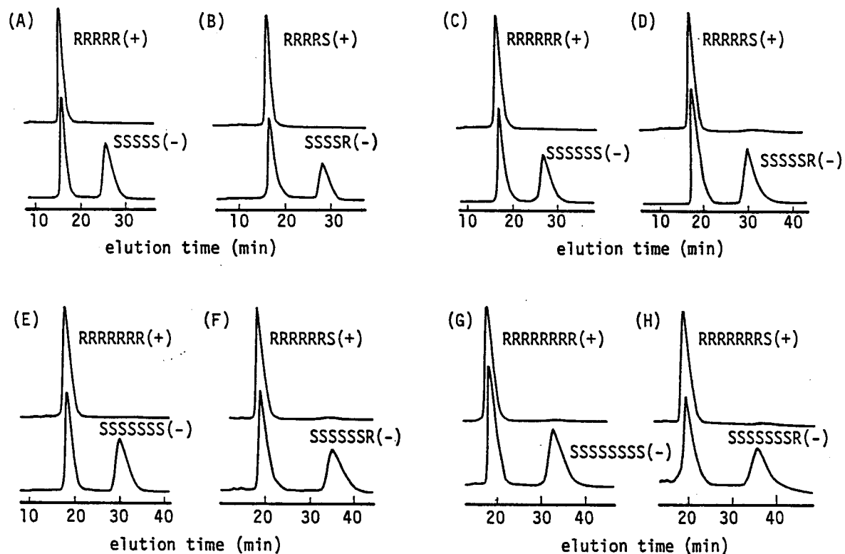
Figure A-1-13. Chromatograms of optical resolution of MMA-pentamers mmmm (A) and mmmr (B), MMA-hexamer mmmm (C) and mmmmr (D), MMA-heptamer mmmmmm (E) and mmmmmr (F), and MMA-octamer mmmmmmmm (G) and mmmmmmmr (H) derived from corresponding TrMA-oligomers prepared with Sp-FlLi and corresponding racemic TrMA-oligomers prepared with FlLi in THF (top of each: optically active oligomers, bottom of each: racemic oligomers). Pentamers and hexamers were isolated from the products of oligomerization at [TrMA]/[Li]=3 and heptamers and octamers from those at [TrMA]/[Li]=5 .
