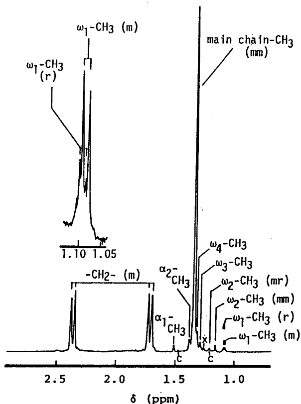
Figure A-1-1. 500 MHz ^1\text{H} NMR spectrum of poly(MMA) derived from benzene-hexane (1/1 v/v)-insoluble poly(TrMA) of DP = 60 (Run 1 in Table A-1-1) (nitrobenzene- d_5 , 110^\circ\text{C} ). c and x denote ^{13}\text{C} satellite bands of the main chain- \text{CH}_3 signal and impurity, respectively.
