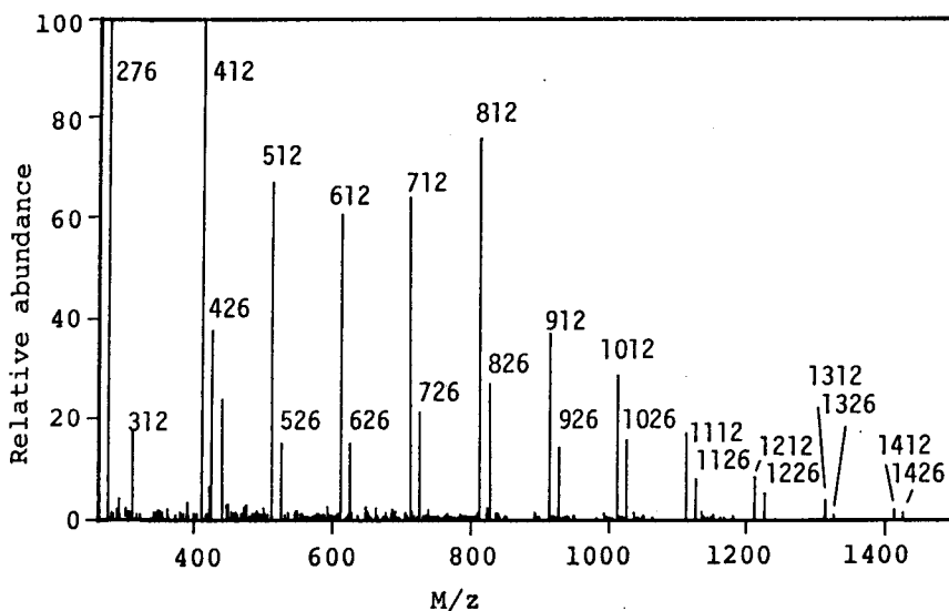
Figure B-3-2. FD mass spectrum of oligo(MMA) derived from oligo(D2PyMA) prepared with PMP-DPEDA-Li at [D2PyMA]/[Li]=3 in toluene at -78^{\circ}C . The peak of M/z=276 corresponds to the molecular weight of methyl diphenyl-2-pyridylmethyl ether produced in the process of conversion of ester group.
