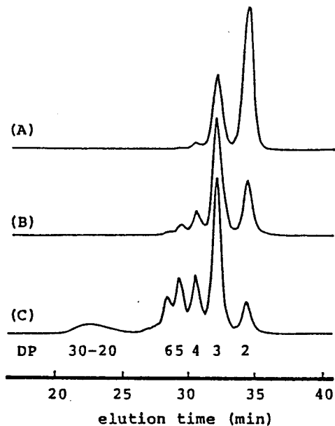
Figure A-1-4. GPC curves of oligo-(MMA)s derived from oligo(TrMA)s prepared with DDB-FILi at [\text{TrMA}]/[\text{Li}] = 2 (A), 3 (B), and 5 (C).
