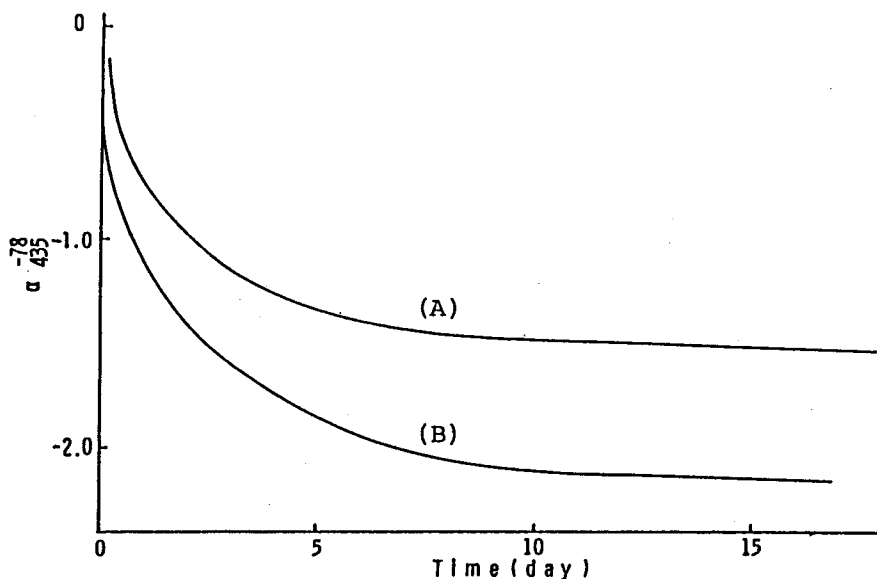
Figure B-2-1. Change of optical activity of polymerization systems of DMPMA with (+)-DDB-DPEDA-Li (A) and with TMEDA-DPEDA-Li (B) in toluene at -78^{\circ}\text{C} . (DMPMA 0.15 g, toluene 3 ml, [\text{DMPMA}]/[\text{Li}]=20 , cell length 1.0 cm)
