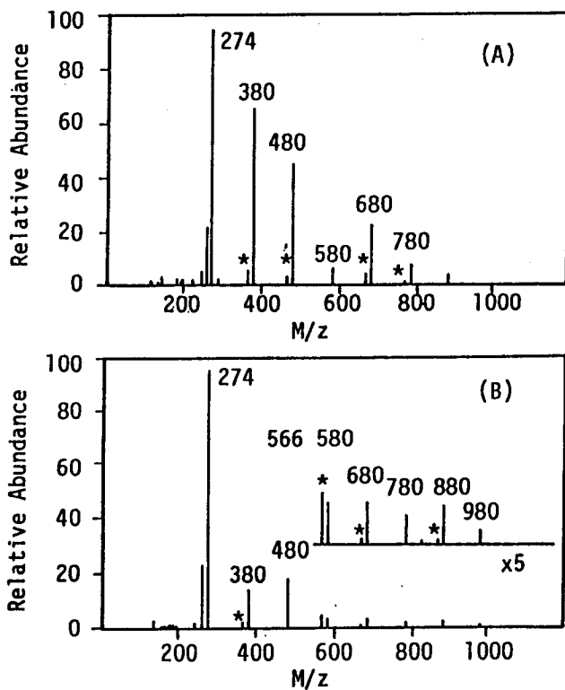
Figure A-2-1. FD mass spectra of oligo(MMA)s derived from oligo(TrMA)s prepared with Sp-F1Li at [TrMA]/[Li] =3 (A) and 5 (B) and terminated with methyl iodide. * denotes the peaks of M/z of oligo(MMA) having a hydrogen at the \omega -end.
