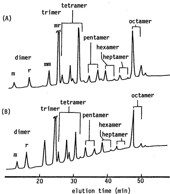
Figure A-3-3. Chromatograms of separation of diastereomers of oligo(MMA)s derived from oligo(TrMA)s prepared with Sp\text{-MeFlLi} (A) and Sp\text{-EtFlLi} (B) at [\text{TrMA}]/[\text{Li}]=5 .
