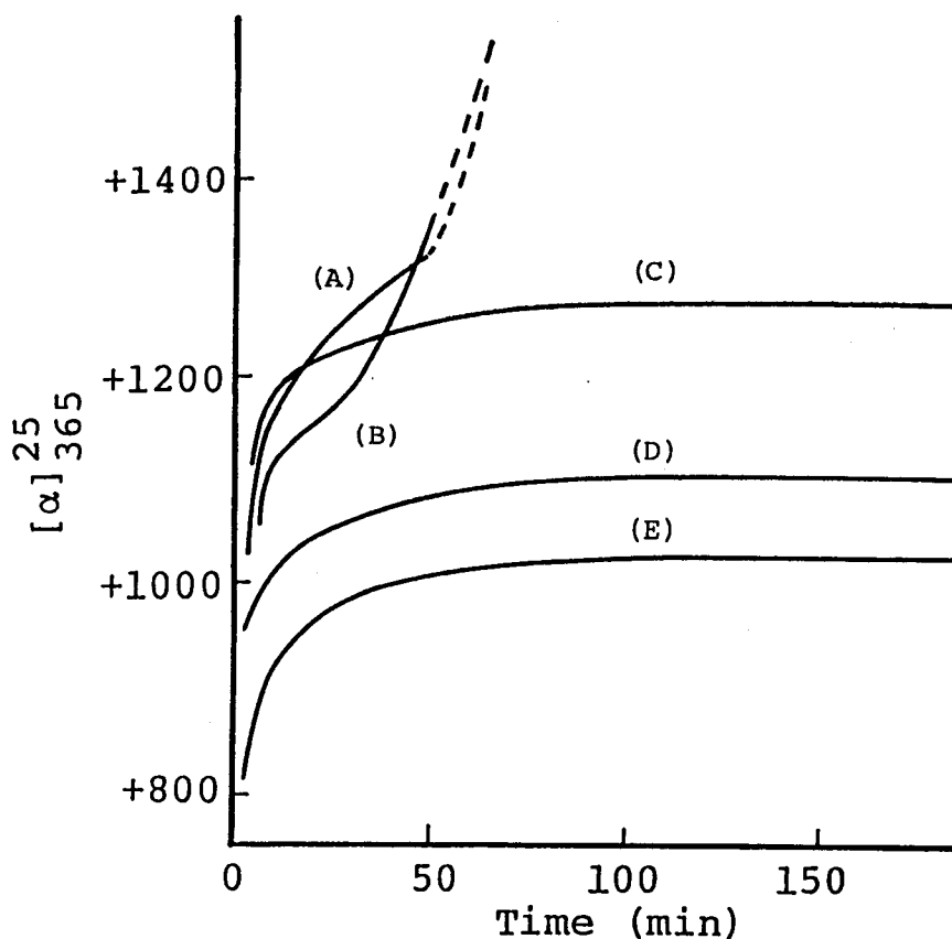
Figure B-2-3. Change of specific rotation of poly(DMPMA)s of DP=130 (A), 160 (B), 105 (C), 65 (D), and 37 (E) in \text{CH}_3\text{OH}-20\%\text{CH}_3\text{SO}_3\text{H} at 25^\circ\text{C} .
