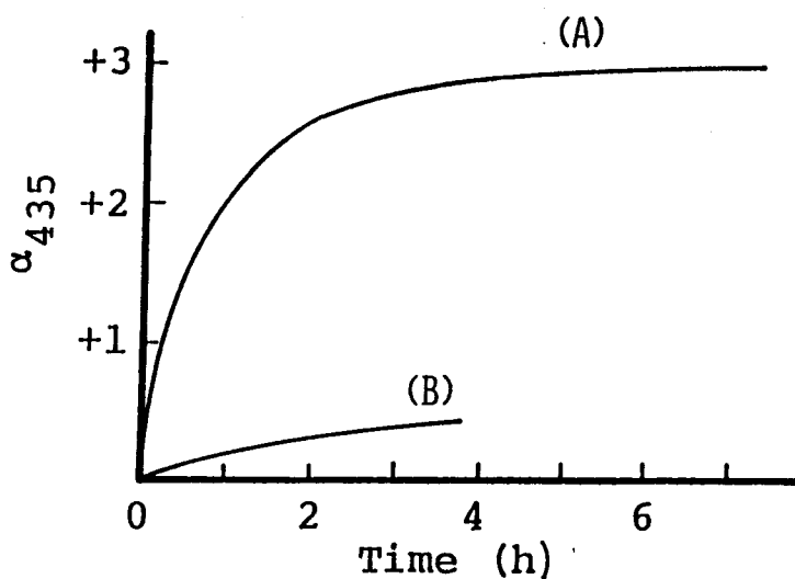
Figure B-1-4. Change of optical activity of polymerization systems of CHDPMA with PMP-DPEDA-Li at -78°C (A) and with DDB-DPEDA-Li at -40°C (B) in toluene. (CHDPMA 0.15 g, toluene 3 ml, [CHDPMA]/[Li]=20, cell length 1.0 cm)
