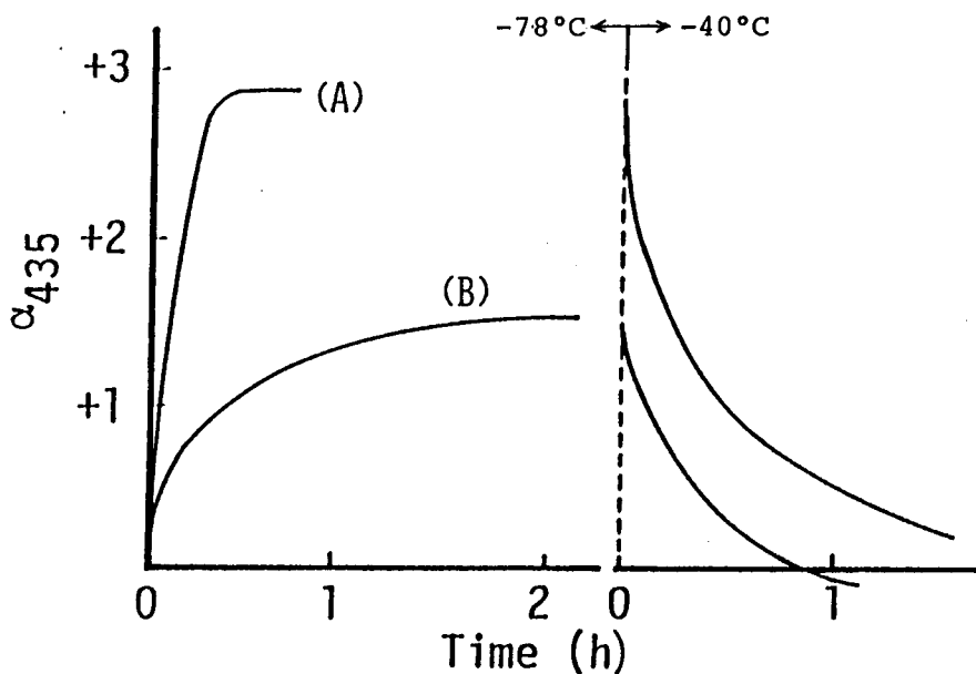
Figure B-1-2. Change of optical activity of polymerization systems of CBDPMA with DDB-DPEDA-Li (A) and with PMP-DPEDA-Li (B) in toluene at -78^{\circ}\text{C} and -40^{\circ}\text{C} . (CBDPMA 0.15 g, toluene 3 ml, [\text{CBDPMA}]/[\text{Li}]=20 , cell length 1.0 cm)
