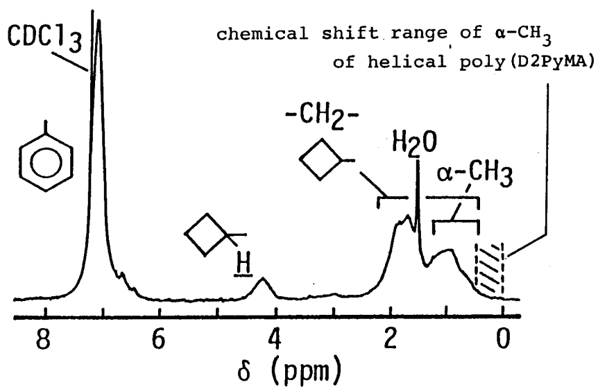
Figure B-1-3. 200 MHz 1 H NMR spectrum of poly(CBDPMA) of DP=29 (Run 1 in Table B-1-2). (CDCl 3 , 25°C)
