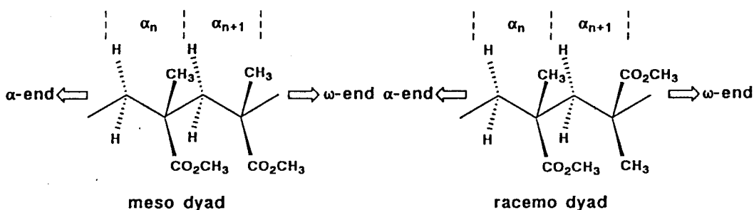
Scheme A-1-3. Meso and racemo dyads in the main chain of oligo- and poly(MMA).
