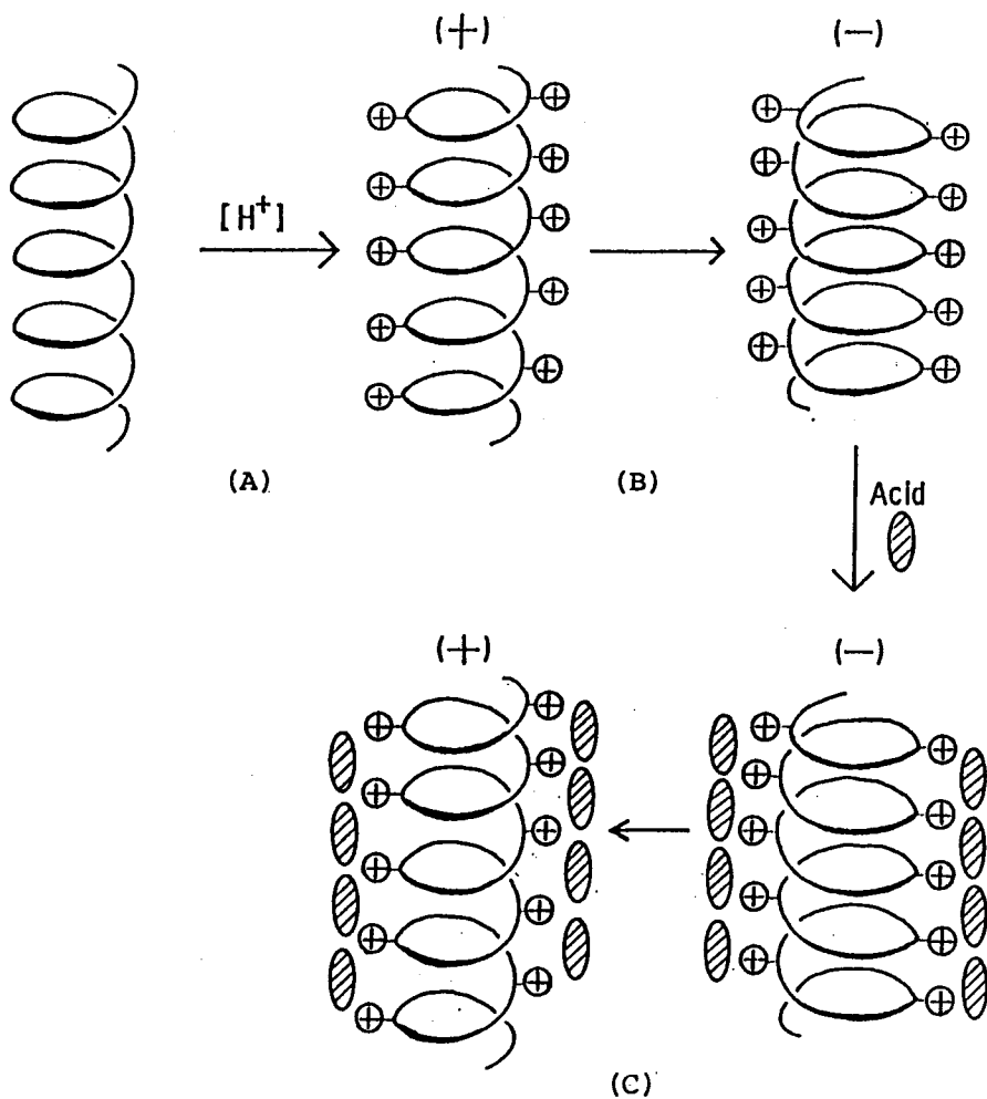
Scheme B-2-1. A possible mechanism of reversible helix-helix transition of poly(DMPMA) dependent on acidity of solution.
