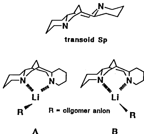
Scheme A-1-6. Transoid Sp and two types of complexes of cisoid Sp with oligomer anion.
