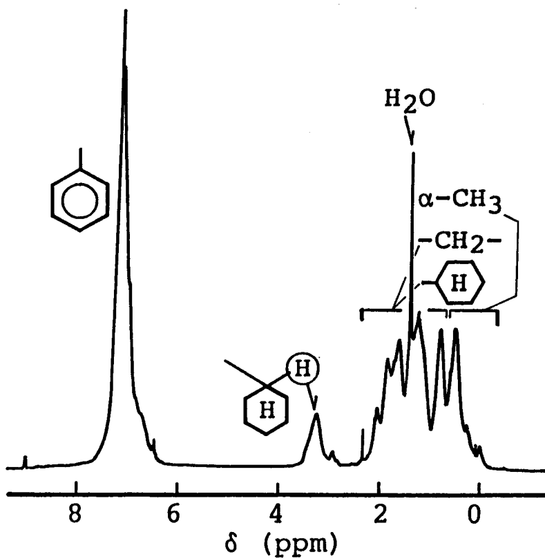
Figure B-1-7. 270 MHz ^1\text{H} NMR spectrum of poly(CHDPMA) of DP=34 (Run 1 in Table B-1-3). ( \text{CDCl}_3 , 60^\circ\text{C} )
