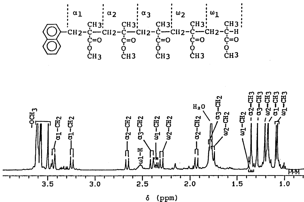
Figure B-4-4. 500 MHz ^1\text{H} NMR spectrum of MMA-pentamer mmmmr having a 1-naphthyl group at the \alpha -end. (Nitrobenzene- d_5 , 110°C)
