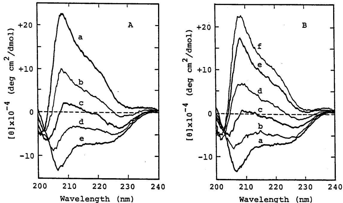
Figure B-2-5. Change of CD spectra of poly(DMPMA) of DP=37 (Run 5 in Table B-2-1) at 25°C. A: in \text{CH}_3\text{OH}-0.01\%\text{CH}_3\text{SO}_3\text{H} ; (a) immediately after dissolution ( [\alpha]_{365}^{25} +780^\circ ), (b) 2 h 5 min ( +240^\circ ), (c) 4 h 4 min ( +81^\circ ), (d) 22 h 18 min ( -163^\circ ), and (e) 70 h ( -410^\circ ). B: in \text{CH}_3\text{OH}-13\%\text{CH}_3\text{SO}_3\text{H} after completion of the change in A; (a) the last spectrum in A, (b) 5 min after the addition of \text{CH}_3\text{SO}_3\text{H} (13%) ( -278^\circ ), (c) 52 min ( -26^\circ ), (d) 2 h 30 min ( +252^\circ ), (e) 16 h 20 min ( +570^\circ ), and (f) 30 h ( +779^\circ ).
