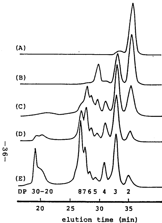
Figure A-1-3. GPC curves of oligo-(MMA)s derived from oligo(TrMA)s prepared with Sp-FILi at [\text{TrMA}]/[\text{Li}] = 2 (A), 3 (B), 5 (C), 10 (D), and 20 (E).
