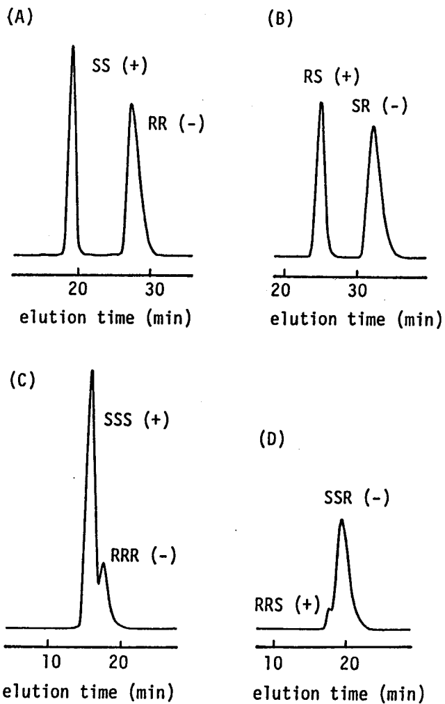
Figure A-3-5. Chromatograms of optical resolution of MMA-dimers m (A) and r (B) and MMA-trimers mm (C) and mr (D) derived from corresponding oligo(TrMA) prepared with Sp-MeFlLi at [\text{TrMA}]/[\text{Li}]=2 .
