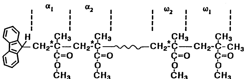
Scheme A-2-1. Structure and numbering system of monomeric units of oligo(MMA) having two \text{CH}_3 groups at the \omega -end. * denotes asymmetric centers.
