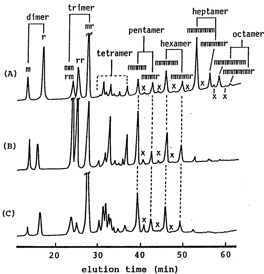
Figure A-1-6. Chromatograms of separation of diastereomers of oligo(MMA)s derived from oligo(TrMA)s prepared with Sp-FlLi (A), DDB-FlLi (B), and PMP-FlLi (C) at [\text{TrMA}]/[\text{Li}] = 5 .
