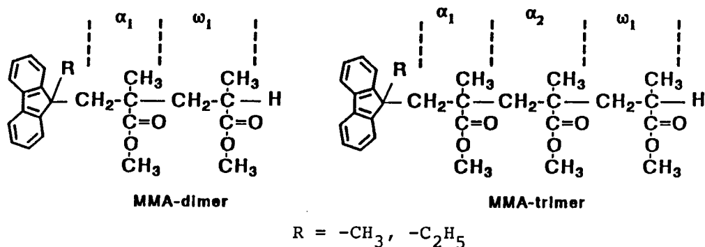
Scheme A-3-2. Structure and numbering system of monomeric units of MMA-dimer and -trimer having a 9-methylfluorenyl or a 9-ethylfluorenyl group at the \alpha -end.
