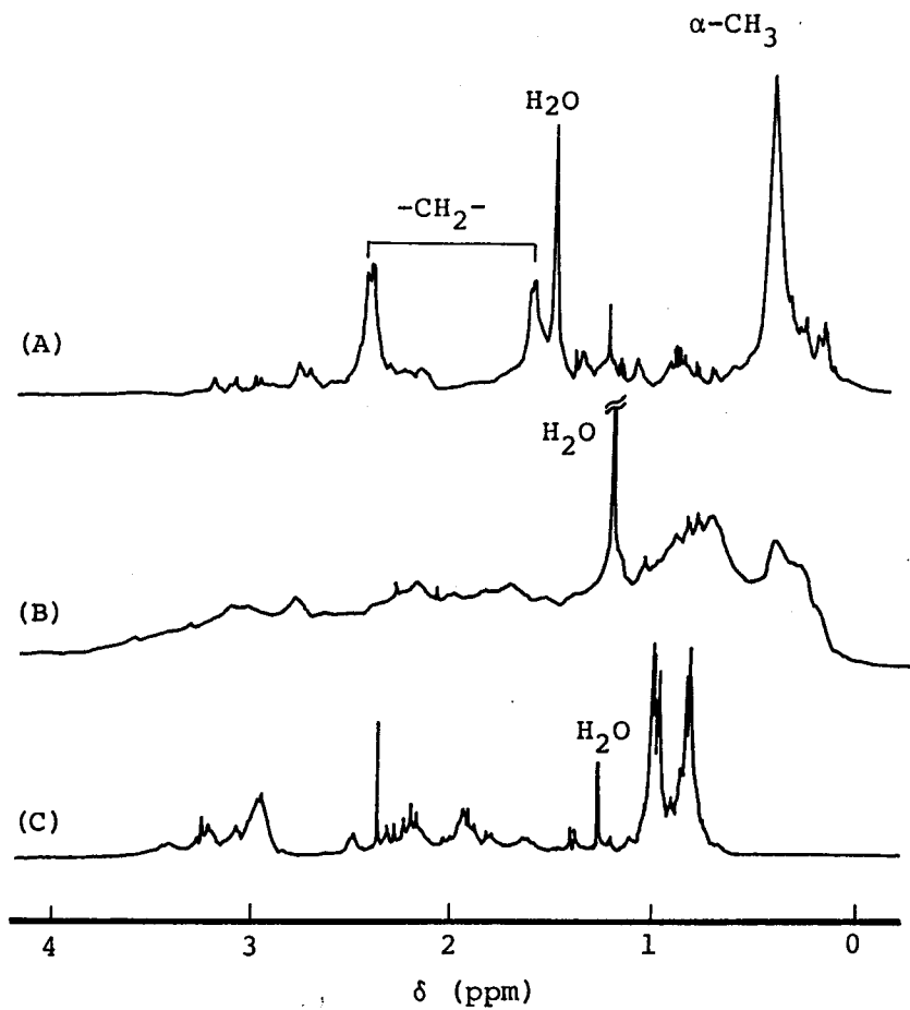
Figure B-3-3. 500 MHz ^1\text{H} NMR spectra of poly(D2PyMA) of DP=27 at 35°C (A), oligomer A at 30°C (B), and oligomer B at 35°C. ( \text{CDCl}_3 )
