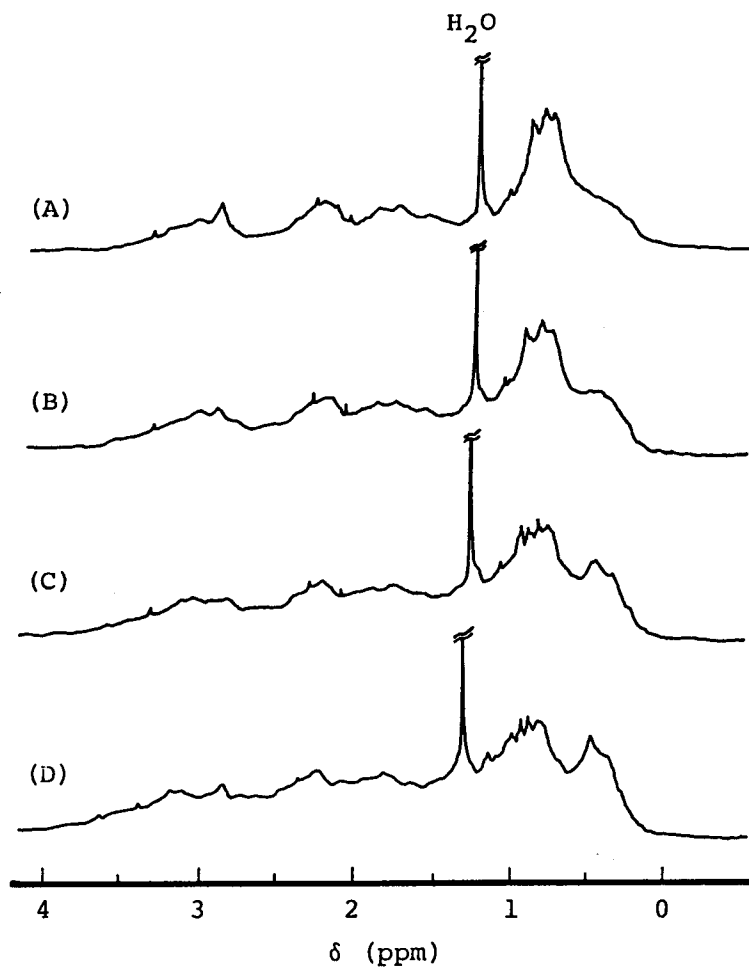
Figure B-3-4. 500 MHz ^1\text{H} NMR spectra of oligomer A taken at 60°C (A), 50°C (B), 40°C (C), and 30°C (D). ( \text{CDCl}_3 )
