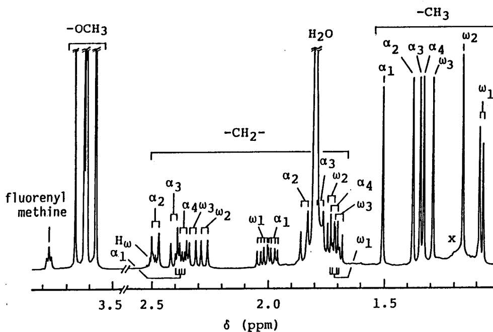
Figure A-1-9. 500 MHz ^1\text{H} NMR spectrum of MMA-heptamer mmmmmm (nitrobenzene- d_5 , 110°C).
