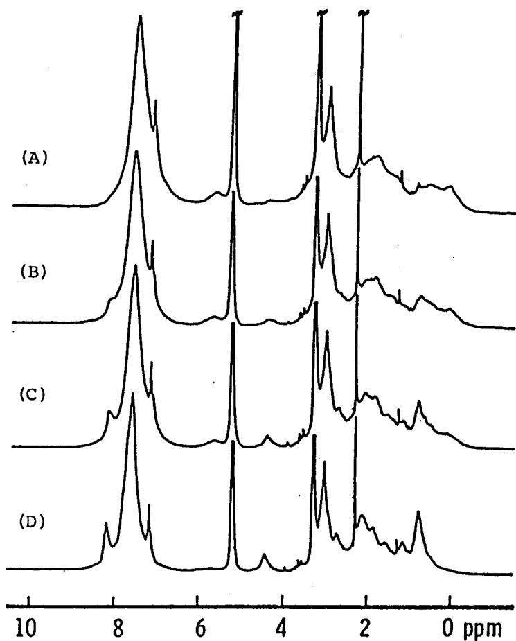
Figure B-2-6. Change of ^1\text{H} NMR spectra of poly(DMPMA) of DP=37 (Run 5 in Table B-2-1) in \text{CD}_3\text{OD}-8.3\%\text{CF}_3\text{CO}_2\text{D} at 25^\circ\text{C} : 7 min (A), 33 min (B), 65 min (C), and 200 min (D) after dissolution.
