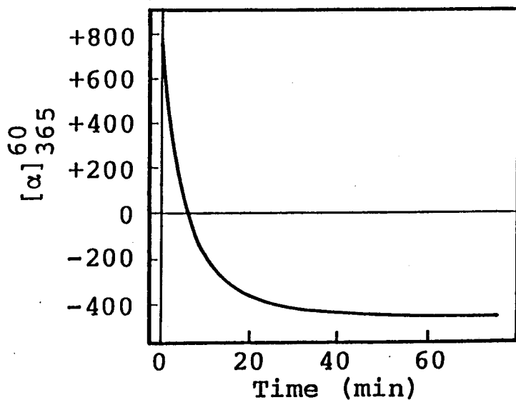
Figure B-1-5. Change of specific rotation of poly(CHDPMA) of DP=34 (Run 1 in Table B-1-3) in \text{CHCl}_3 at 60^\circ\text{C} .
