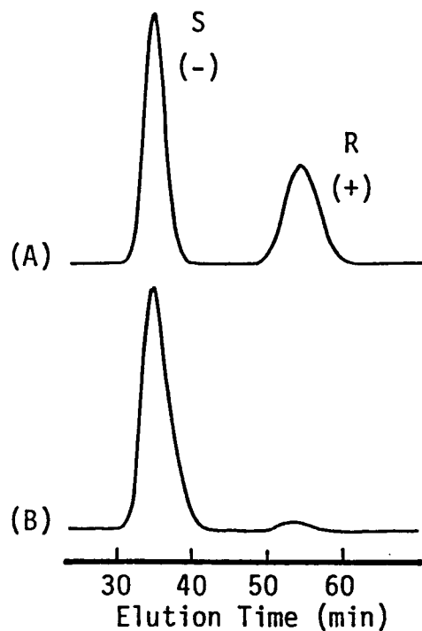
Figure A-2-3. Chromatograms of optical resolution of MMA-dimer derived from TrMA-dimer prepared with Sp-FlLi at [TrMA]/[Li]=2 (A) and 3 (B) and terminated with methyl iodide.
