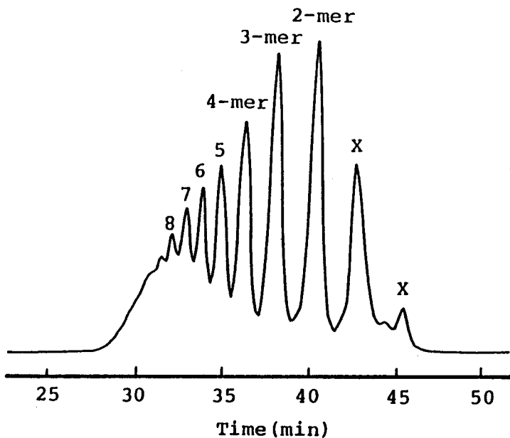
Figure B-4-1. GPC curve of hexane-soluble oligo(MMA) prepared with 1-NpMgBr at [1\text{-NpMgBr}]/[\text{MMA}] = 1/5 in toluene at -78^\circ\text{C} . x denotes unknown products.
