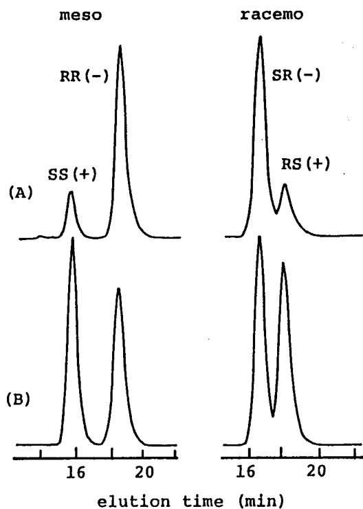
Figure A-1-11. Chromatograms of optical resolution of MMA-dimers prepared from (-)-(2R,4R)-2,4-dimethylglutaric acid (A) and (+)- and meso-dimethylglutaric acid (B) (right: meso, left: racemo).
