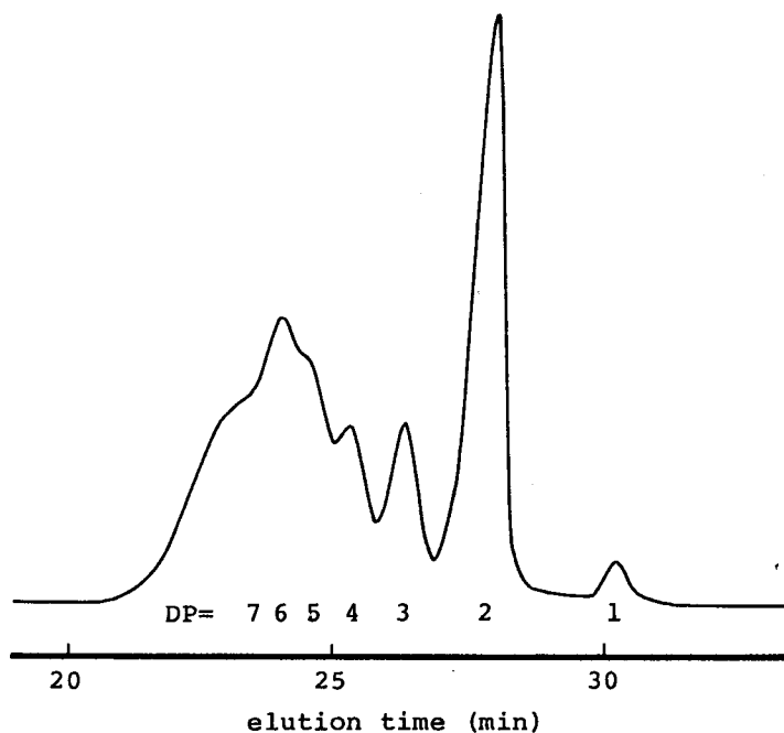
Figure B-3-1. GPC curve of oligo(D2PyMA) prepared with PMP-DPEDA-Li at [D2PyMA]/[Li]=3 in toluene at -78^{\circ}C .
