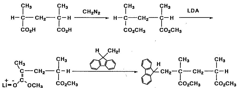
Scheme A-1-4. Synthesis of MMA-dimer from 2,4-dimethylglutaric acid.
