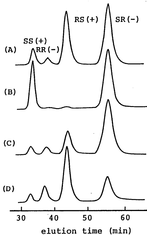
Figure A-1-10. Chromatograms of optical resolution of MMA-dimer derived from TrMA-dimer prepared with Sp-F1Li at [\text{TrMA}]/[\text{Li}] = 2 (A), 3 (B), 10 (C), and 20 (D).
