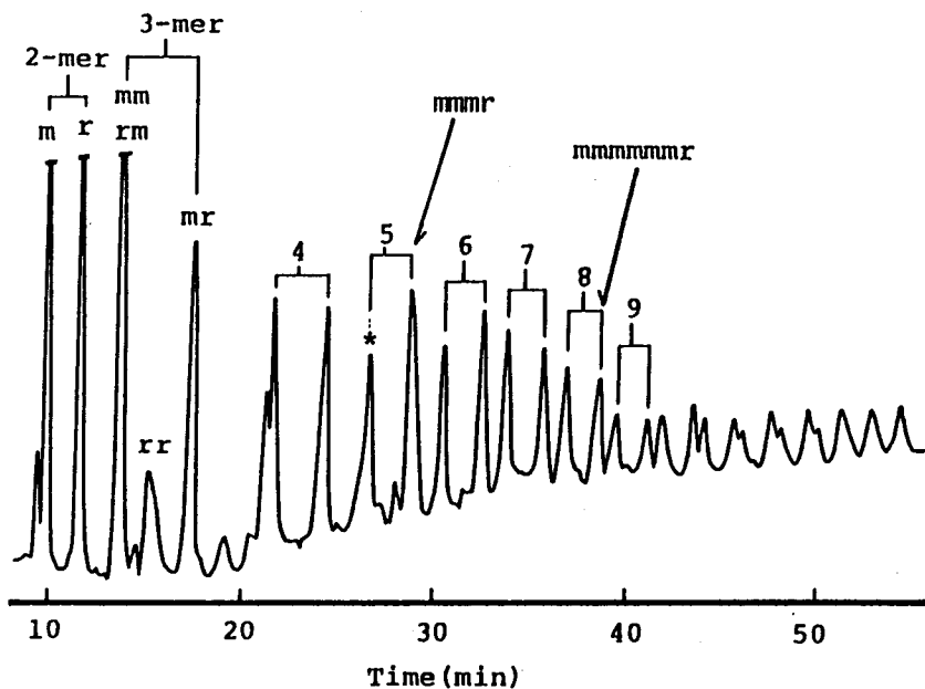
Figure B-4-3. Chromatogram of separation of diastereomers of oligo(MMA) prepared with 1-NpMgBr.
