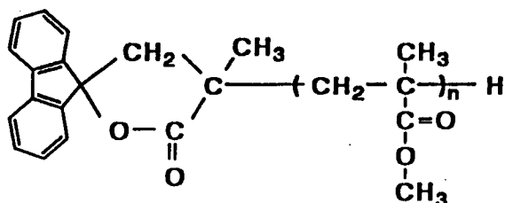
Scheme A-3-1. Structure of oligo(MMA) which corresponds to M/z = 350, 450, 550 \dots in FD mass spectrum.
