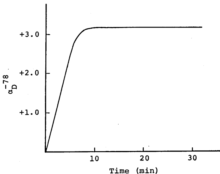
Figure A-1-2. Change of optical activity of polymerization system of TrMA with PMP-DEPDA-Li in toluene at -78^\circ\text{C} . (TrMA 0.15 g, toluene 3 ml, [\text{TrMA}]/[\text{Li}]=20 , cell length 1.0 cm)
