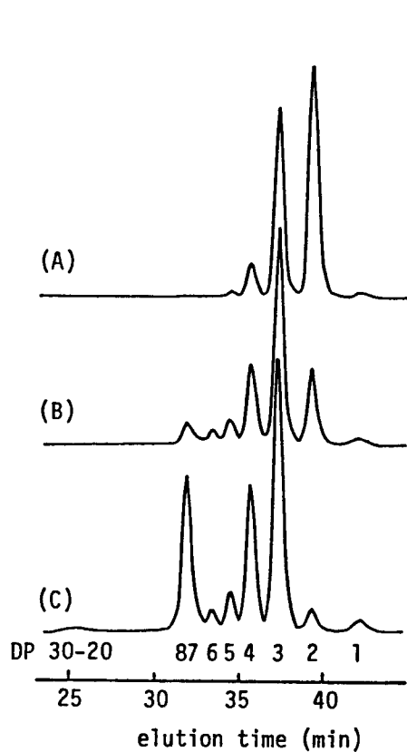
Figure A-3-1. GPC curves of oligo(MMA)s derived from oligo(TrMA)s prepared with Sp-MeFlLi at [TrMA]/[Li]=2 (A), 3 (B), and 5 (C).
