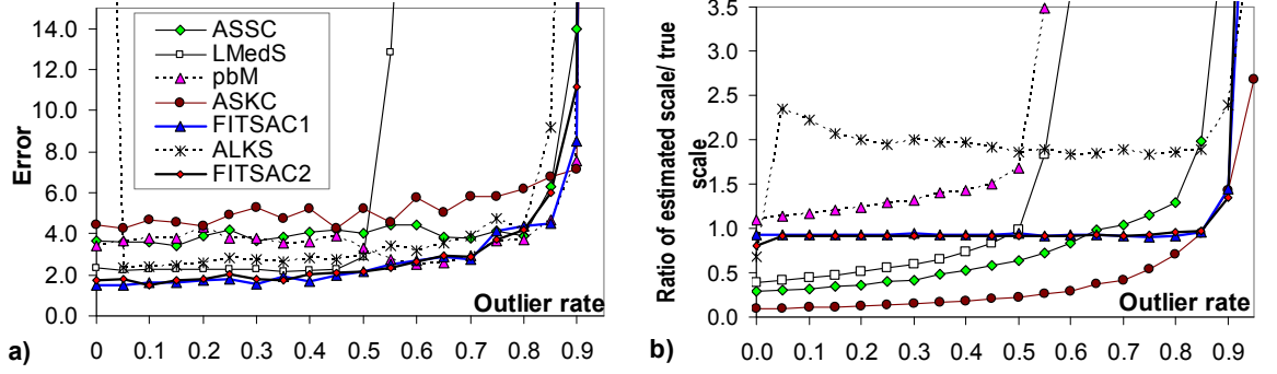
Figure 2.9: Experiments with varying outlier rates for single-line data: (a) estimation error, (b) ratio between the scale of the estimated inlier residuals and the scale of residuals of true inliers.
