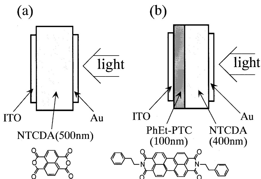
Fig. 6-1 The cell structures of (a) a single-layered device of NTCDA and (b) a double-layered device consisting of NTCDA and PhEt-PTC. The Au electrode was biased negatively with respect to the ITO electrode. Monochromatic light of 400 nm, which excites the NTCDA only, irradiated the Au electrode. Chemical structures of NTCDA and PhEt-PTC are also shown.
