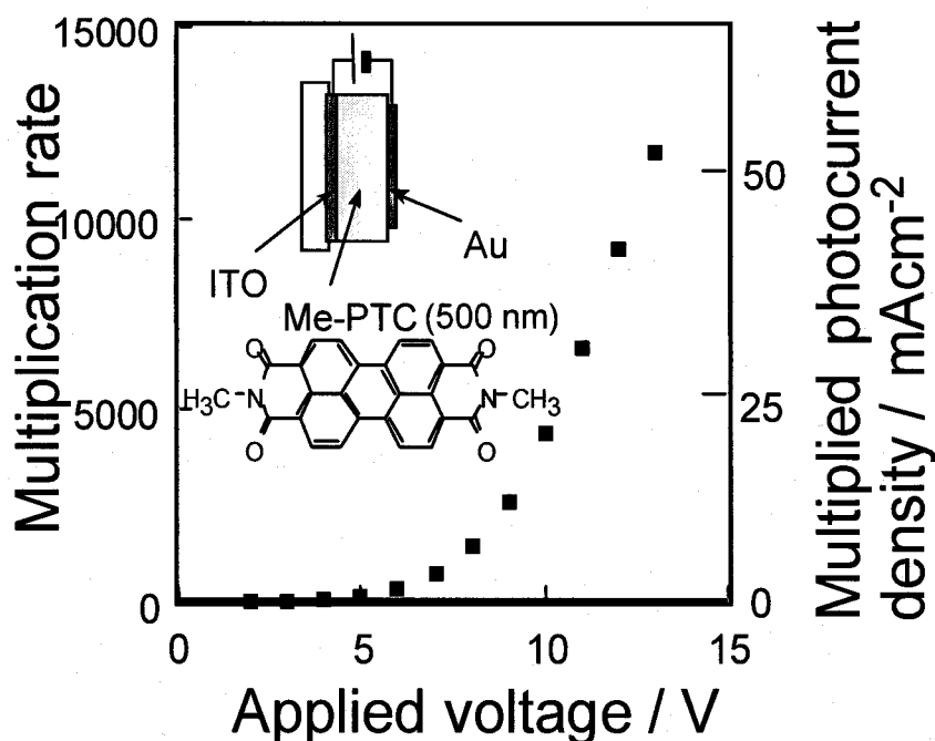
Fig.3-1 Dependence of multiplication rate and multiplied photocurrent density on applied voltage for the cell composed of ITO/Me-PTC(500nm)/Au. Monochromatic light of 600 nm ( 0.04 \text{ mW/cm}^2 ) was shone onto the Au electrode. Cell structure and chemical formula of Me-PTC are also shown.
