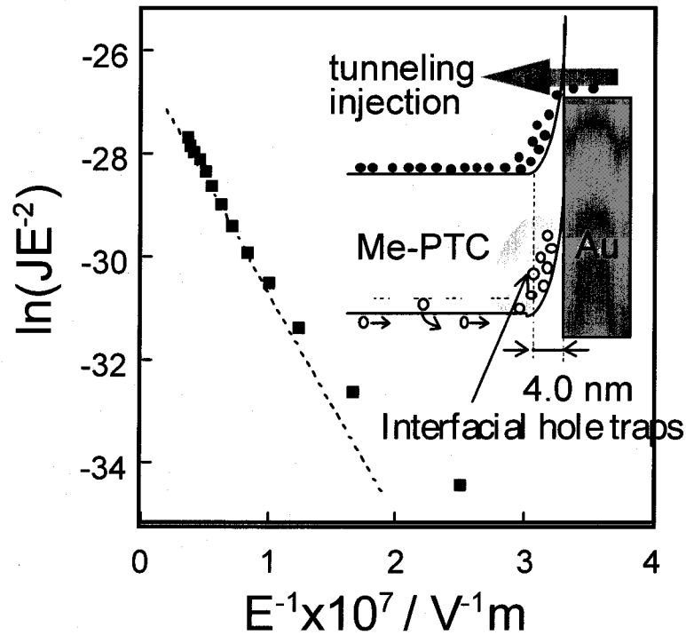
Fig.3-2 Fowler-Nordheim plot obtained from the multiplied photocurrent-voltage characteristics in Fig.3-1. Inset is the energy structure of the Me-PTC/Au interface during multiplication. The Au electrode is biased negatively. Filled and open circles indicate electrons and holes, respectively.
