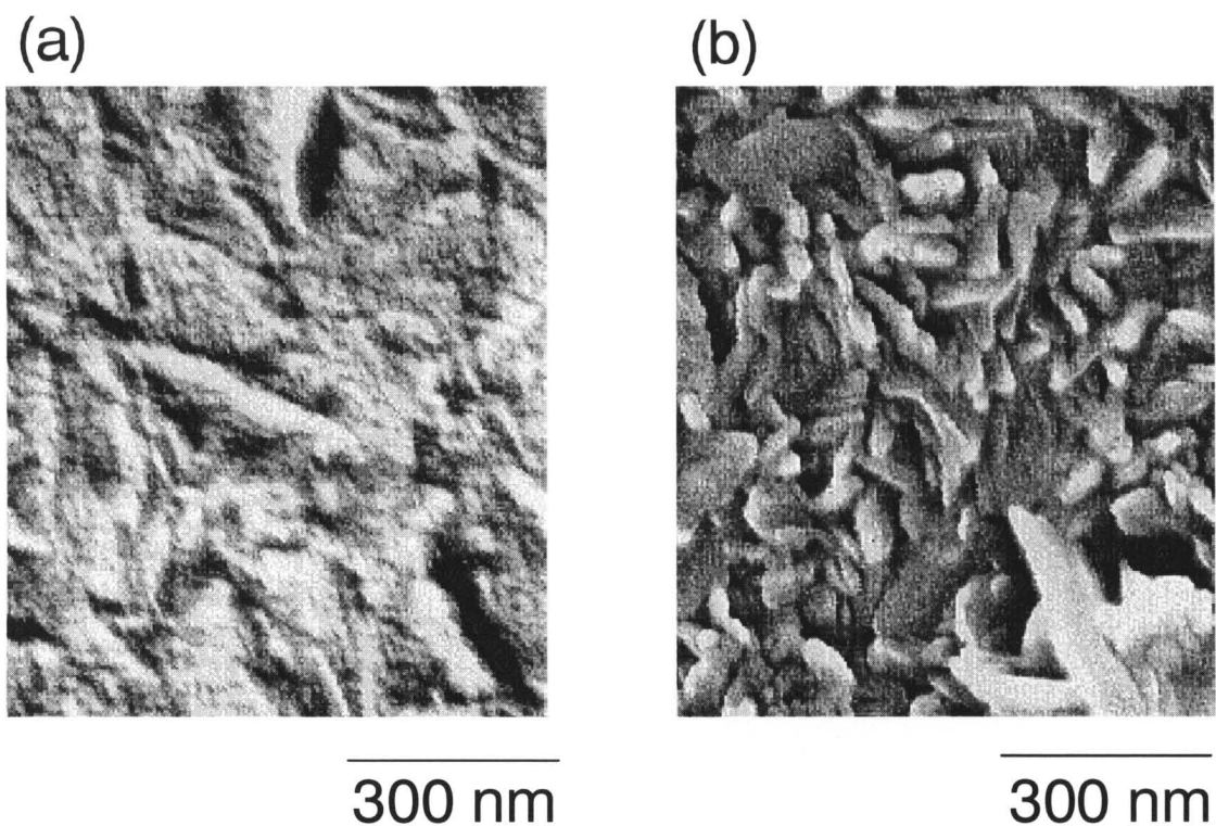
Fig. 4-14 SEM micrographs of Me-PTC films covered with Au films (thickness: 2 nm) deposited by the low-rate vacuum evaporation of 0.008 \text{ nms}^{-1} (a) and by the ion sputtering technique (b).
