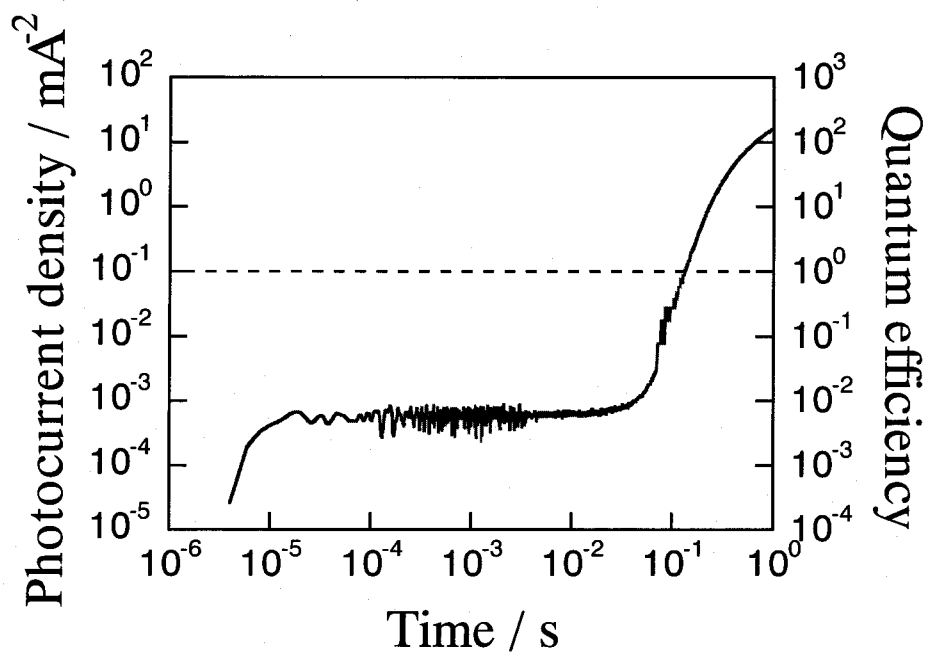
Fig.2-2 Typical transient response of photocurrent in multiplication device. The Au electrode was negatively biased 15 V with respect to the ITO electrode. The measurement was performed at 203 K.
