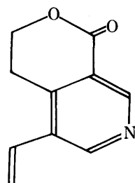
gentianine ( IV )
