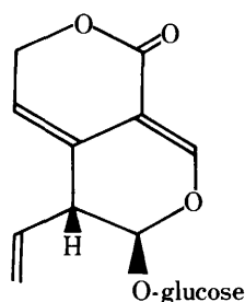
gentiopicroside ( I )
