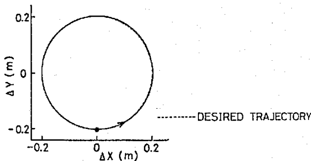
Fig.6-7 Simulation result in the cylindrical coordinates.
