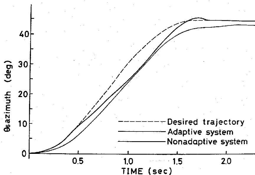
Fig.7-7 Response of the system with adaptive compensation of acceleration term ( \theta_e azimuth)
