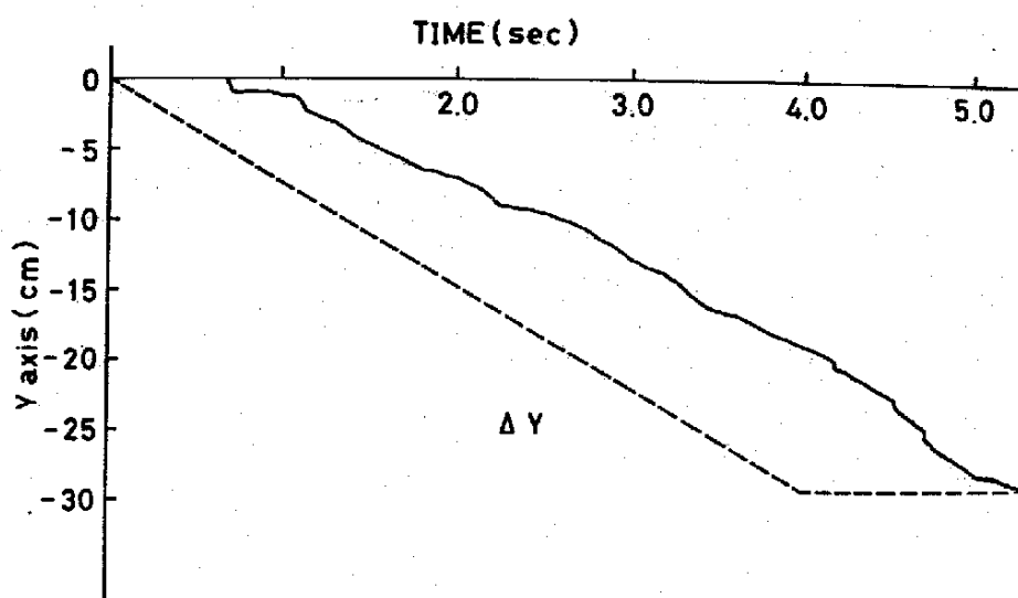
Fig.7-4 Response of Y-axis under the control of C_a.C.S. (ramp reference)
