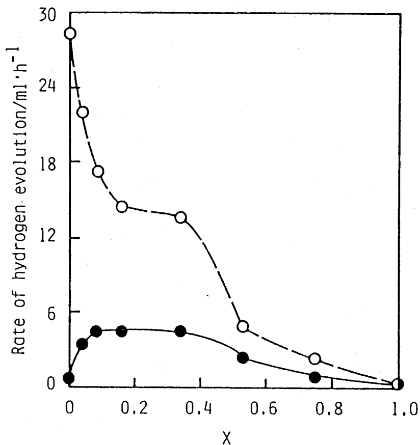
Fig. 4. The rate of the photocatalytic hydrogen evolution from an aqueous solution of 1 M sodium sulfite (pH 8.0) by use of \text{CdS}_{1-x}\text{Se}_x mixed-crystal powder as a function of X . Illumination was made through cut-off glass filters, Toshiba L-39 (○) and VO-52 (●), which showed 50 % transparency at 390 and 520 nm, respectively.
