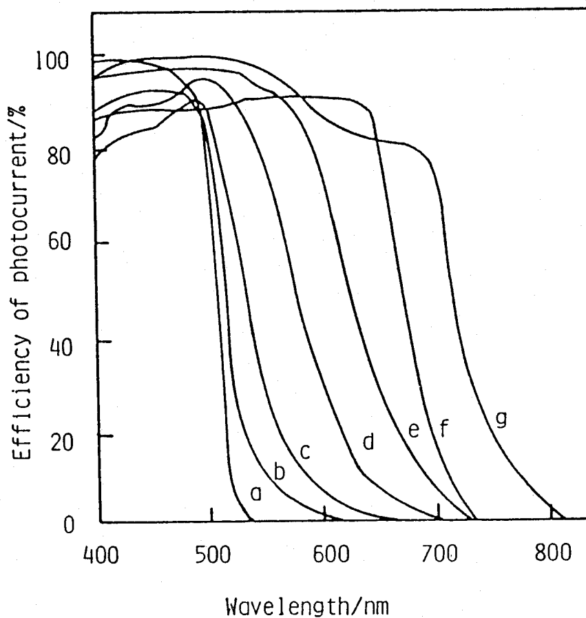
Fig. 6. The photocurrent quantum efficiency spectra for the CdS 1-x Se x sinter electrodes in an aqueous solution of 1 M sodium sulfite under anodic polarization (at +0.5 V vs SCE), for X values 0 (a), 0.08 (b), 0.16 (c), 0.34(d), 0.53 (e), 0.75 (f), and 1.0 (g).
