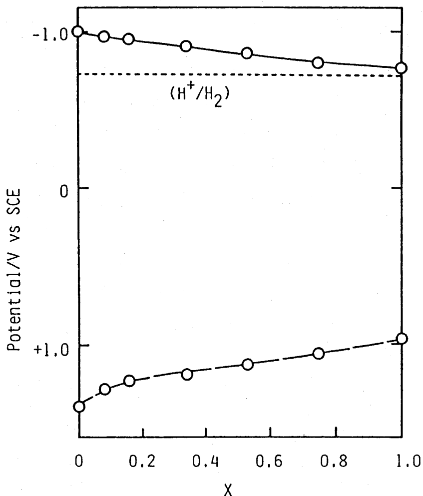
Fig. 7. The estimated energy levels of the conduction band of the CdS_{1-x}Se_x mixed-crystal ( solid line ) and those of the valence band ( broken line ) as a function of X in an aqueous solution of 1 M sodium sulfite. The dotted line represents the potential for the hydrogen evolution in the same solution.
