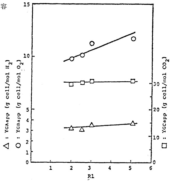
Fig. 9. Apparent yields to geseous substrates under various gas ratios
