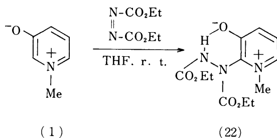
Scheme VIII
