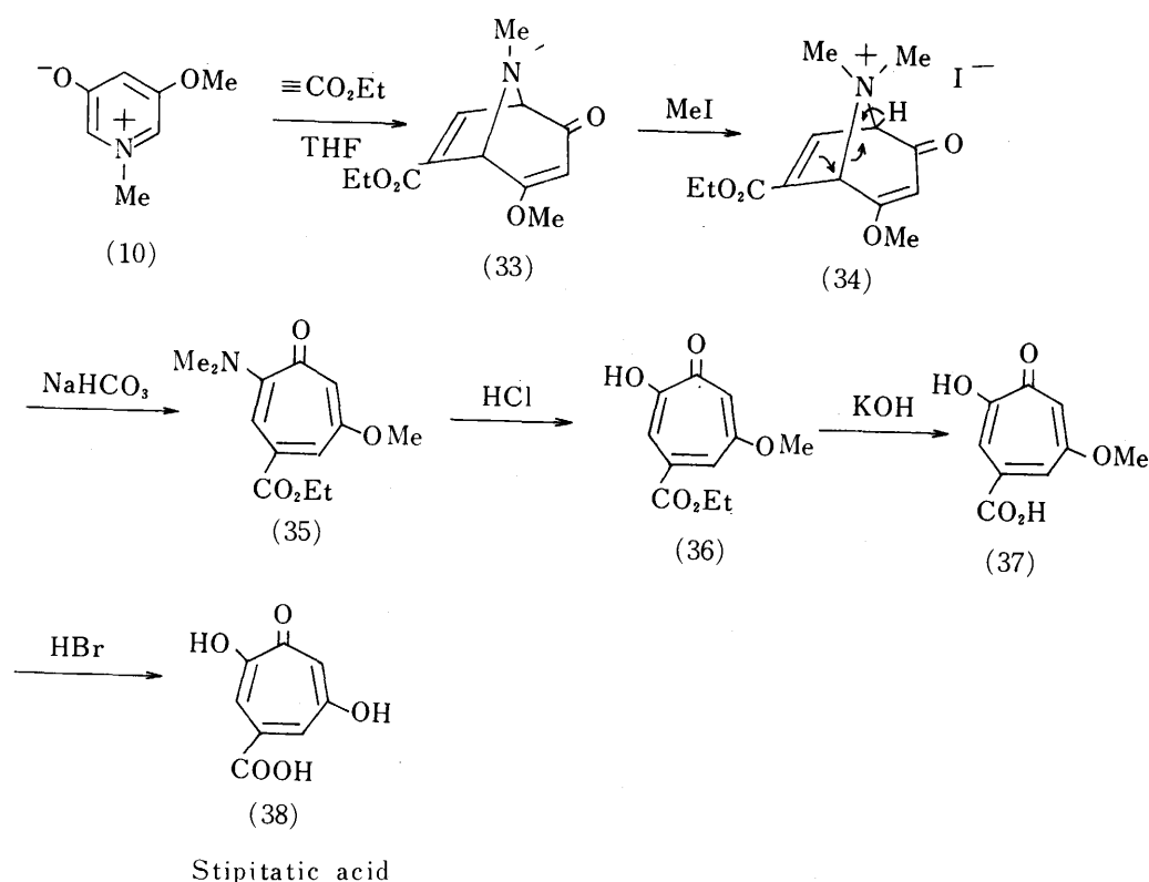
Scheme XII
