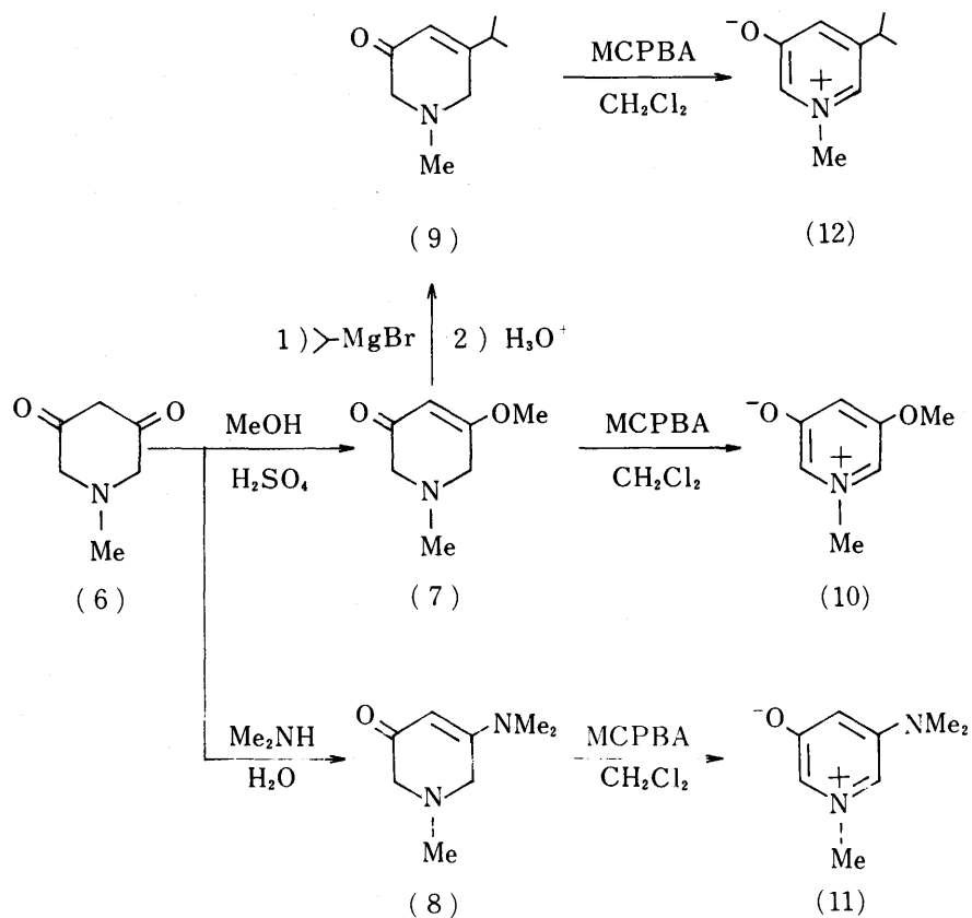
Scheme III
