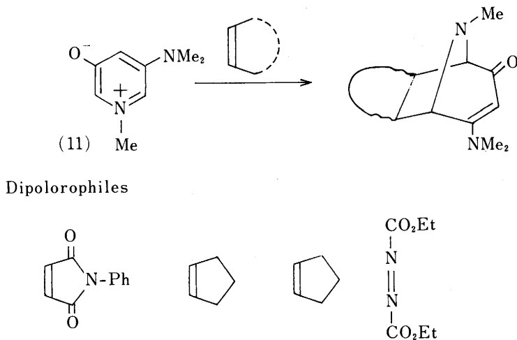
Scheme IX
