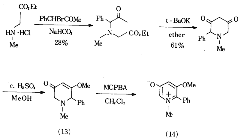
Scheme IV
