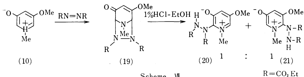
Scheme VII
