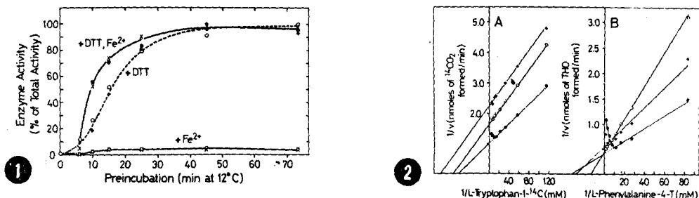
Fig. 1. Effect of preincubation on tryptophan and phenylalanine monooxygenase activities. The preincubation of the enzyme was carried out at 12^{\circ} in the presence of either \text{Fe}^{2+} , DTT or \text{Fe}^{2+} plus DTT as described previously (6). At various time intervals an aliquot (50 \mu\text{l} ) of the preincubated enzyme was removed and assayed for tryptophan ( \bullet and \circ ) and phenylalanine ( \times and + ) monooxygenase activities as described under "Methods".
