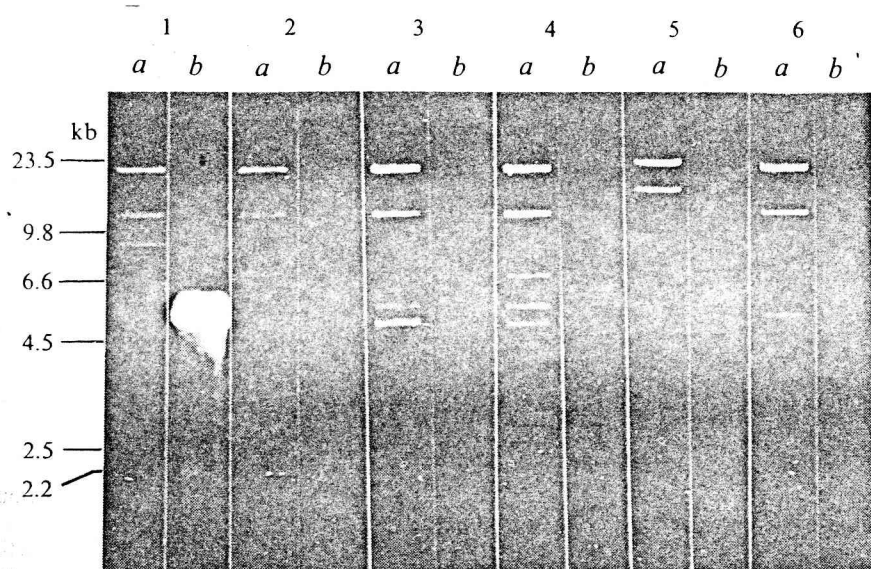
Fig. 6 Hybridization analysis with J-region probe. DNAs from isolated clones covering the region between the \gamma 1 and \gamma 2a genes were digested with Eco RI and run on 0.7% agarose gel electrophoresis. DNAs were transferred to a nitrocellulose filter 19 and hybridized with the 1.5-kilobase Hind III- Eco RI fragment that is located 6.5 kilobases 5' to the \mu gene. This fragment contains the J_{H4} region 24 . Ethidium bromide stains (a) and autoradiograms (b) of Southern blots are shown. DNA in each lane is as follows: (1) the expressed \gamma 1 gene of MC101 myeloma (Ig \gamma 1 -706) 25,47,48 that contains V, D, J 3 , J 4 , S 4 and C \gamma 1 gene segments; (2) clone 3; (3) clone 69; (4) clone 2; (5) the 6.6-kilobase \gamma 2b gene clone (IgH22) 28,30 ; (6) clone 9.
