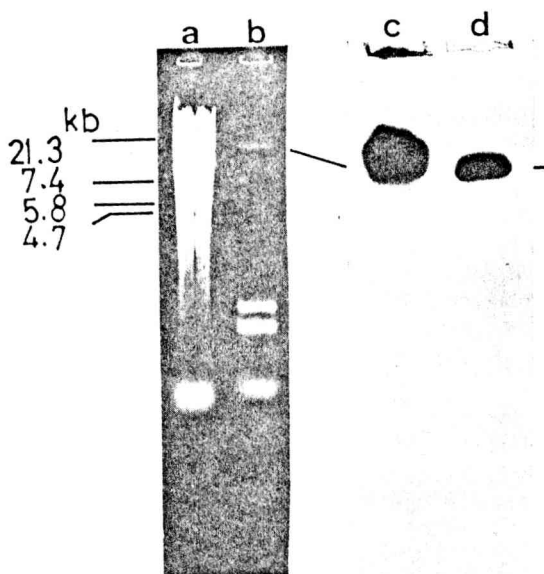
Fig. 4. Presence of 18S rRNA sequence in clone # (1-4). (a, b) shows the ethidium bromide-stained 1% agarose gel and (c, d) represents the autoradiography which was hybridized with ^{32}\text{P} -18S-cDNA. DNA of columns (a) and (c) was the fraction #30 of RPC-5 column chromatography containing the 14-17 kb rDNA fragment. DNA of column (b) and (d) was EcoRI-digested # (1-4) plasmid clone. EcoRI fragments of \lambda CI857 were used as size markers.
