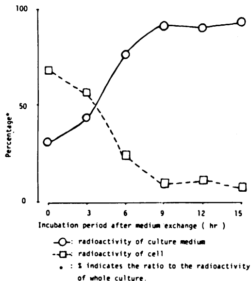
Fig.12. Release of ^{35}\text{S} -labeled Compound into Cultures Medium at Late Sporulation Stages of B. subtilis NRRL B 558
