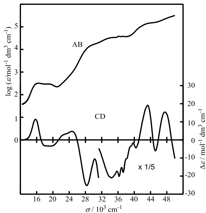
Figure III-9. Electronic absorption and CD spectra of [8']( \text{NO}_3 ) 3 in water.
