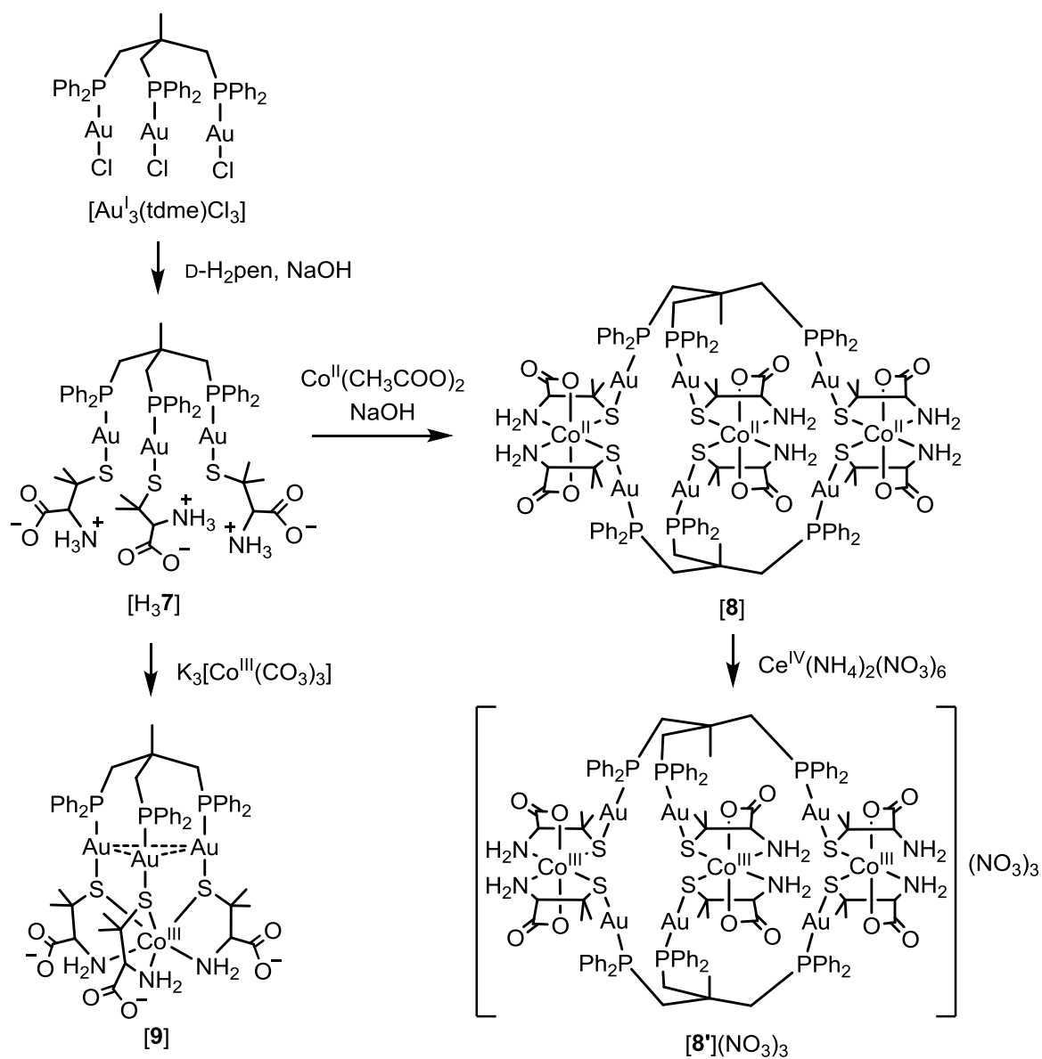
Scheme III-1. Synthesis of complexes [\text{H}_3\text{7}] , [\text{8}] , [\text{8'}](\text{NO}_3)_3 , and [\text{9}] .
