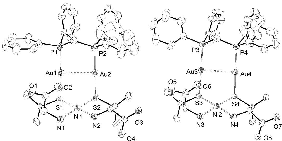
Figure II-13. ORTEP drawings of complex cations in [H 1.5 5a'](Et 4 N) 0.5 Cl 2 with 50% probability level of thermal ellipsoids. H atoms are omitted for clarity.
