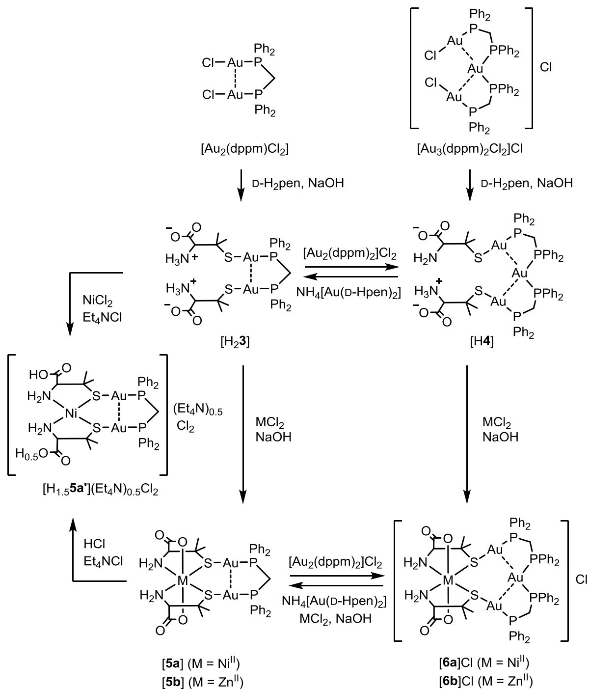
Scheme II-1. Syntheses and conversions of complexes [H 2 3], [H 4 ], [5a], [H 1.5 5a']( Et 4 N) 0.5 Cl 2 , [5b], [6a]Cl, and [6b]Cl.
