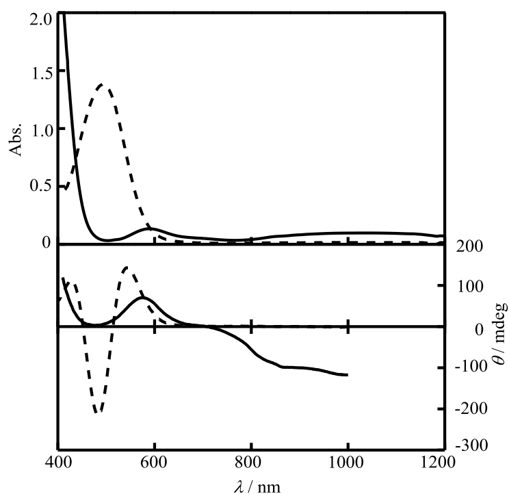
Figure II-12. Electronic absorption and CD spectra of ethanolic solution containing [5a] (solid line) and [H 2 5a'] 2+ generated from the reaction of [5a] with 2 molar equiv of triflic acid (dashed line).
