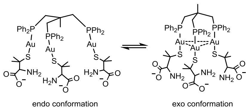
Chart III-1. Conformational conversion of [\text{7}]^{3-} .
