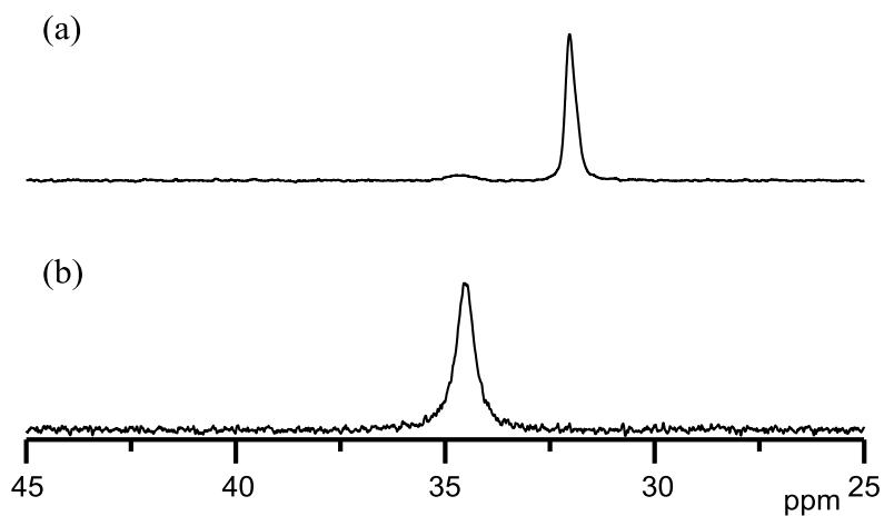
Figure II-2. ^{31}\text{P} NMR spectra of (a) [\text{H}_2\mathbf{3}] , (b) [\text{H}\mathbf{4}] in methanol- d_4 .
