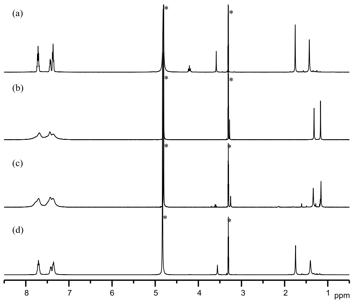
Figure II-1. ^1\text{H} NMR spectra of (a) [\text{H}_2\mathbf{3}] , (b) [\text{H}\mathbf{4}] , (c) reaction solution of [\text{H}_2\mathbf{3}] with [\text{Au}^{\text{I}}_2(\text{dppm})_2]\text{Cl}_2 , and (d) reaction solution of [\text{H}\mathbf{4}] with \text{NH}_4[\text{Au}^{\text{I}}(\text{D-Hpen})_2] in methanol- d_4 . (*) denotes the signals from solvents.
