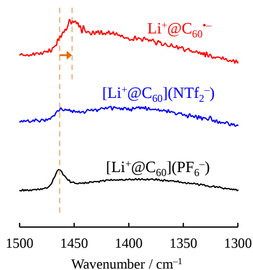
Figure 6. Raman spectra of the product, [\text{Li}^+\text{@C}_{60}](\text{NTf}_2^-) and [\text{Li}^+\text{@C}_{60}](\text{PF}_6^-) solids. Spectra were recorded using 532 nm excitation.
