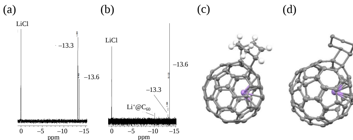
Figure 2. ^7\text{Li} NMR spectra of the crude products synthesized (a) under photo-irradiated condition and (b) under dark, and X-ray structure of [4+2] (c) and [2+2] (d) adducts obtained from co-crystal of the crude product synthesized under photo-irradiation condition.
