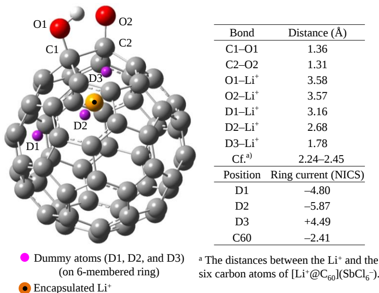
Figure 4. Theoretical calculation (B3LYP/6-31G* method) of the location of encapsulated lithium cation and of NICS (GIAO/B3LYP/6-31G*) on the center of 6-membered ring near the modified carbon atoms calculated for model \text{Li}^+@C_{60}(\text{O}^-)(\text{OH}) .
