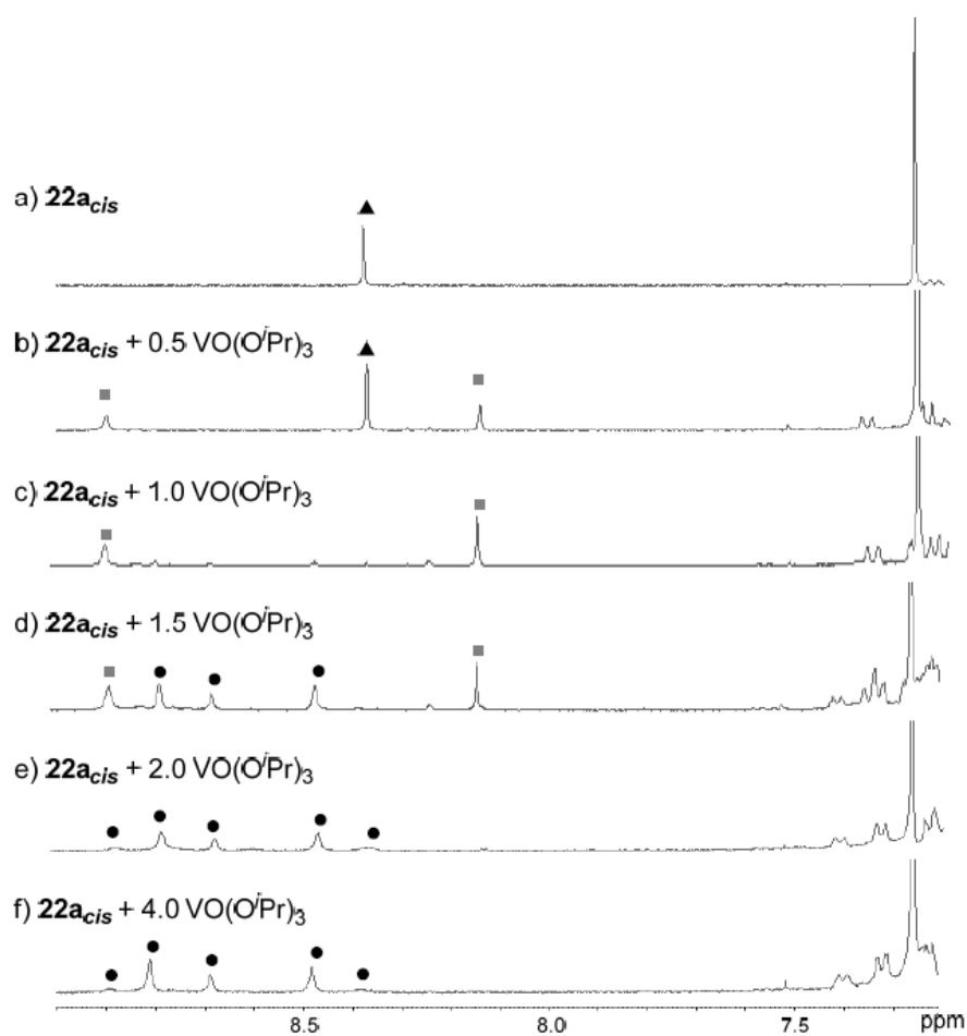
Figure 1. ^1\text{H} NMR spectra for the complexation of 22\text{a}_{cis} with \text{VO}(\text{O}^i\text{Pr})_3 . Each reaction was carried out in ethanol/dichloromethane at room temperature for 1 h under argon. Then, the solvent was replaced by \text{CDCl}_3/\text{CD}_3\text{OD} (20 : 1) for the ^1\text{H} NMR study.
