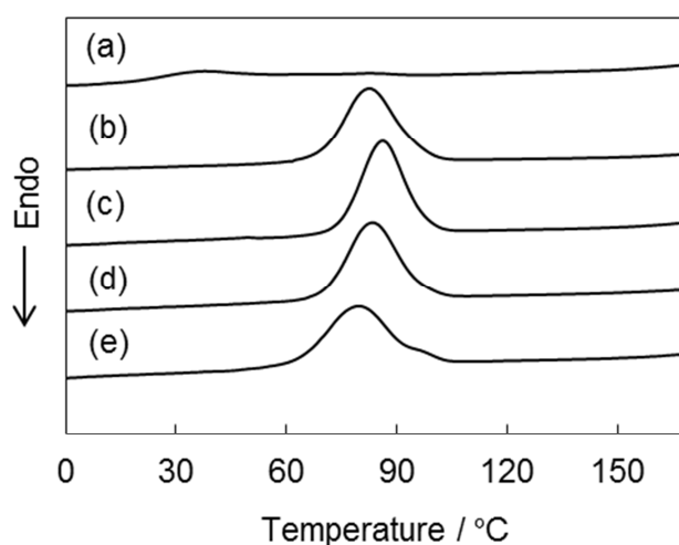
Figure 2-2. DSC curves of non-isothermal crystallization at a cooling rate of 10 °C/min; (a) neat PHBV, (b) PHBV/BP-L25, (c) PHBV/BP-L50, (d) PHBV/BP-L75, and (e) PHBV/BP-L100 blends. Additive amount of the branched poly(lactic acid) are 5 wt%.
