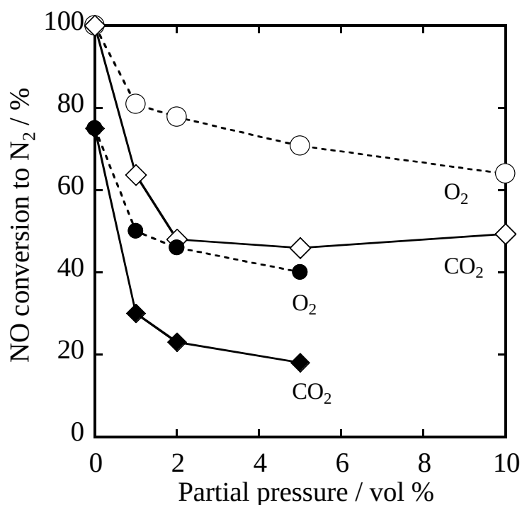
Figure 4.2 The effects of the presence of O 2 or CO 2 on catalytic activity of (Y 0.69 Tb 0.30 Ba 0.01 ) 2 O 2.99+δ (900 °C; open symbols) and Ba 0.8 La 0.2 Mn 0.8 Mg 0.2 O 3 (850 °C; closed symbols).
