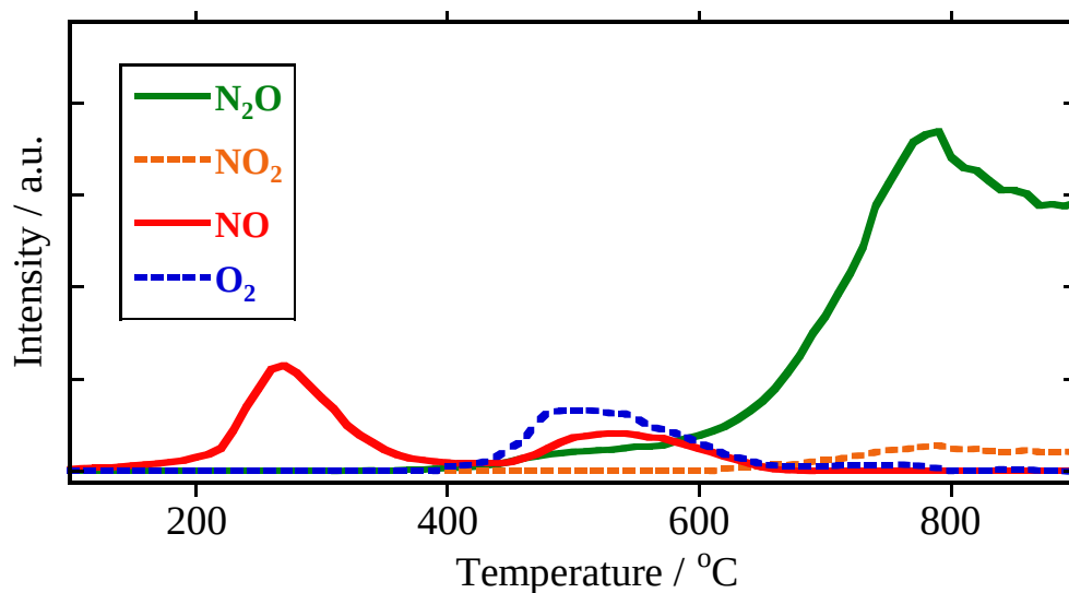
Figure 3.3 \text{N}_2\text{O} , \text{NO}_2 , \text{NO} , and \text{O}_2 desorption profiles ( \text{NO}_x -TPD) for (\text{Y}_{0.69}\text{Tb}_{0.30}\text{Ba}_{0.01})_2\text{O}_{2.99+\delta} exposed to 1 vol% \text{NO}/\text{He} for 30 min at 600 °C.
