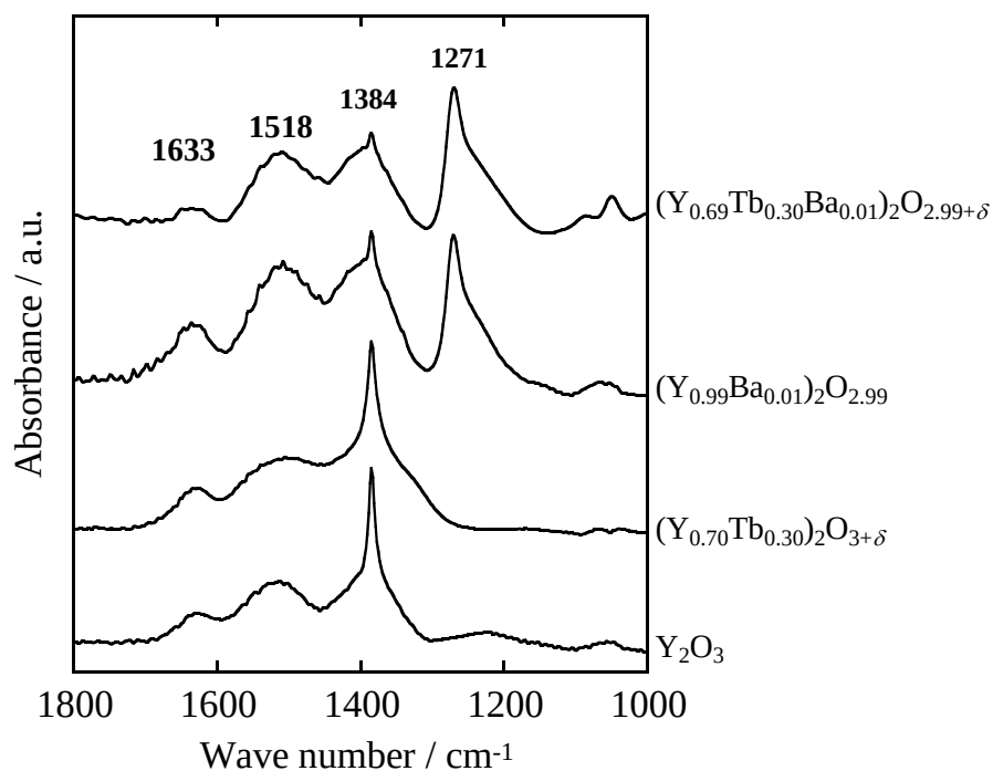
Figure 2.12 FT-IR spectra of (\text{Y}_{0.69}\text{Tb}_{0.30}\text{Ba}_{0.01})_2\text{O}_{2.99+\delta} , (\text{Y}_{0.99}\text{Ba}_{0.01})_2\text{O}_{2.99} , (\text{Y}_{0.70}\text{Tb}_{0.30})_2\text{O}_{3+\delta} , and \text{Y}_2\text{O}_3 exposed to 1 vol% NO/He for 30min at room temperature.
