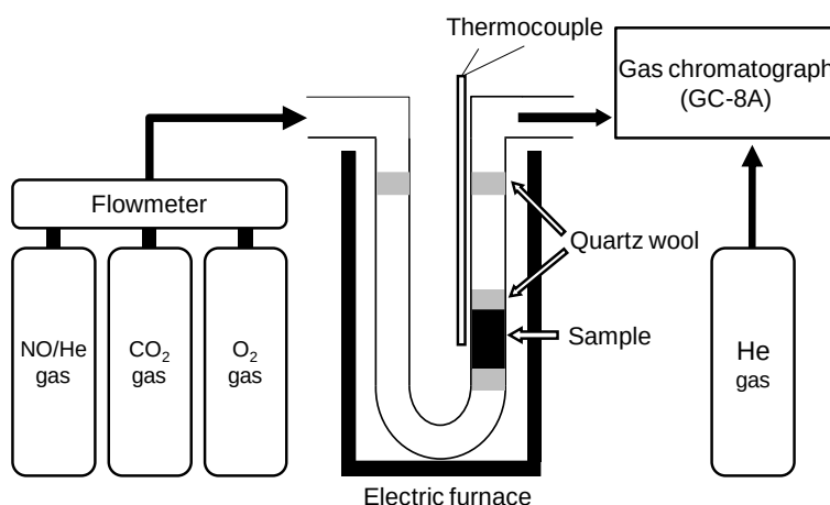
Figure 1.1 A schematic view of the catalyst performance testing apparatus for direct NO decomposition.
