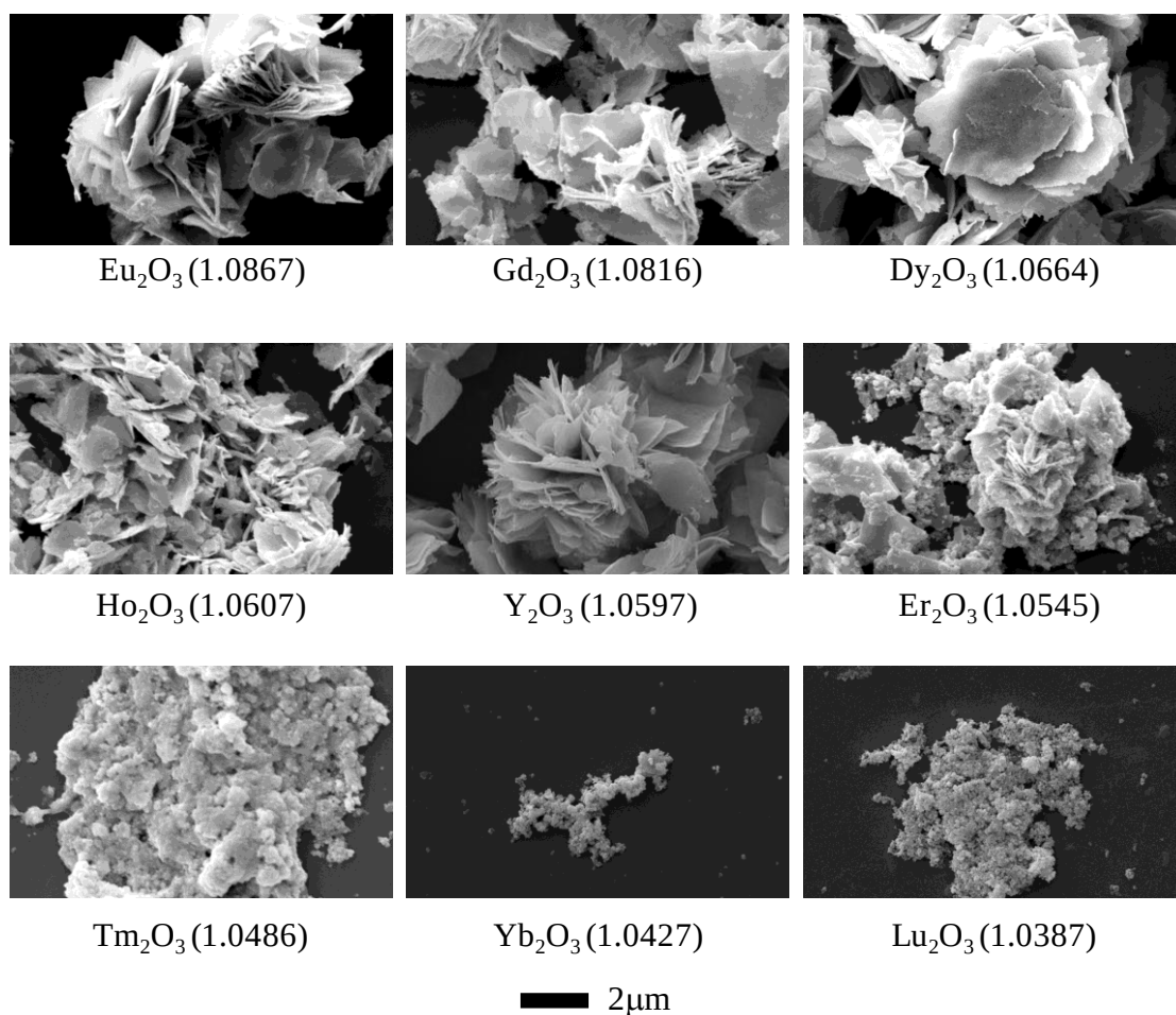
Figure 1.8 SEM images of C-type cubic REOs ( \text{Eu}_2\text{O}_3 , \text{Gd}_2\text{O}_3 , \text{Dy}_2\text{O}_3 , \text{Y}_2\text{O}_3 , \text{Ho}_2\text{O}_3 , \text{Er}_2\text{O}_3 , \text{Tm}_2\text{O}_3 , \text{Yb}_2\text{O}_3 , and \text{Lu}_2\text{O}_3 ).
