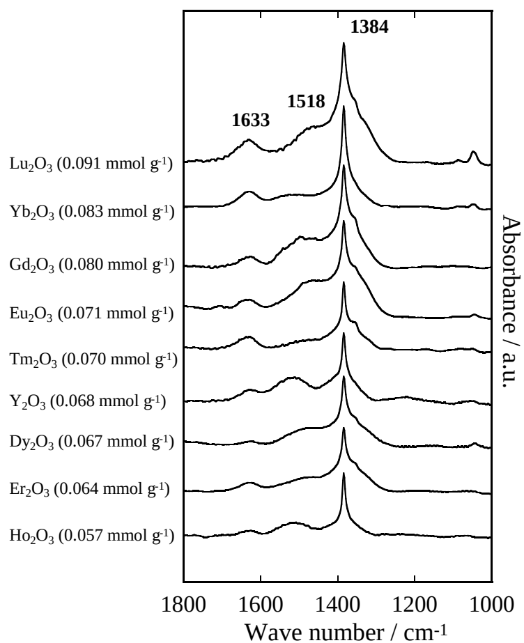
Figure 1.5 FT-IR spectra of C-type cubic REOs ( \text{Eu}_2\text{O}_3 , \text{Gd}_2\text{O}_3 , \text{Dy}_2\text{O}_3 , \text{Y}_2\text{O}_3 , \text{Ho}_2\text{O}_3 , \text{Er}_2\text{O}_3 , \text{Tm}_2\text{O}_3 , \text{Yb}_2\text{O}_3 , and \text{Lu}_2\text{O}_3 ) exposed to 1 vol% NO/He for 30 min at room temperature.
