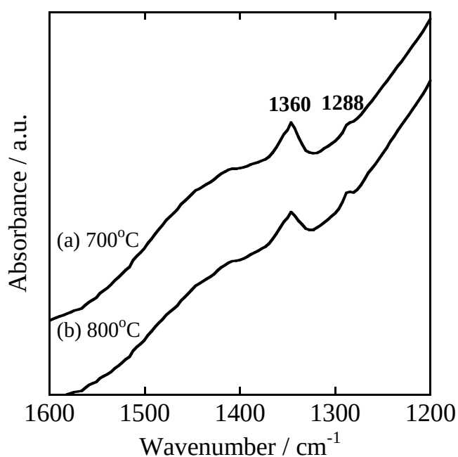
Figure 3.2 DRIFT-IR spectra of (Y_{0.69}Tb_{0.30}Ba_{0.01})_2O_{2.99+\delta} in a flow of 1 vol% NO/He at (a) 700 and (b) 800 °C.
