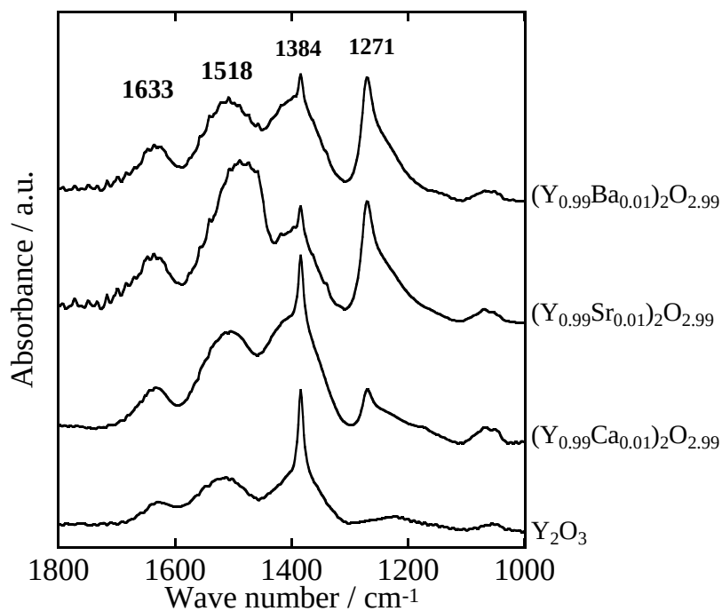
Figure 2.5 FT-IR spectra for (\text{Y}_{0.99}\text{A}_{0.01})_2\text{O}_{2.99} (A : Ba, Sr, and Ca) exposed to 1 vol% NO/He for 30 min at room temperature.
