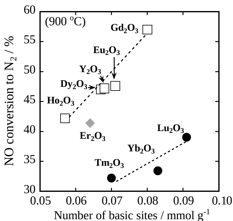
Figure 1.7 Dependence of N_2 yield for C-type cubic REOs on the number of basic sites. The oxides having a lattice parameter of 1.0597 nm or more (group 1) are shown in open squares ( \square ) and those of 1.0486 nm or less (group 2) are plotted in closed circles ( \bullet ). Er_2O_3 , which has an intermediate one of 1.0545 nm, is expressed in a gray diamond ( \blacklozenge ).
