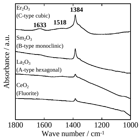
Figure 1.4 FT-IR spectra of \text{Er}_2\text{O}_3 , \text{Sm}_2\text{O}_3 , \text{La}_2\text{O}_3 , and \text{CeO}_2 exposed to 1 vol% NO/He for 30 min at room temperature.
