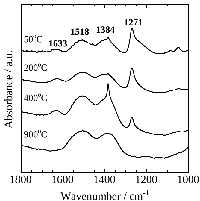
Figure 3.1 (a) FT-IR spectra for (Y_{0.69}Tb_{0.30}Ba_{0.01})_2O_{2.99+\delta} exposed to 1 vol% NO/He for 30 min at 600 °C and subsequently cooled to 50 °C in He. FT-IR spectra after heating the sample in He at (b) 200, (c) 400, and (d) 900 °C.
