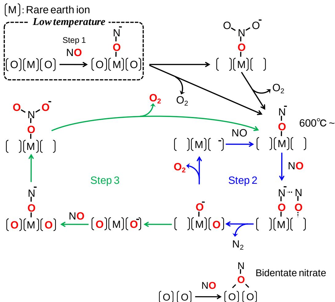
Scheme 1 Overall reaction mechanism for direct NO decomposition on a C-type cubic rare earth oxide-based catalyst.
