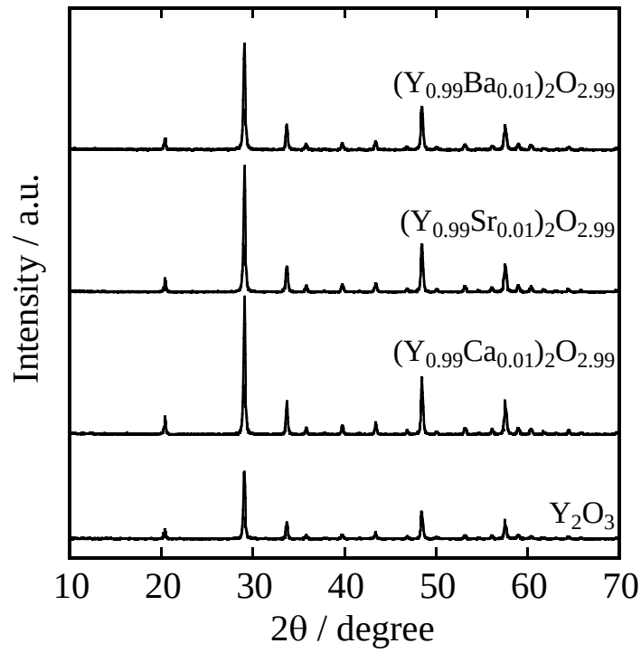
Figure 2.1 XRD patterns of (Y_{0.99}A_{0.01})_2O_{2.99} (A: Ba, Sr, and Ca) and Y_2O_3 .
