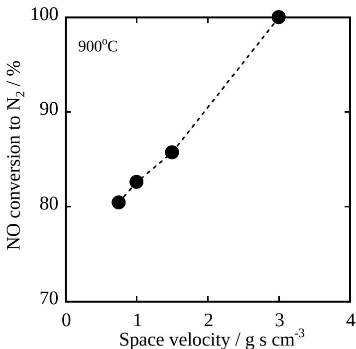
Figure 4.1 Space velocity dependence of NO conversion to N 2 over (Y 0.69 Tb 0.30 Ba 0.01 ) 2 O 2.99+δ at 900 °C (NO: 1vol%, He balance).
