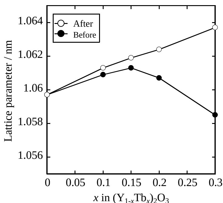
Figure 2.8 Dependence of the lattice parameter on the concentration of \text{Tb}^{3+/4+} in (\text{Y}_{1-x}\text{Tb}_x)_2\text{O}_{3+\delta} ( 0 \leq x \leq 0.30 ) before (●) and after (○) the catalytic test for NO decomposition.
