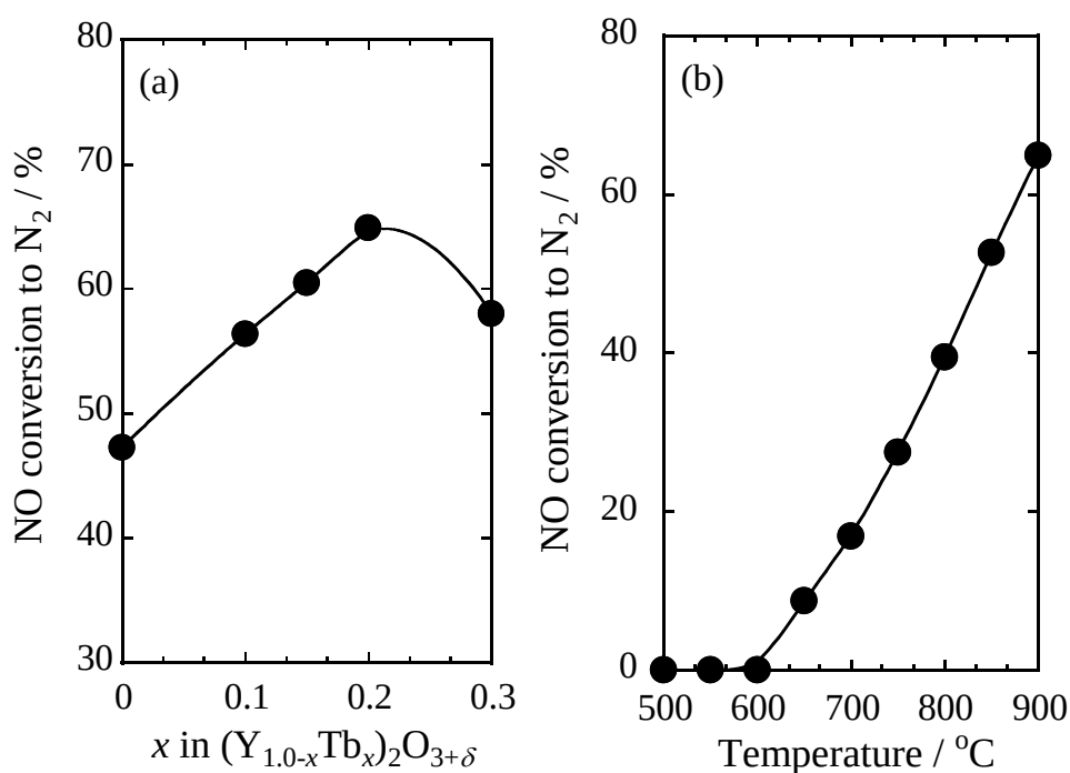
Figure 2.7 Variations in NO conversion to N_2 at 900 °C as a function of (a) the terbium concentration in (Y_{1-x}Tb_x)_2O_{3+\delta} ( 0 \leq x \leq 0.30 ) and (b) temperature (over the (Y_{0.80}Tb_{0.20})_2O_{3+\delta} catalyst).
