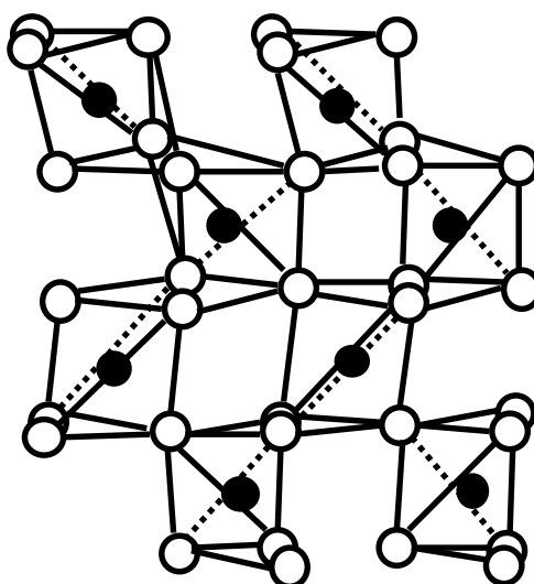
C-type cubic structure
