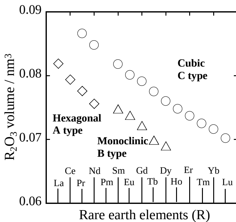
Figure G-3 Lattice volume of rare earth sesquioxides.
