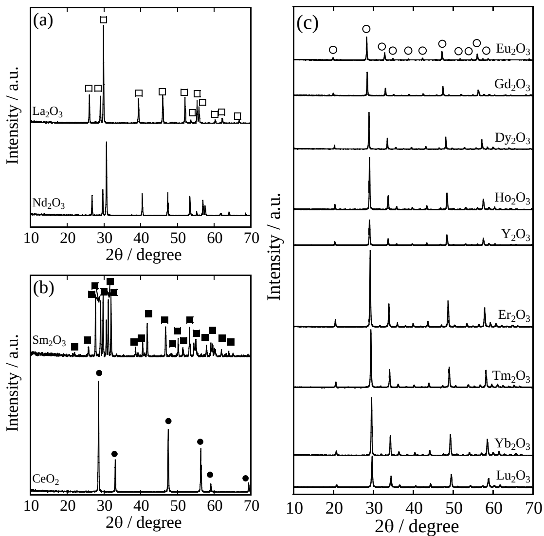
Figure 1.2 XRD patterns of (a) \text{La}_2\text{O}_3 and \text{Nd}_2\text{O}_3 , (b) \text{Sm}_2\text{O}_3 and \text{CeO}_2 , and (c) \text{Eu}_2\text{O}_3 , \text{Gd}_2\text{O}_3 , \text{Dy}_2\text{O}_3 , \text{Ho}_2\text{O}_3 , \text{Y}_2\text{O}_3 , \text{Er}_2\text{O}_3 , \text{Tm}_2\text{O}_3 , \text{Yb}_2\text{O}_3 , and \text{Lu}_2\text{O}_3 . The open squares and solid squares indicate the A-type hexagonal and the B-type monoclinic phases, respectively. The open and solid dots indicate C-type cubic and cubic fluorite-type phases, respectively.
