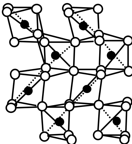
C-type cubic ( Ia3 )
