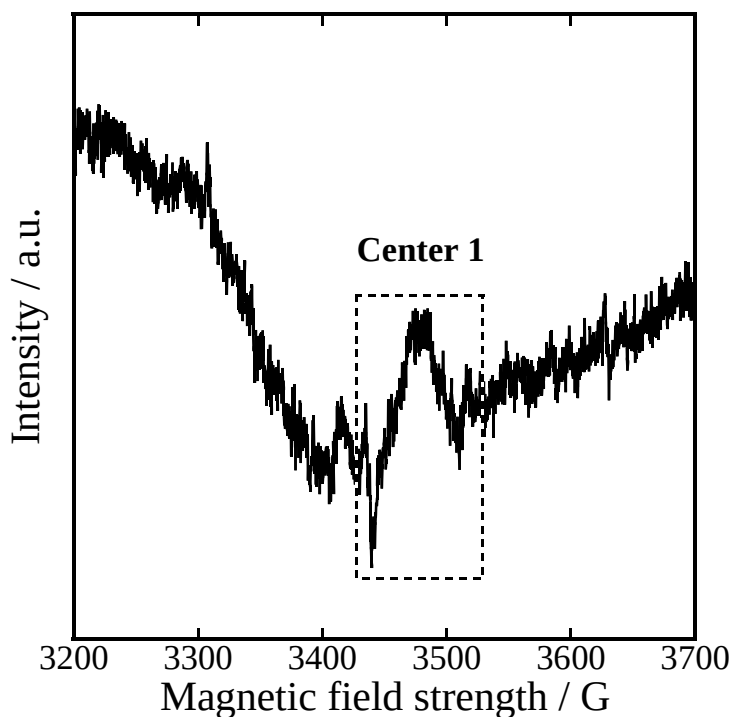
Figure 1.6 Room temperature ESR spectrum of Y 2 O 3 after NO adsorption.
