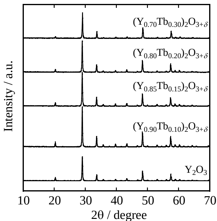
Figure 2.6 XRD patterns of (Y_{1-x}Tb_x)_2O_{3+\delta} ( 0 \leq x \leq 0.30 ).
