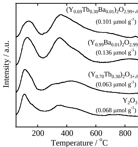
Figure 2.10 \text{CO}_2 -TPD profiles for (\text{Y}_{0.69}\text{Tb}_{0.30}\text{Ba}_{0.01})_2\text{O}_{2.99+\delta} , (\text{Y}_{0.99}\text{Ba}_{0.01})_2\text{O}_{2.99} , (\text{Y}_{0.70}\text{Tb}_{0.30})_2\text{O}_{3+\delta} , and \text{Y}_2\text{O}_3 .
