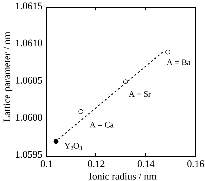
Figure 2.2 Dependence of the lattice parameters of (Y_{0.99}A_{0.01})_2O_{2.99} (A: Ba, Sr, and Ca) (○) on the ionic radius of the dopant. The lattice parameter of Y_2O_3 was also plotted as a reference (●).
