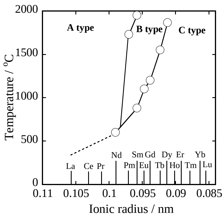
Figure G-4 Polymorphic transformation for the rare earth sesquioxides.
