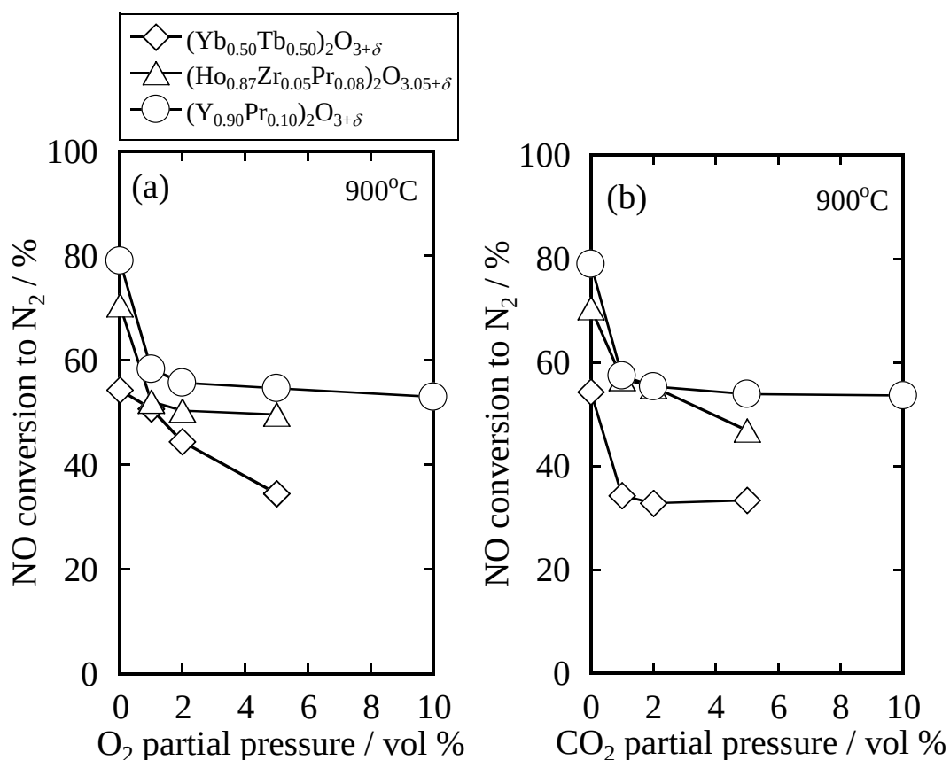
Figure 4.3 Effects of \text{O}_2 (a) and \text{CO}_2 (b) on the \text{N}_2 yield obtained over (\text{Yb}_{0.50}\text{Tb}_{0.50})_2\text{O}_{3+\delta} , (\text{Ho}_{0.87}\text{Zr}_{0.05}\text{Pr}_{0.08})_2\text{O}_{3.05+\delta} , and (\text{Y}_{0.90}\text{Pr}_{0.10})_2\text{O}_{3+\delta} .
