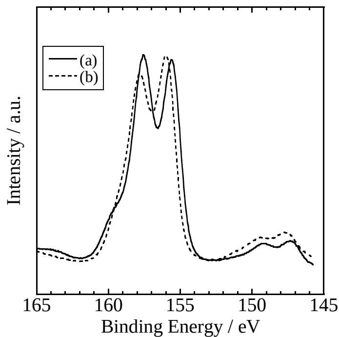
Figure 2.13 XPS spectra for (\text{Y}_{0.69}\text{Tb}_{0.30}\text{Ba}_{0.01})_2\text{O}_{2.99+\delta} before (a) and after (b) the catalytic test for NO decomposition.
