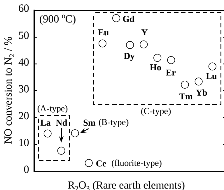
Figure 1.3 Dependence of the rare earth elements on the NO conversion to N 2 on the REOs.
