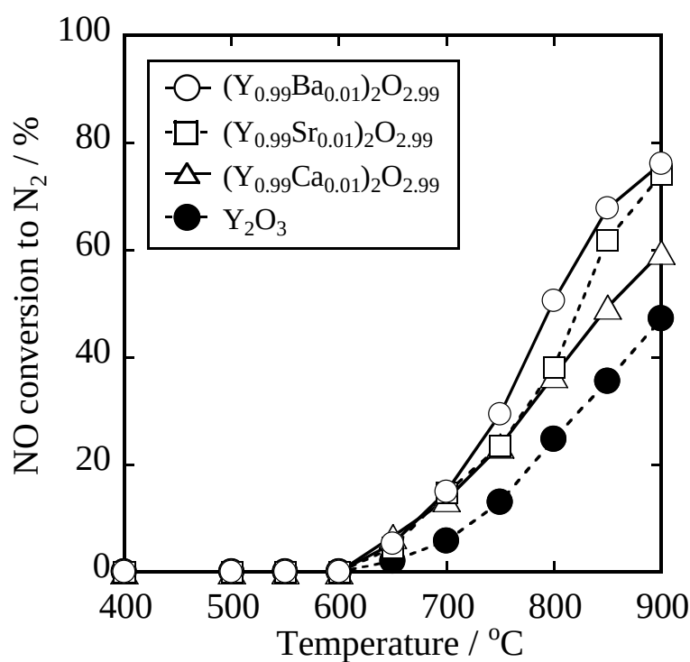
Figure 2.3 Temperature dependence of NO conversion to N 2 over (Y 0.99 A 0.01 ) 2 O 2.99 (A: Ba, Sr, and Ca) and Y 2 O 3 (NO: 1 vol%; He balance; W/F = 3.0 g s cm -3 ).
