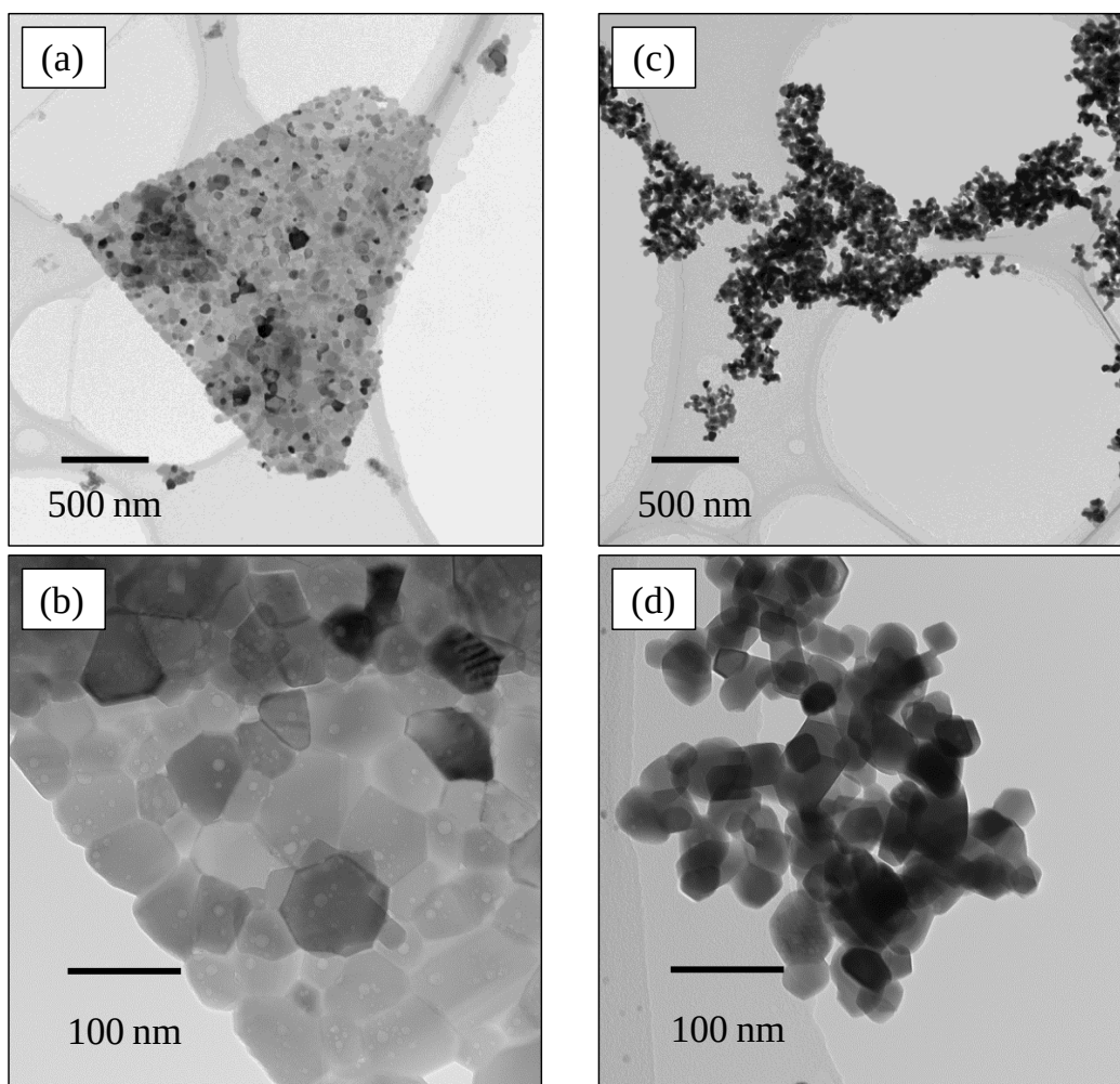
Figure 1.9 TEM images of \text{Y}_2\text{O}_3 (Direct Mag: (a) 8000 \times , (b) 50,000 \times ) and \text{Lu}_2\text{O}_3 (Direct Mag: (c) 8000 \times , (d) 50,000 \times ).
