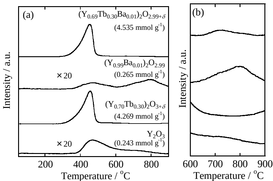
Figure 2.11 \text{O}_2 -TPD profiles for (\text{Y}_{0.69}\text{Tb}_{0.30}\text{Ba}_{0.01})_2\text{O}_{2.99+\delta} , (\text{Y}_{0.99}\text{Ba}_{0.01})_2\text{O}_{2.99} , (\text{Y}_{0.70}\text{Tb}_{0.30})_2\text{O}_{3+\delta} , and \text{Y}_2\text{O}_3 in the temperature range from 50 to 900 °C (a) and 600 to 900 °C (b).
