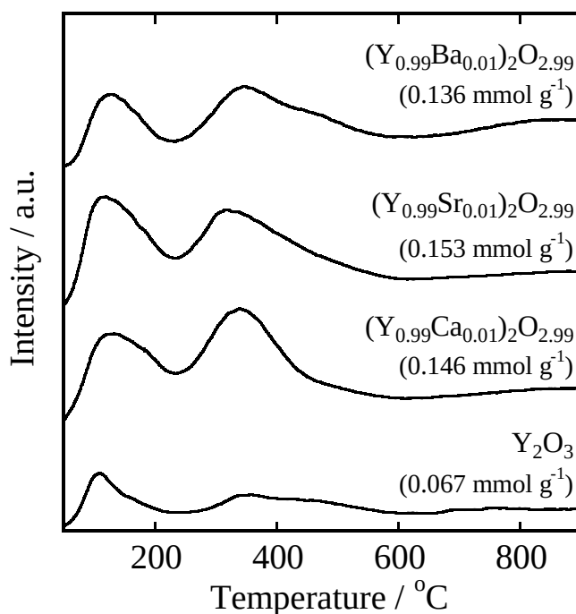
Figure 2.4 CO 2 -TPD profiles for (Y 0.99 A 0.01 ) 2 O 2.99 (A : Ba, Sr, and Ca).
