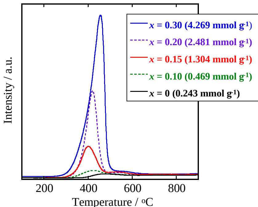
Figure 2.9 O 2 -TPD profiles for (Y 1-x Tb x ) 2 O 3+δ (0 ≤ x ≤ 0.30).
