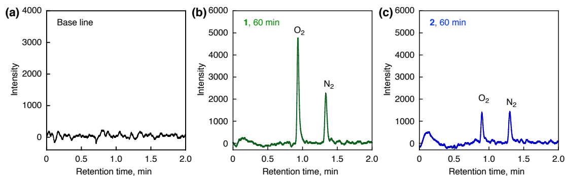
Figure S1. GC charts of (a) a base line and the gas evolved at 60 min in the catalytic water oxidation with (b) 1 (12.5 μM) and (c) 2 (12.5 μM) by CAN (125 mM) in a non-buffered aqueous solution (2.0 mL).
