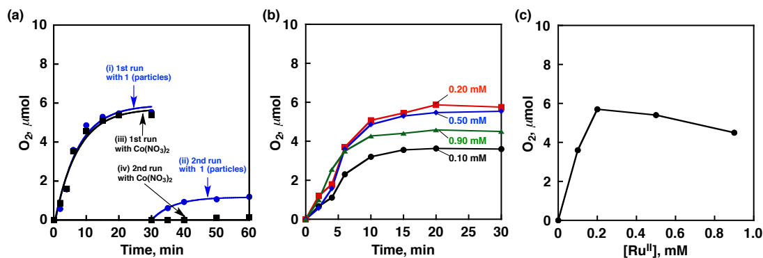
Figure 6. (a) Time courses of O 2 evolution under photoirradiation (Xe lamp, \lambda > 420 nm) of a buffer solution (pH 8.0, 2.0 mL) containing [Ru(bpy) 3 ] 2+ (0.50 mM) and Na 2 S 2 O 8 (10 mM) with a precatalyst (i and ii) 1 (50 \mu M) and (iii and iv) Co(NO 3 ) 2 (50 \mu M). 2 nd runs were performed by adding Na 2 S 2 O 8 (5.0 \mu mol) to the solutions after 1 st run and adjusted pH to 8.0 by NaOH (1M, 40 \mu L). (b) Time courses of O 2 evolution under photoirradiation (Xe lamp, \lambda > 420 nm) of a buffer solution (pH 8.0, 2.0 mL) containing precatalyst 1 (50 \mu M), Na 2 S 2 O 8 (10 mM) and [Ru(bpy) 3 ](ClO 4 ) 2 [0.10 mM (black cycle), 0.20 mM (red square), 0.50 mM (blue diamond), 0.90 mM (green triangle)]. (c) Dependence of O 2 evolution on concentrations of [Ru(bpy) 3 ](ClO 4 ) 2 after 20 min photoirradiation (Xe lamp, \lambda > 420 nm) of the solution (pH 8.0).
