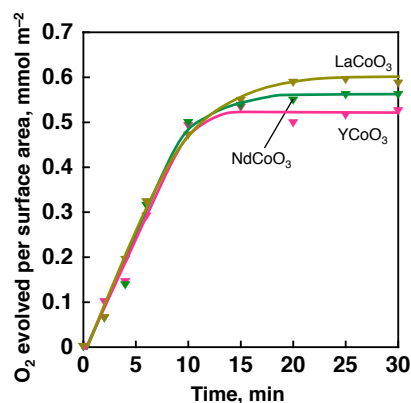
Figure 10. Time courses of oxygen evolution normalized by a catalyst surface area in the photocatalytic water oxidation with \text{Na}_2\text{S}_2\text{O}_8 ( 5.0 \text{ mM} ) and [\text{Ru}(\text{bpy})_3](\text{ClO}_4)_2 ( 0.25 \text{ mM} ) using perovskites ( 0.25 \text{ g L}^{-1} , \text{LaCoO}_3 , brown; \text{NdCoO}_3 , green and \text{YCoO}_3 , pink) under photoirradiation ( \lambda > 420 \text{ nm} ) of a phosphate buffer solution ( 2.0 \text{ mL} ) at \text{pH } 7.0 .
