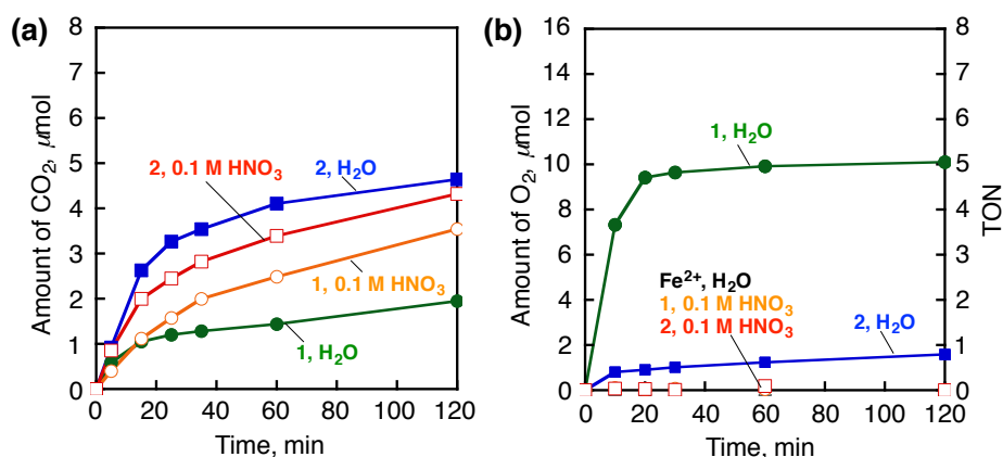
Figure 4. Time courses of (a) \text{CO}_2 evolution and (b) \text{O}_2 evolution in the catalytic water oxidation by CAN (0.10 M) with 1 , 2 and \text{FeSO}_4 (1.0 mM) in a non-buffered aqueous solution and in an aqueous solution containing 0.10 M \text{HNO}_3 (2.0 mL). The product yields were determined using GC.
