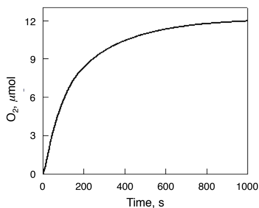
Figure 5. Time courses of \text{O}_2 evolution monitored by manometry in the catalytic water oxidation by CAN (0.10 M) with 1 (1.0 mM) in a non-buffered aqueous solution (2.0 mL).
