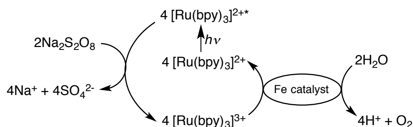
Scheme 2. Catalytic Cycle of Light-Driven Water Oxidation with \text{Na}_2\text{S}_2\text{O}_8 and [\text{Ru}(\text{bpy})_3]^{2+} Using an Iron-Based Catalyst
