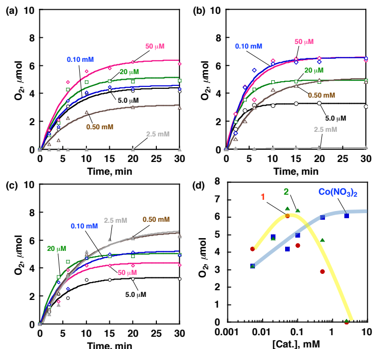
Figure 7. Time courses of O 2 evolution under irradiation with visible light (Xe lamp, \lambda > 420 nm) at different concentrations of precatalyst (a) 1 , (b) 2 and (c) Co(NO 3 ) 2 [5.0 μM (black circle), 20 μM (green square), 50 μM (pink diamond) and 0.10 mM (blue diamond), 0.50 mM (blown triangle) and 2.5 mM (grey triangle)] in the solution containing [Ru(bpy) 3 ] 2+ (0.50 mM) and Na 2 S 2 O 8 (10 mM) in 2.0 mL of borate buffer (100 mM, pH 9.0). (d) Dependence of O 2 evolution on concentrations of precatalysts, 1 (red circles), 2 (green triangles) and Co(NO 3 ) 2 (blue square) after 20 min photoirradiation (Xe lamp, \lambda > 420 nm) of the solution (pH 9.0).
