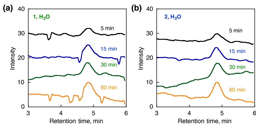
Figure S2. GC charts of CO 2 evolution in the catalytic water oxidation with (a) 1 (12.5 μM) and (b) 2 (12.5 μM) by CAN (125 mM) in a non-buffered aqueous solution (2.0 mL).
