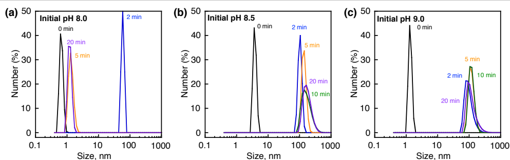
Figure 19. Particle size distribution determined by DLS measurements at initial pH (a) 8.0, (b) 8.5, and (c) 9.0 in borate buffer solutions containing 1 (5.0 \mu\text{M} ), Na_2S_2O_8 (5.0 mM) and [Ru(bpy)_3]SO_4 (0.25 mM) at the irradiation times of 2.0 min (blue line), 5.0 min (orange line), 10 min (green line), and 20 min (purple line). The black line shows the particle size distribution in the absence of 1 at 0 min.
