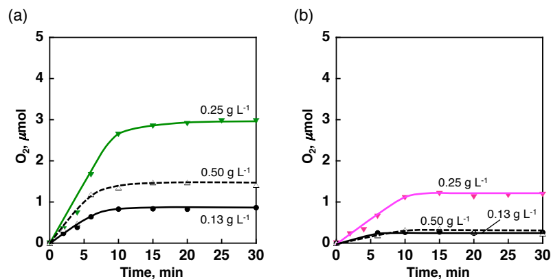
Figure 9. Time courses of oxygen evolution in the photocatalytic water oxidation with [\text{Ru}(\text{bpy})_3](\text{ClO}_4)_2 ( 0.25 \text{ mM} ), \text{Na}_2\text{S}_2\text{O}_8 ( 5.0 \text{ mM} ) and different concentrations ( 0.13 \text{ g L}^{-1} , 0.25 \text{ g L}^{-1} and 0.50 \text{ g L}^{-1} , green) of a cobalt-based catalyst (a) \text{NdCoO}_3 and (b) \text{YCoO}_3 . [photoirradiation ( \lambda > 420 \text{ nm} ) of a phosphate buffer solution ( 2.0 \text{ mL} ) at \text{pH } 7 ].
