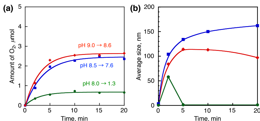
Figure 18. Time courses of O_2 evolution under photoirradiation ( \lambda > 420 nm) of a borate buffer solution (0.10 M, 2.0 mL) containing Na_2S_2O_8 (5.0 mM), [Ru(bpy)_3]SO_4 (0.25 mM), and 1 (5.0 \mu\text{M} ) at different initial pH conditions (green circles: pH 8.0, blue squares: pH 8.5, red rhombi: pH 9.0). (b) Time courses of average particle size formed in the photocatalytic reaction. See Figure 19 for particle size distribution determined by dynamic light scattering (DLS) measurements.
