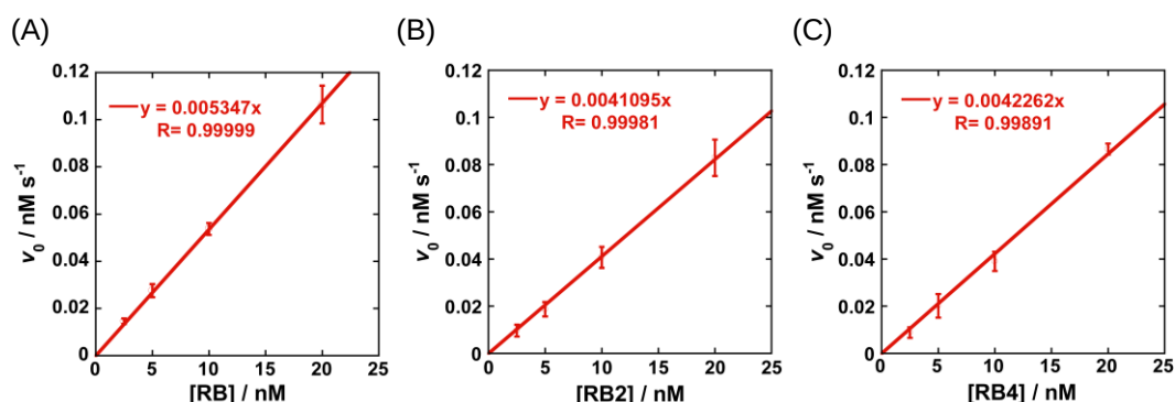
Figure 2-5. Kinetic study of (A) RB , (B) RB2 , and (C) RB4 . Plot of initial labeling reaction rate v_0 versus probe concentration. [BL-tag] = 100 nM.
