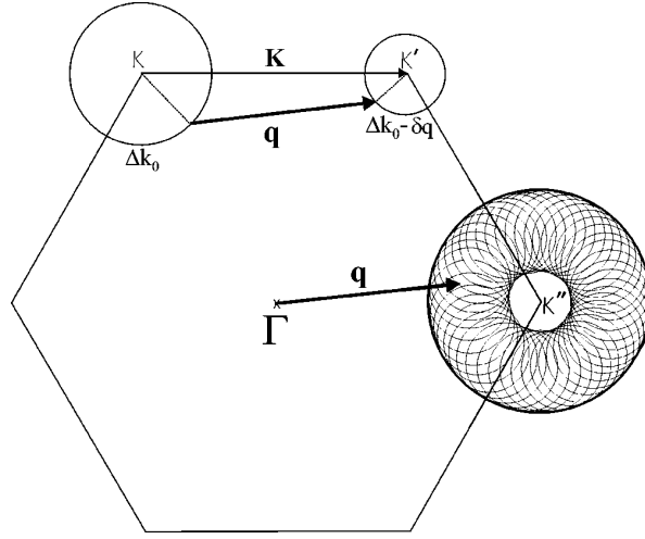
Fig. 14 | One of the possible double-resonance (DR) Stokes Raman processes involving the emission of a phonon with wave vector \mathbf{q} . The set of all phonon wave vectors \mathbf{q} which are related to transitions from points on the two circles around K and K' gives rise to the collection of small circles around the K'' point. Note that this collection of circles is confined to a region between the two circles with radii \Delta q and 2\Delta k_0 - \Delta q . The differences of the radii of the circles around K and K' and thus the radius of the inner circle around K'' were artificially enlarged for clarity [21].
