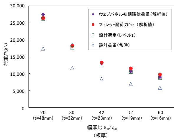
(c) SM570, 突出率 20%
