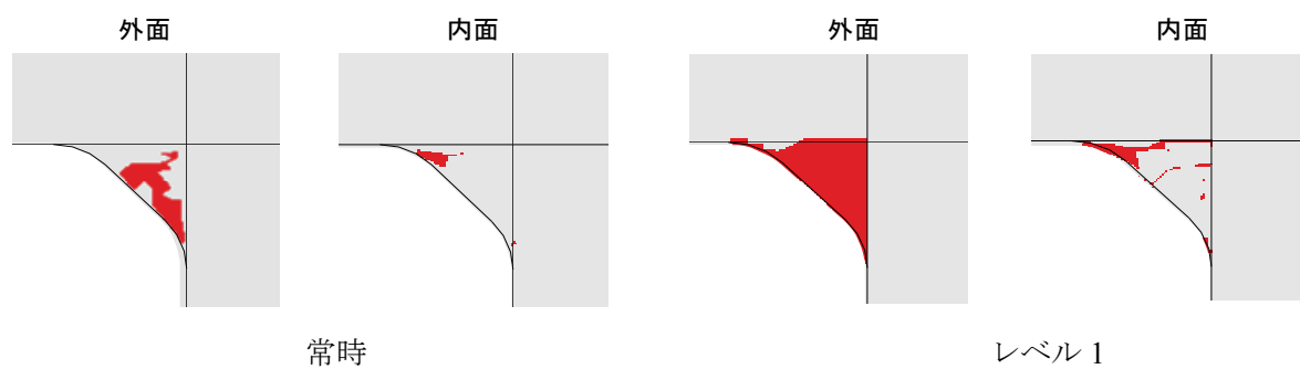
(c) CASE19 (板厚 19mm)
