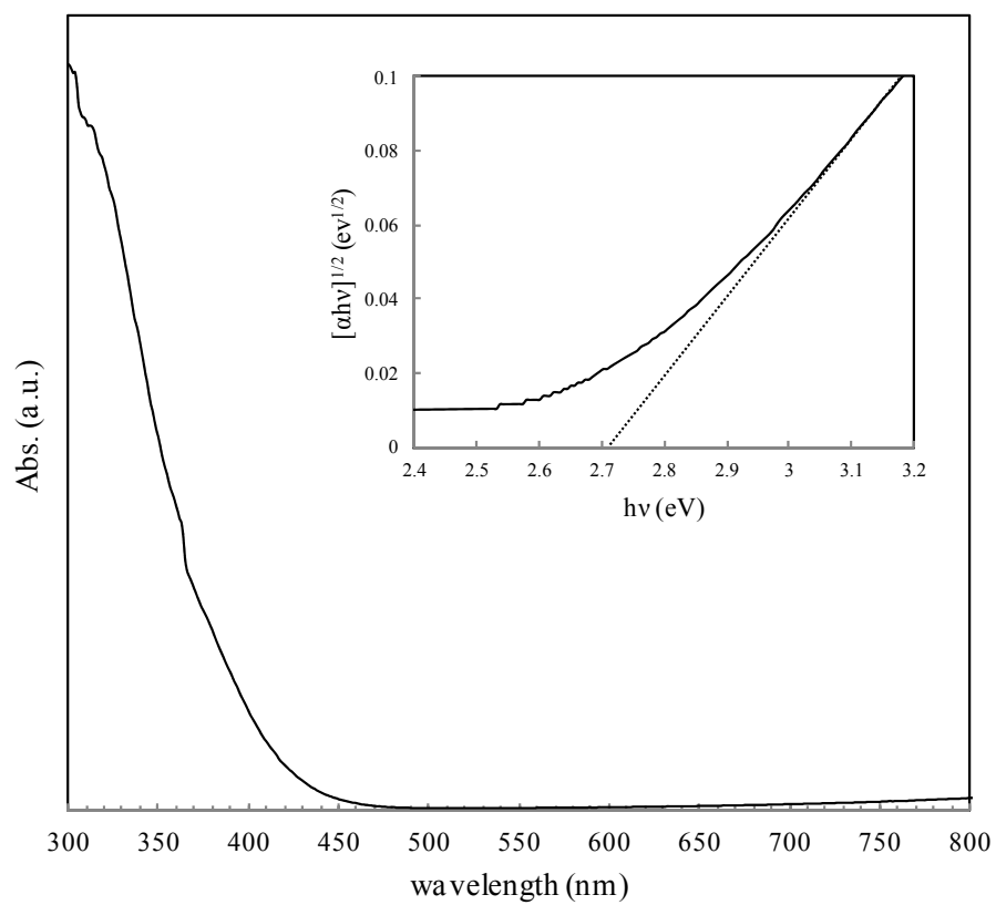
Fig. 3.8 Absorption spectrum of hexagonal \text{WO}_3 nanoneedles. The inset shows the plot of (\alpha h\nu)^{1/2} versus h\nu .
