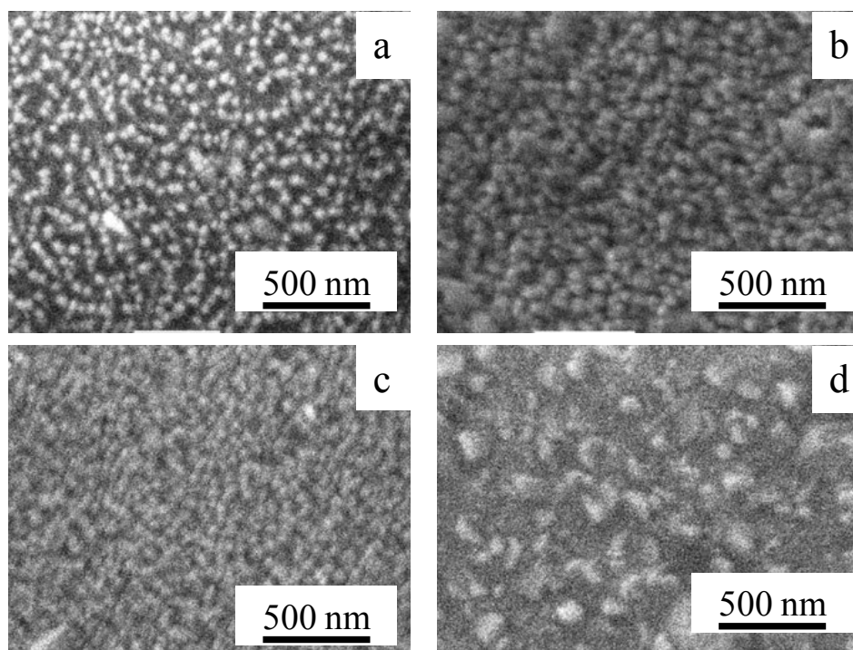
Fig. 5.4 SEM micrographs of \text{WO}_3 thin films deposited at pH 2, 0.1 M of \text{W}^+ using different current densities of : (a) 0.5 \text{ mA/cm}^2 , (b) 0.75 \text{ mA/cm}^2 , (c) 1 \text{ mA/cm}^2 and (d) 1.5 \text{ mA/cm}^2 .
