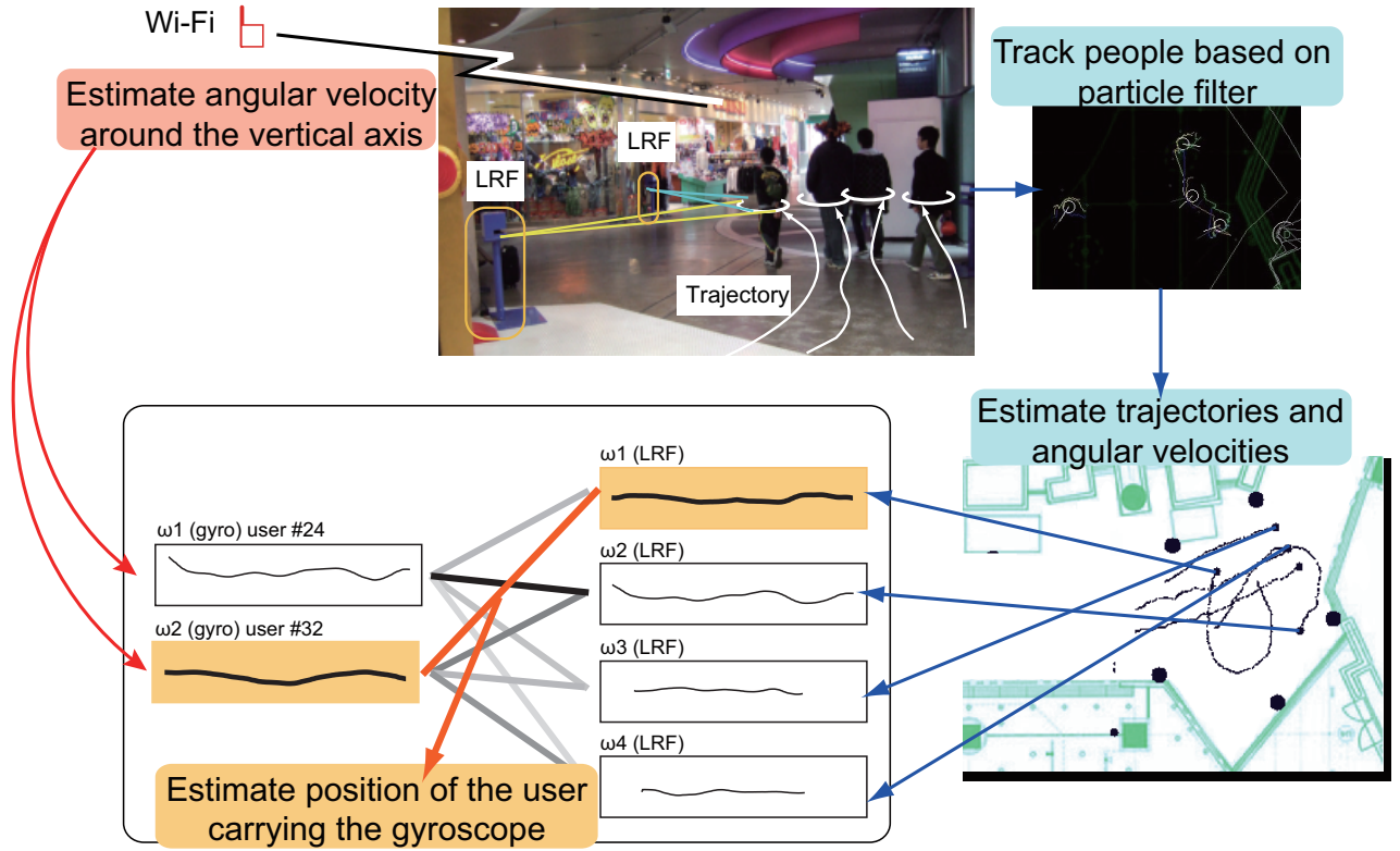
Figure 4.4 System overview
