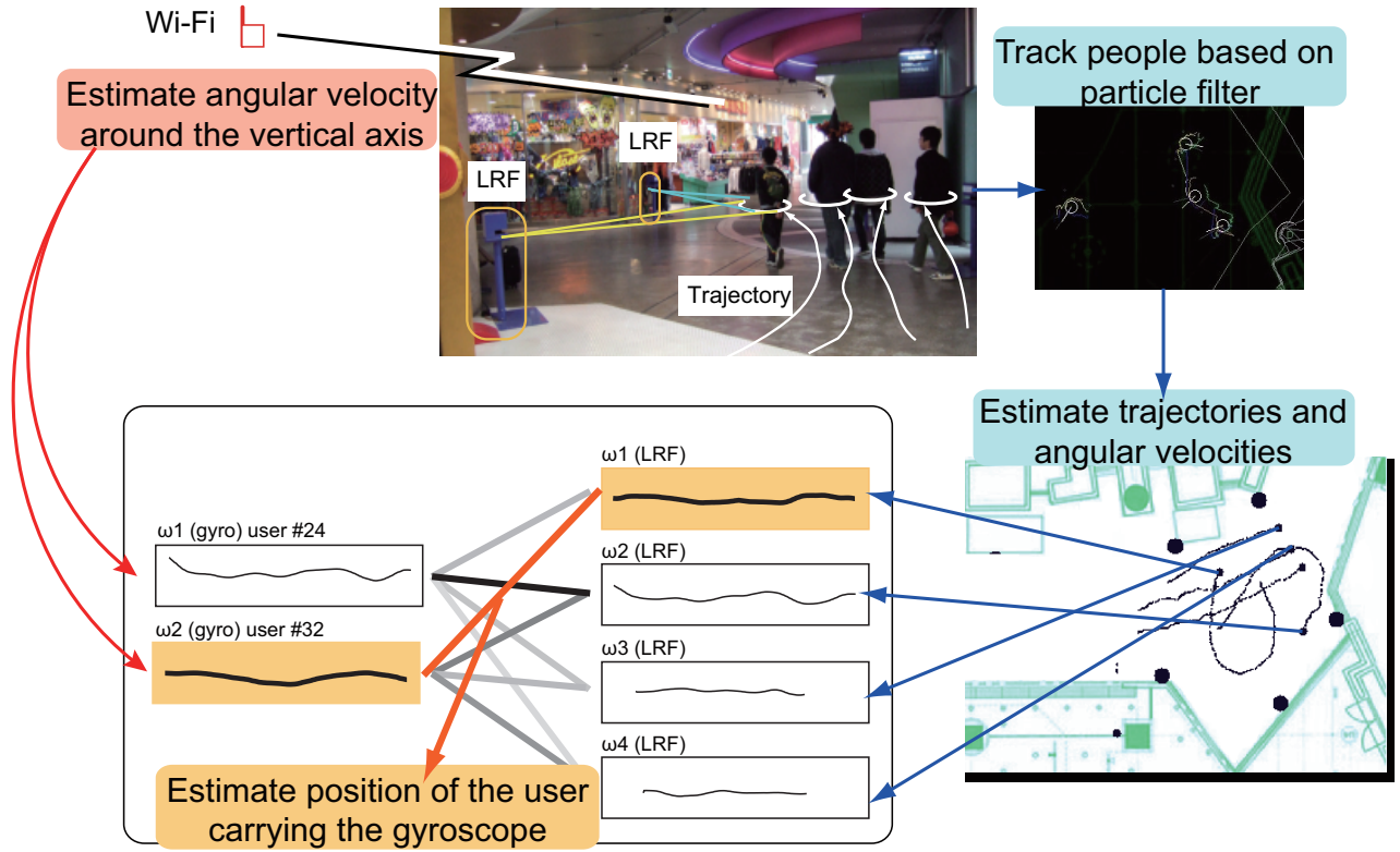
Figure 4.4 System overview
