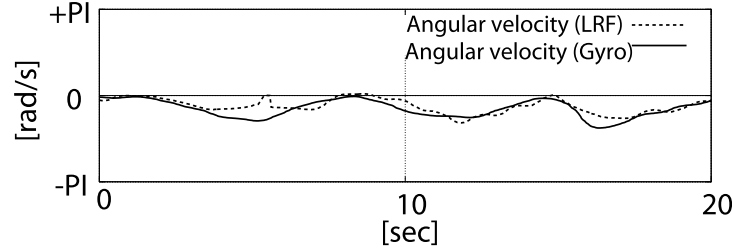
c) Angular velocity estimates for the person: they are very similar.
