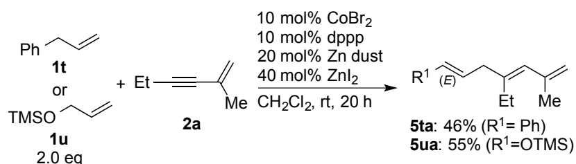
Scheme 4.5. Cobalt-catalyzed 1,2-hydrovinylolation of a 1,3-enyne with alkenes
