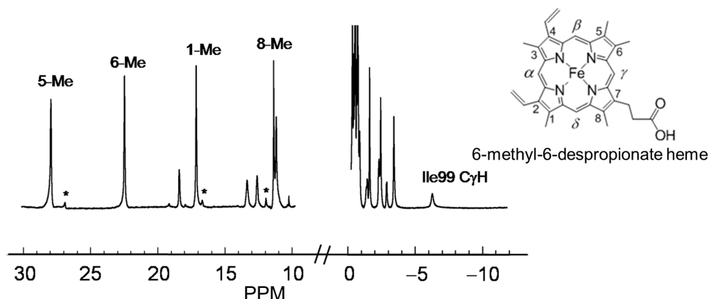
Figure 1-8. ^1\text{H} NMR spectrum of cyanomet Mb(H64D) mutant reconstituted with 6-methyl-6-despropionate heme in 10 mM KPi D _2 O buffer (pD = 7.4) at 25 ^{\circ}\text{C} . The peaks with an asterisk are assignable to the heme methyl protons accommodated in the reversed orientation.
