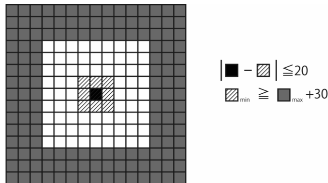
Fig.4-3. Pixels searched for detection of optical point (1 block = 1 pixel)
