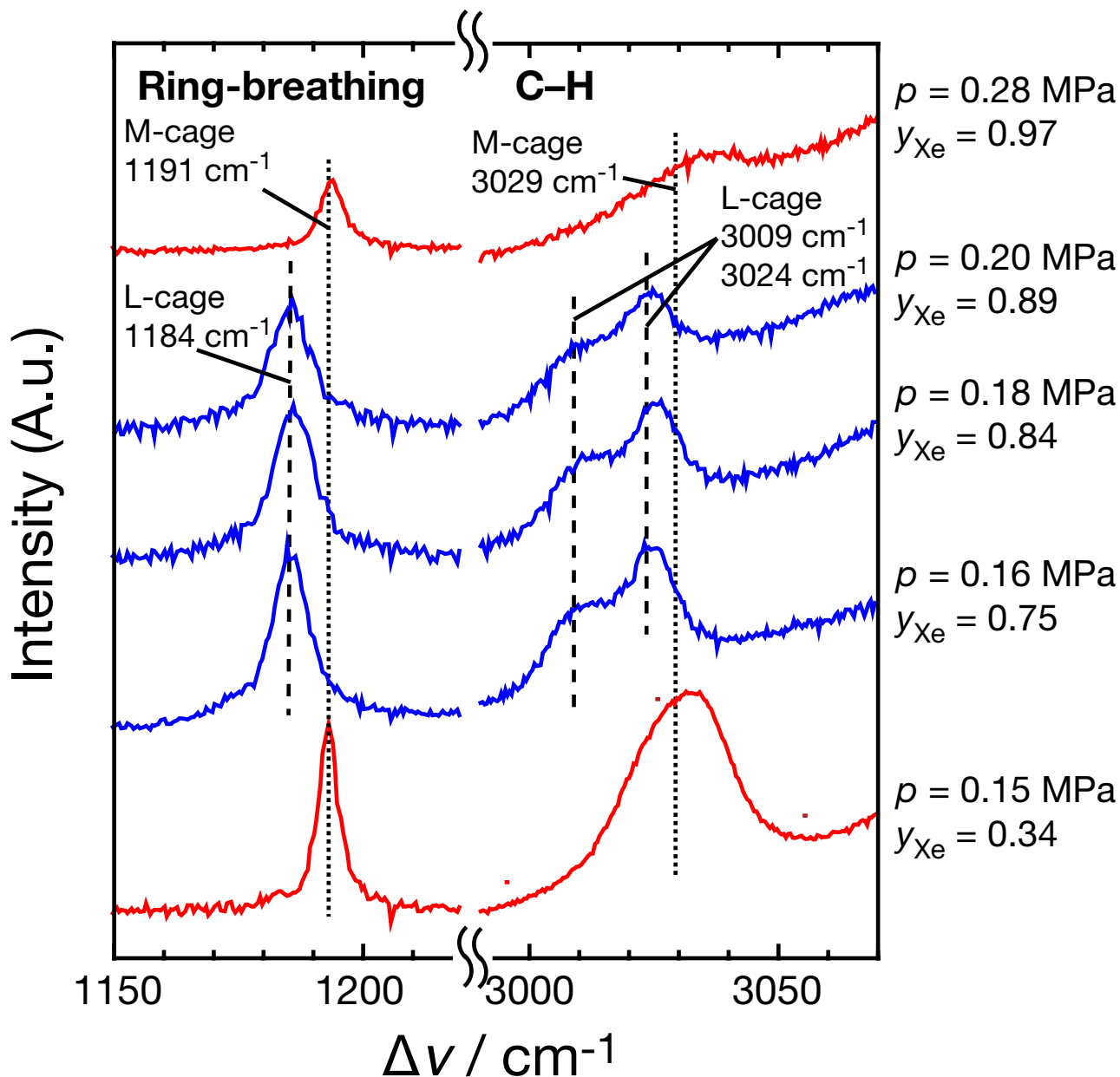
Figure II-5-3. Raman spectra corresponding to the ring-breathing ( \Delta\nu = 1190 cm -1 ) and C-H stretching vibration ( \Delta\nu = 3000 – 3040 cm -1 ) modes of c -C 3 H 6 in the Xe+ c -C 3 H 6 mixed-gas hydrate at T = 279.15 K. The dotted and broken lines correspond to the Raman shifts in the s-I and s-II Xe+ c -C 3 H 6 mixed-gas hydrates, respectively.
