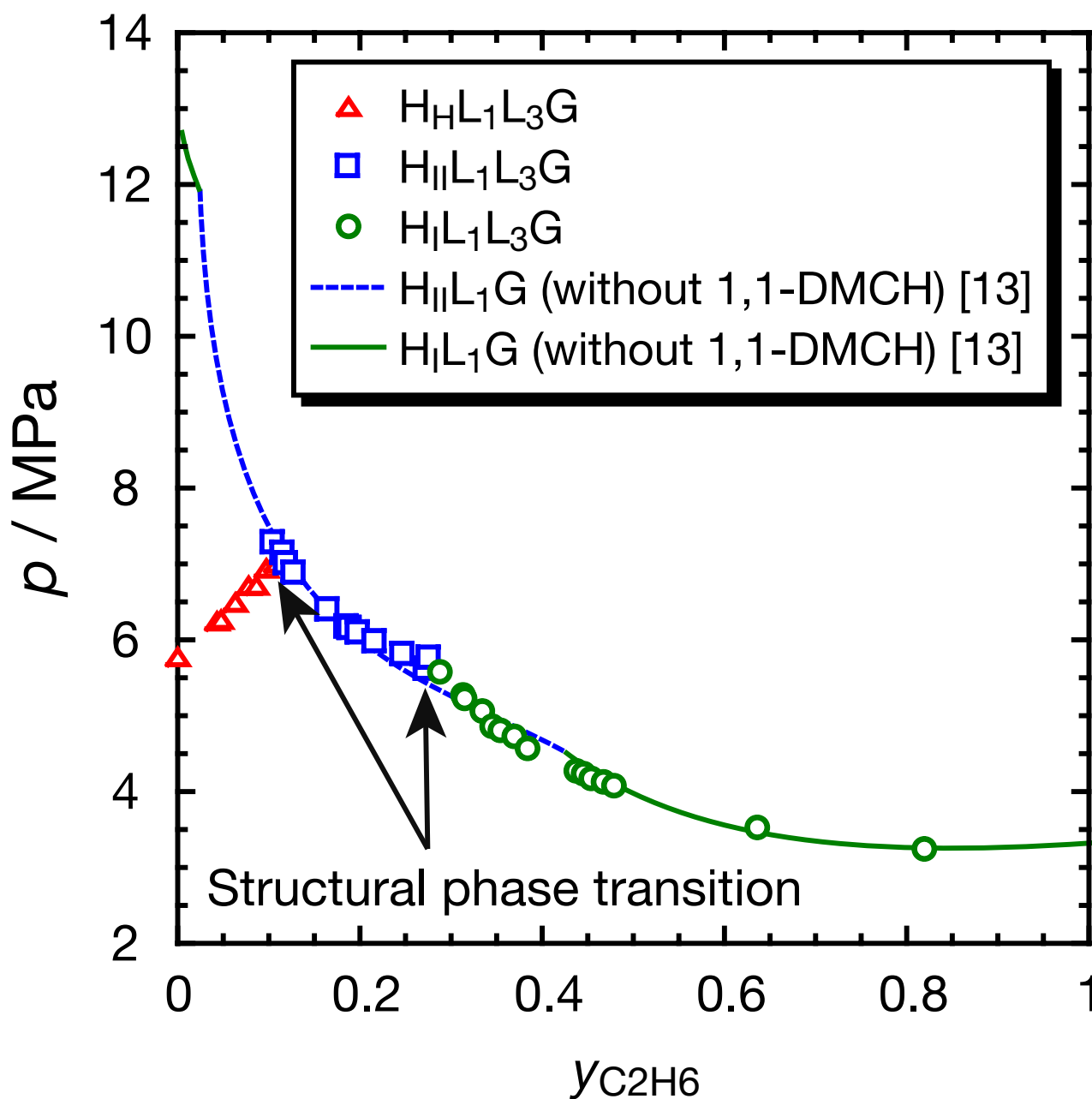
Figure III-4-2. Four-phase ( \text{H}_\text{I}\text{L}_1\text{L}_3\text{G} ) equilibrium pressure-composition projection for the \text{CH}_4+\text{C}_2\text{H}_6+1,1\text{-DMCH}+\text{water} system and three-phase ( \text{H}_\text{I}\text{L}_1\text{G} ) equilibrium pressure-composition projection for the \text{CH}_4+\text{C}_2\text{H}_6+\text{water} system [13] at T = 288.15\text{ K} .
