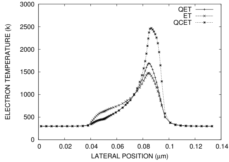
Figure 5.6: Lateral profiles of electron temperature distributions calculated by QET, ET, and QCET models at the same drain bias of V_d=0.8\text{V} and the same gate bias of V_g=1.2\text{V} .
