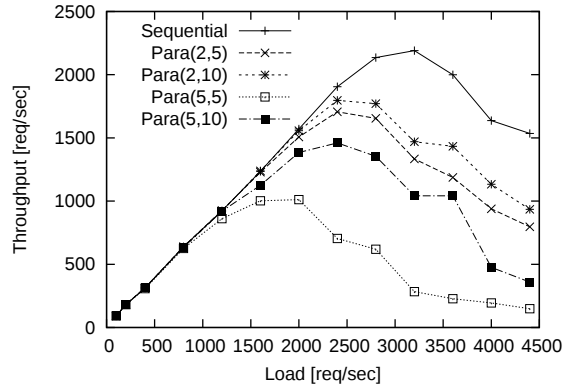
(a) Throughput
