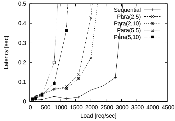
(b) Latency
