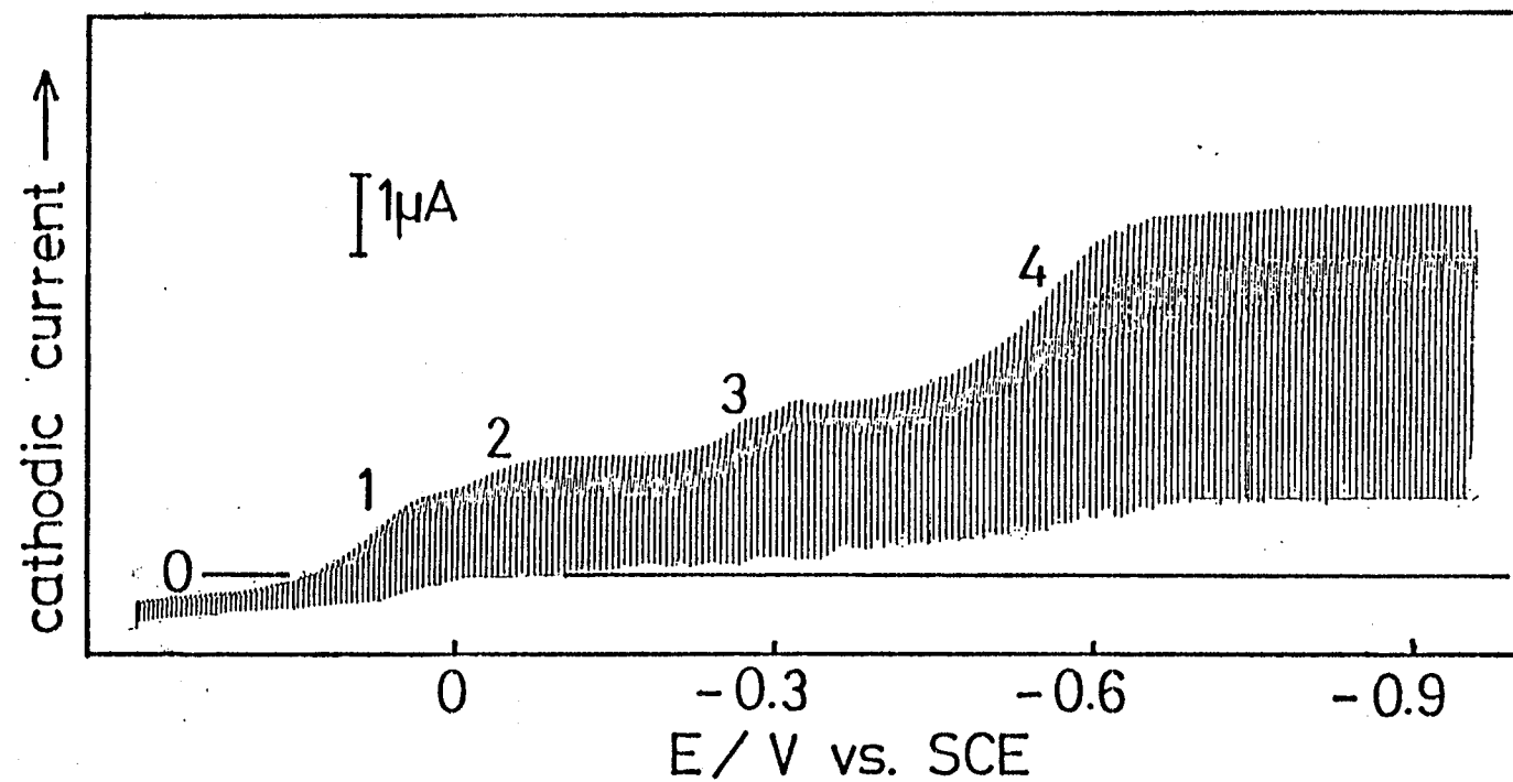
Fig.II-1. Polarogram of 0.5mM Mo(VI) in 0.1M H_2SO_4 .
