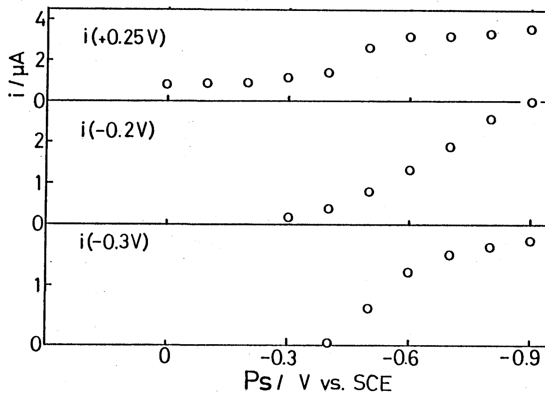
Fig.V-4. Dependence of the anodic peak current on the switching potential ( scan rate: 0.1Vs^{-1} ).
