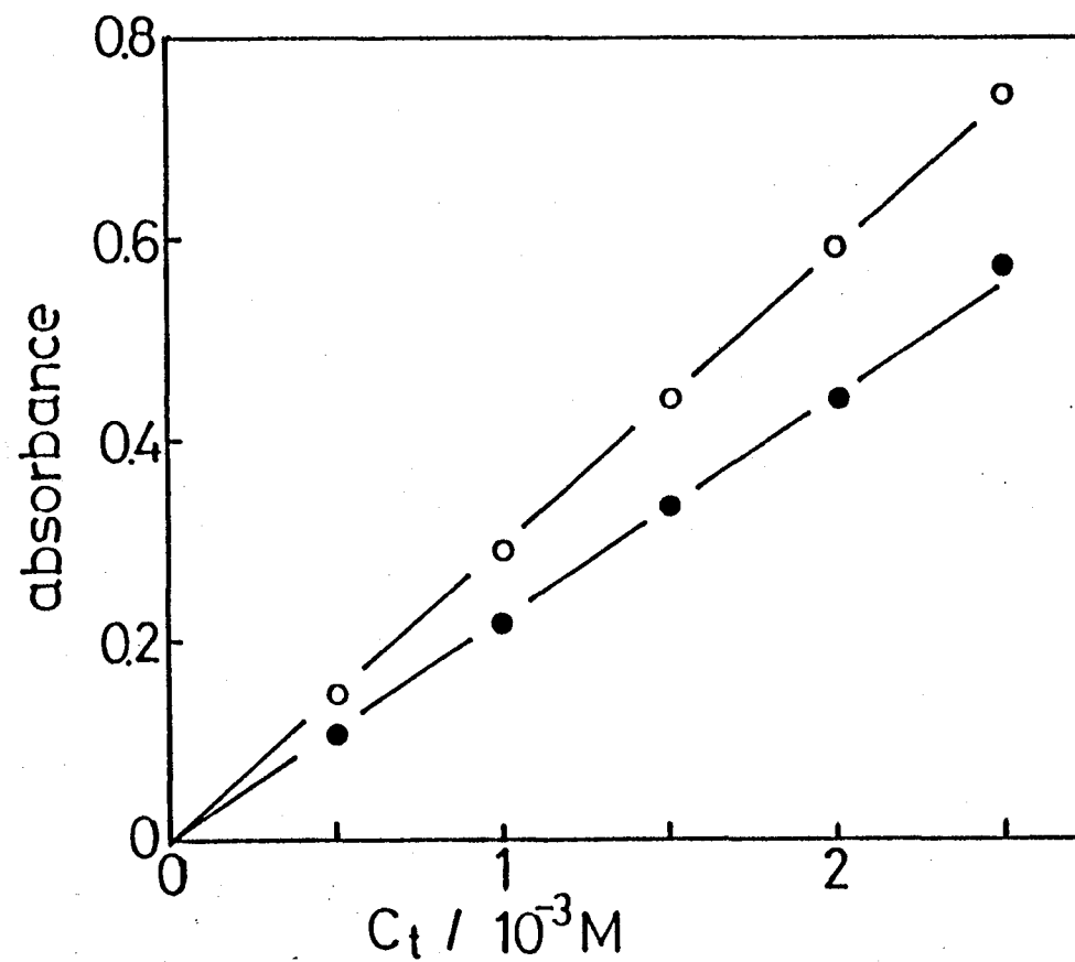
Fig.IV-5. Dependence of A_{407} on C_t in 7.5M (●) and 8M (O) H_2SO_4 .
