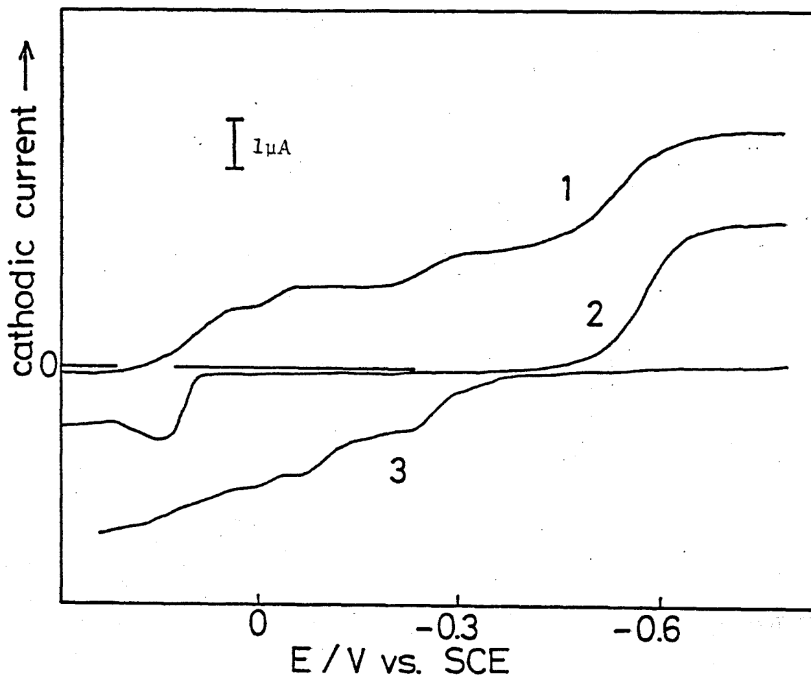
Fig.II-7. Polarograms of Mo solutions in 0.1M H_2SO_4 , (1) 0.5mM Mo(VI); (2) after CPE at +0.03V vs. SCE on (1); (3) after CPE at -0.70V vs. SCE on (2).
