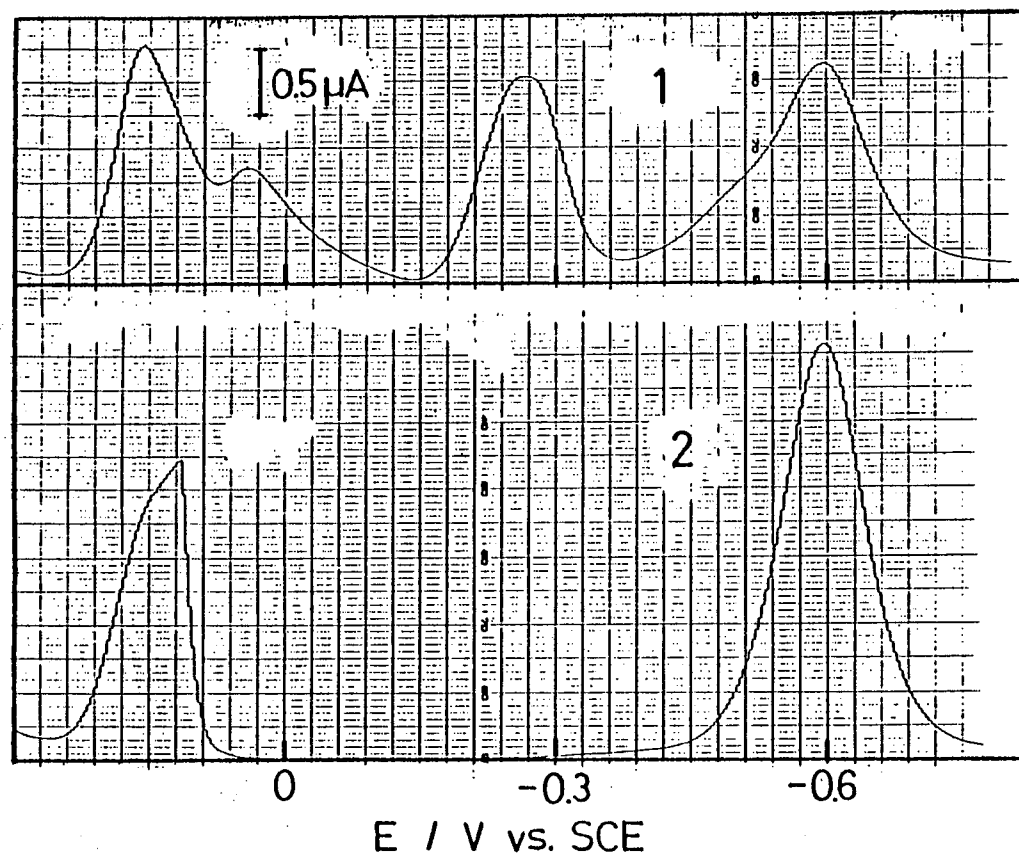
Fig.V-10. DP polarogram in 0.1\text{M H}_2\text{SO}_4 : (1) 0.5\text{mM Mo(VI)} ; (2) 0.5\text{mM Mo(V)} . t = 3.5\text{s}
