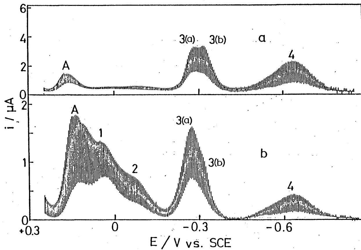
Fig.III-3. Ac polarogram of Mo(VI) in 0.1M H_2SO_4 ( 0° component ); C_{Mo(VI)} : (a) 2.0mM: (b) 0.5mM.
