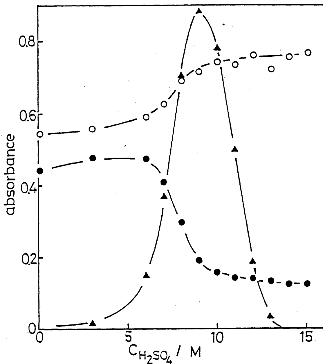
Fig.IV-4. Effect of the concentrations of \text{H}_2\text{SO}_4 on absorbances of 2.5 \times 10^{-4} \text{M} Mo(V) solution at 254nm (○), 293nm (●) and 407nm (▲). l = 1\text{cm}
