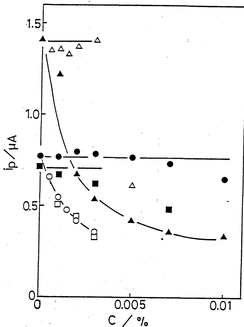
Fig.III-7. Dependence of peak heights on the concentration of surfactants ( C_{Mo(VI)} are as those in Fig.III-6 ). Sodium n-dodecylbenzenesulfonate ( anionic ): ( ○ ) peak 1; ( □ ) peak 2; ( △ ) peak 3. Dodecyltrimethylammonium chloride ( cationic ): ( ● ) peak 1; ( ■ ) peak 2; ( ▲ ) peak 3.
