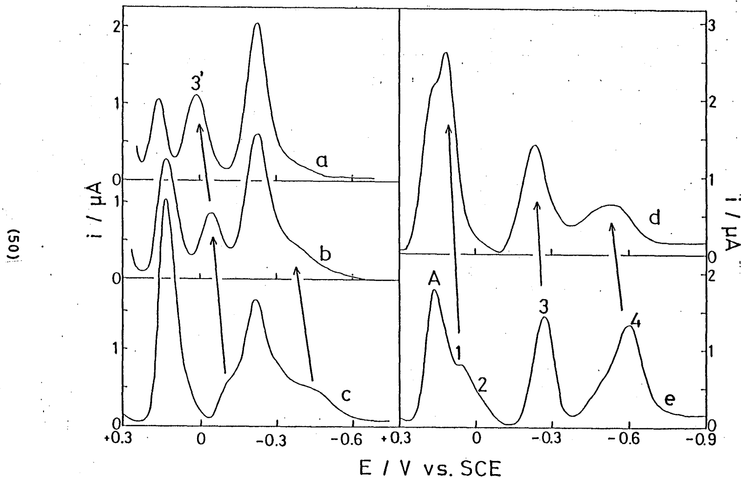
Fig.III-4. DP polarogram of 0.5mM Mo(VI) in various concentration of sulfuric acid; \text{CH}_2\text{SO}_4 : (a) 5M; (b) 3M; (c) 1M; (d) 0.3M; (e) 0.1M.
