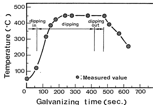
Fig. 2-7 Galvanizing thermal cycle obtained
