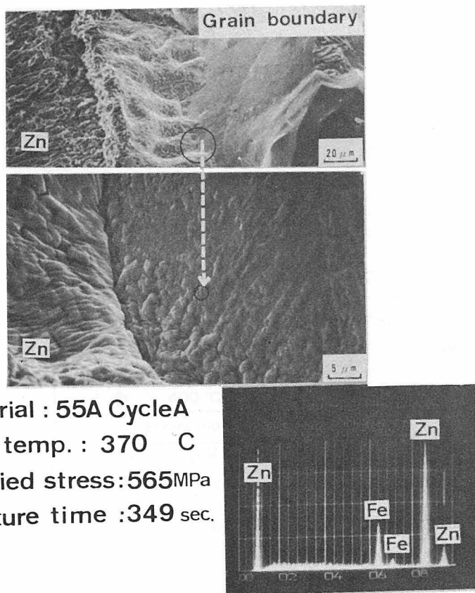
Fig. 3-14 Observation of Zn diffusion phenomena in grain boundary of steel
