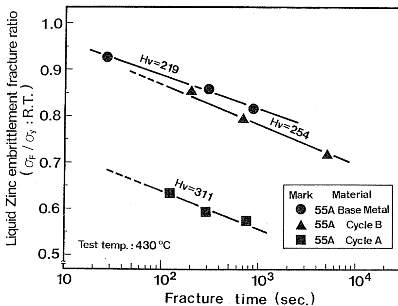
Fig. 3-20 Distributions of \sigma_F/\sigma_{y;R.T.} according to fracture time at 430°C
