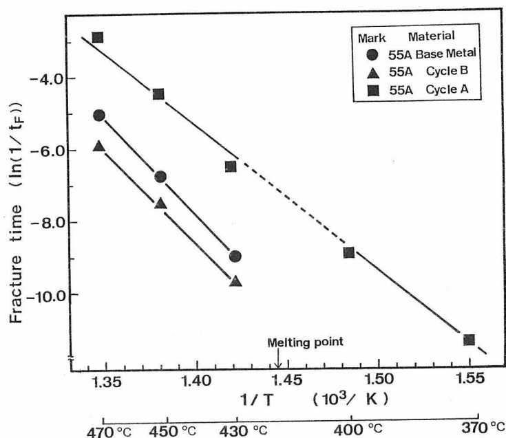
Fig. 3-13 Arrhenius plots of \ln(t_F)
