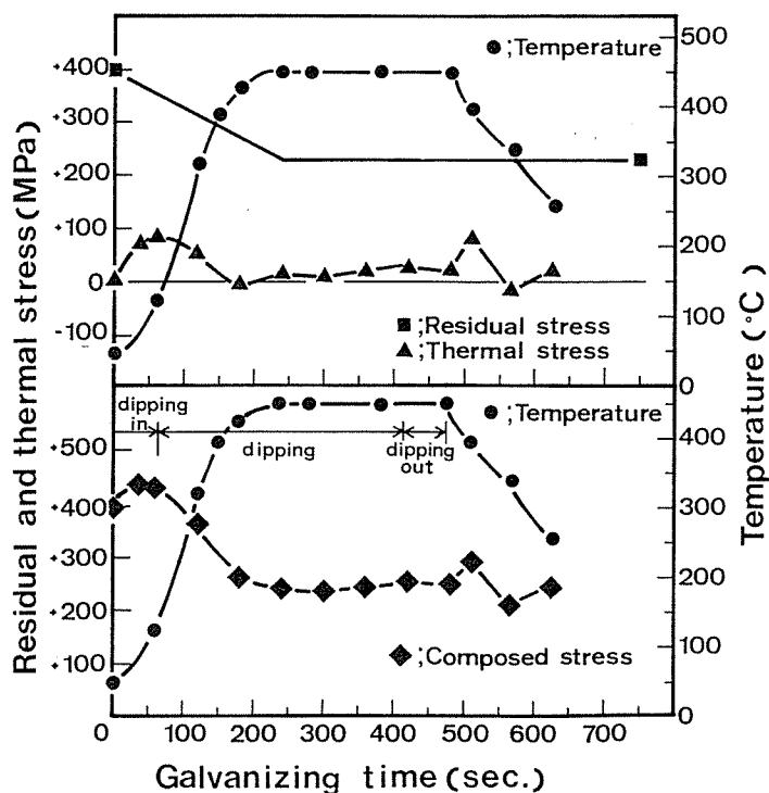
Fig. 2-12 Estimation of effective stress for LMEC during hot dip galvanizing
