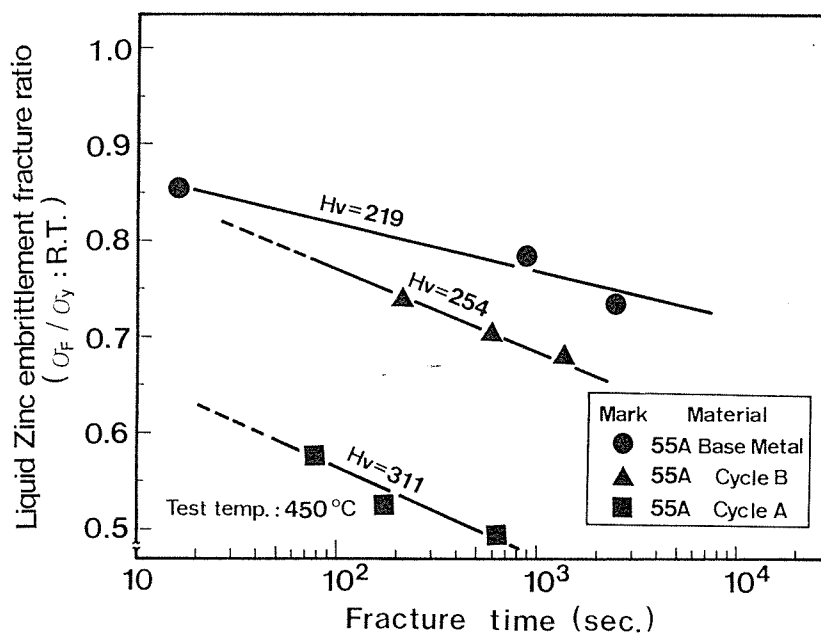
Fig. 3-21 Distributions of \sigma_F/\sigma_{y;R.T.} according to fracture time at 450°C
