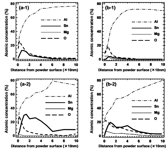
Fig.5 AES analysis results on as-received raw powder (-1) and heated to 823 in XPS analysis (-2). Mg content; 0% (a) and 1% (b).
