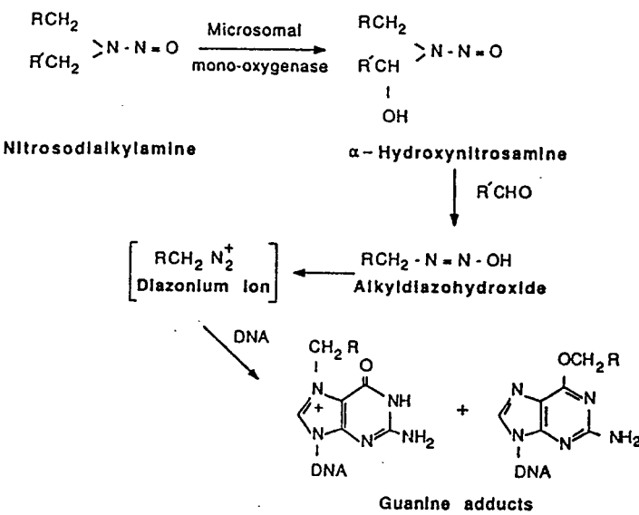
Fig. 2-1. Metabolic Activation of N-nitrosodialkylamines.
