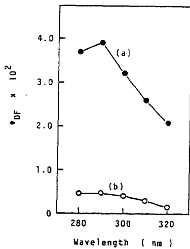
Fig.VI-2. Relationships between the quantum yield for the photodimerization of 6-cyanouracil and the wavelength of the irradiating monochromatic light in DMSO solution: (a) PMAO-6CNU; (b) 6CNU-M.
