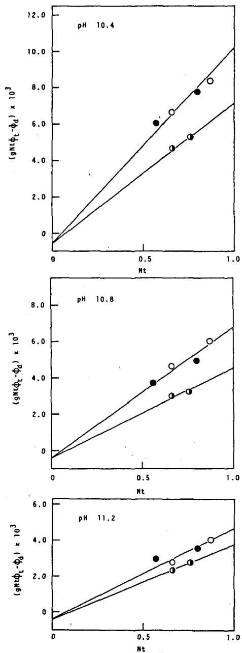
Fig.III-8. Relationships between (gNt\phi_t - \phi_d) and Nt values at each pH poly(Thy-L-lys)s (O); poly(Thy-D-lys)s (●); poly(Thy-DL-lys)s (◐).
