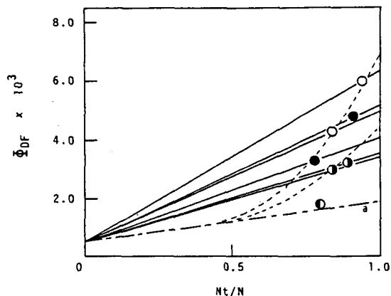
Fig.III-7. Relationship between quantum yield for the photodimerization ( \Phi_{DF} ) and Nt/N value at pH 10.8: poly(Thy-L-lys)s (O); poly(Thy-D-lys)s (●); poly(Thy-DL-lys)s (◐); oligo(Thy-L-lys) (◑). The line a was obtained from the data of the oligomers of ethyleneimine derivatives ( ref. 1 ).
