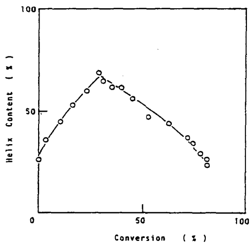
Fig.IV-6. The relationship between the conversion of thymine bases and the helix content of the polymer for poly(Thy-D-lys)-88 at pH 11.2. Photolysis with a glass filter
