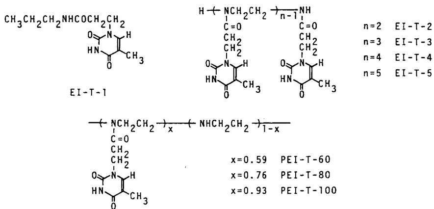
Fig.I-1. Thymine derivatives.
