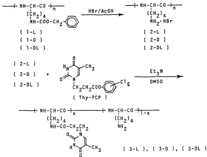
( Scheme III-1 )
