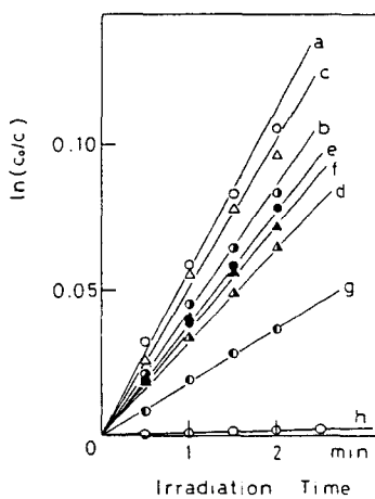
Fig.III-6. Photolysis of thymine base derivatives at pH 10.8: (a) poly(Thy-D-lys)-88; (b) poly(Thy-D-lys)-72; (c) poly(Thy-L-lys)-93; (d) poly(Thy-L-lys)-79; (e) poly(Thy-DL-lys)-85; (f) poly(Thy-DL-lys)-79; (g) oligo(Thy-L-lys); (h) T-M.
