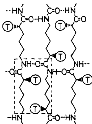
Fig.V-3. Anti-parallel \beta -sheet structure of isopoly(Thy-L-lys): ⊕ = Thymine Base.
