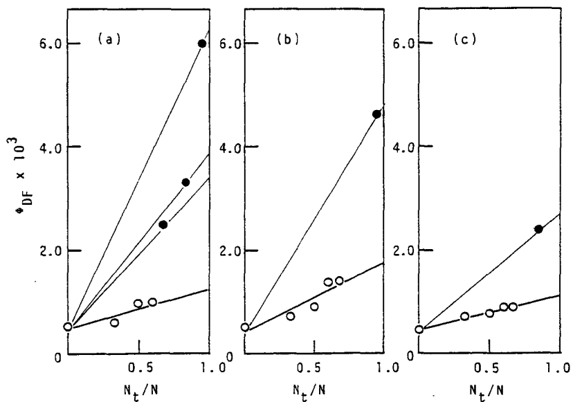
Fig.II-8. Relationships between quantum yields for the photodimerization of tyrosine bases ( \phi_{DF} ) and N_t/N values in aqueous solution at pH 11.3 for (a) EI-T-n and PEI-T-n; (b) EI-T- \beta Ala-n and PEI-T- \beta Ala; (c) EI-T- \alpha Ala-n and PEI-T- \alpha Ala: (O) Oligomers; (●) Copolymers.
