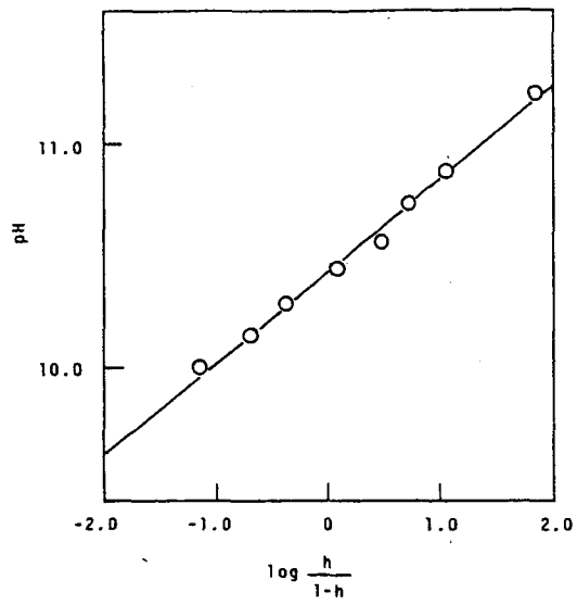
Fig.III-4. Relationship between pH and \log( h/1-h ) of poly(L-lysine)
