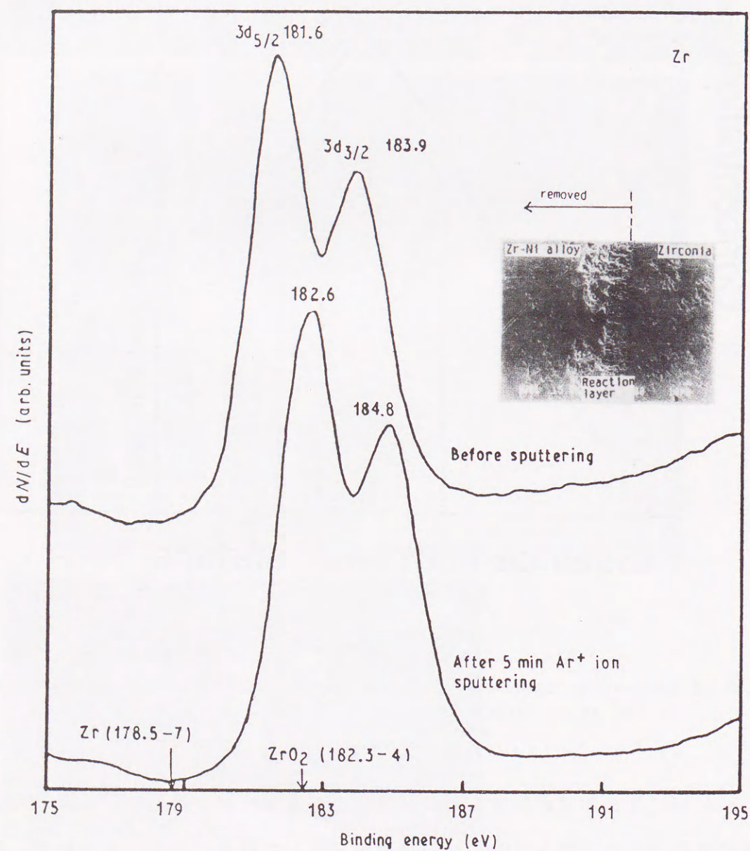
Fig. 4.13 X-ray photoelectron spectra of Zr_{3d} obtained from fracture surface of the joint (Zr-17Ni/1273K 1.8ks).
