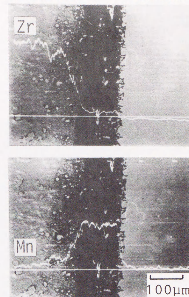
Fig. 3.10 Results of EDX line analysis obtained from the interface of the joint using borate solder (B7) joined at 1173K for 1.8ks.
