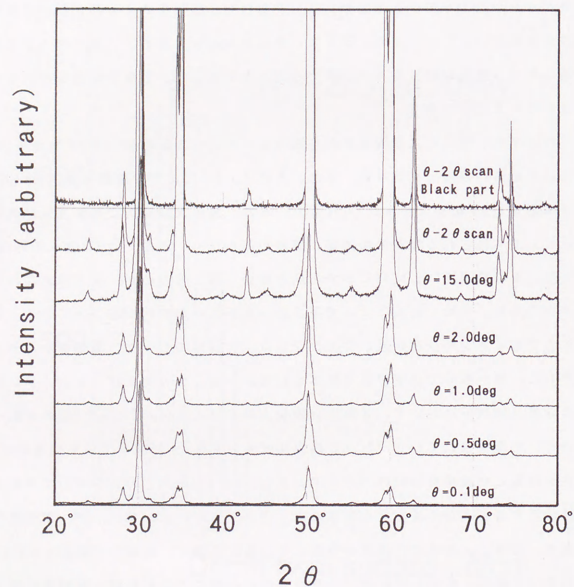
Fig. 5.18 X-ray diffraction patterns obtained from N + ions implanted PSZ.
