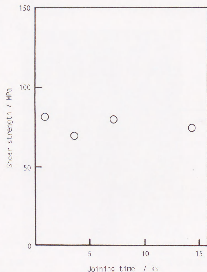
Fig. 3.6 Relation between shear strength of the joints and joining time. (Using silicate solders (S1) and joining at 1173K.)
