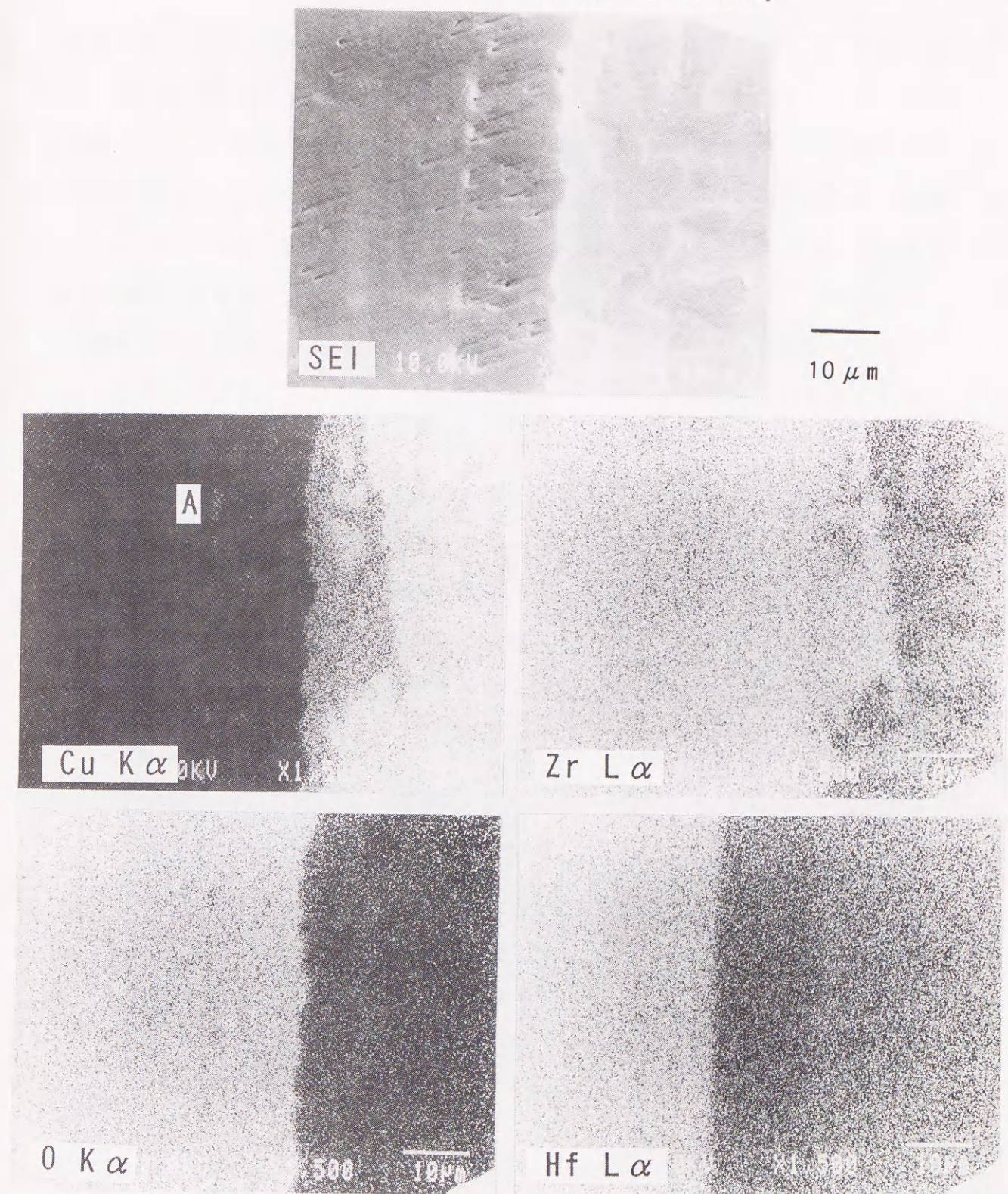
Fig. 5.24 Secondary electron image and X-ray images at N^+ ions implanted PSZ joint interface joined at 1273K.
