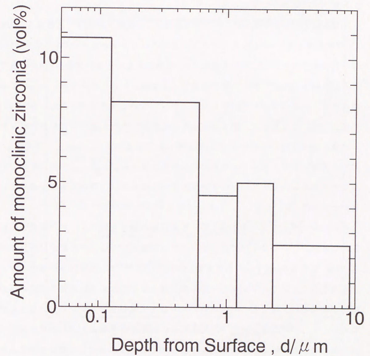
Fig. 5.19 Depth profiles of monoclinic phase zirconia obtained from N + ions implanted PSZ.
