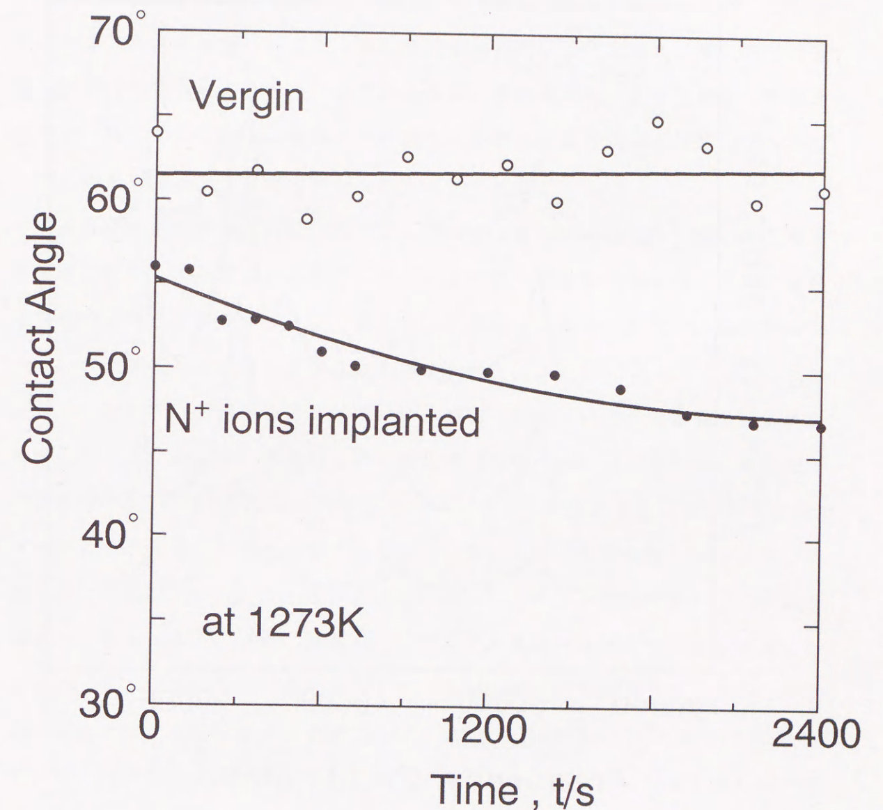
Fig. 5.22 Time dependence of the contact angle for Zr-47Cu alloy against virgin and N + ions implanted PSZ.
