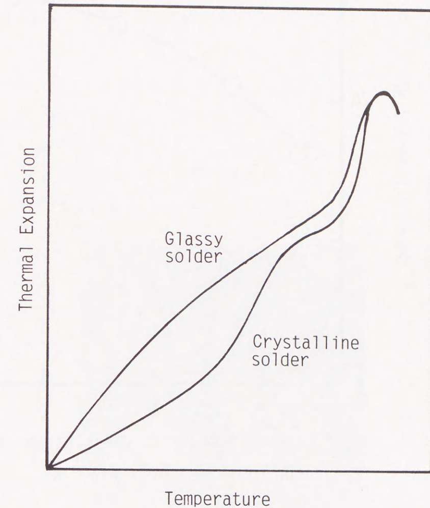
Fig.3.3 Thermal expansion curves of typical solders.
