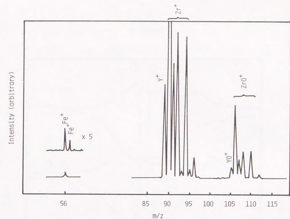
Fig. 2.7 Secondary ion mass spectrum obtained from the fracture surface of zirconia side of zirconia/carbon steel joint after sputtering for 100 min.
