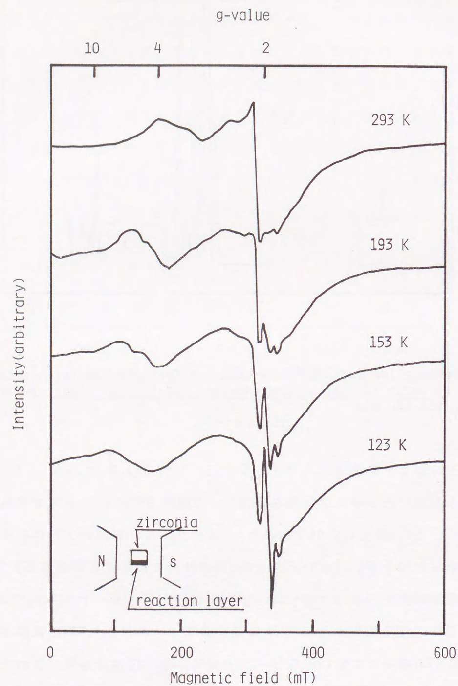
Fig. 2.8 ESR spectra obtained from zirconia after fractured. (Specimen zirconia was cut into the dimension of 2\text{mm} \times 2\text{mm} \times 8\text{mm} and located so that reacted surface of zirconia was parallel to magnetic field.)
