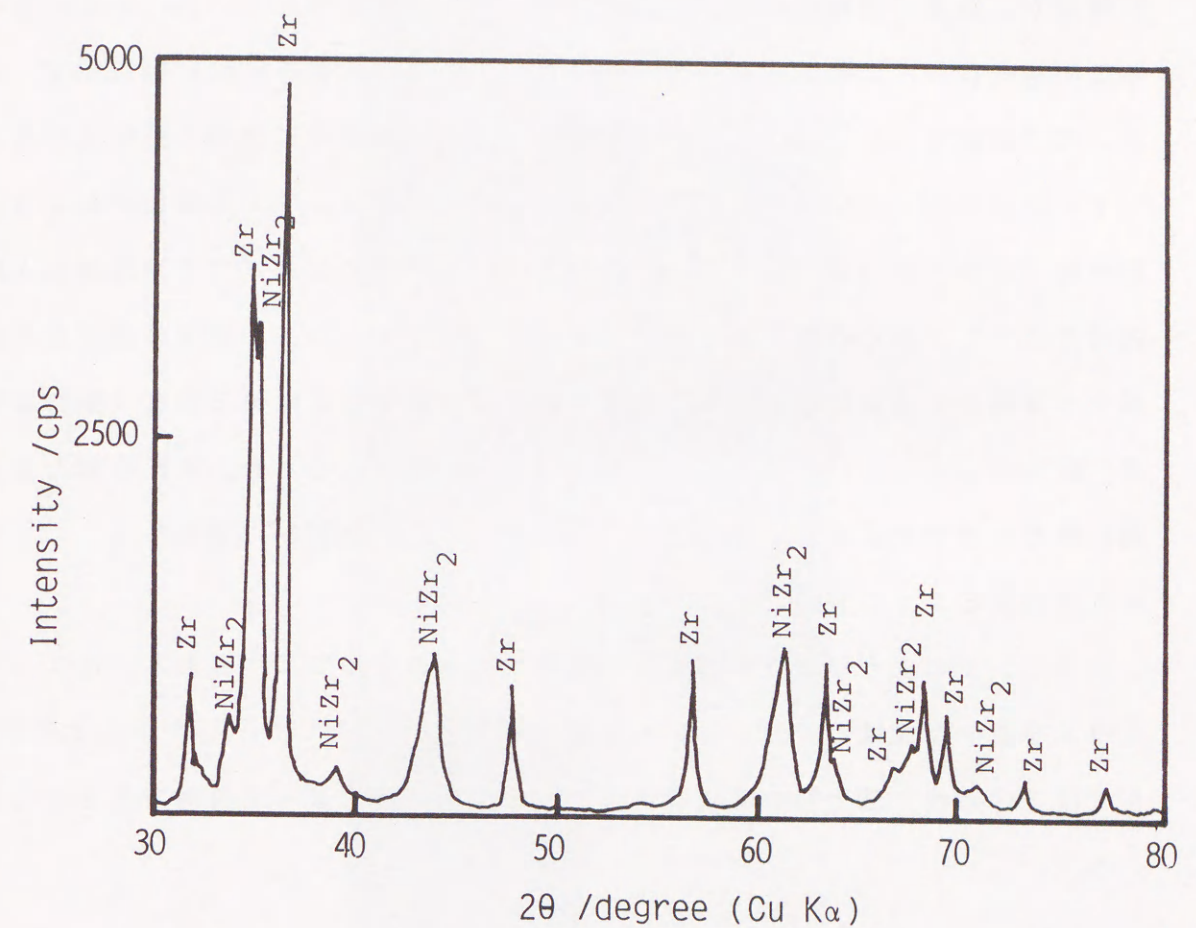
Fig. 4.8 X-ray diffraction pattern of Zr-17Ni alloy.
