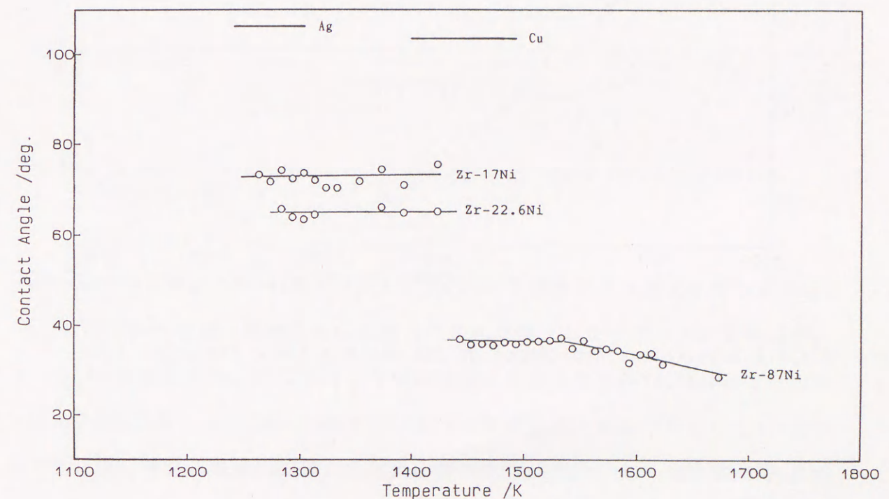
Fig. 4.4 Temperature dependance of the contact angle for Ag, Cu and Zr-Ni alloy against PSZ.
