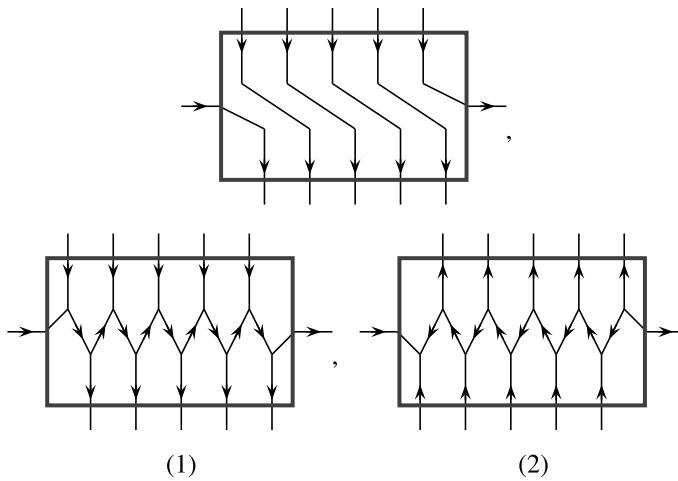
Fig. 9. Fillings for the boxes in equation (5).
