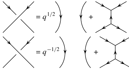
Fig. 17. Expansion of crossings for P_3(q) .
